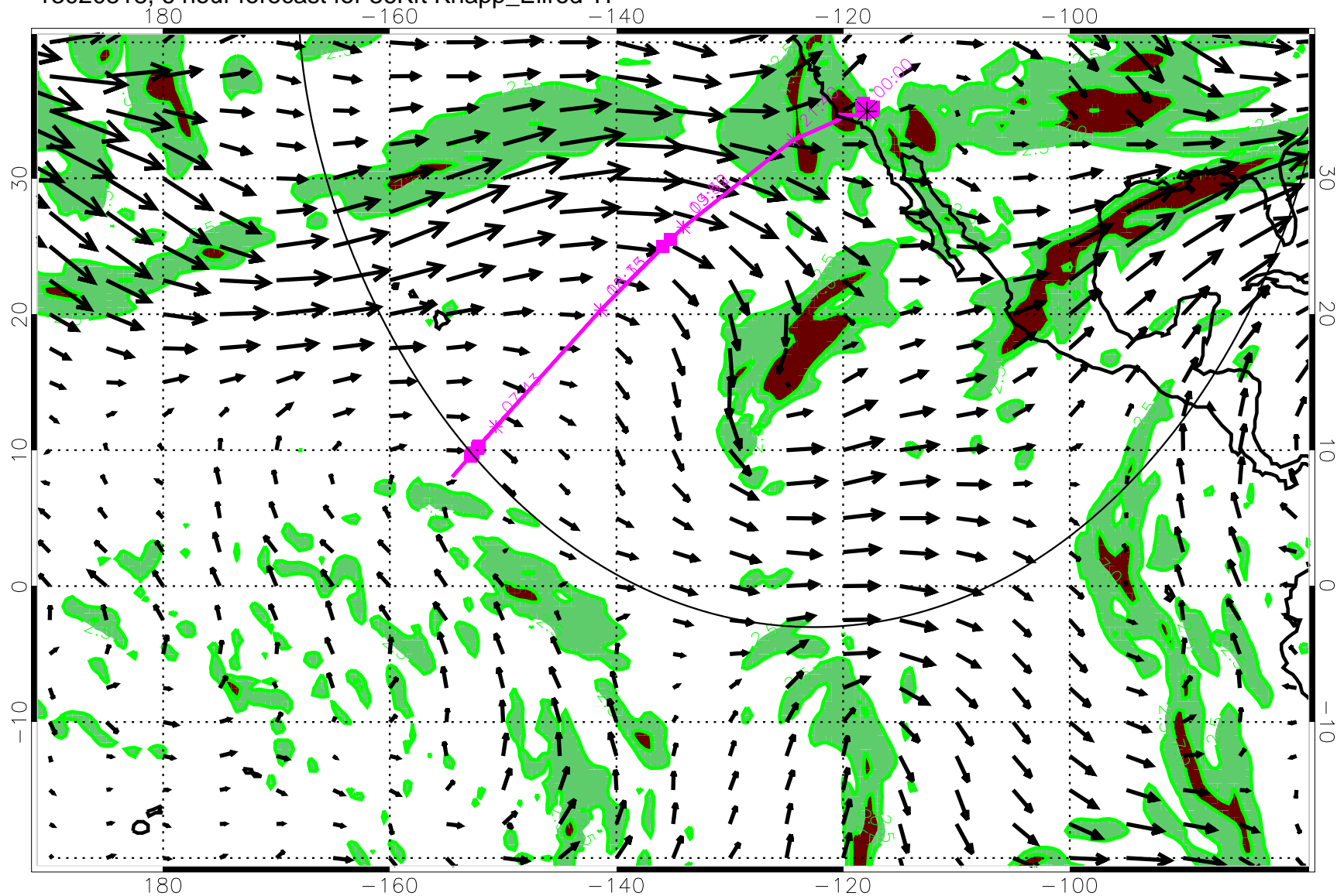
13020518, 6 hour forecast for 36Kft Knapp_Ellrod TI
