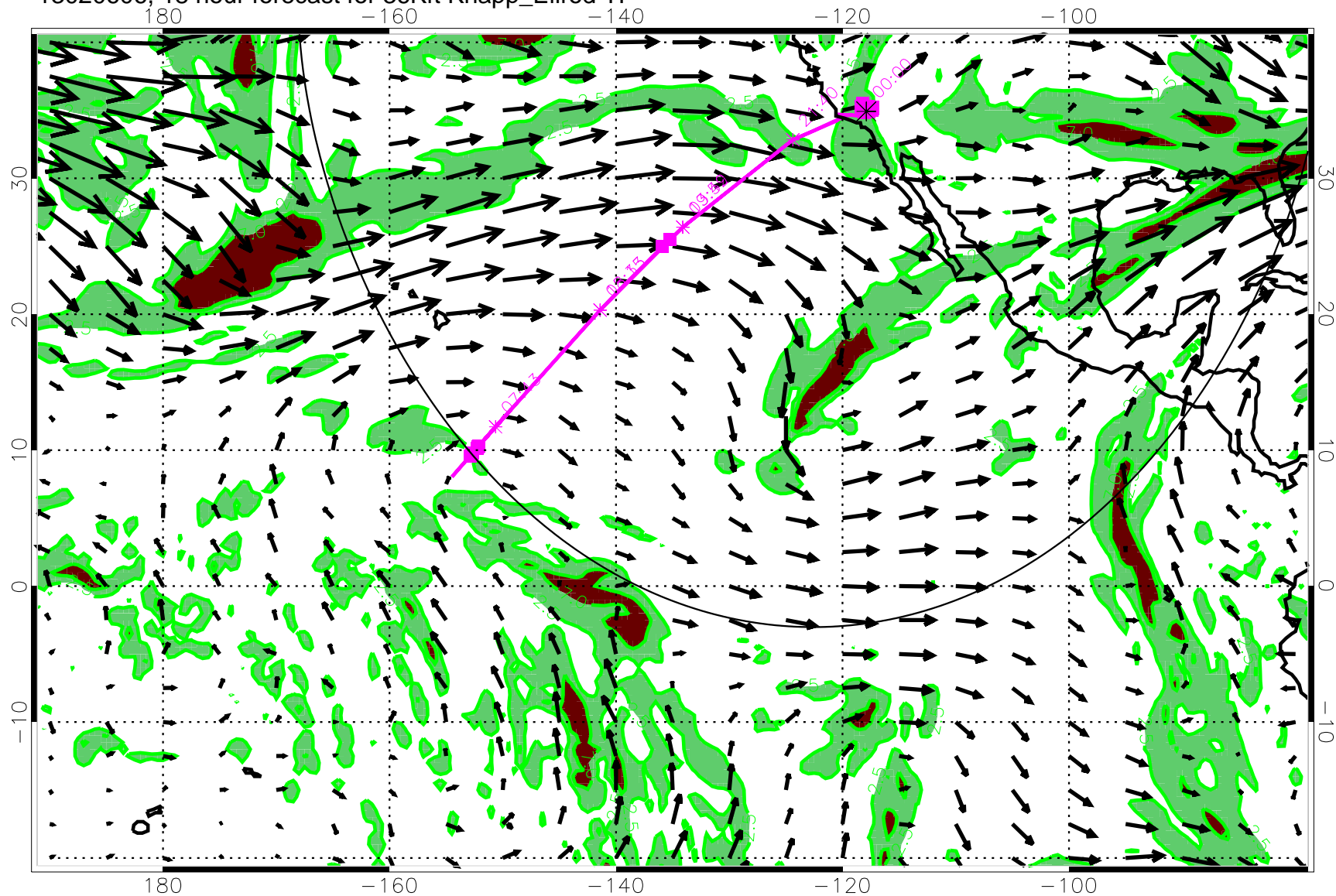
13020606, 18 hour forecast for 36Kft Knapp_Ellrod TI
