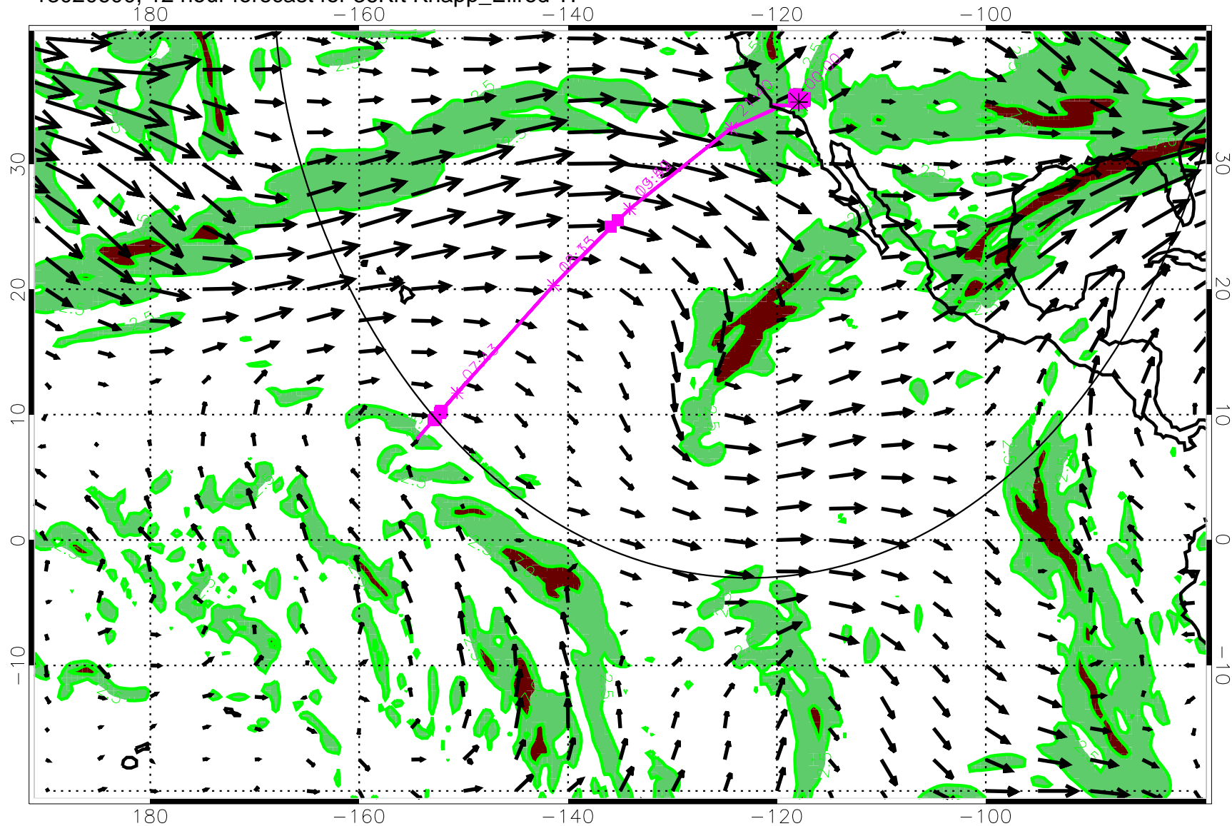
13020600, 12 hour forecast for 36Kft Knapp_Ellrod TI
