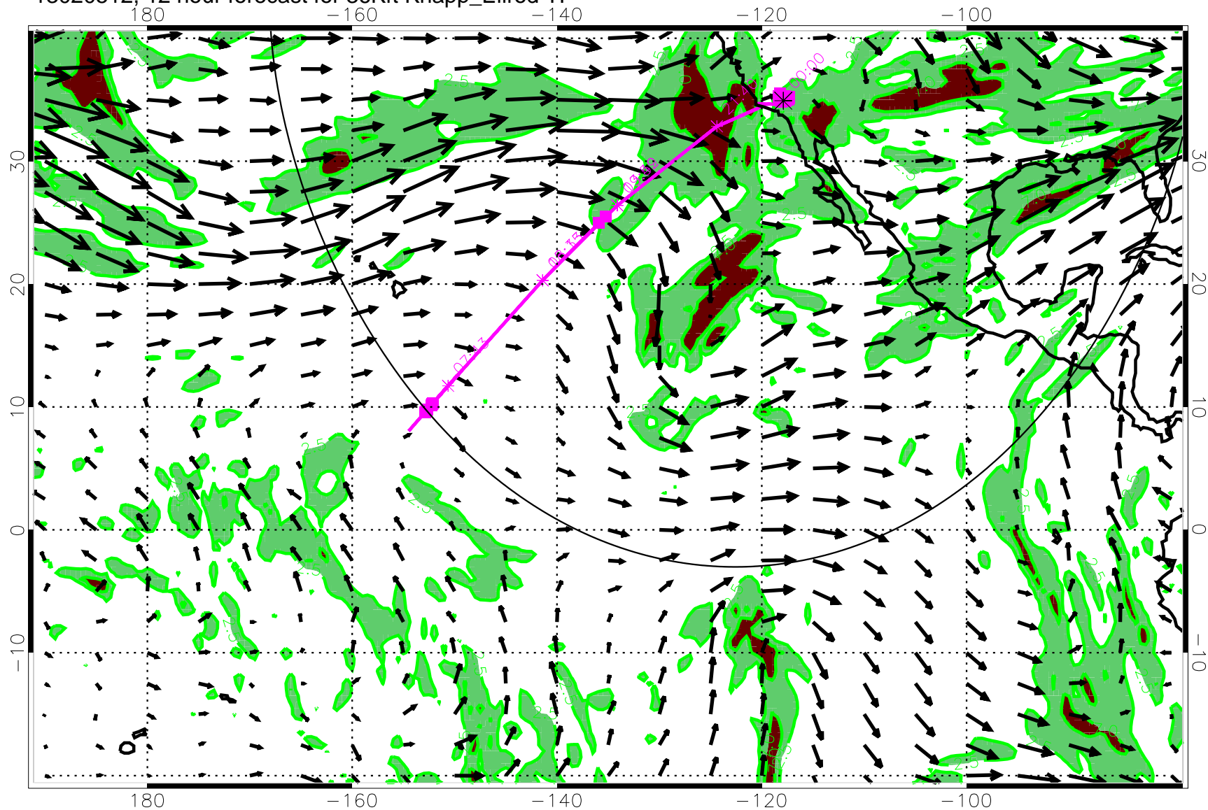
13020512, 12 hour forecast for 36Kft Knapp_Ellrod TI
