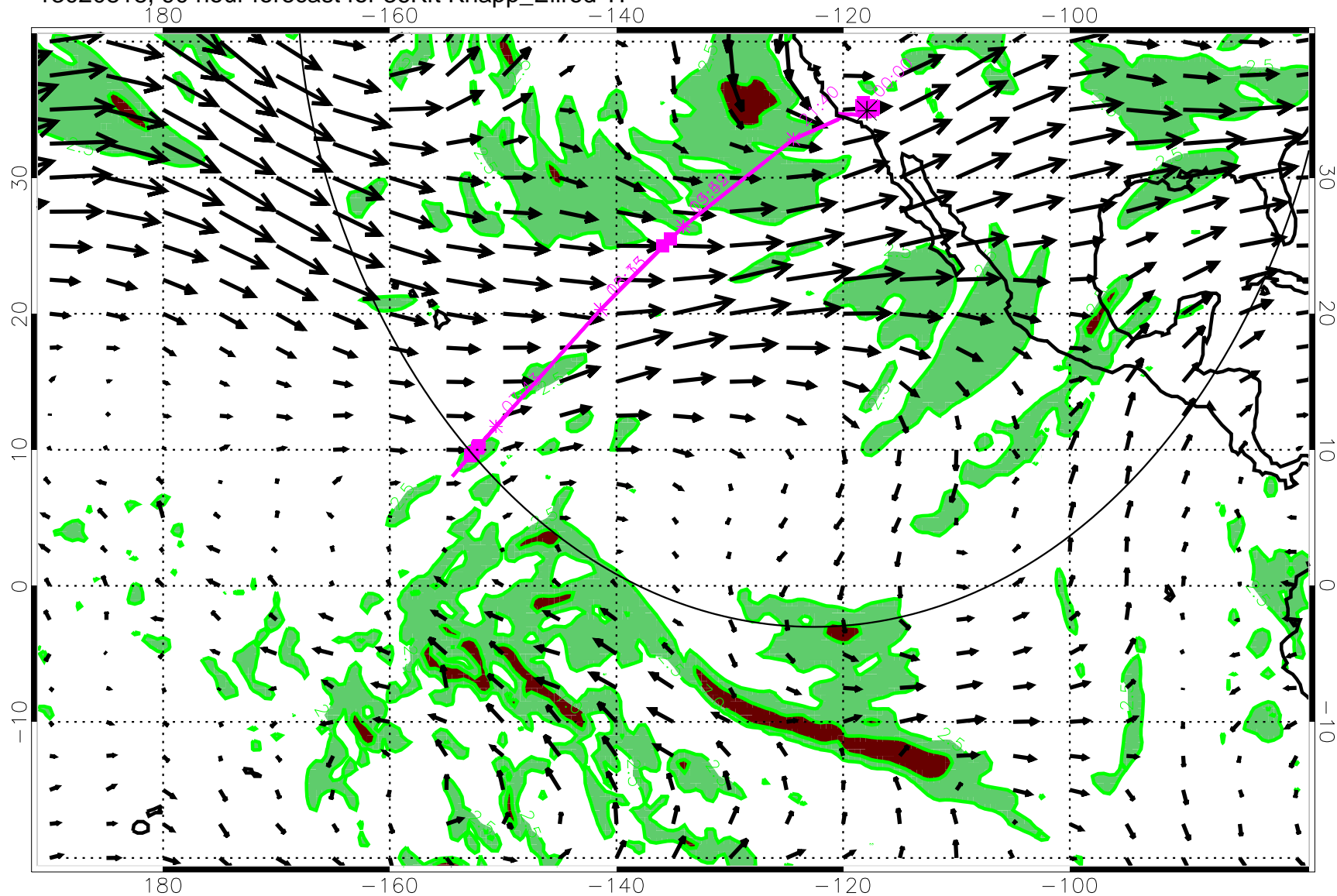
13020818, 90 hour forecast for 36Kft Knapp_Ellrod TI
