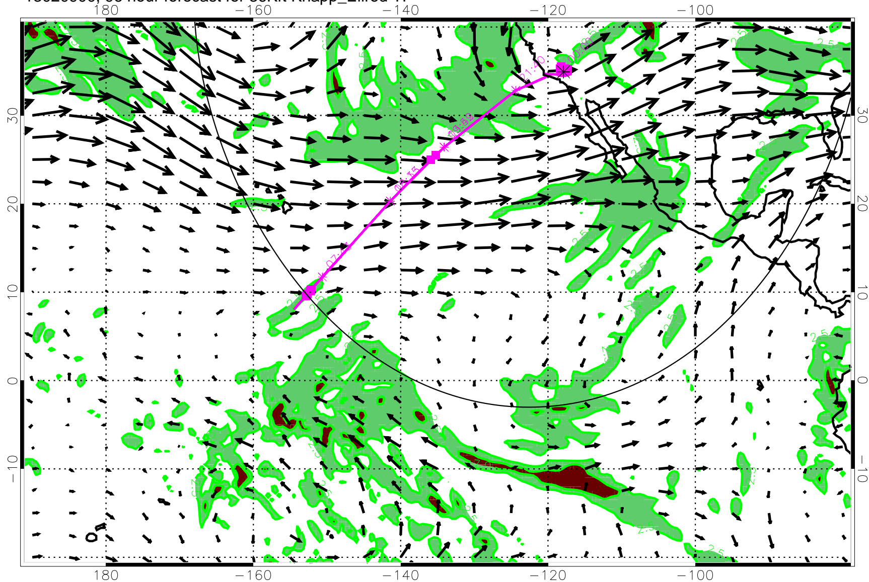
13020900, 96 hour forecast for 36Kft Knapp_Ellrod TI
