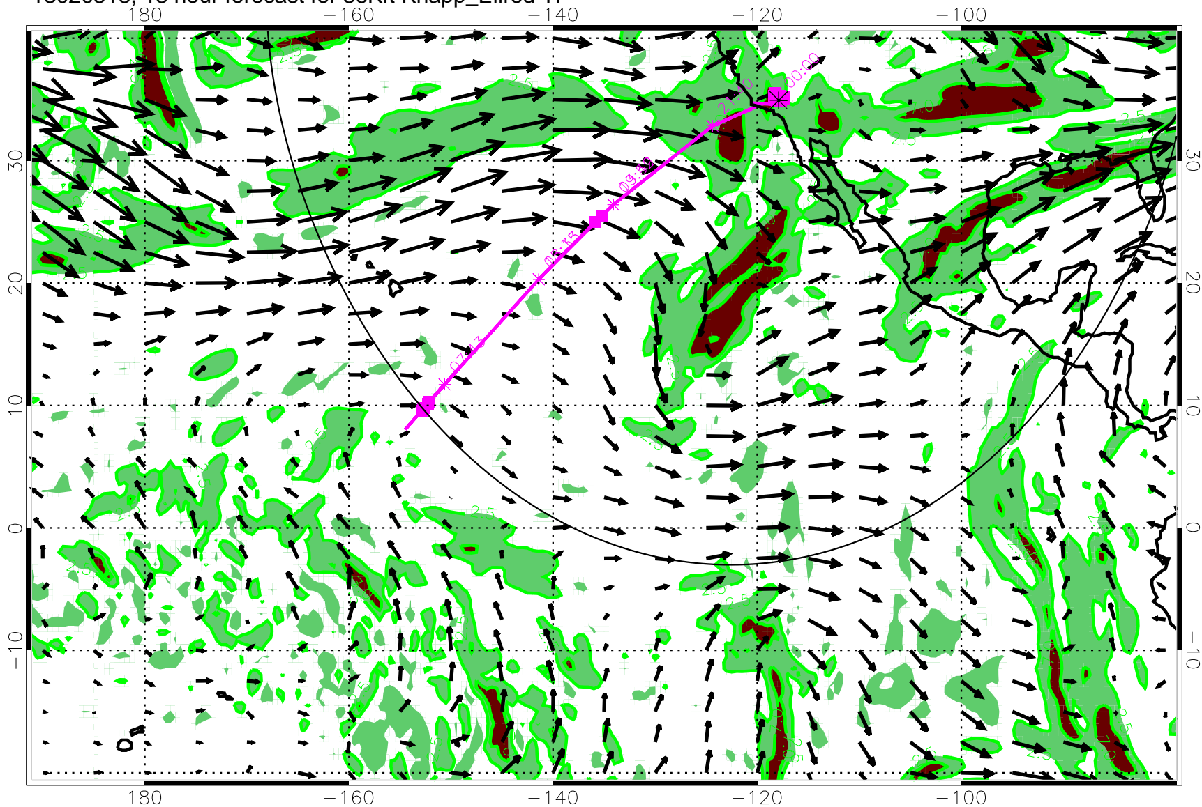
13020518, 18 hour forecast for 36Kft Knapp_Ellrod TI
