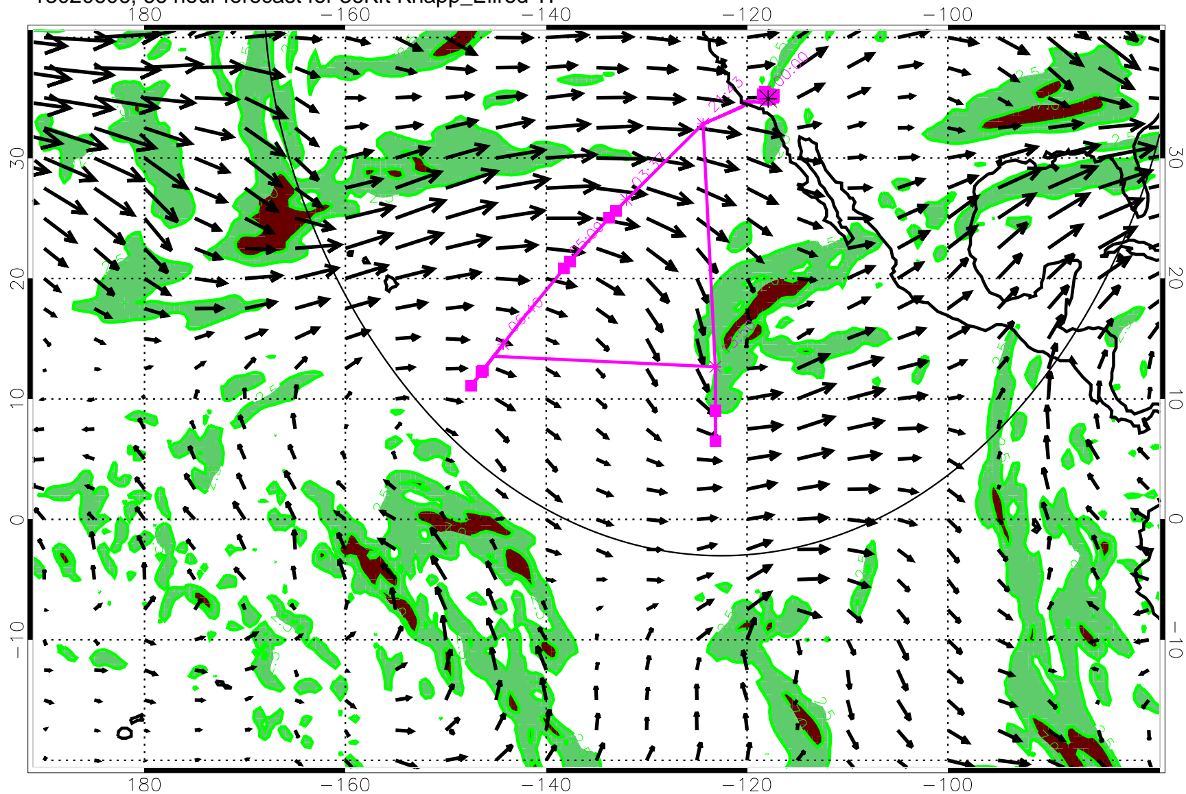
13020606, 66 hour forecast for 36Kft Knapp_Ellrod TI
