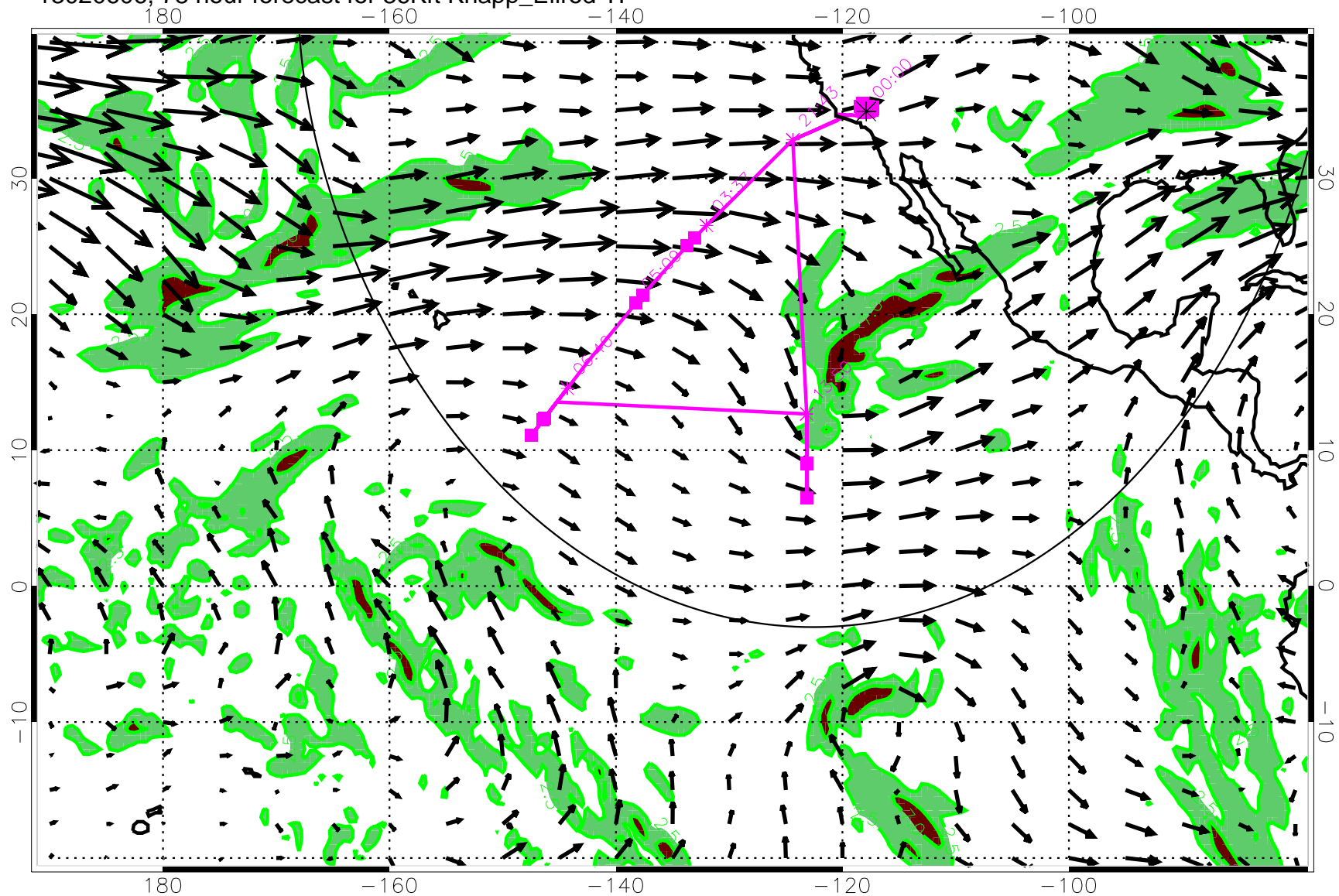
13020606, 78 hour forecast for 36Kft Knapp_Ellrod TI
