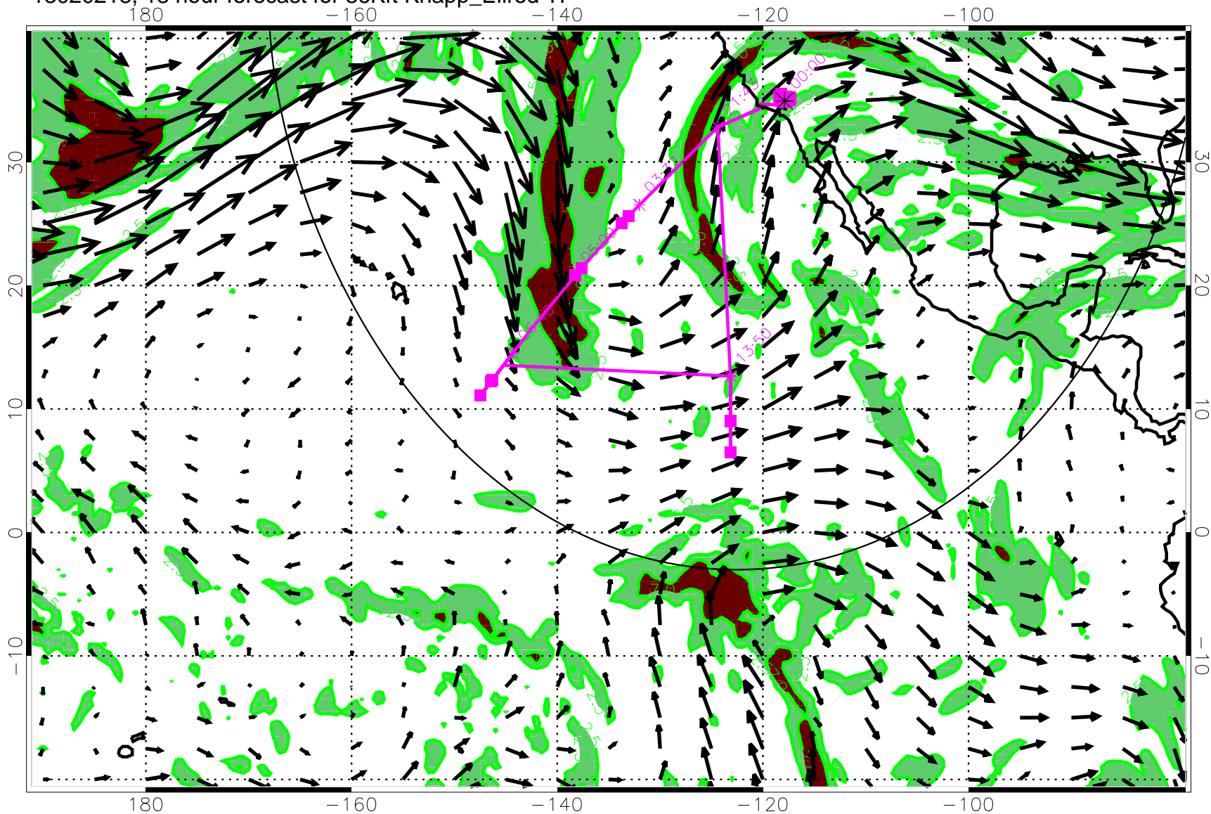
13020218, 18 hour forecast for 36Kft Knapp_Ellrod TI
