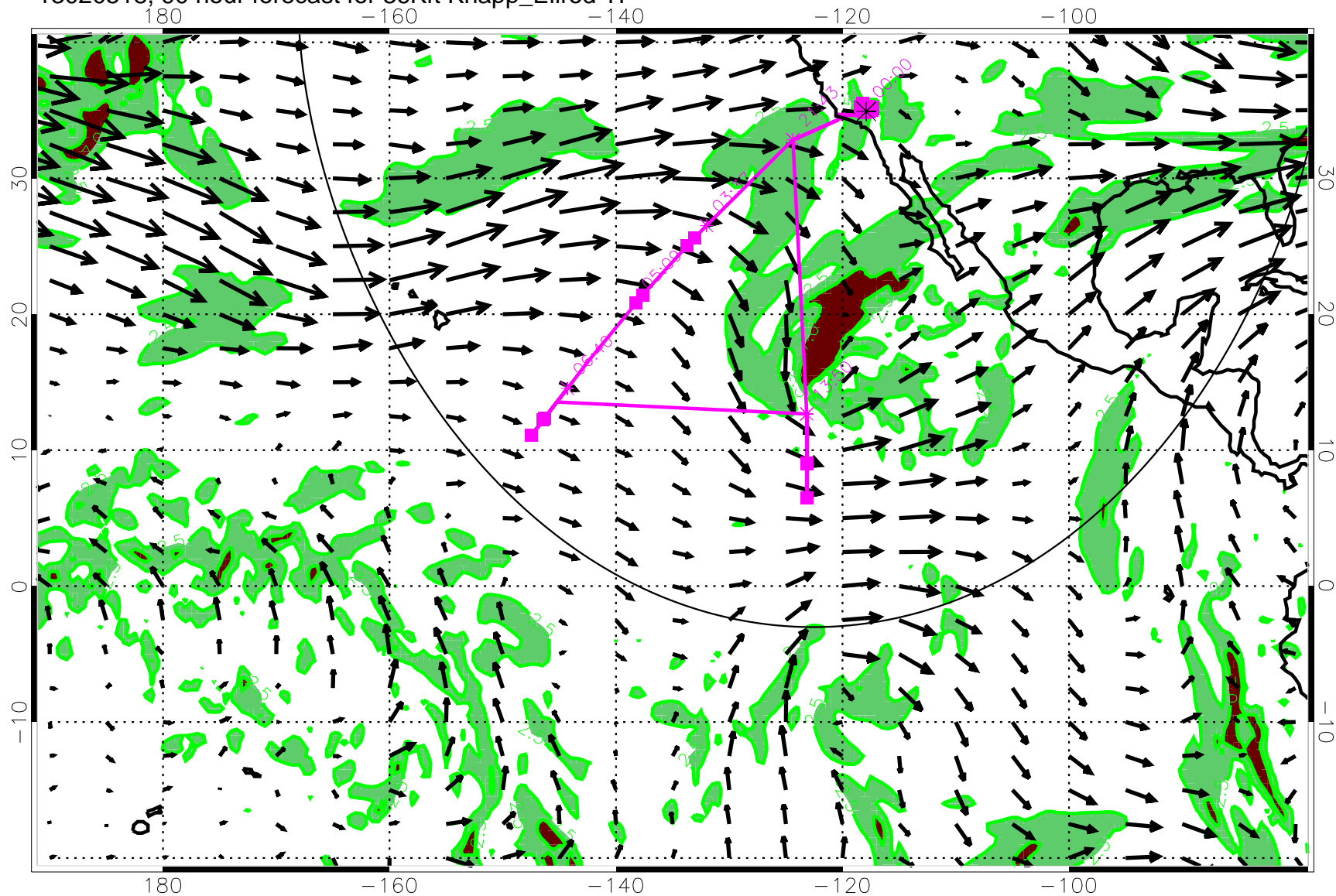
13020518, 90 hour forecast for 36Kft Knapp_Ellrod TI
