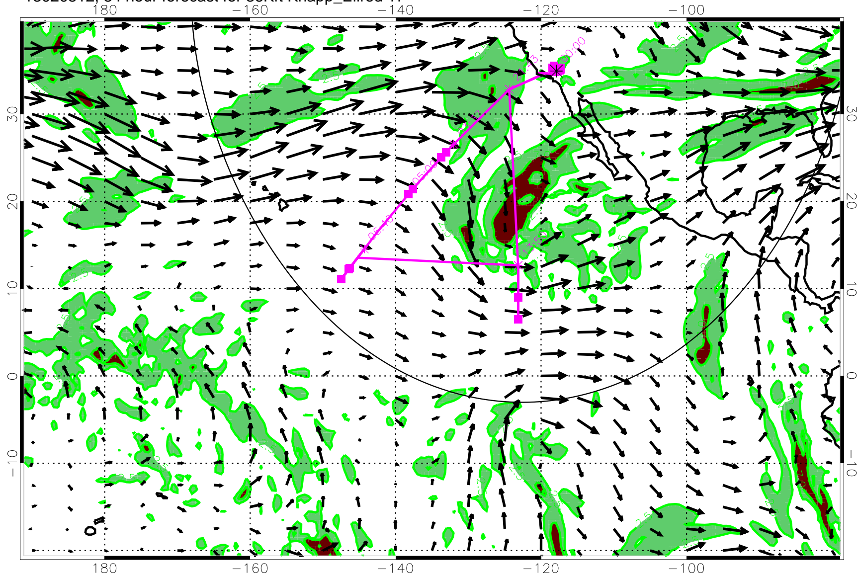
13020512, 84 hour forecast for 36Kft Knapp_Ellrod TI
