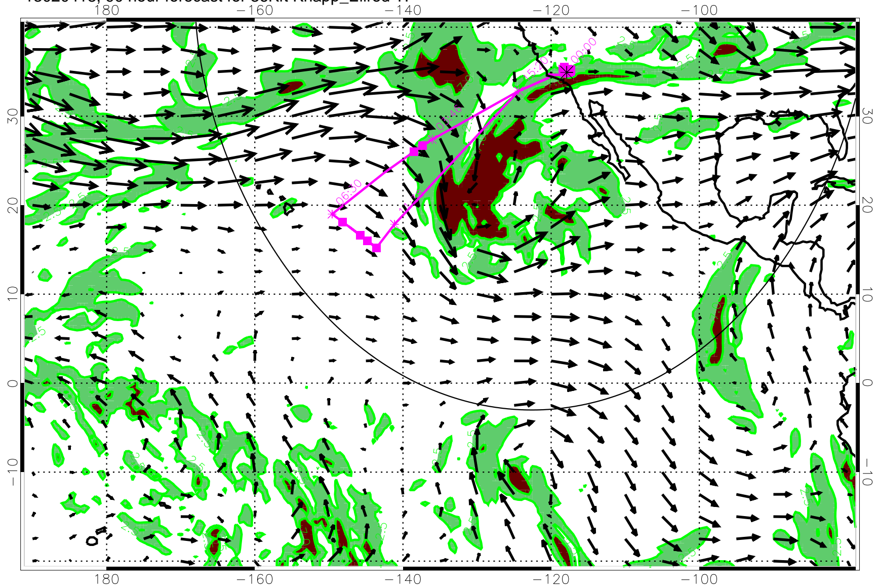
13020418, 90 hour forecast for 36Kft Knapp_Ellrod TI
