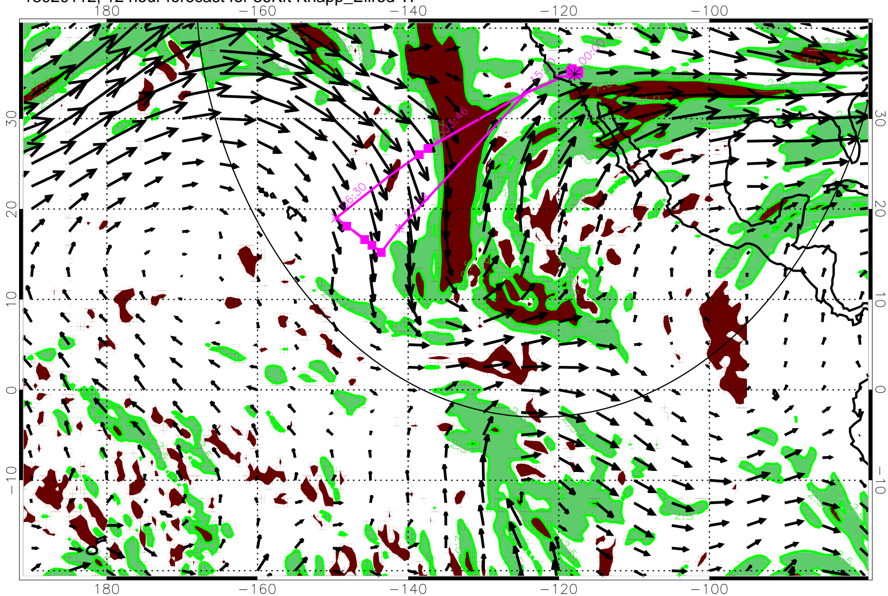
13020112, 12 hour forecast for 36Kft Knapp_Ellrod TI
