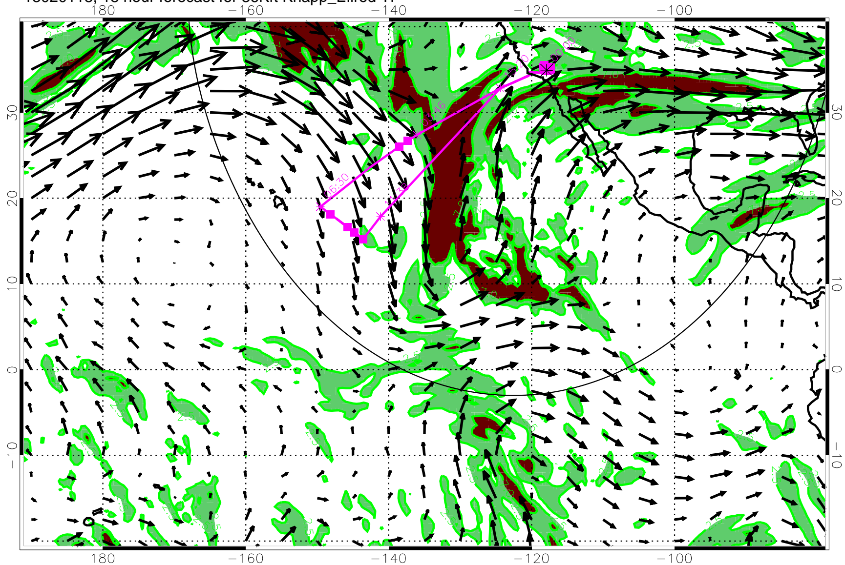
13020118, 18 hour forecast for 36Kft Knapp_Ellrod TI
