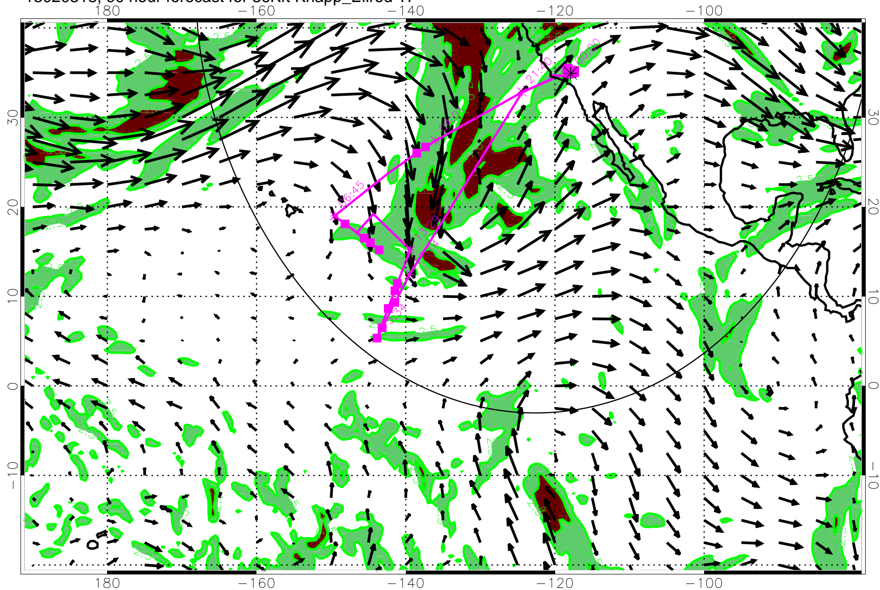
13020318, 90 hour forecast for 36Kft Knapp_Ellrod TI
