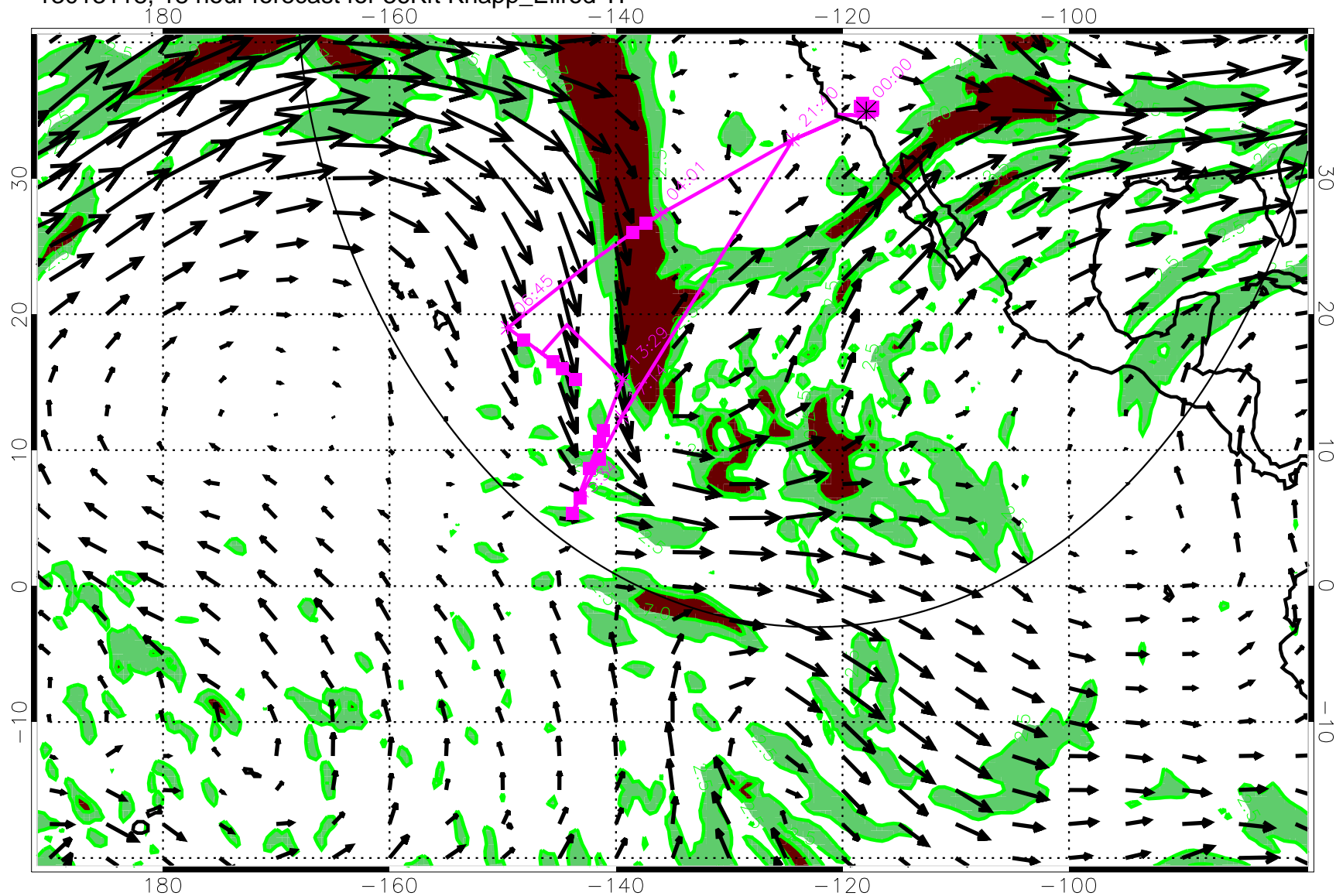
13013118, 18 hour forecast for 36Kft Knapp_Ellrod TI
