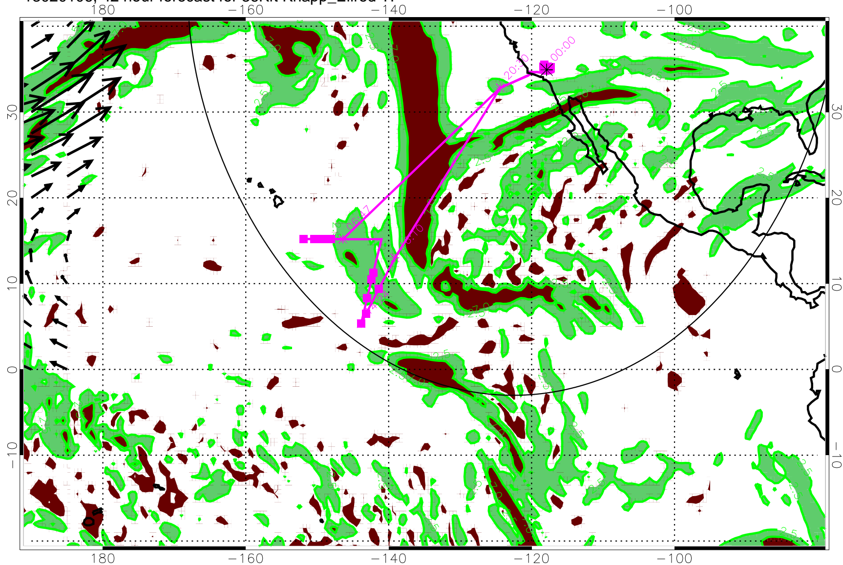
13020106, 42 hour forecast for 36Kft Knapp_Ellrod TI
