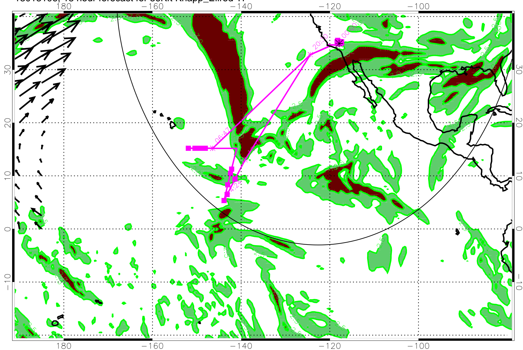
13013106, 18 hour forecast for 36Kft Knapp_Ellrod TI
