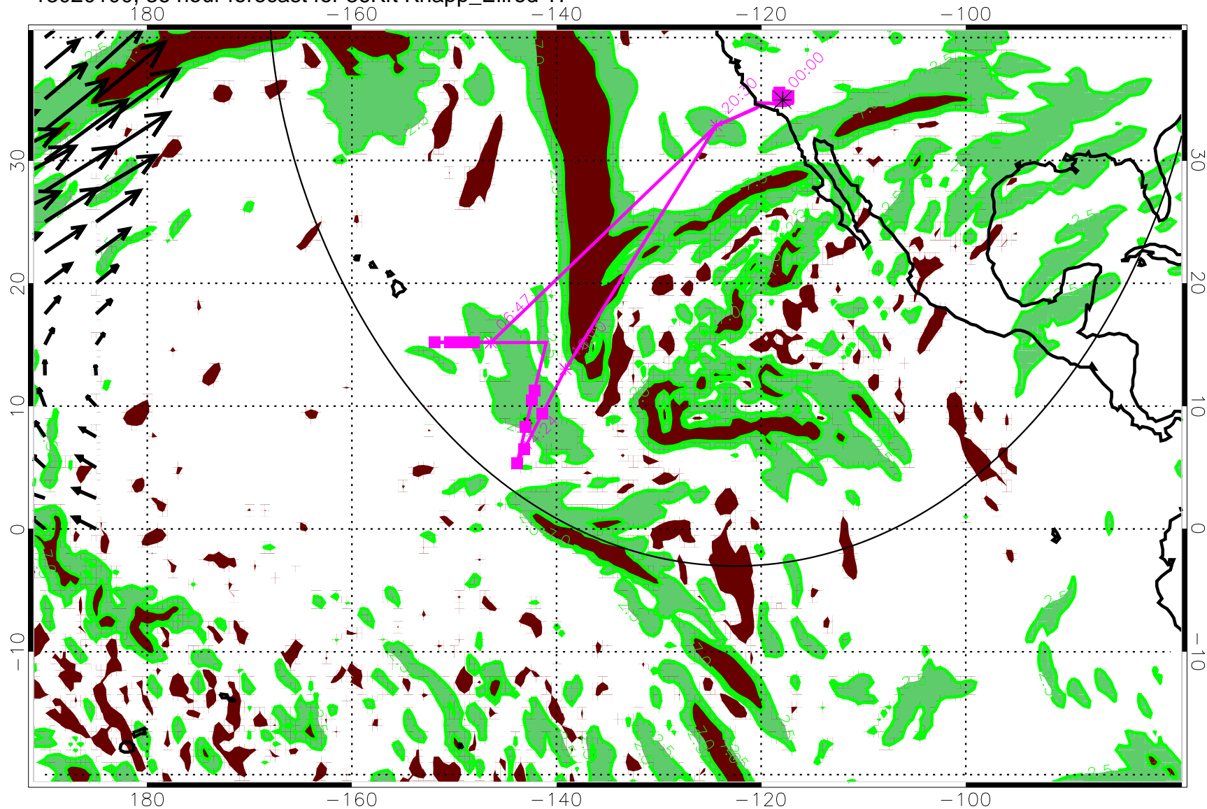
13020100, 36 hour forecast for 36Kft Knapp_Ellrod TI
