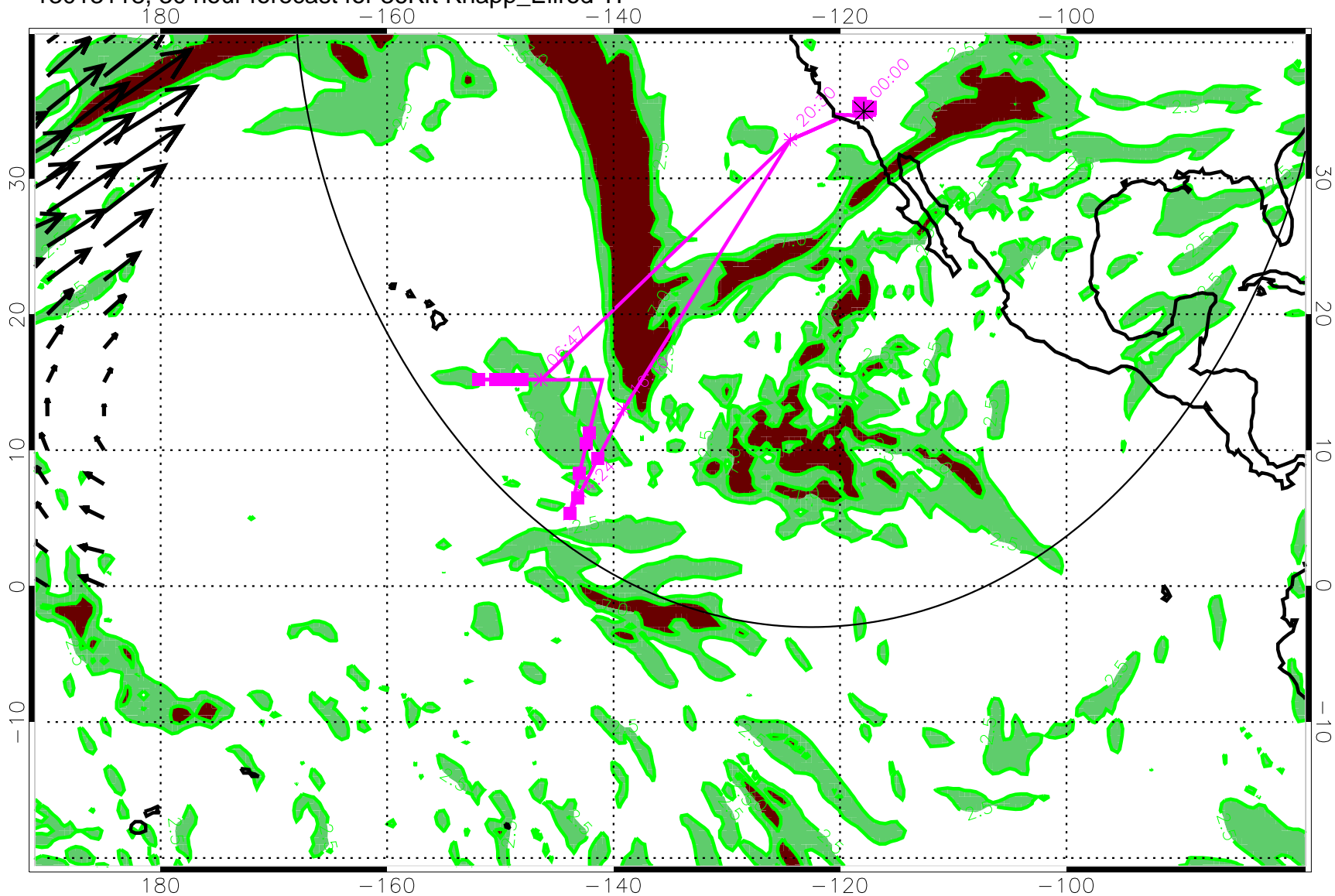
13013118, 30 hour forecast for 36Kft Knapp_Ellrod TI
