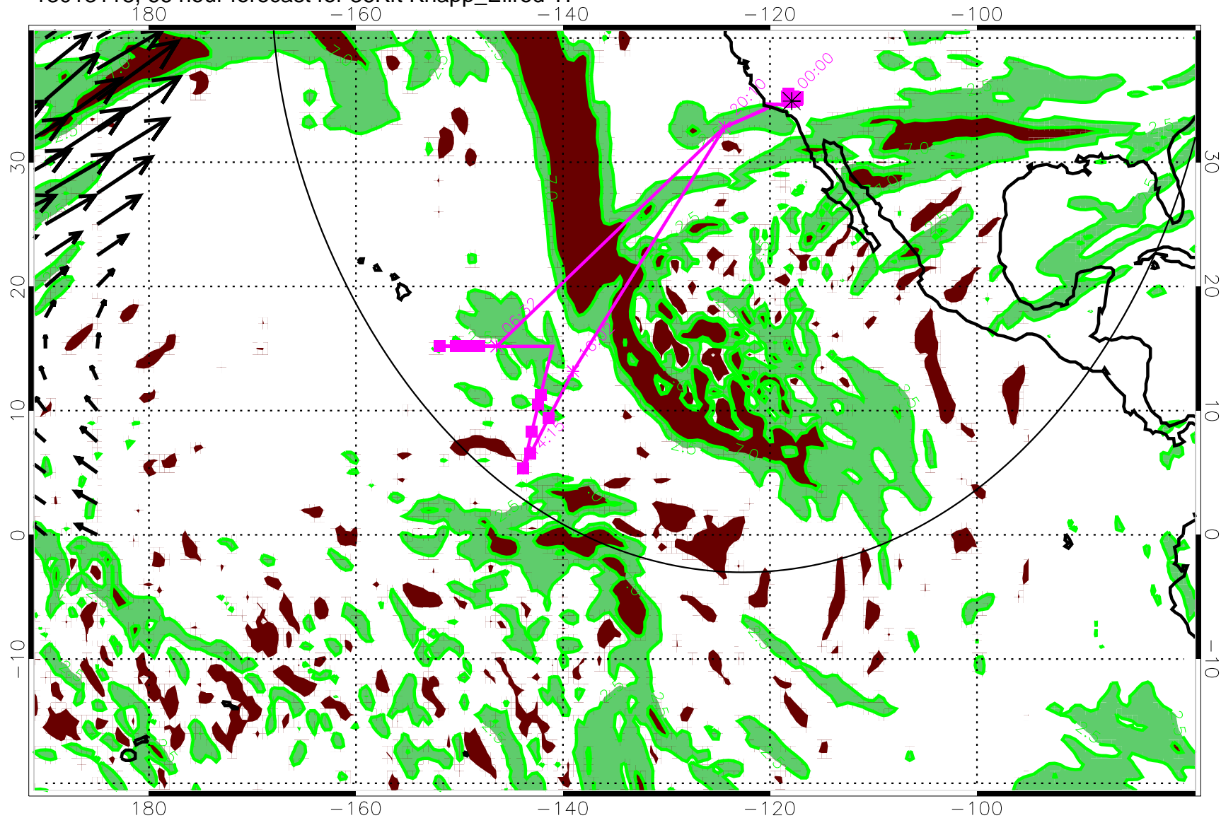
13013118, 66 hour forecast for 36Kft Knapp_Ellrod TI
