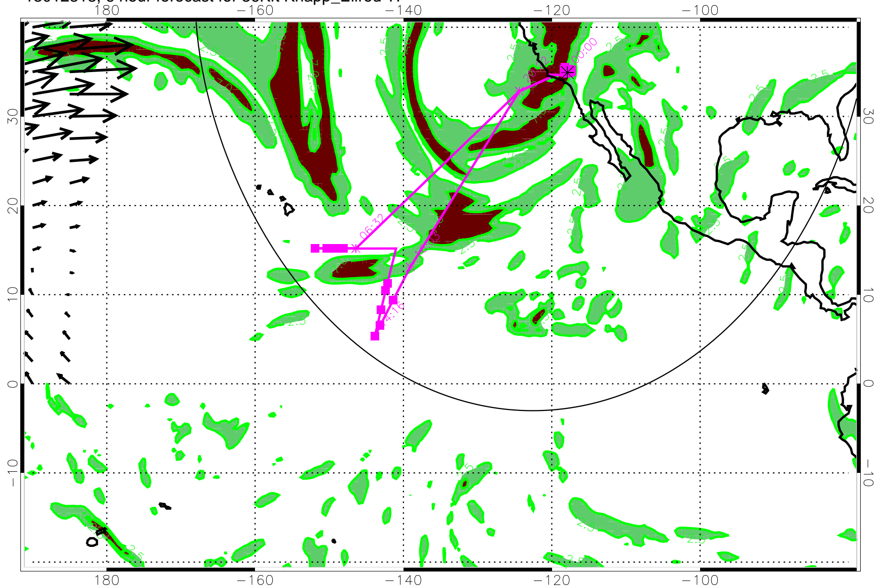
13012818, 6 hour forecast for 36Kft Knapp_Ellrod TI
