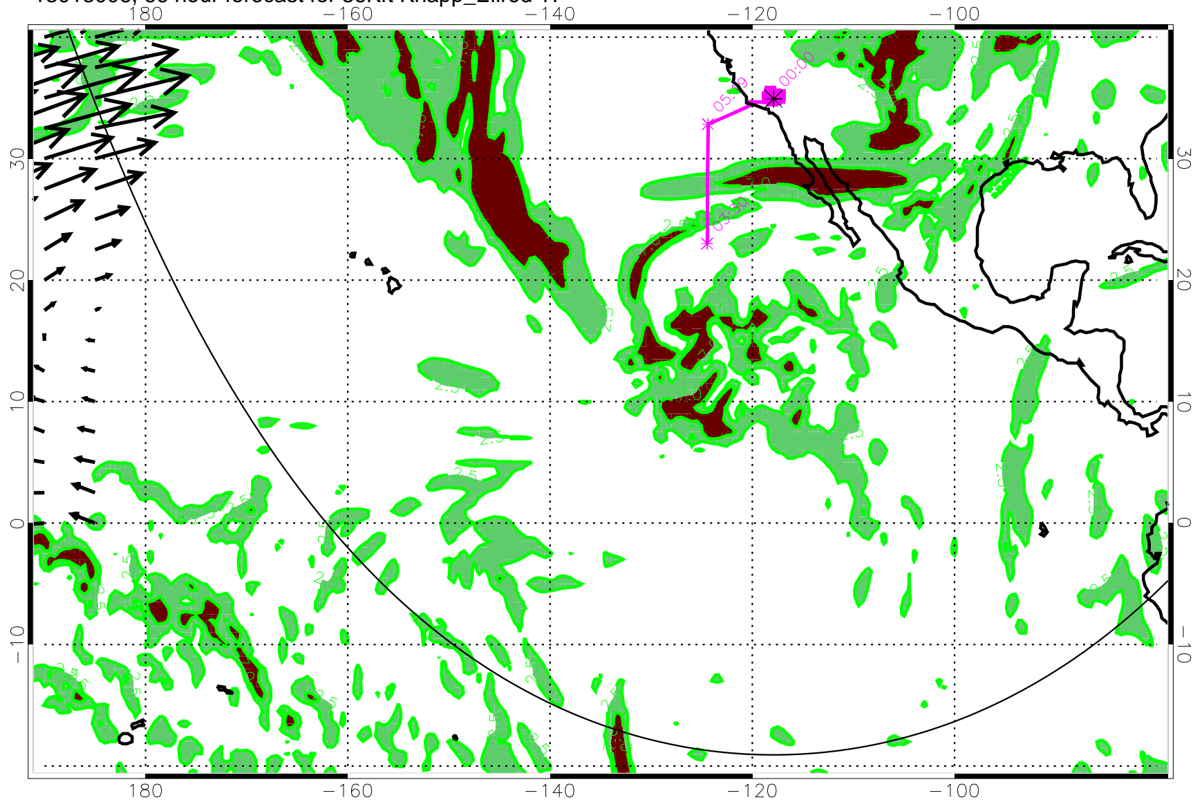
13013006, 66 hour forecast for 36Kft Knapp_Ellrod TI
