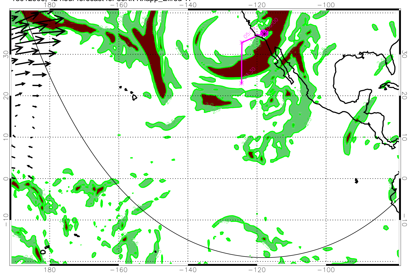
13012906, 42 hour forecast for 36Kft Knapp_Ellrod TI
