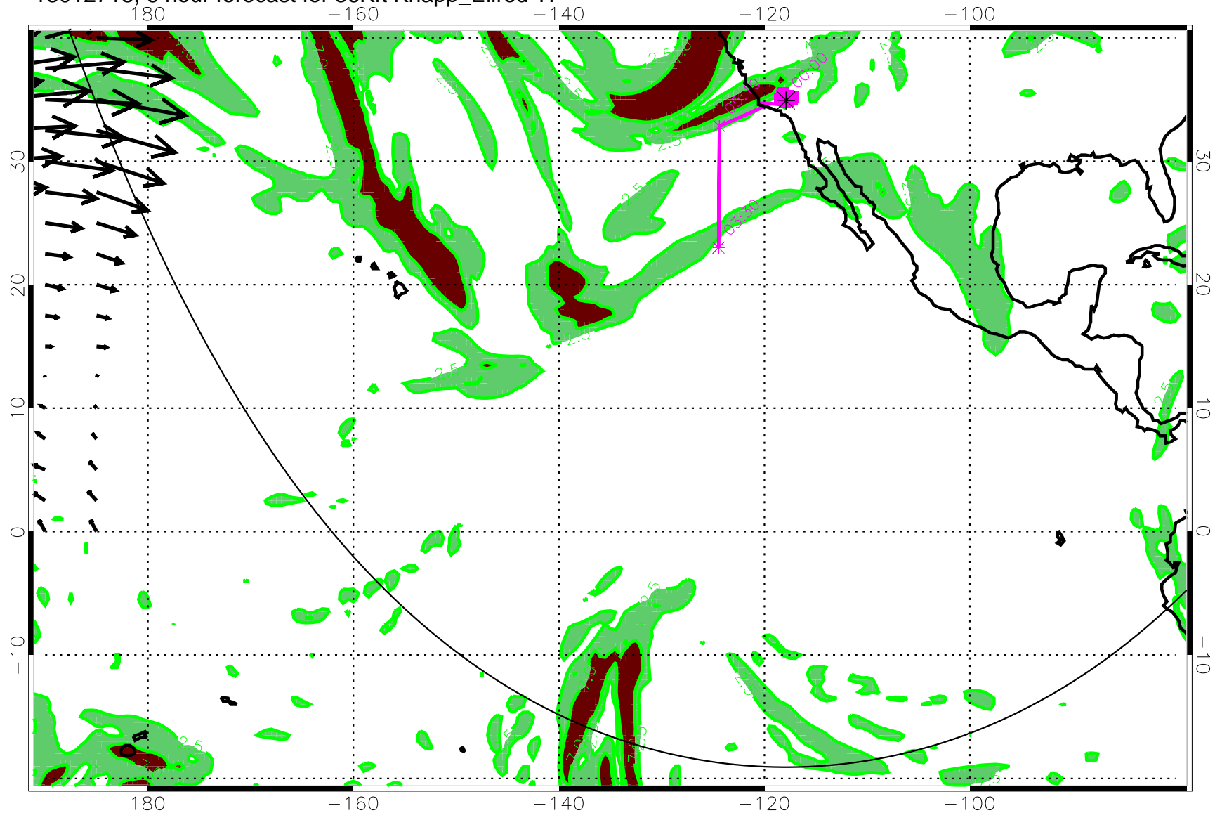
13012718, 6 hour forecast for 36Kft Knapp_Ellrod TI
