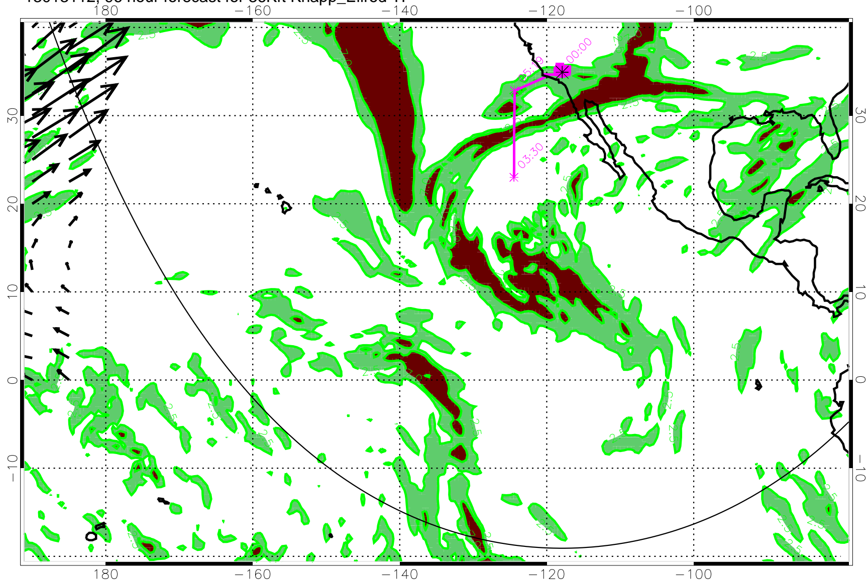
13013112, 96 hour forecast for 36Kft Knapp_Ellrod TI
