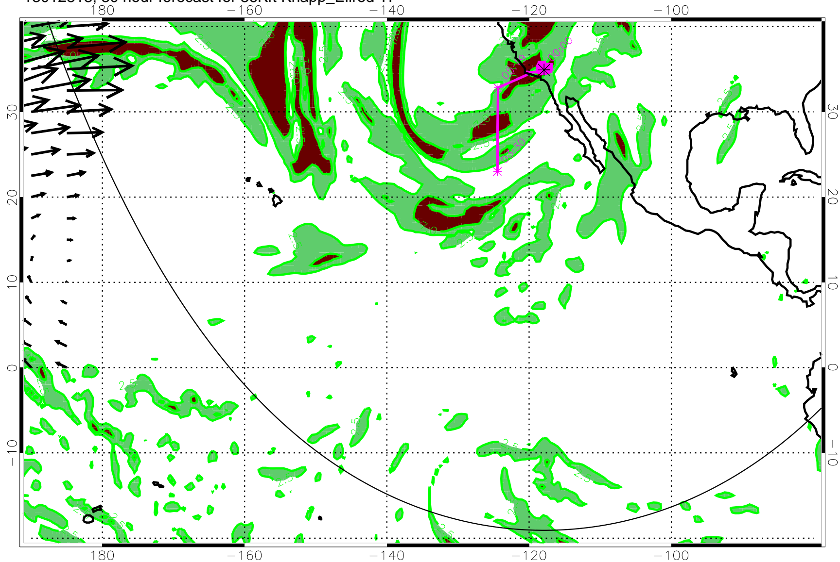
13012818, 30 hour forecast for 36Kft Knapp_Ellrod TI
