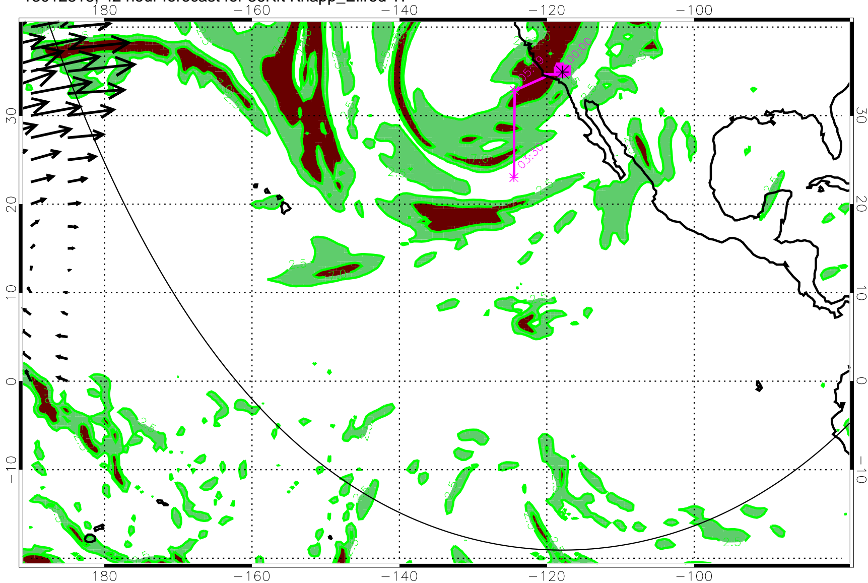
13012818, 42 hour forecast for 36Kft Knapp_Ellrod TI
