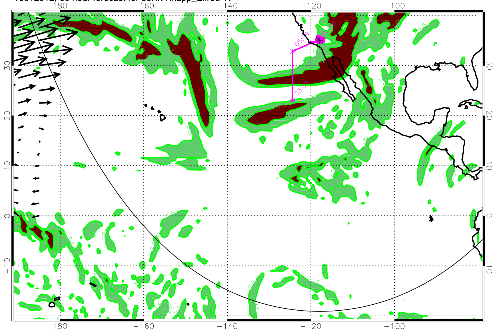
13012912, 60 hour forecast for 36Kft Knapp_Ellrod TI
