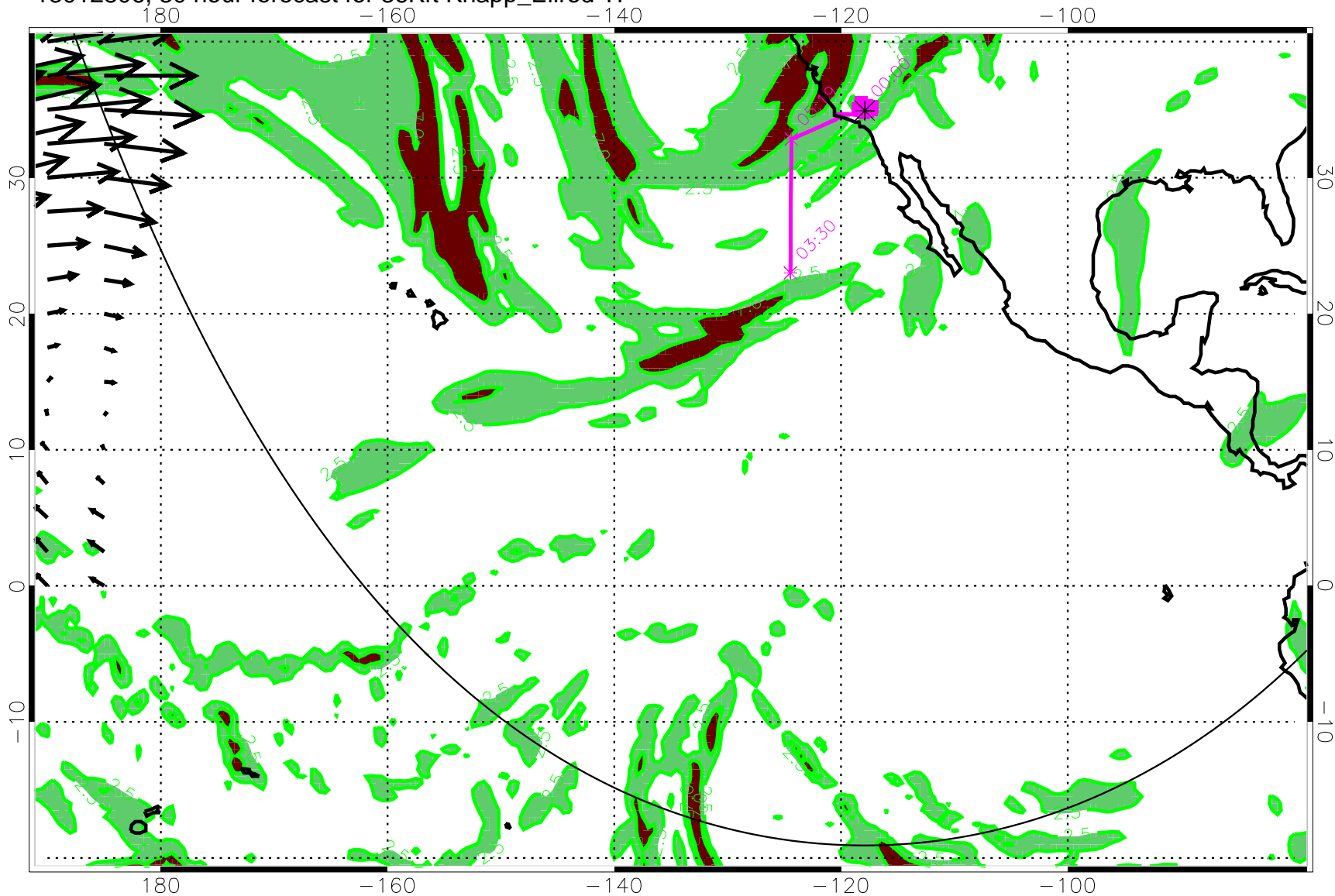
13012806, 30 hour forecast for 36Kft Knapp_Ellrod TI
