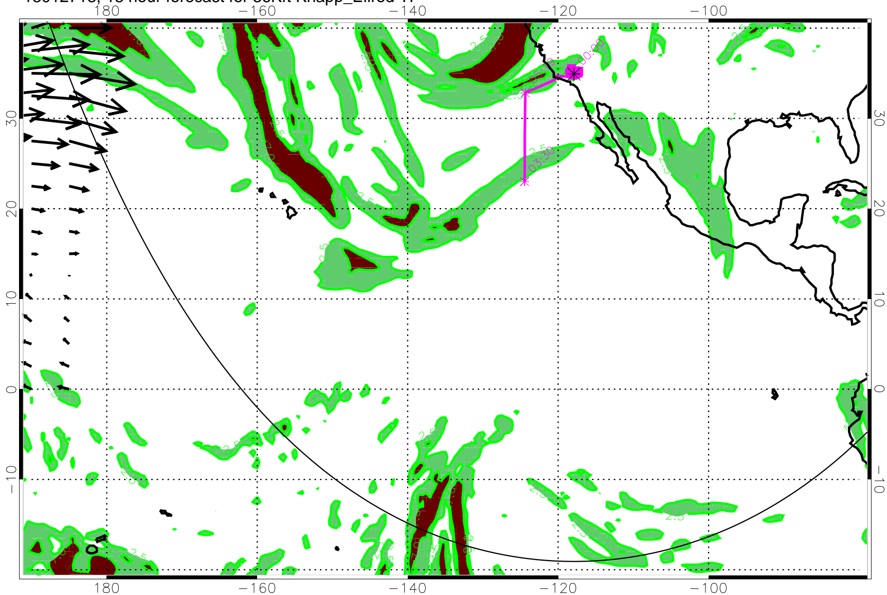
13012718, 18 hour forecast for 36Kft Knapp_Ellrod TI
