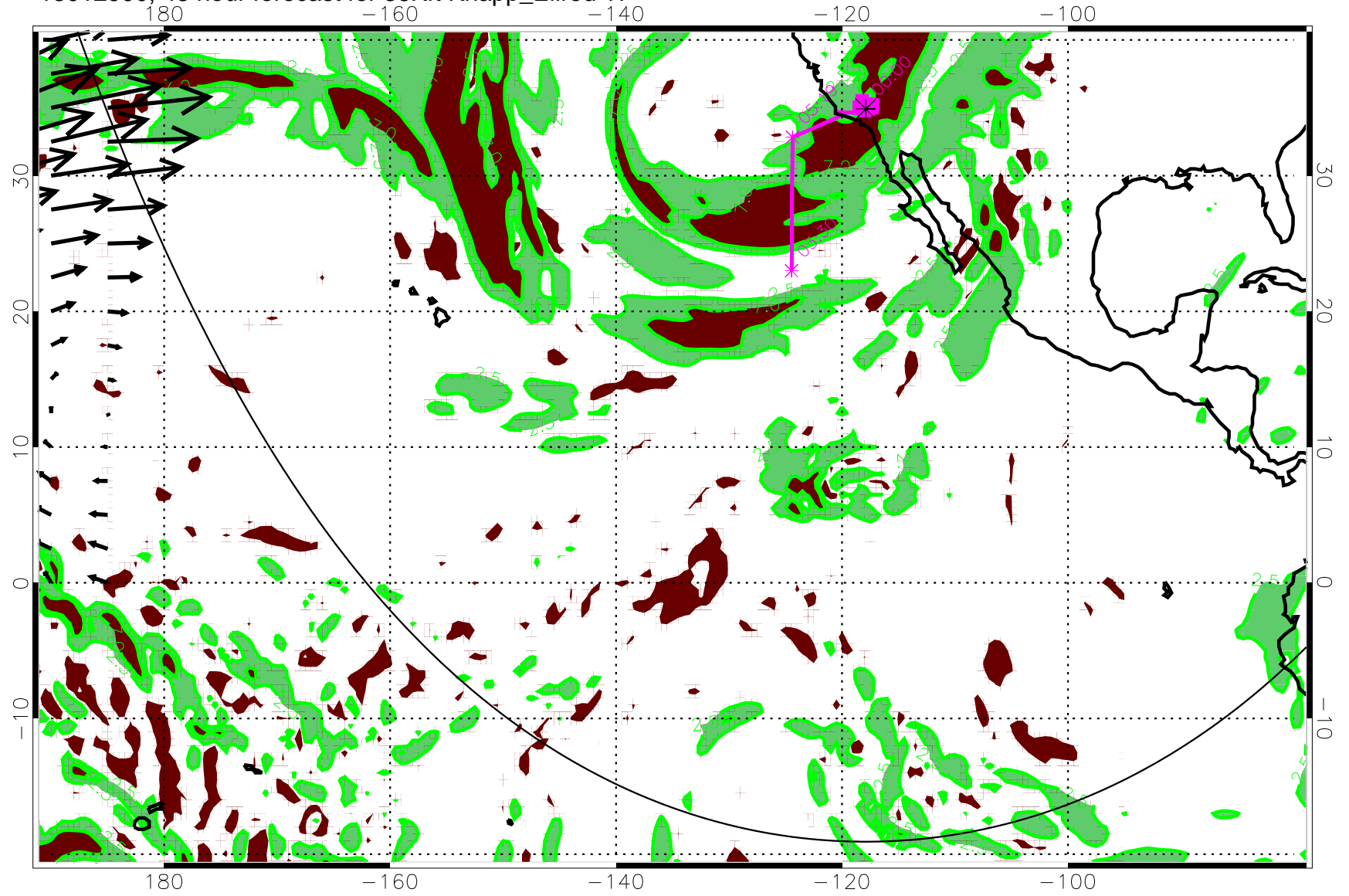
13012900, 48 hour forecast for 36Kft Knapp_Ellrod TI
