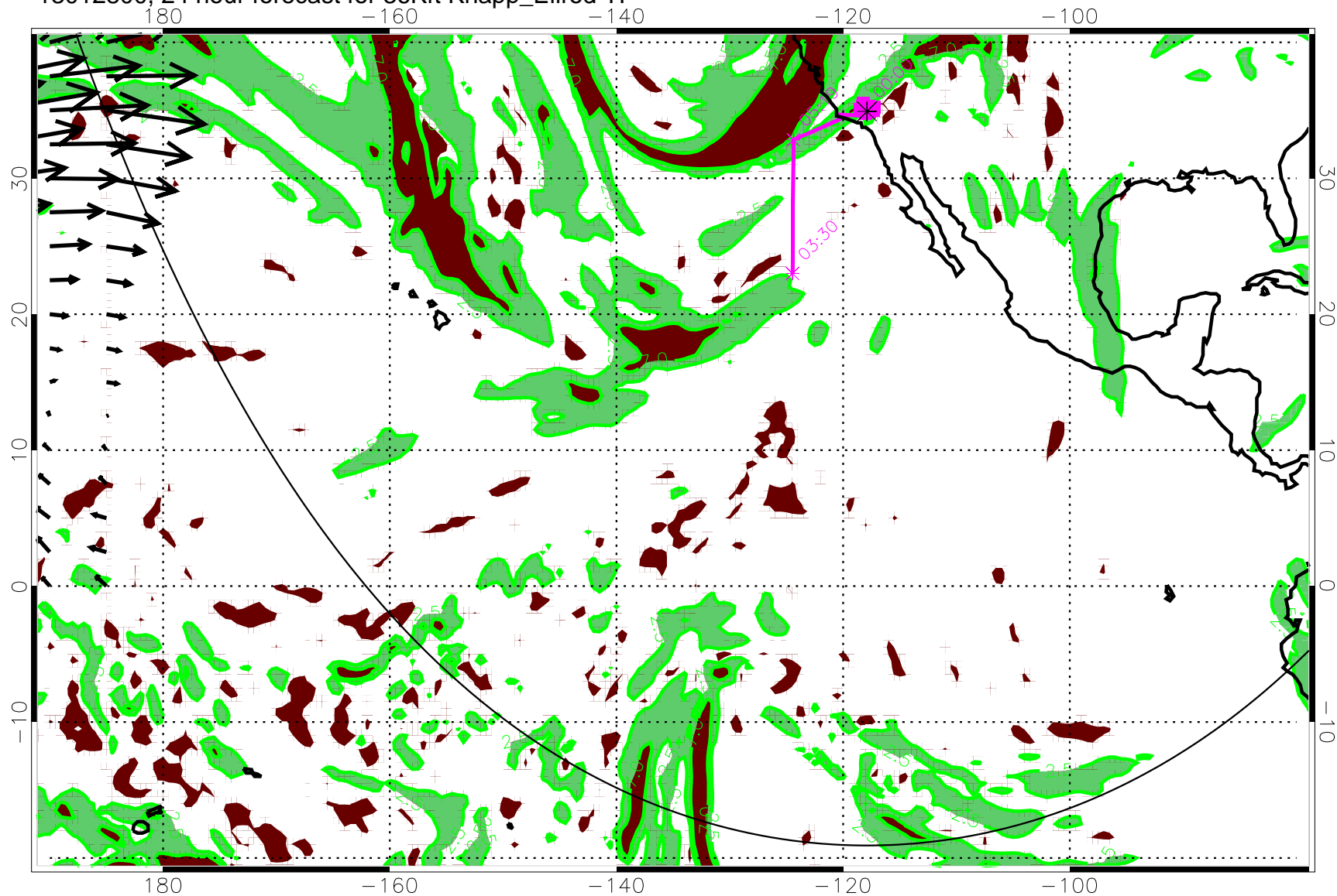
13012800, 24 hour forecast for 36Kft Knapp_Ellrod TI
