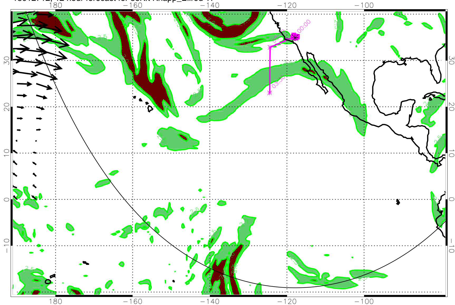
13012712, 12 hour forecast for 36Kft Knapp_Ellrod TI
