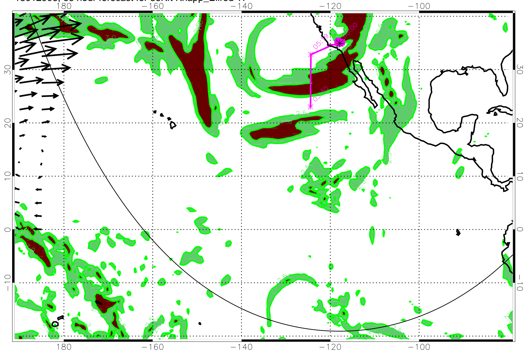
13012906, 66 hour forecast for 36Kft Knapp_Ellrod TI
