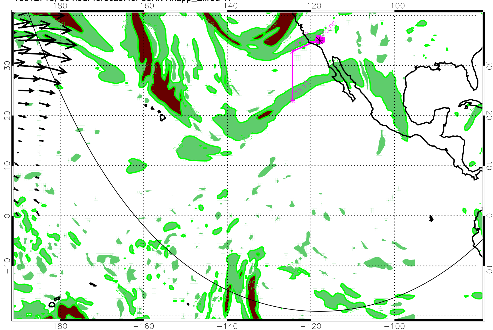
13012718, 30 hour forecast for 36Kft Knapp_Ellrod TI
