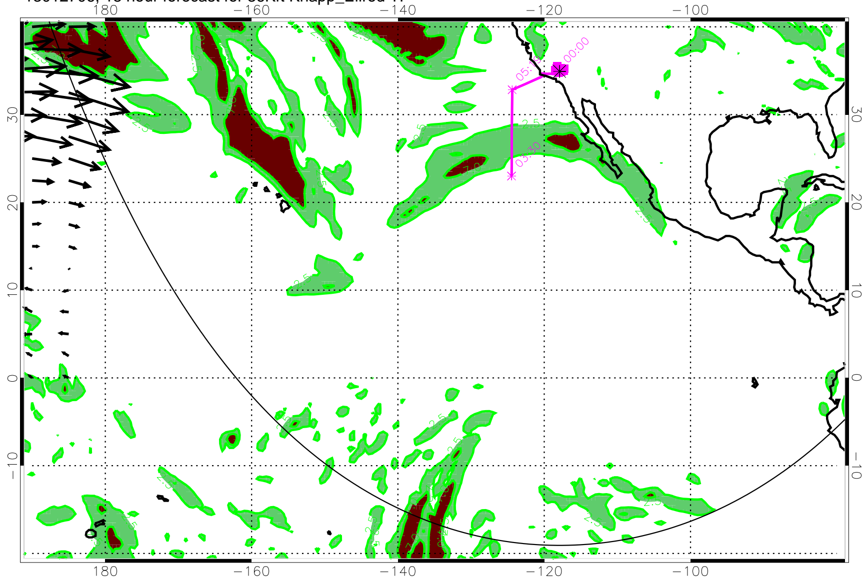
13012706, 18 hour forecast for 36Kft Knapp_Ellrod TI
