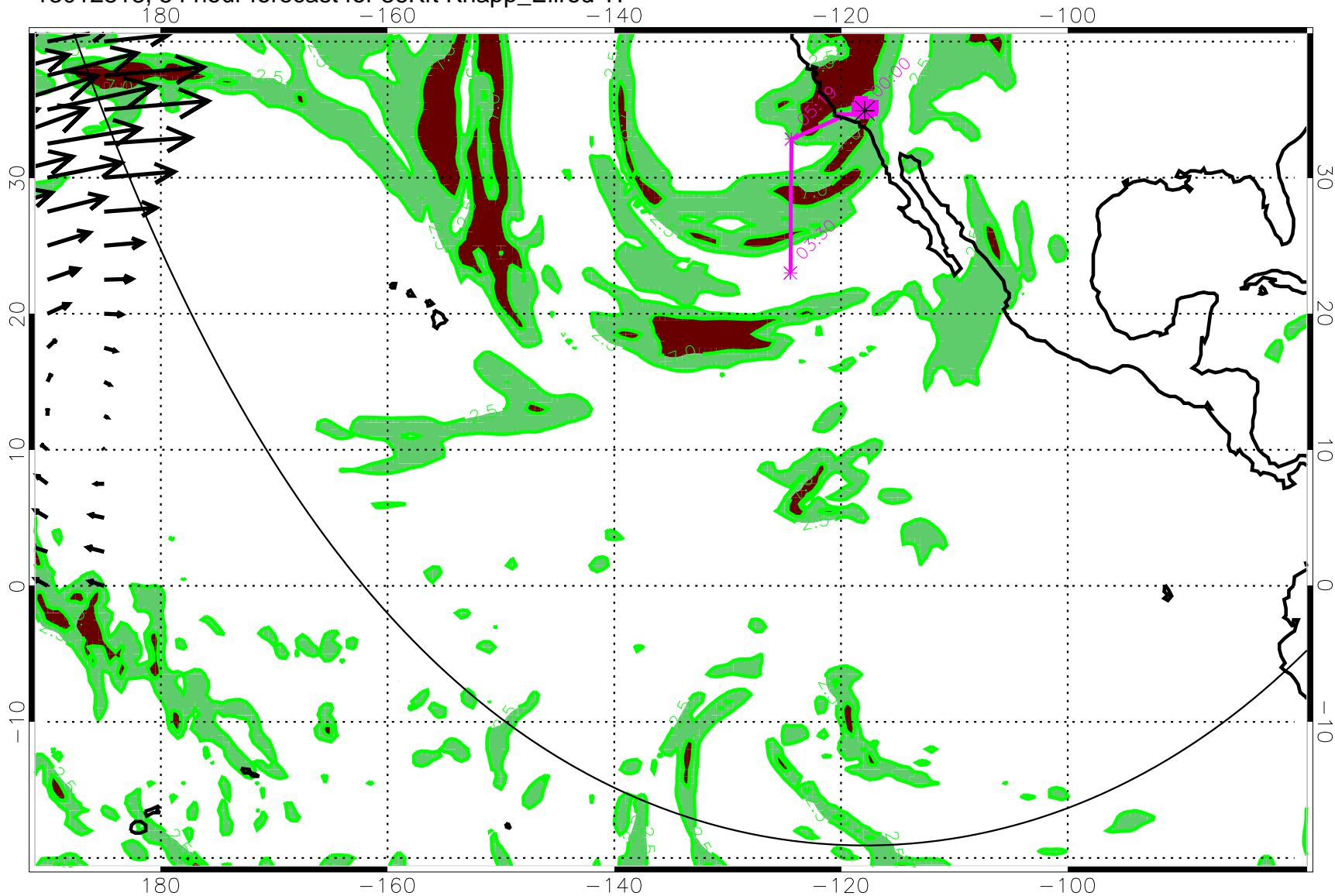
13012818, 54 hour forecast for 36Kft Knapp_Ellrod TI
