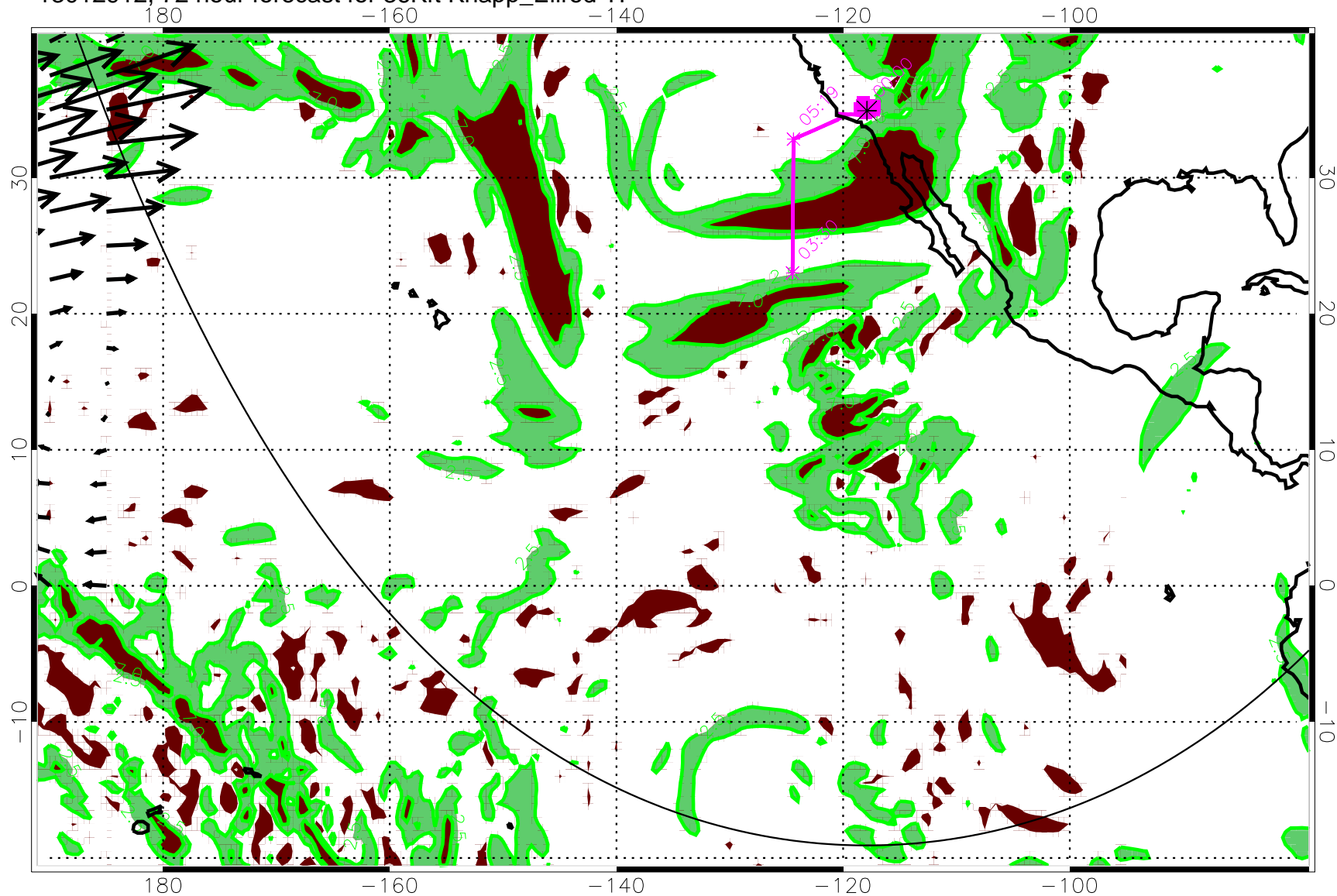
13012912, 72 hour forecast for 36Kft Knapp_Ellrod TI
