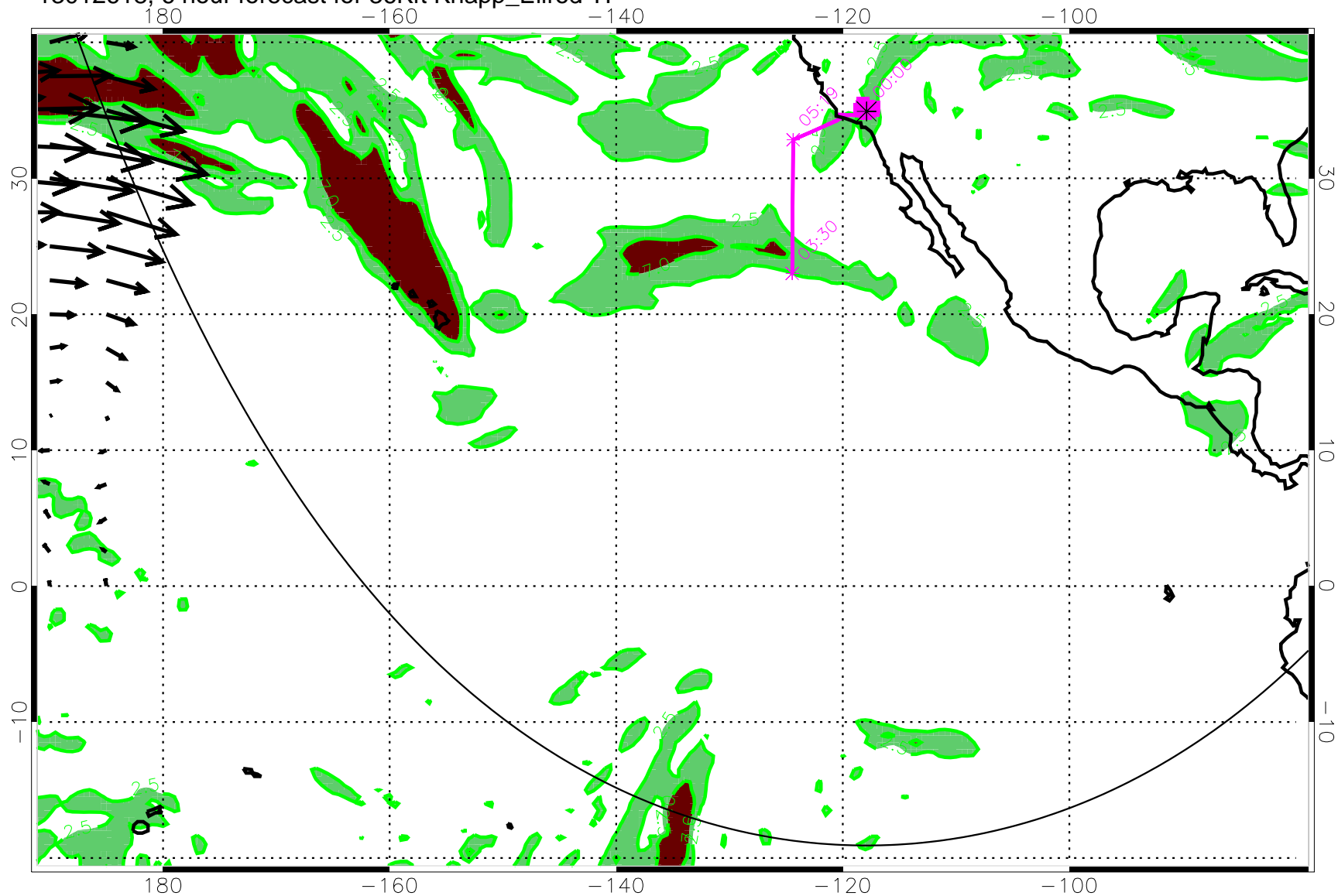
13012618, 6 hour forecast for 36Kft Knapp_Ellrod TI
