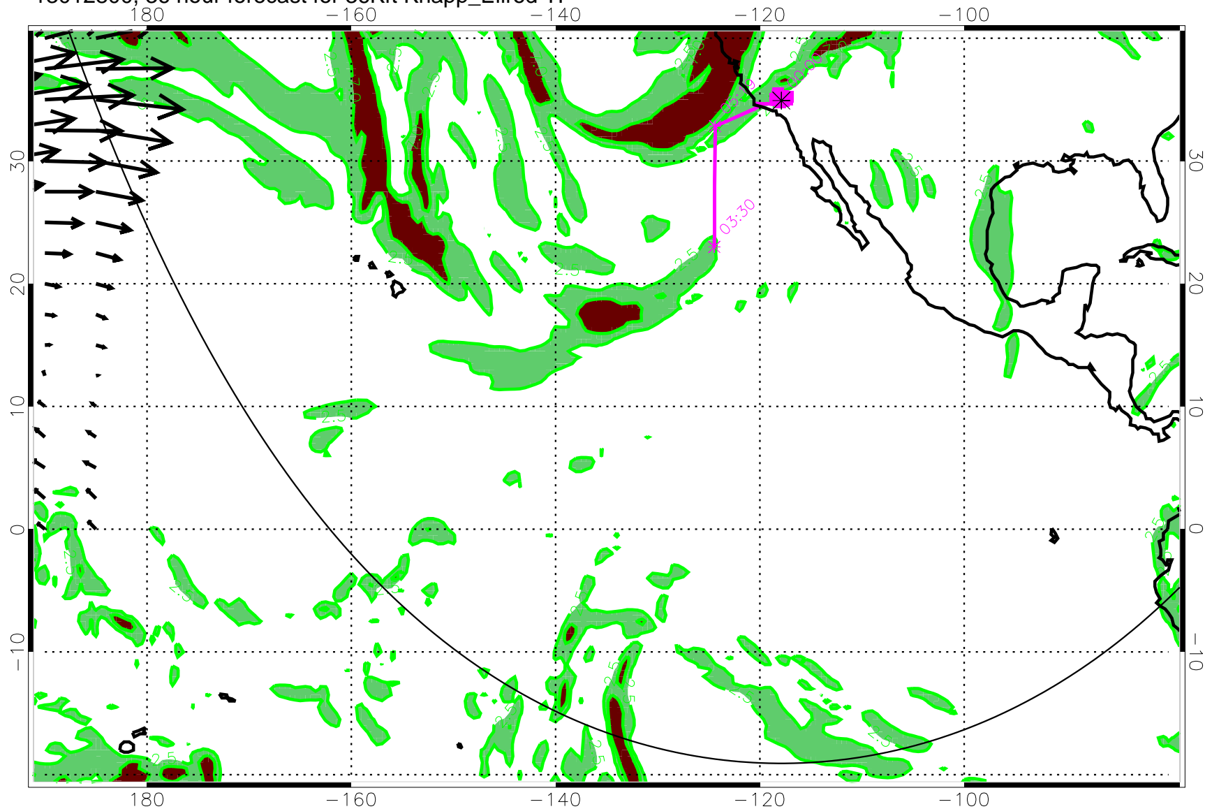
13012800, 36 hour forecast for 36Kft Knapp_Ellrod TI
