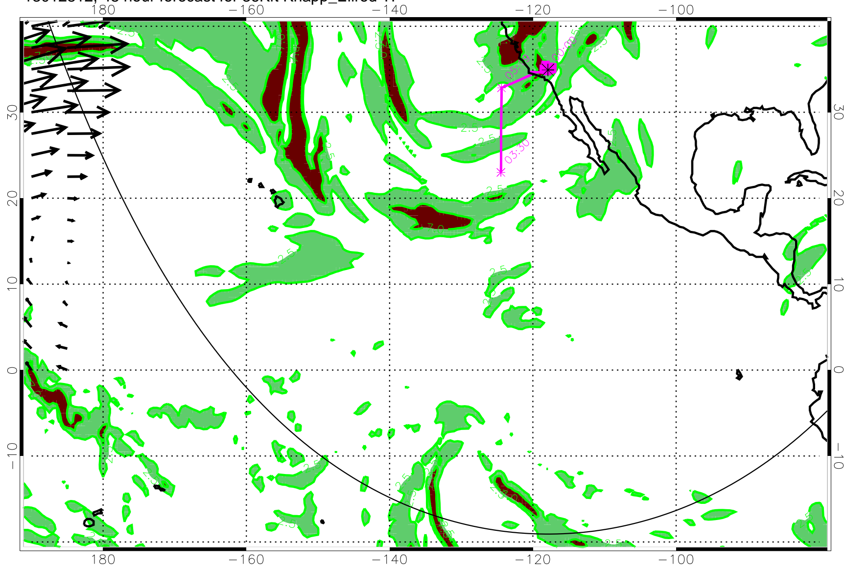
13012812, 48 hour forecast for 36Kft Knapp_Ellrod TI
