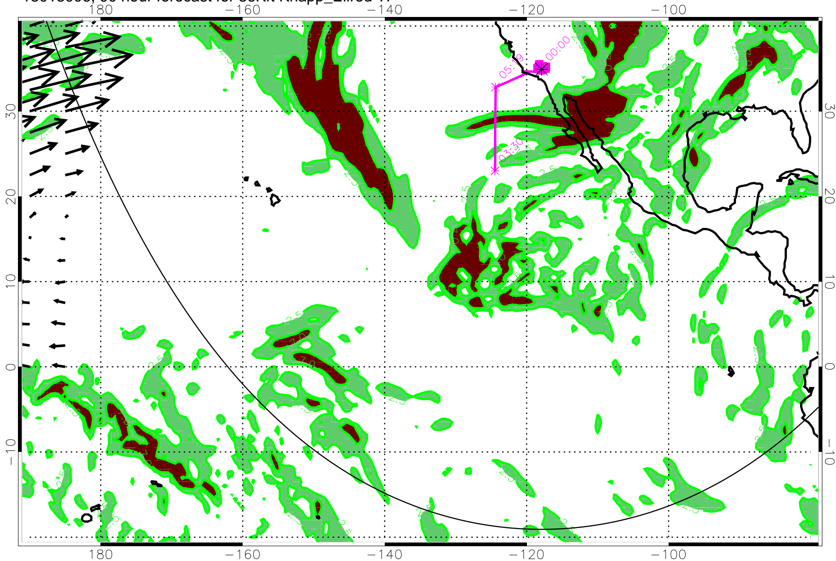
13013006, 90 hour forecast for 36Kft Knapp_Ellrod TI
