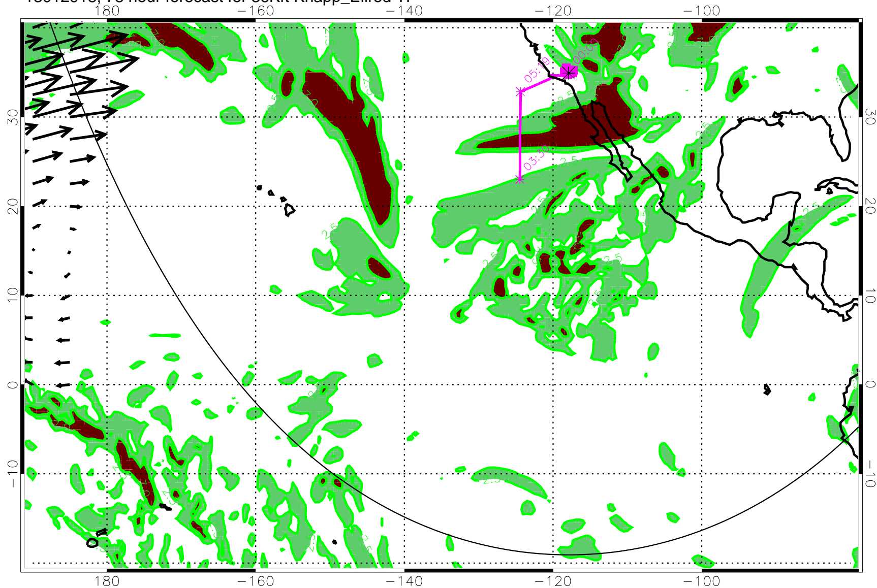
13012918, 78 hour forecast for 36Kft Knapp_Ellrod TI
