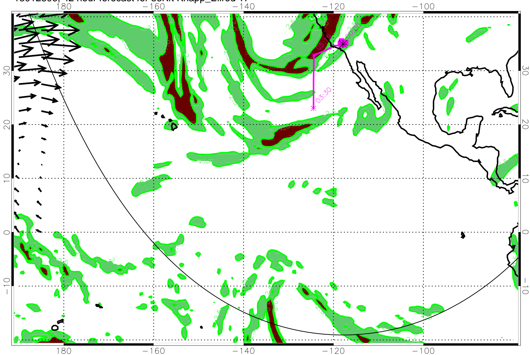
13012806, 42 hour forecast for 36Kft Knapp_Ellrod TI
