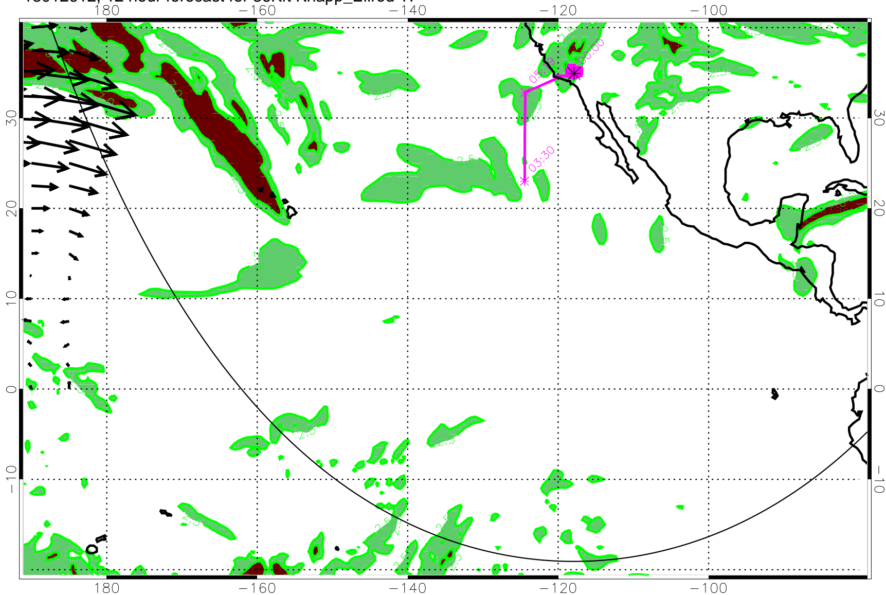
13012612, 12 hour forecast for 36Kft Knapp_Ellrod TI
