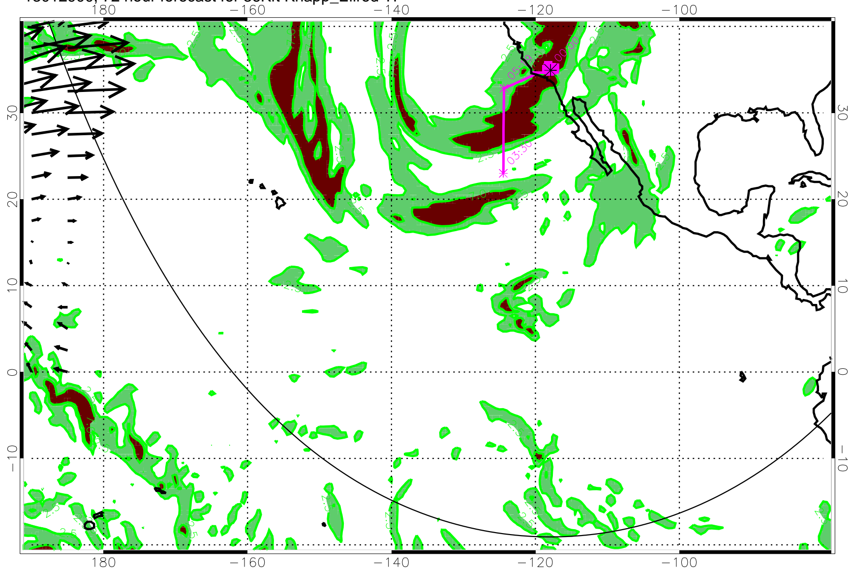
13012900, 72 hour forecast for 36Kft Knapp_Ellrod TI
