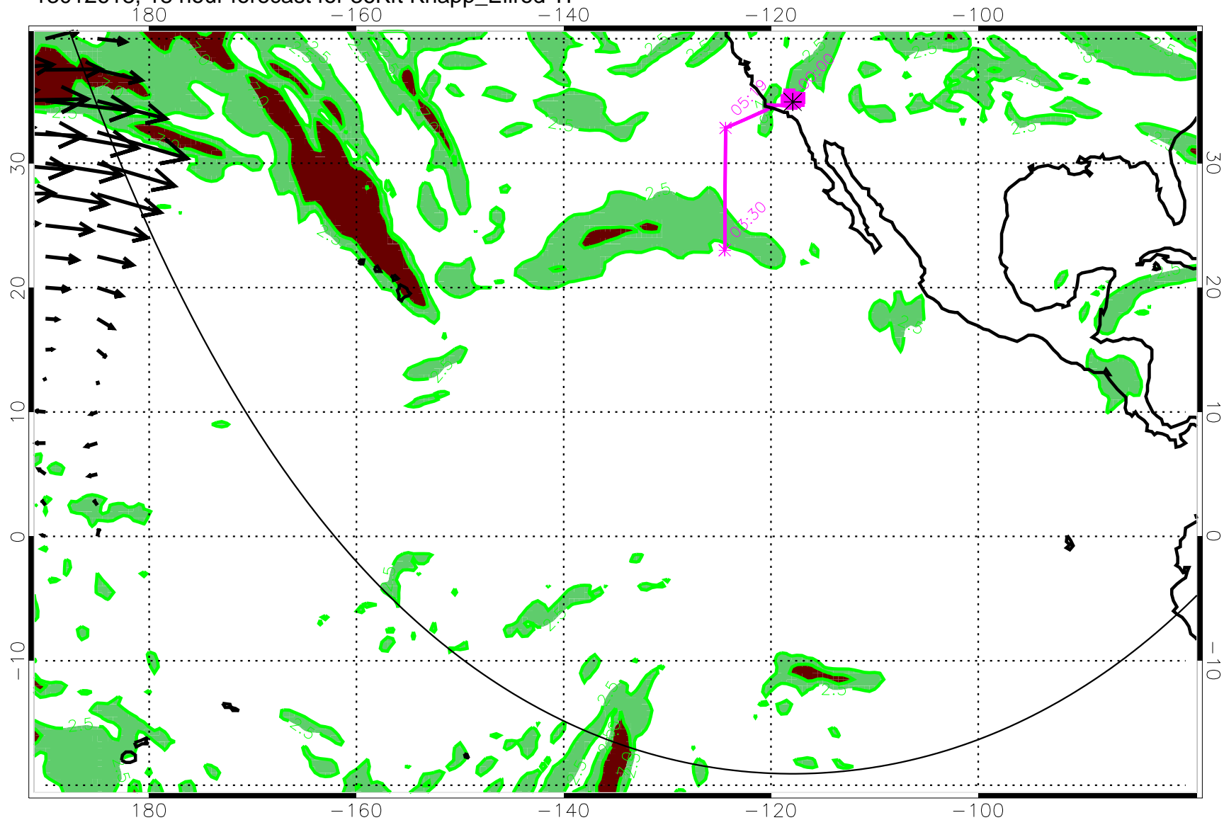
13012618, 18 hour forecast for 36Kft Knapp_Ellrod TI
