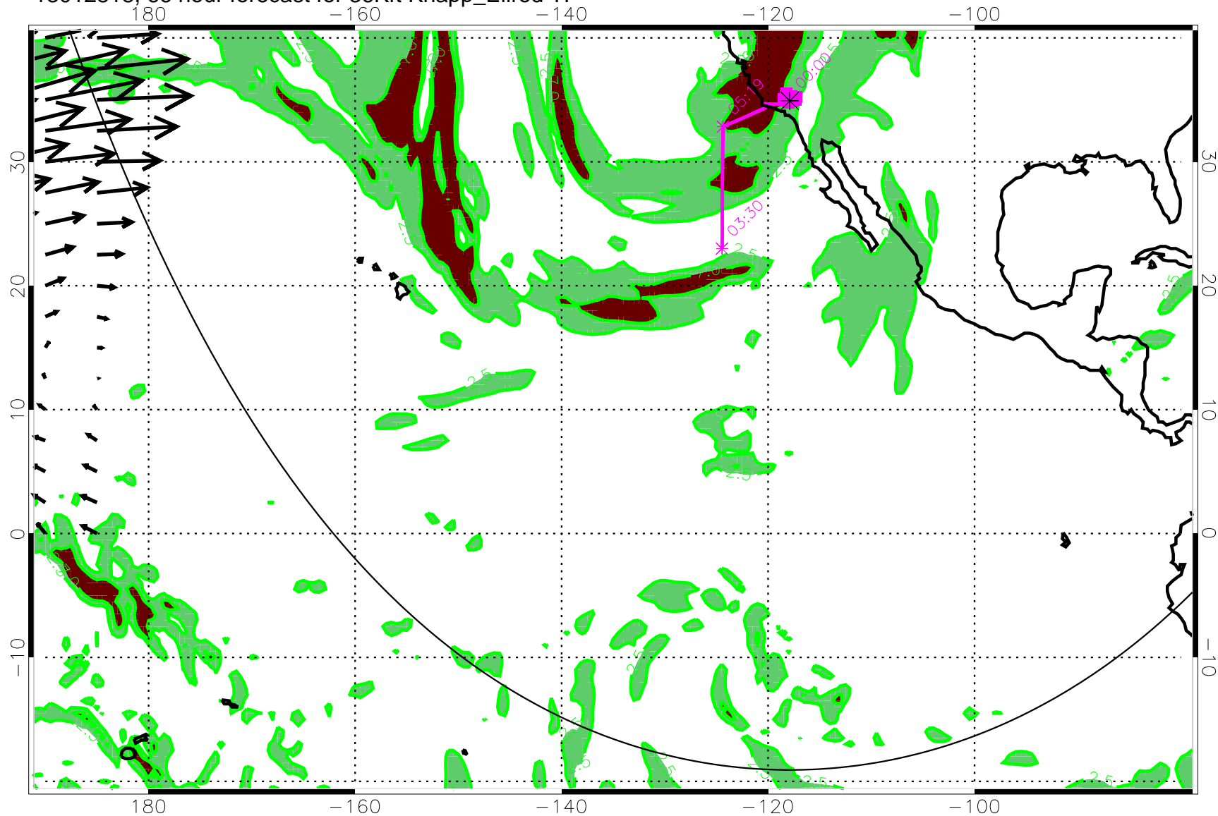
13012818, 66 hour forecast for 36Kft Knapp_Ellrod TI
