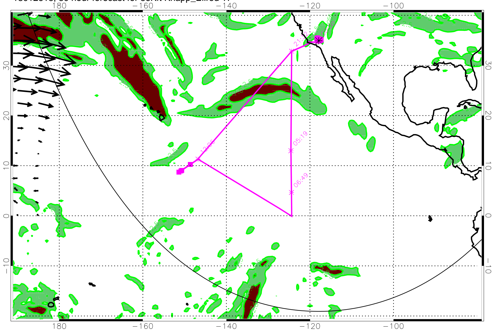
13012618, 30 hour forecast for 36Kft Knapp_Ellrod TI
