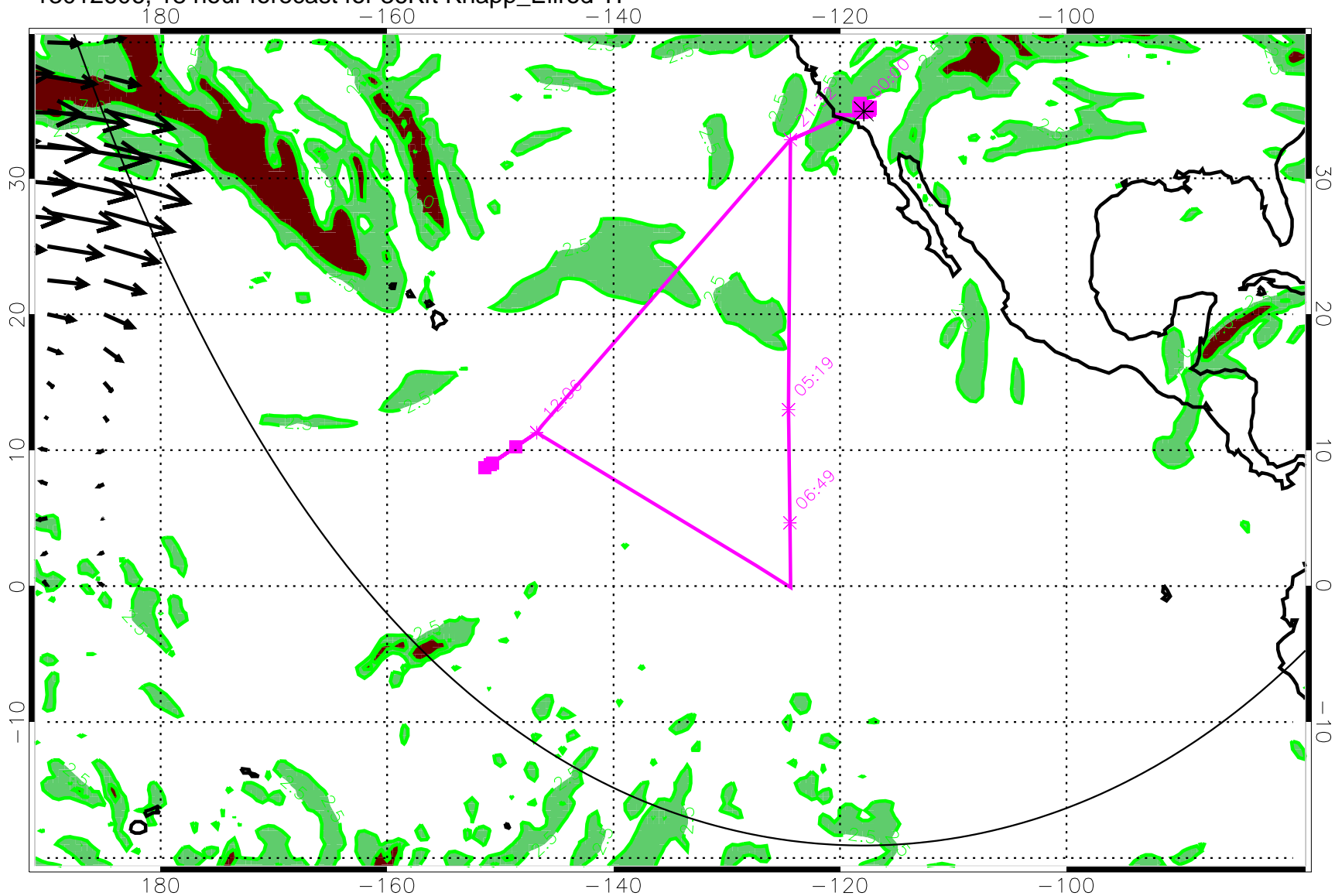
13012606, 18 hour forecast for 36Kft Knapp_Ellrod TI
