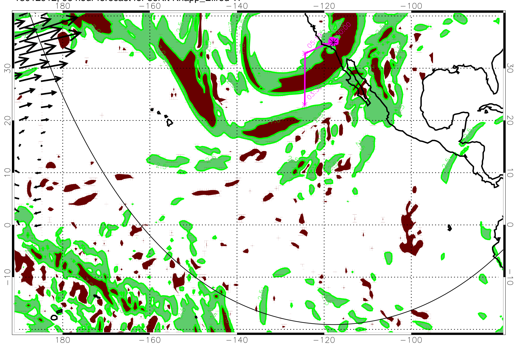
13012912, 96 hour forecast for 36Kft Knapp_Ellrod TI
