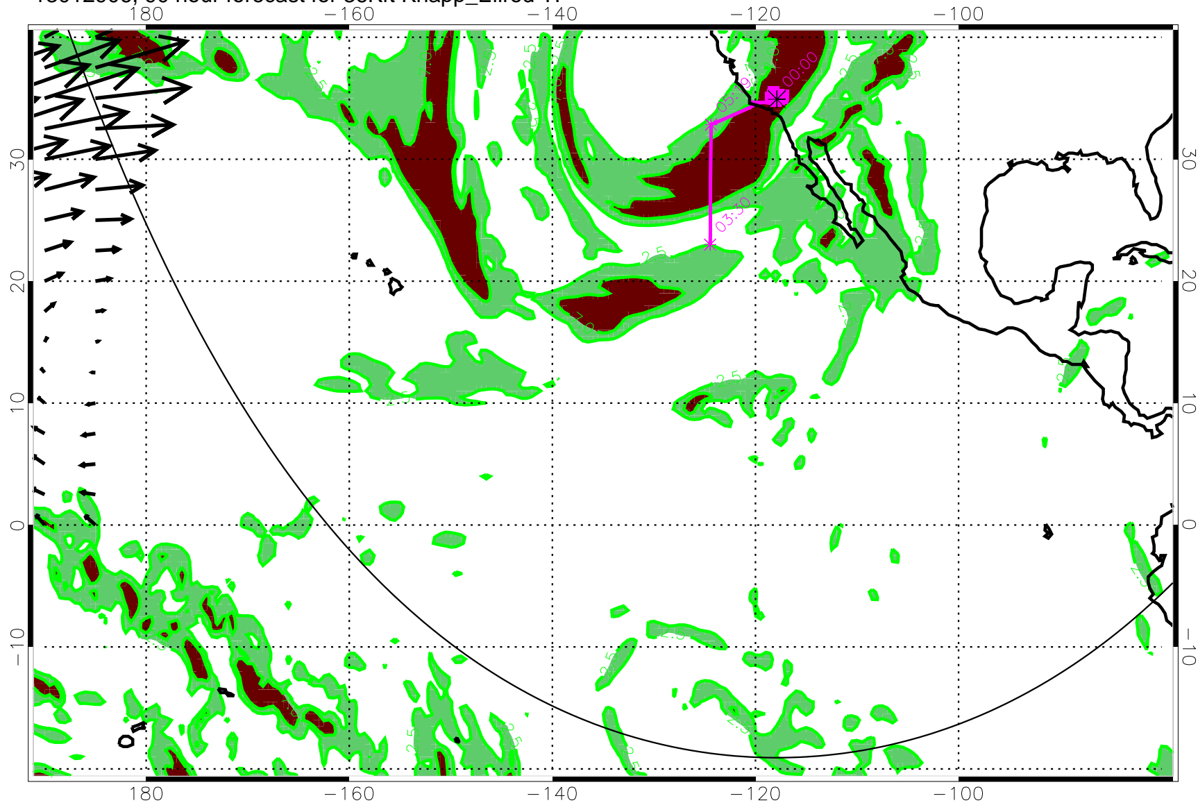
13012906, 90 hour forecast for 36Kft Knapp_Ellrod TI
