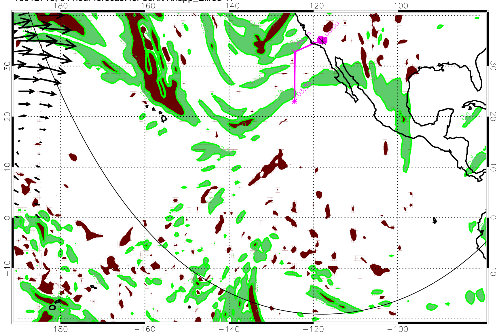
13012718, 54 hour forecast for 36Kft Knapp_Ellrod TI
