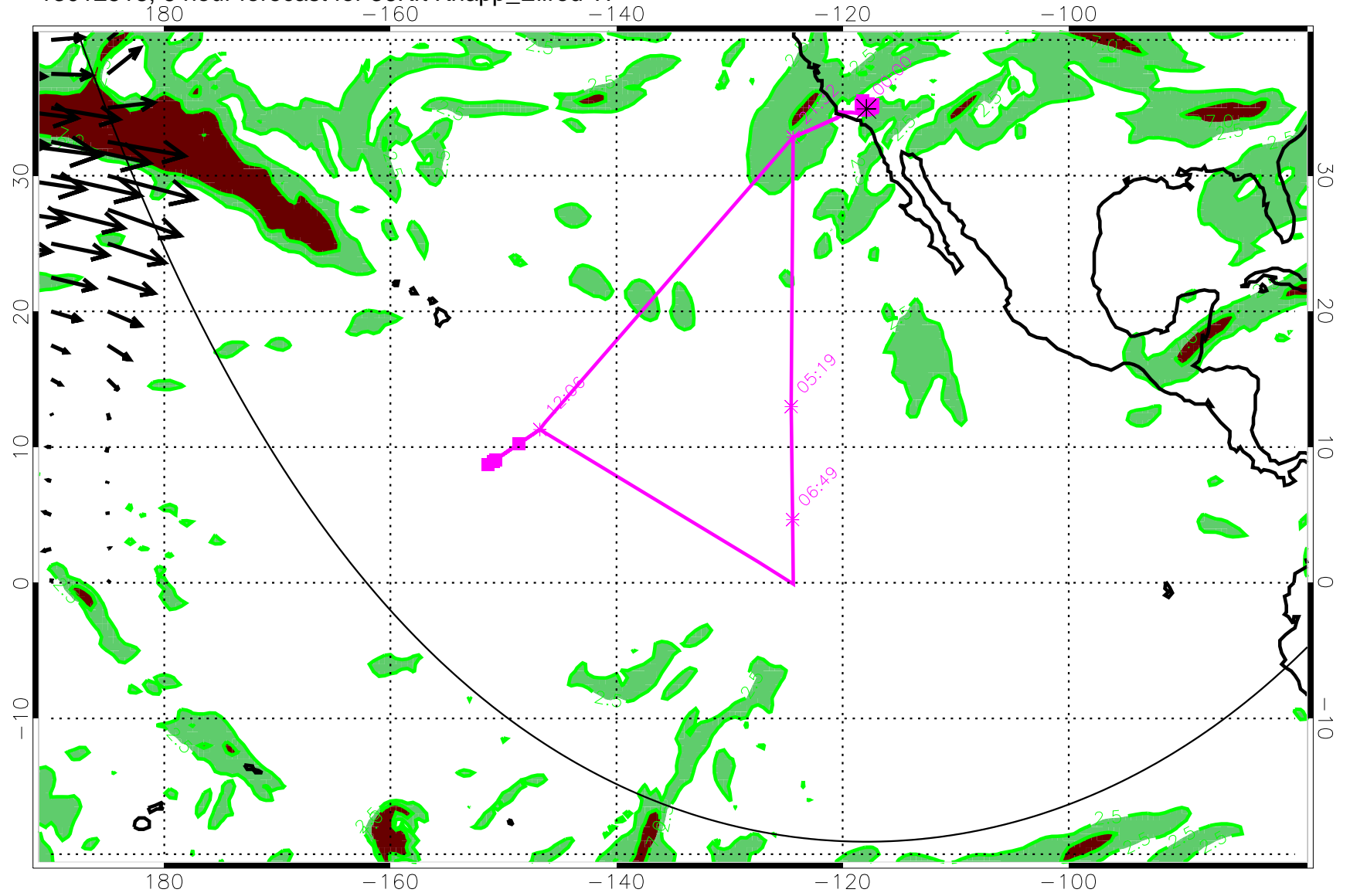
13012518, 6 hour forecast for 36Kft Knapp_Ellrod TI
