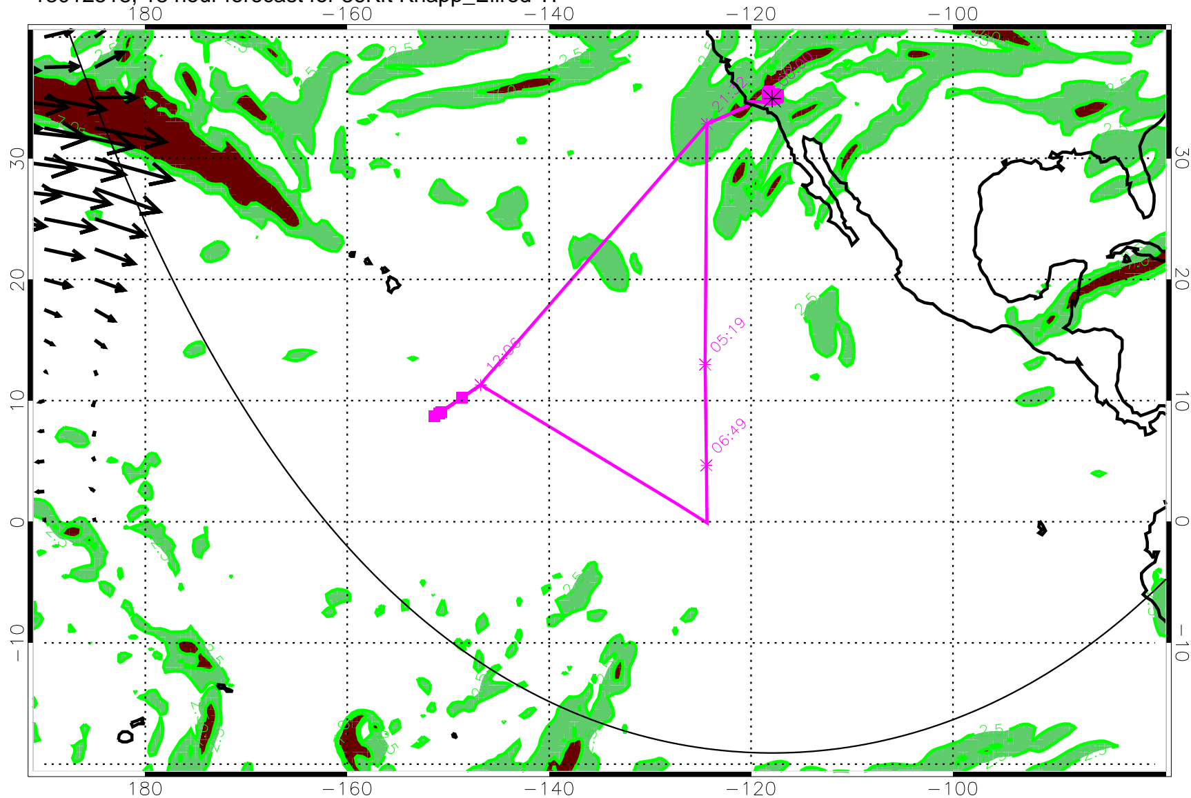
13012518, 18 hour forecast for 36Kft Knapp_Ellrod TI
