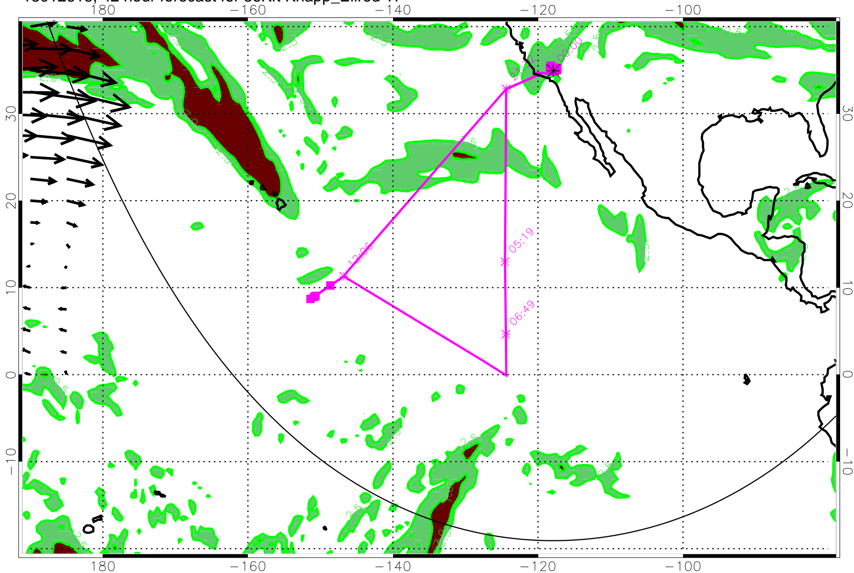
13012618, 42 hour forecast for 36Kft Knapp_Ellrod TI
