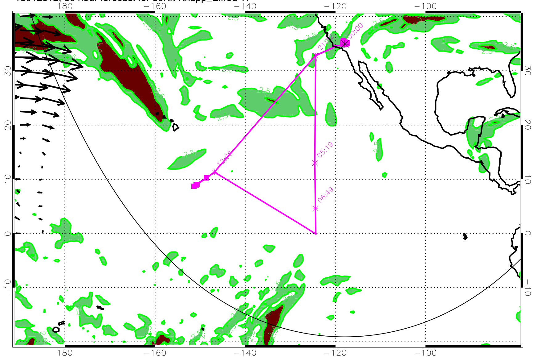
13012612, 36 hour forecast for 36Kft Knapp_Ellrod TI
