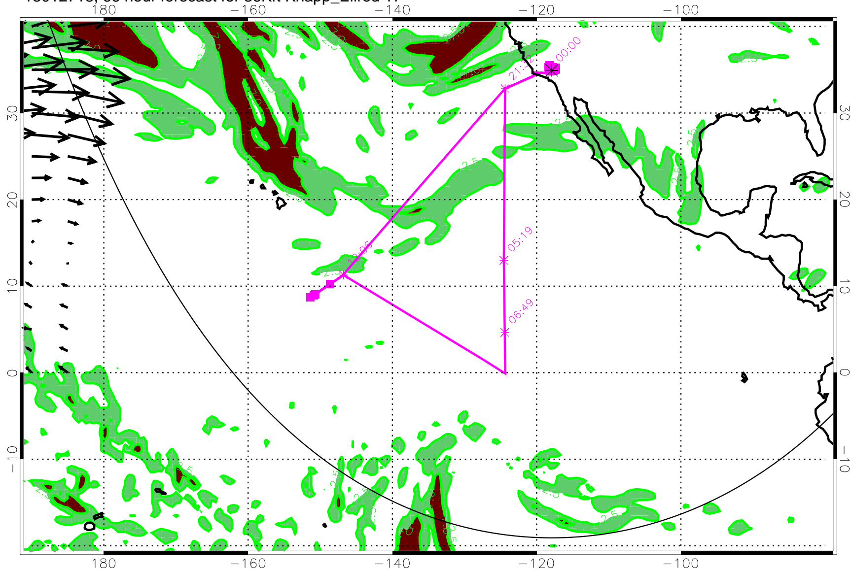
13012718, 66 hour forecast for 36Kft Knapp_Ellrod TI
