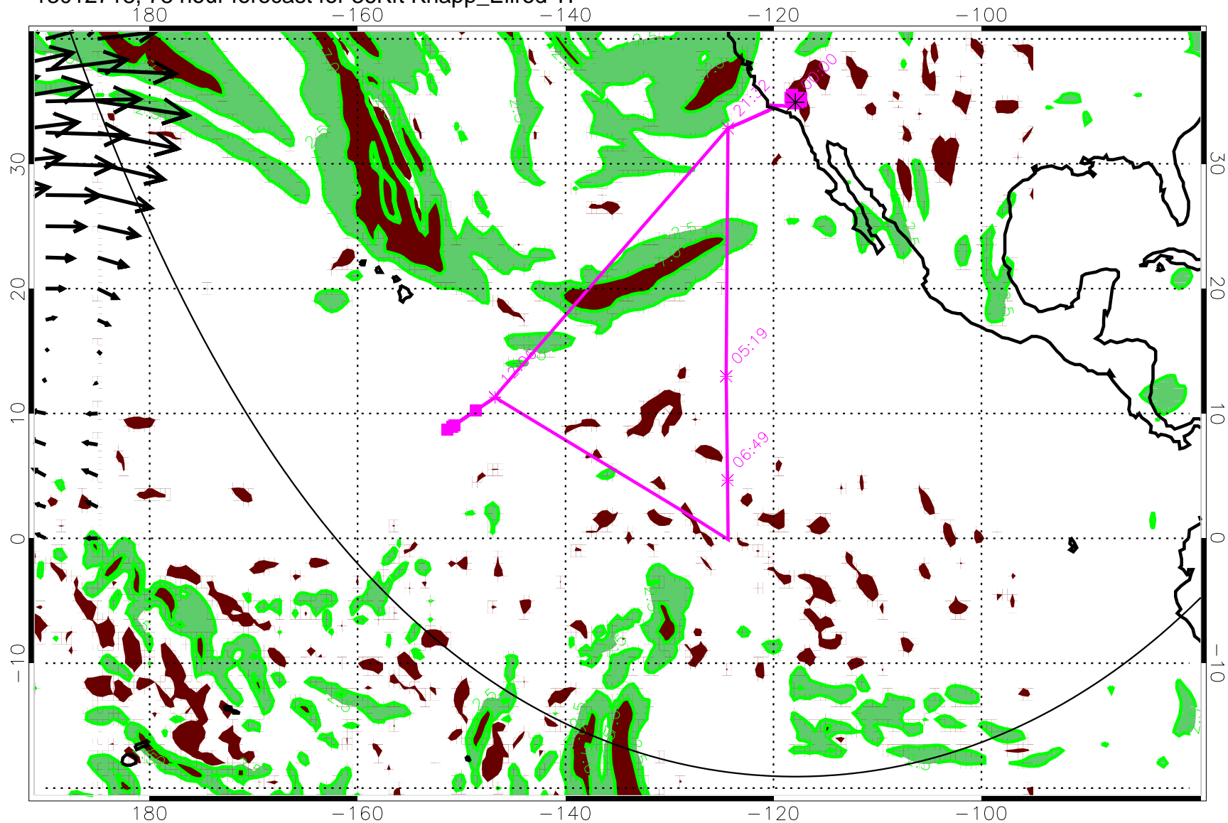
13012718, 78 hour forecast for 36Kft Knapp_Ellrod TI
