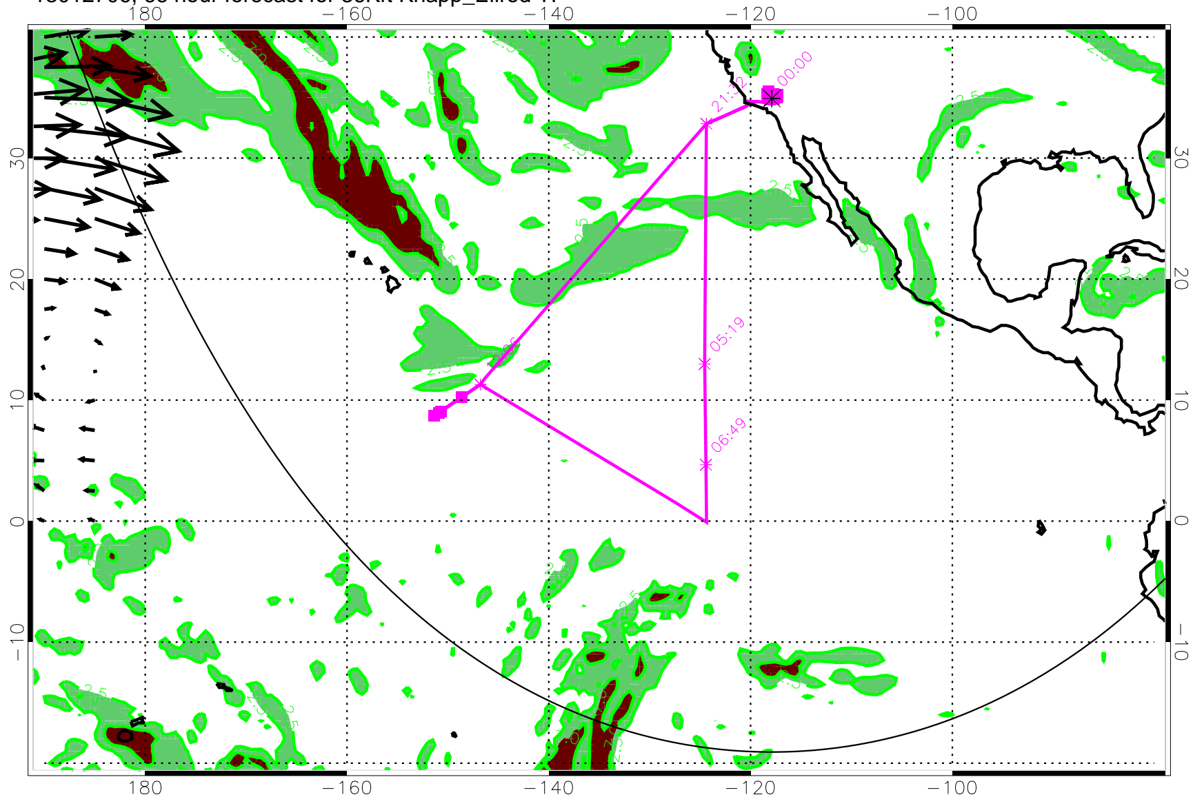
13012706, 66 hour forecast for 36Kft Knapp_Ellrod TI
