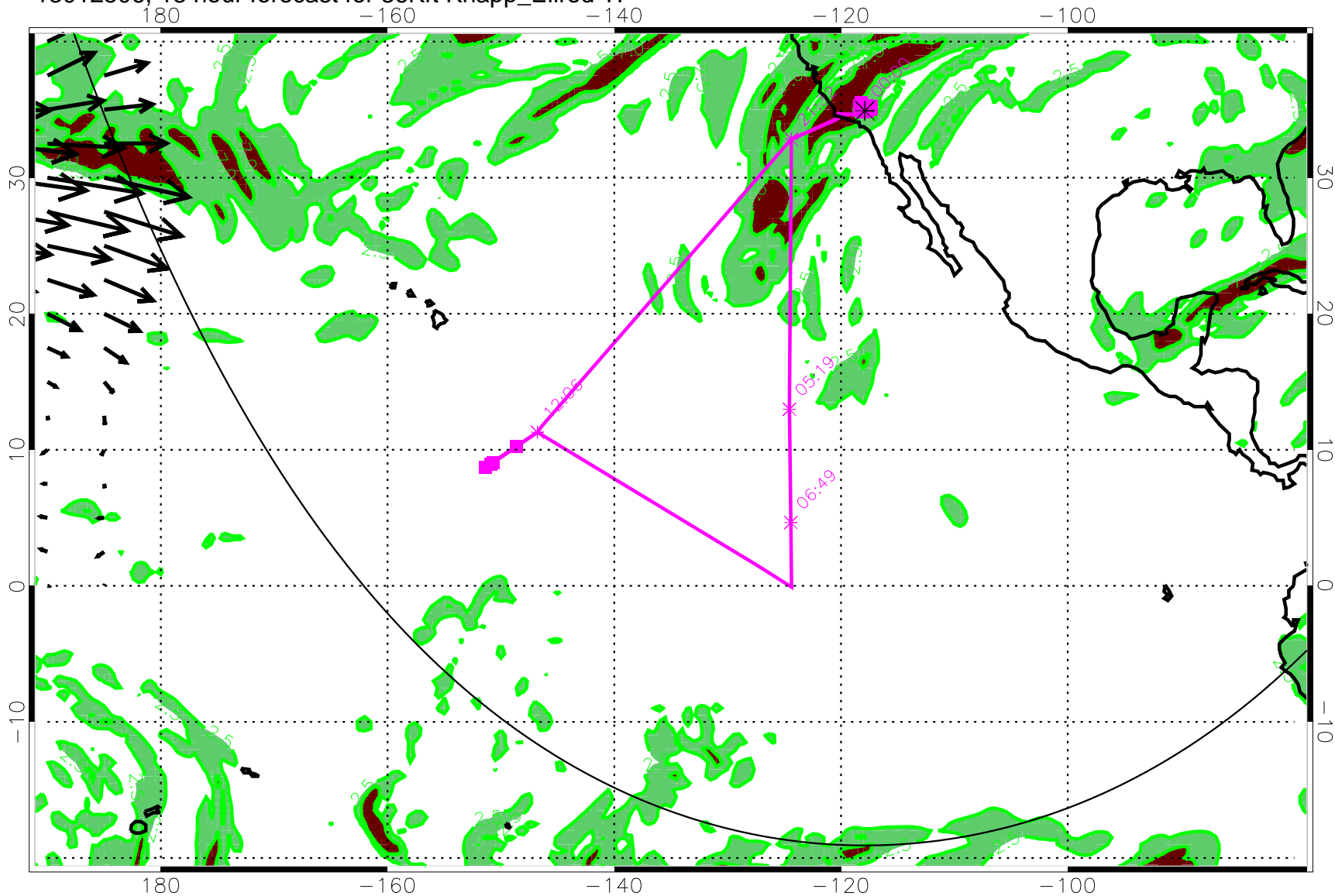
13012506, 18 hour forecast for 36Kft Knapp_Ellrod TI
