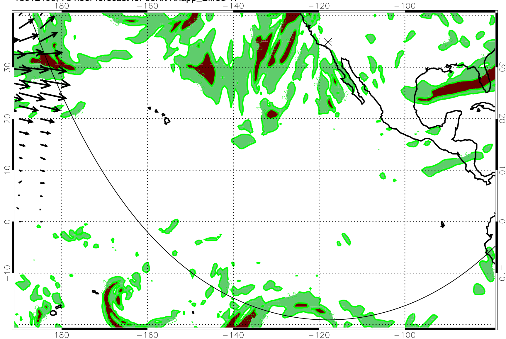
13012406, 78 hour forecast for 36Kft Knapp_Ellrod TI
