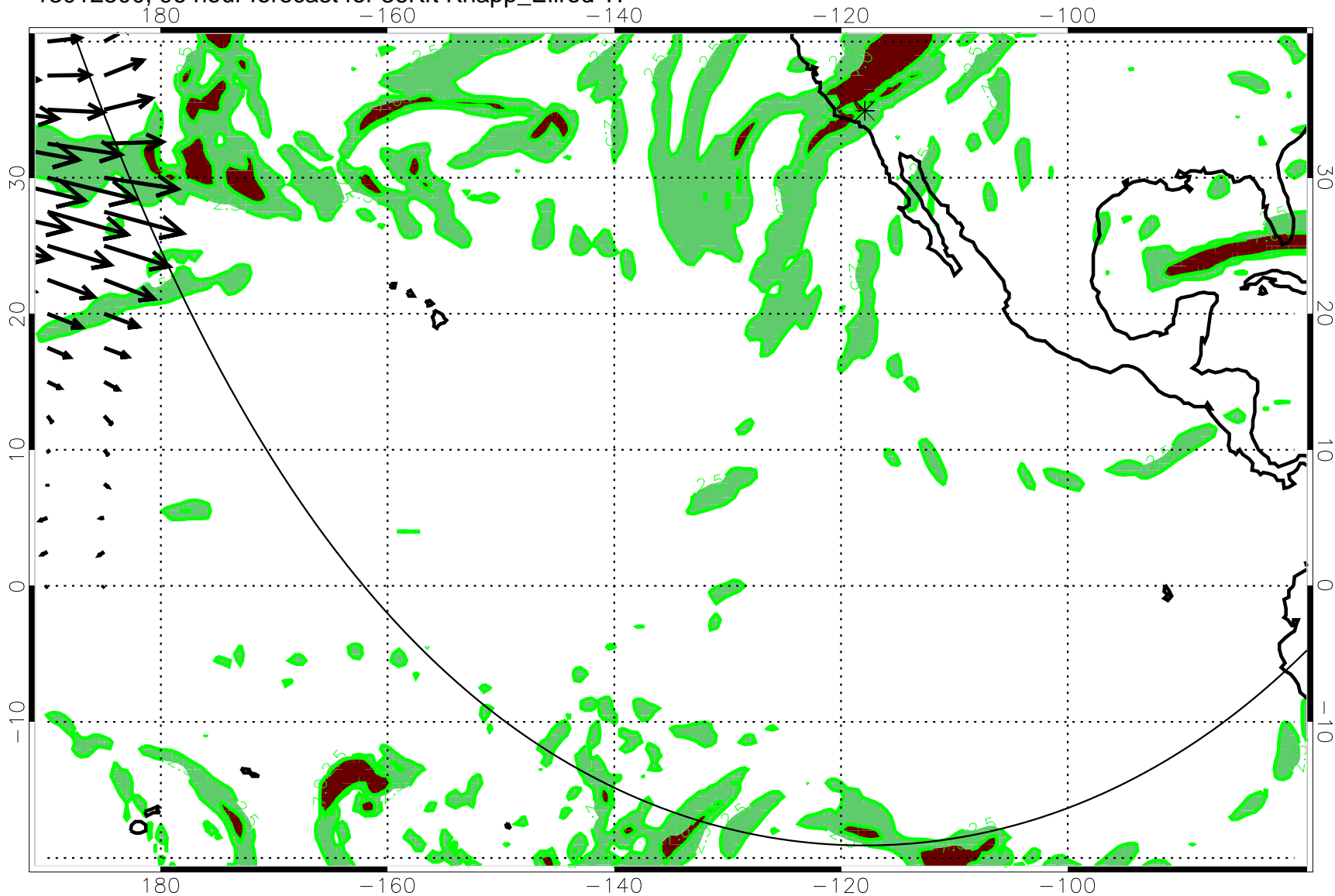
13012500, 96 hour forecast for 36Kft Knapp_Ellrod TI
