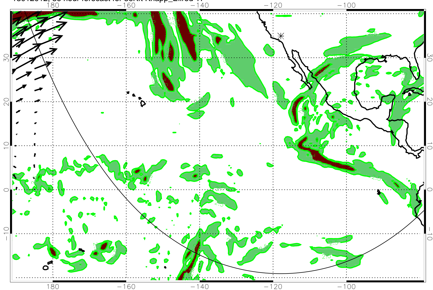
13012012, 36 hour forecast for 36Kft Knapp_Ellrod TI
