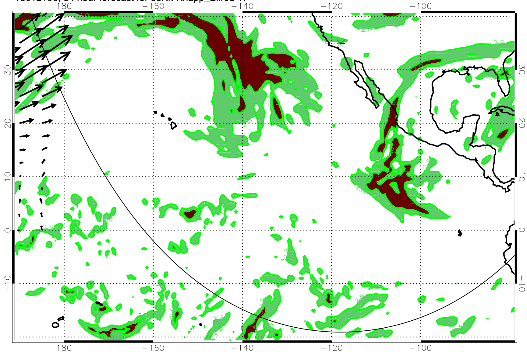
13012106, 54 hour forecast for 36Kft Knapp_Ellrod TI
