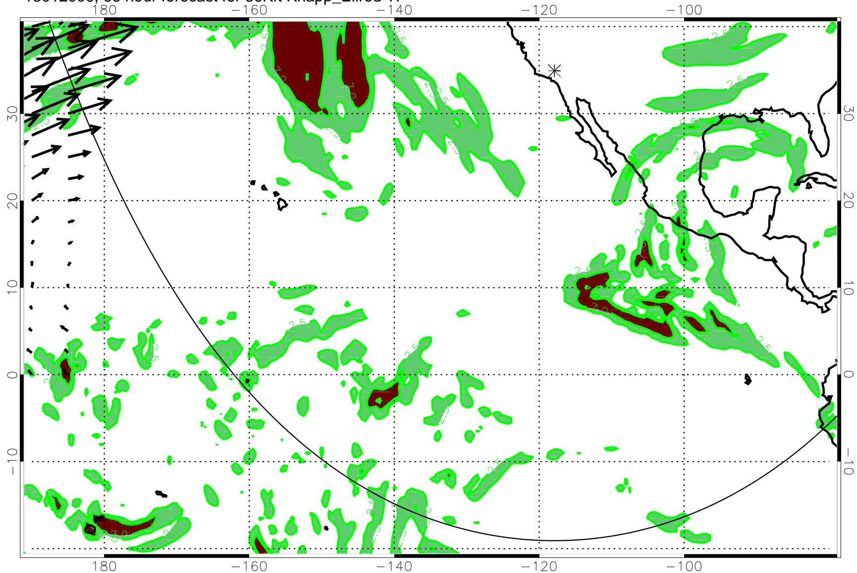
13012006, 66 hour forecast for 36Kft Knapp_Ellrod TI
