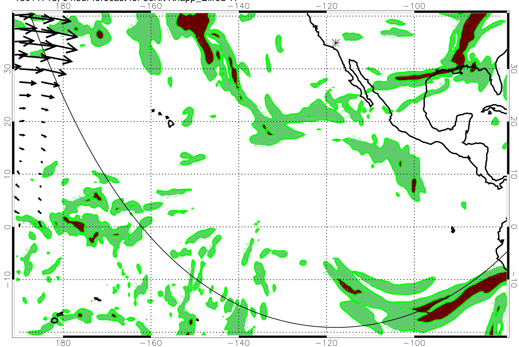
13011718, 6 hour forecast for 36Kft Knapp_Ellrod TI
