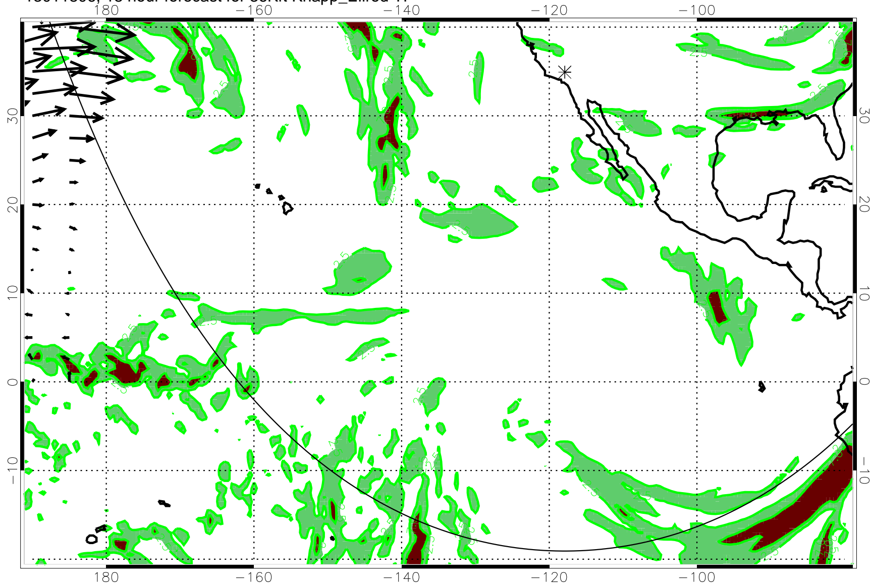
13011806, 18 hour forecast for 36Kft Knapp_Ellrod TI
