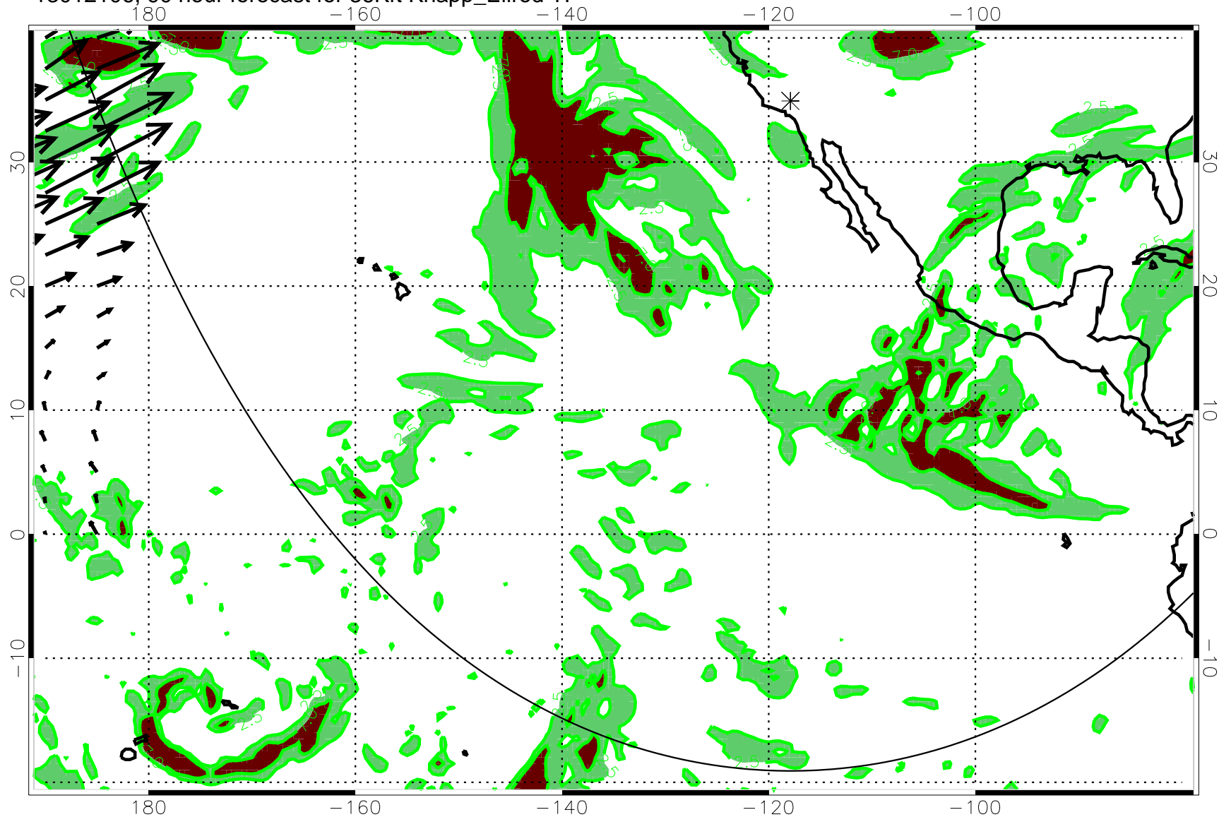
13012106, 90 hour forecast for 36Kft Knapp_Ellrod TI
