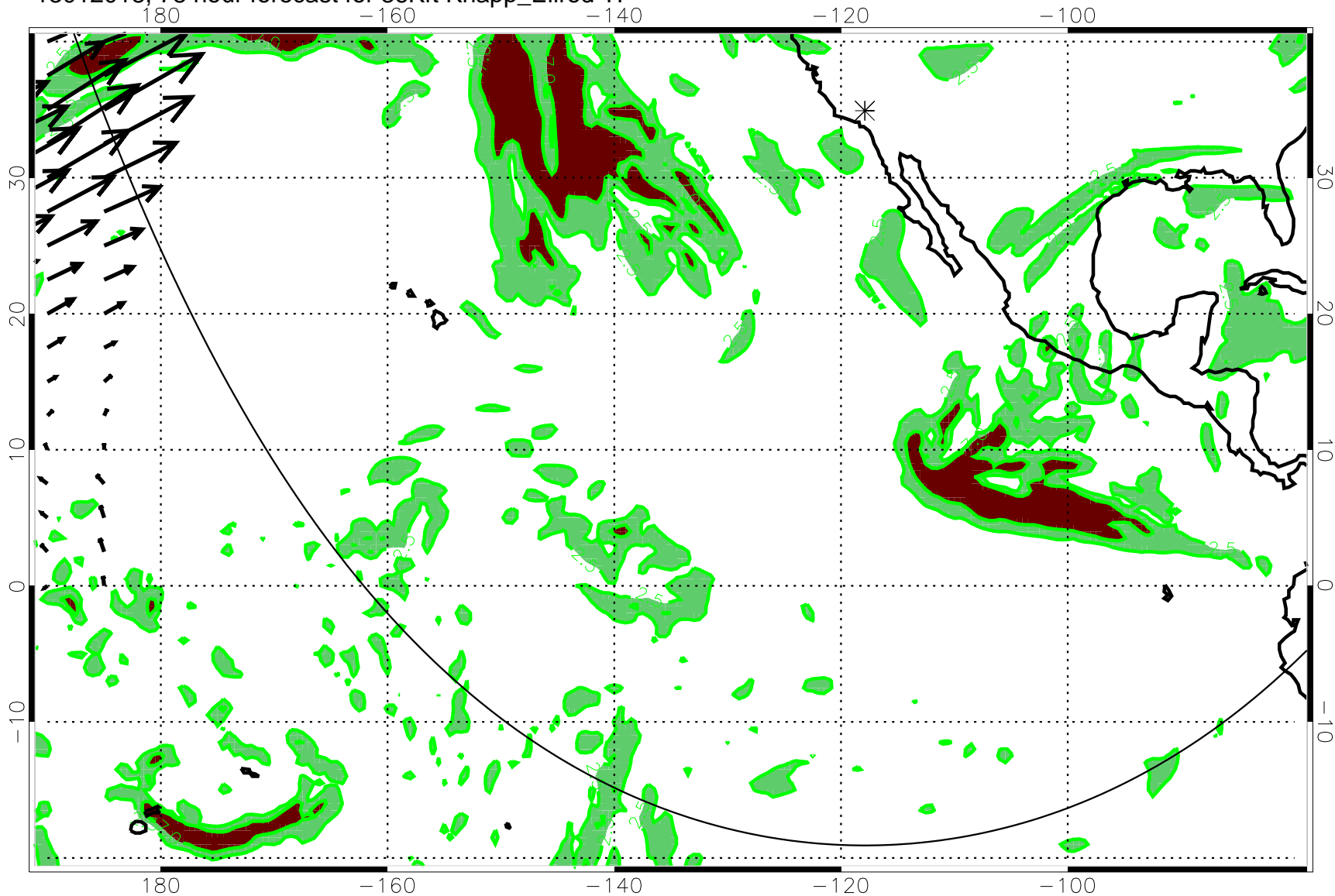
13012018, 78 hour forecast for 36Kft Knapp_Ellrod TI
