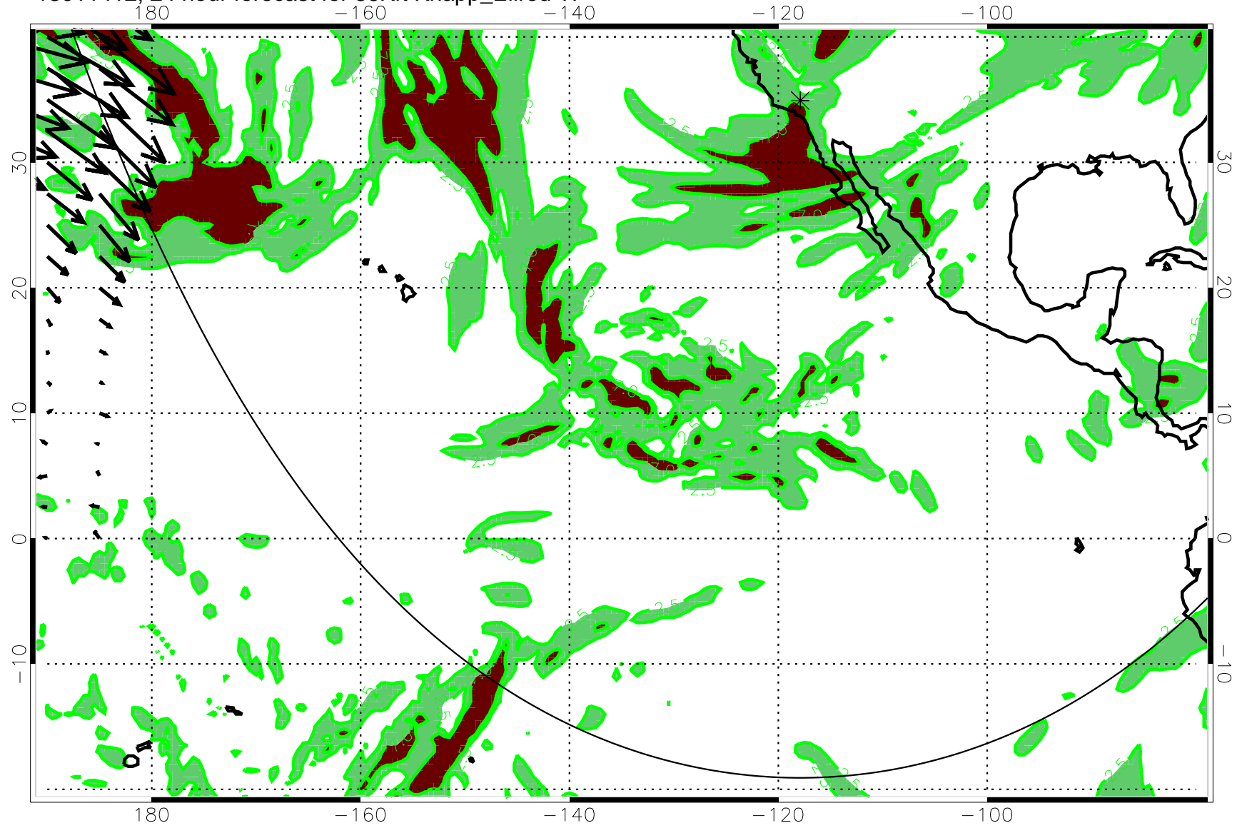
13011412, 24 hour forecast for 36Kft Knapp_Ellrod TI
