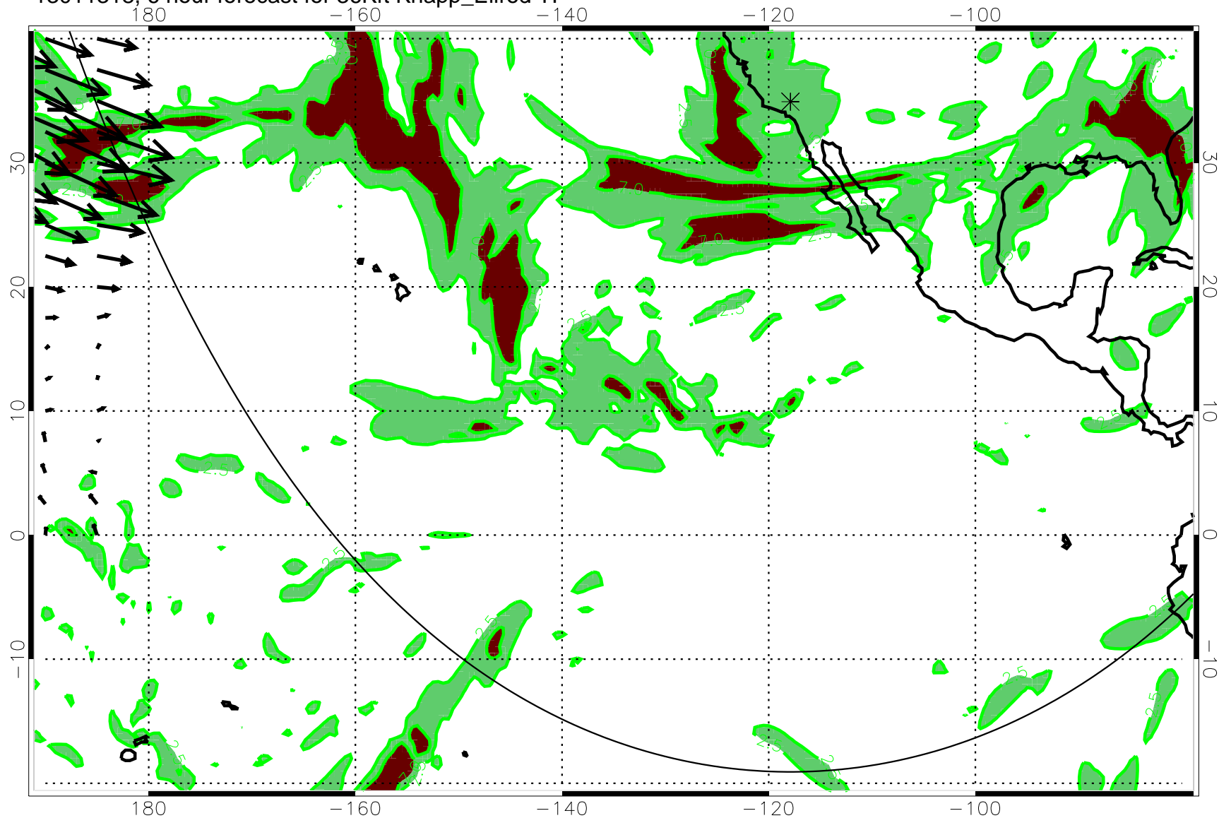
13011318, 6 hour forecast for 36Kft Knapp_Ellrod TI
