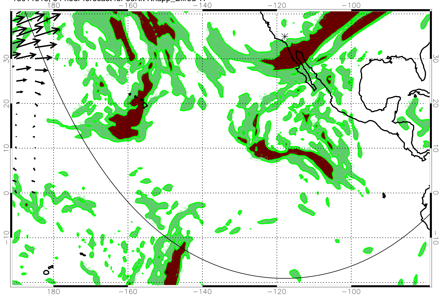
13011518, 54 hour forecast for 36Kft Knapp_Ellrod TI
