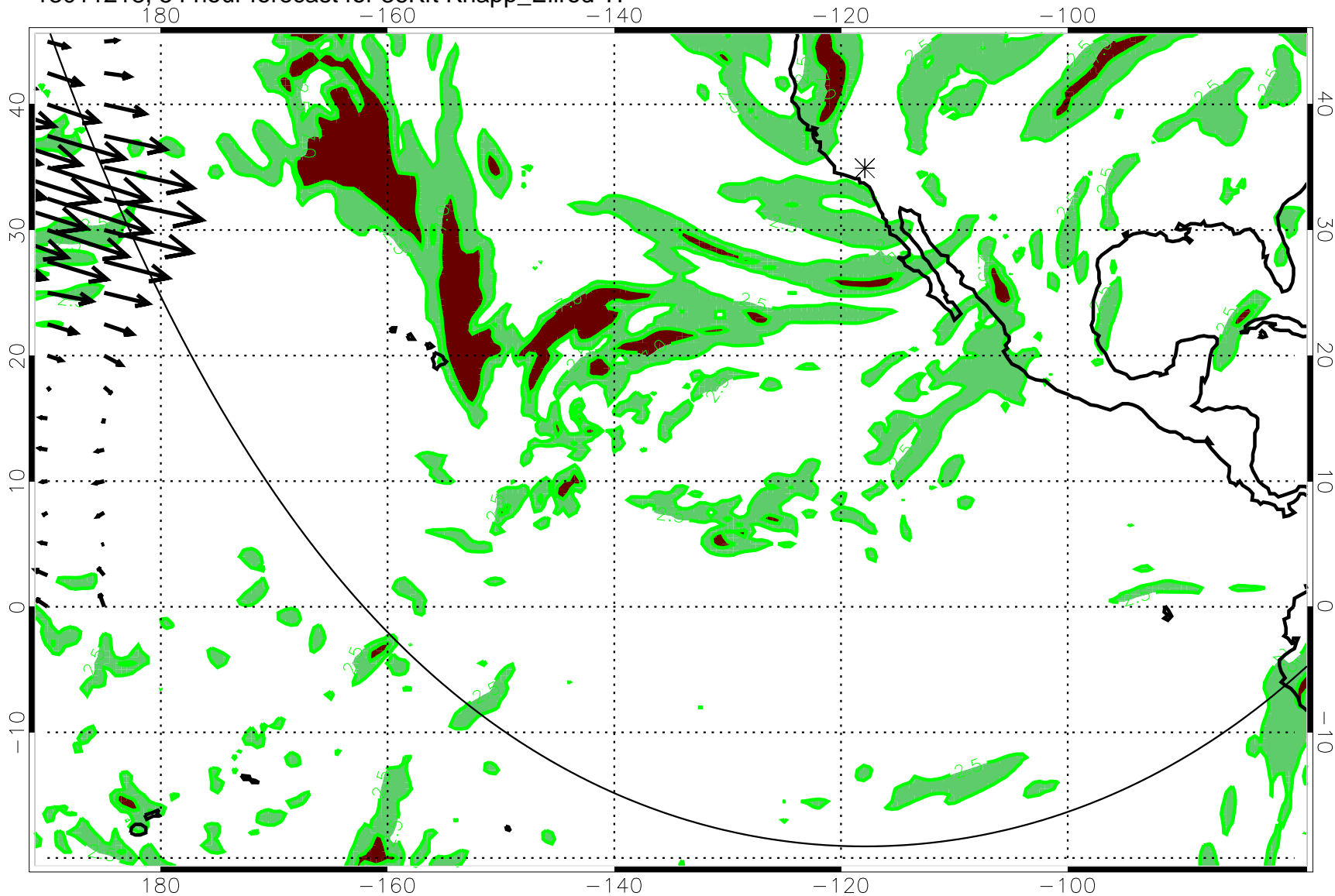
13011218, 54 hour forecast for 36Kft Knapp_Ellrod TI
