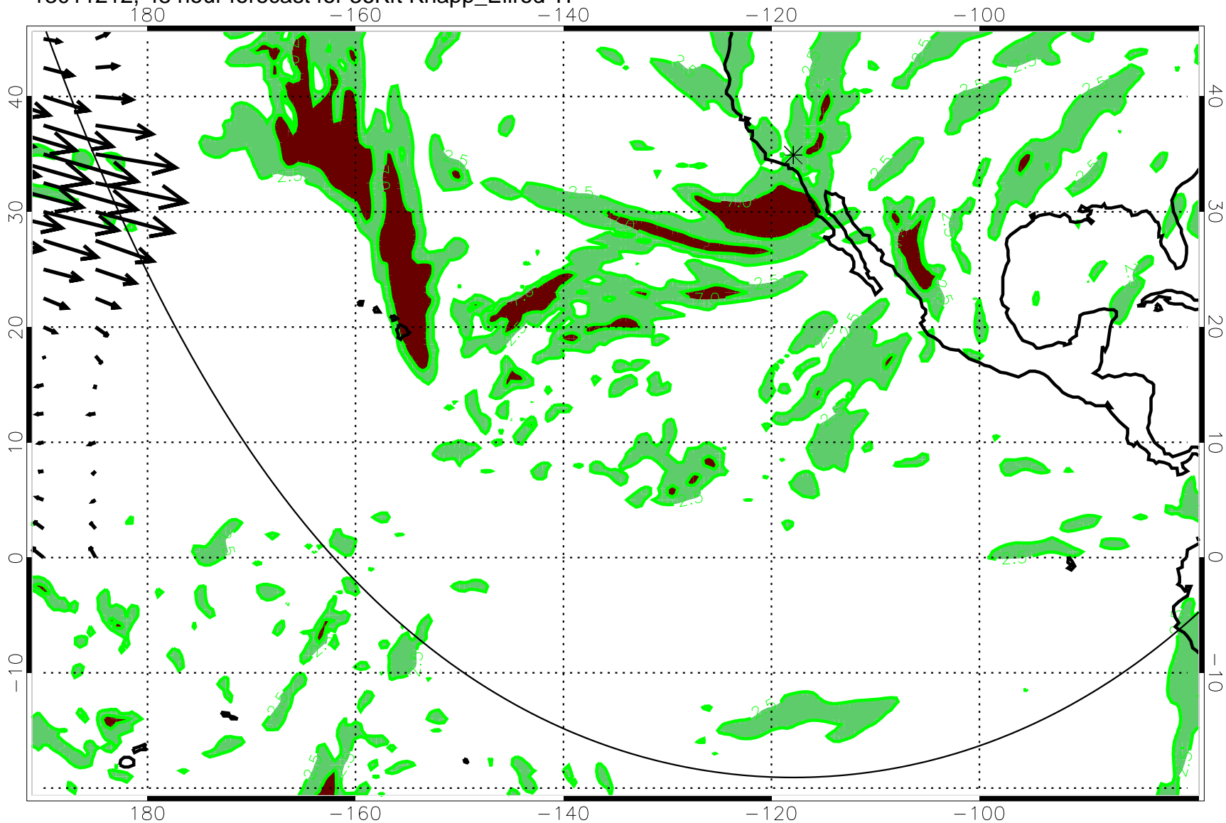
13011212, 48 hour forecast for 36Kft Knapp_Ellrod TI
