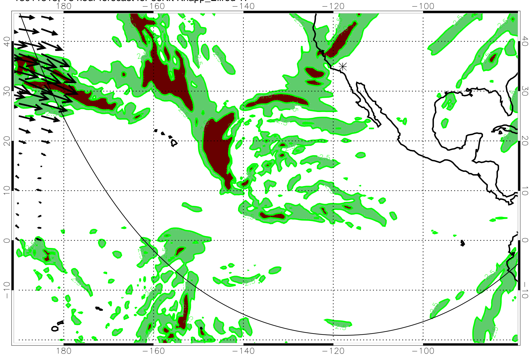
13011318, 78 hour forecast for 36Kft Knapp_Ellrod TI
