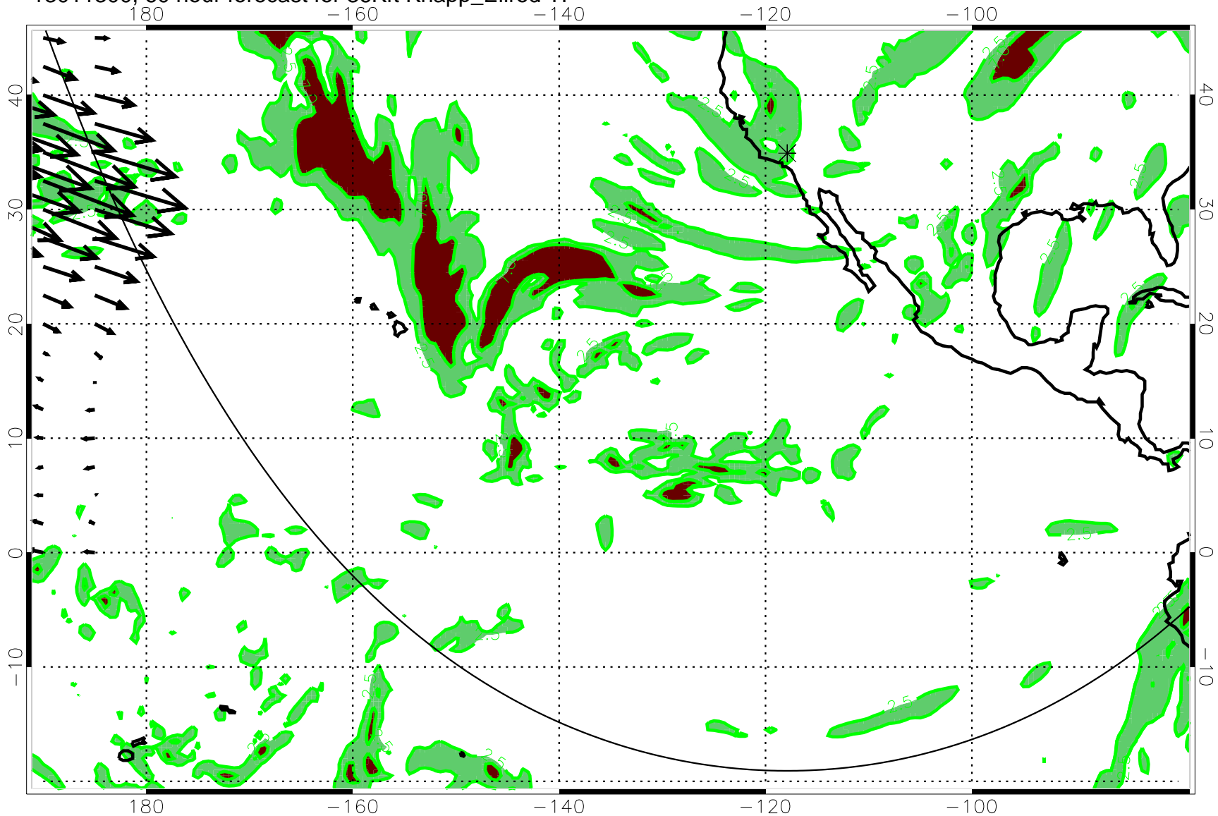
13011300, 60 hour forecast for 36Kft Knapp_Ellrod TI
