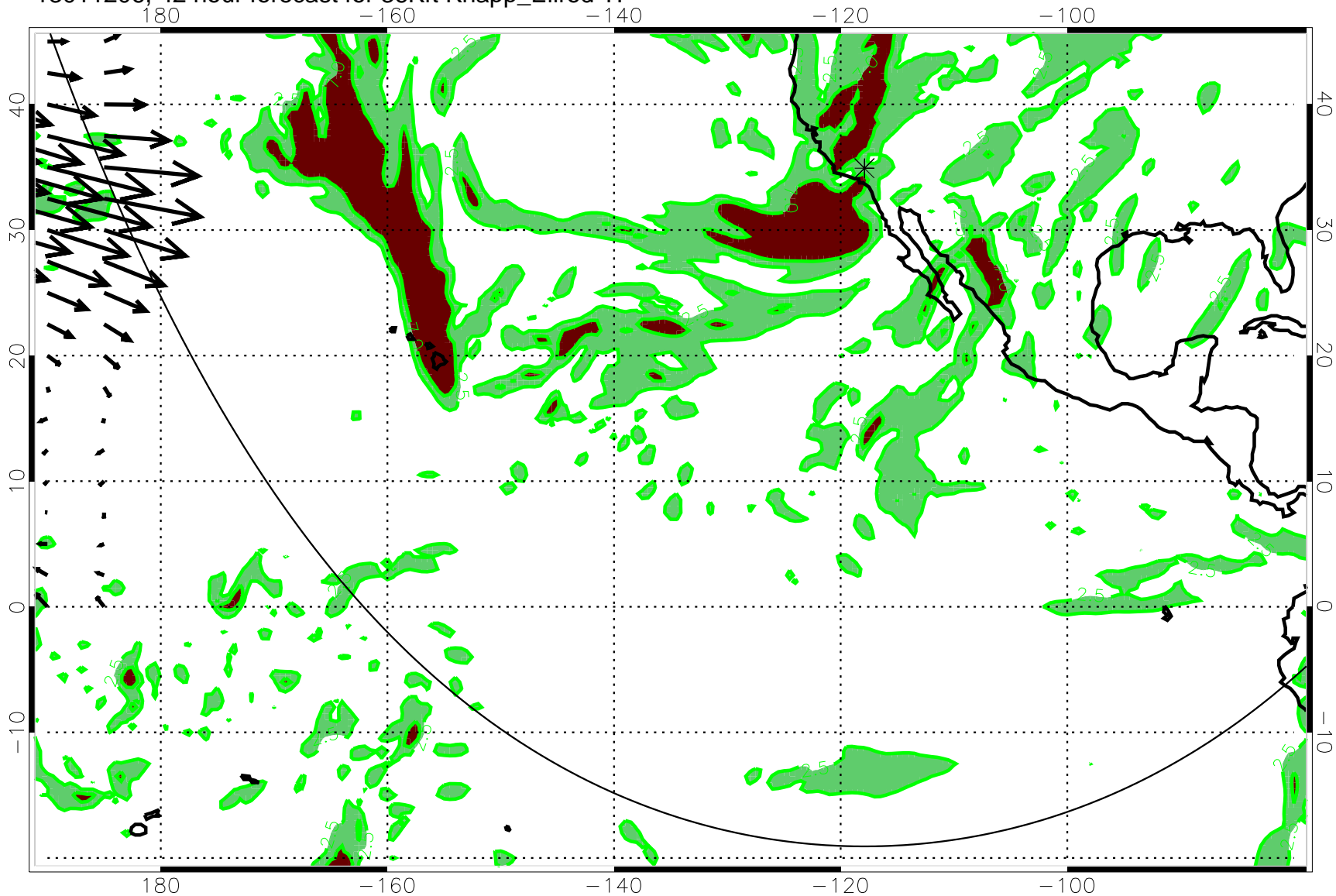
13011206, 42 hour forecast for 36Kft Knapp_Ellrod TI
