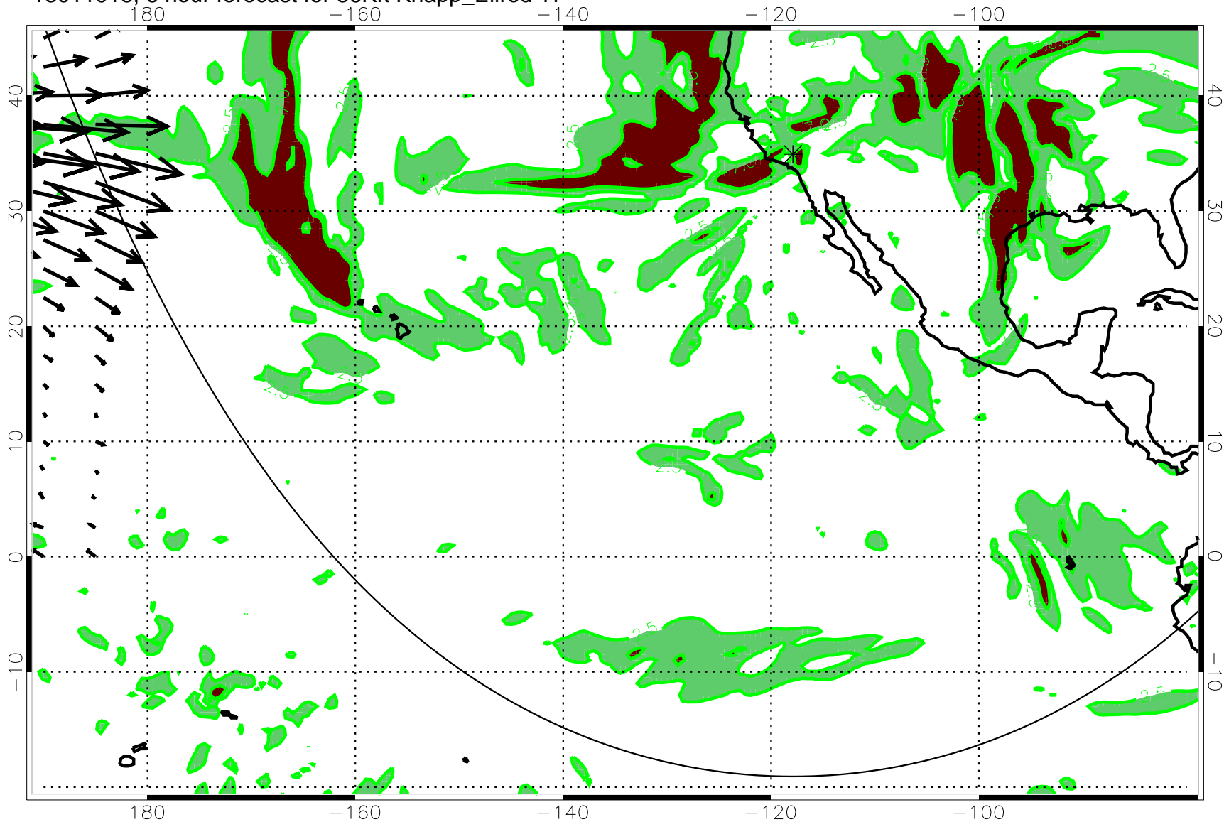
13011018, 6 hour forecast for 36Kft Knapp_Ellrod TI
