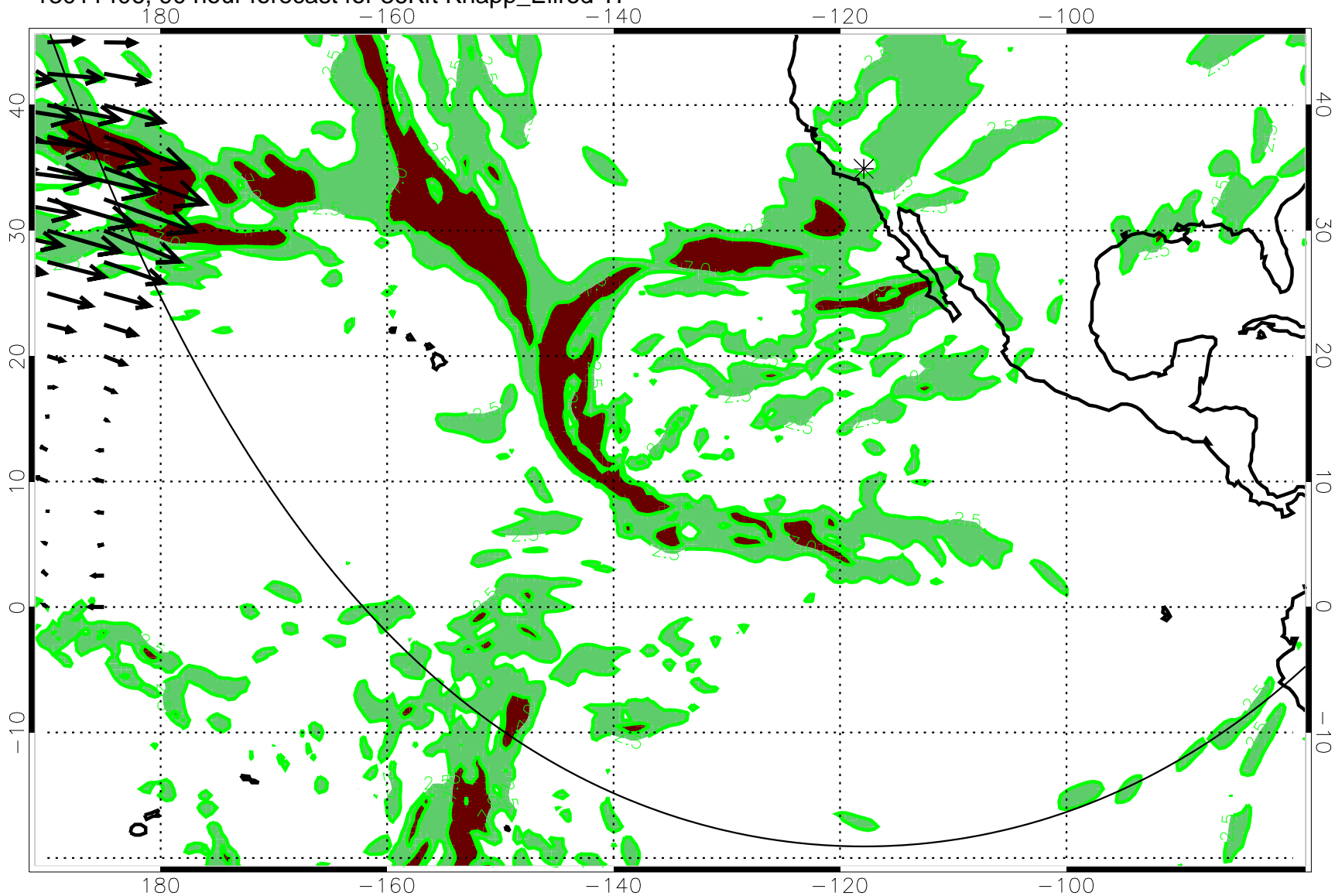
13011406, 90 hour forecast for 36Kft Knapp_Ellrod TI
