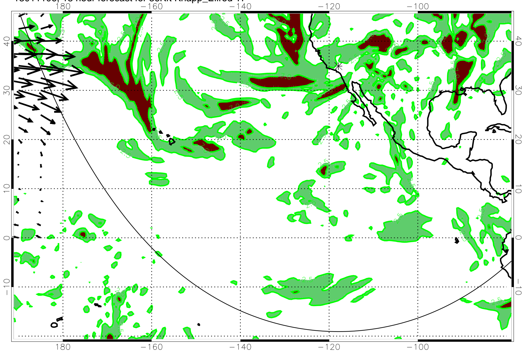
13011106, 18 hour forecast for 36Kft Knapp_Ellrod TI
