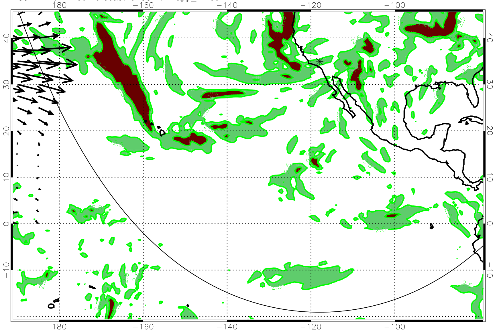
13011112, 24 hour forecast for 36Kft Knapp_Ellrod TI
