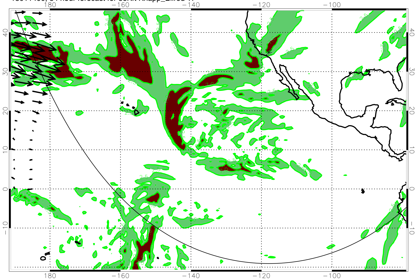
13011400, 84 hour forecast for 36Kft Knapp_Ellrod TI
