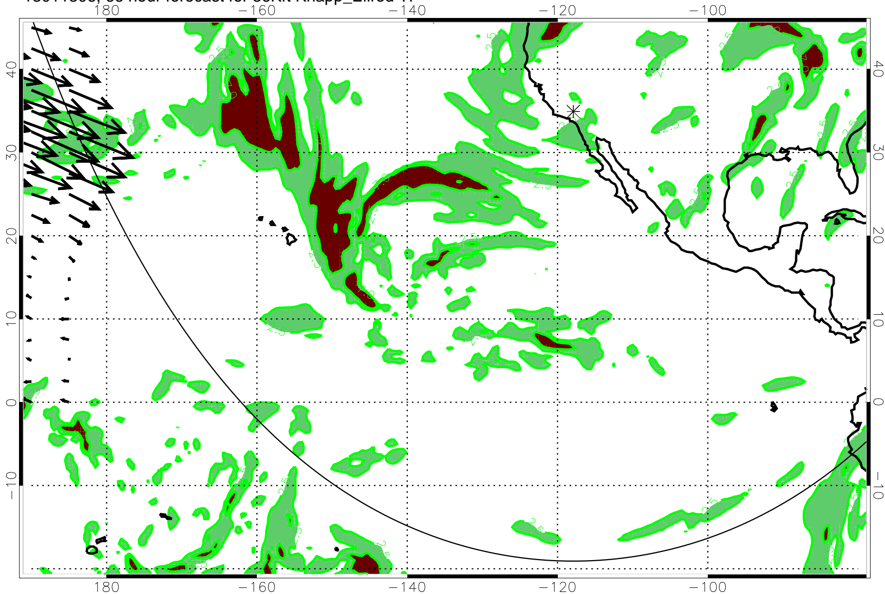
13011306, 66 hour forecast for 36Kft Knapp_Ellrod TI
