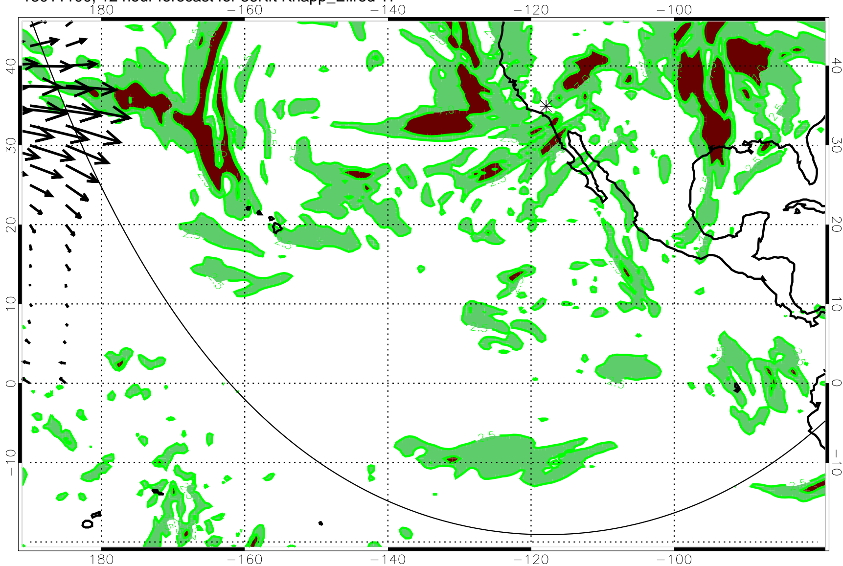
13011100, 12 hour forecast for 36Kft Knapp_Ellrod TI
