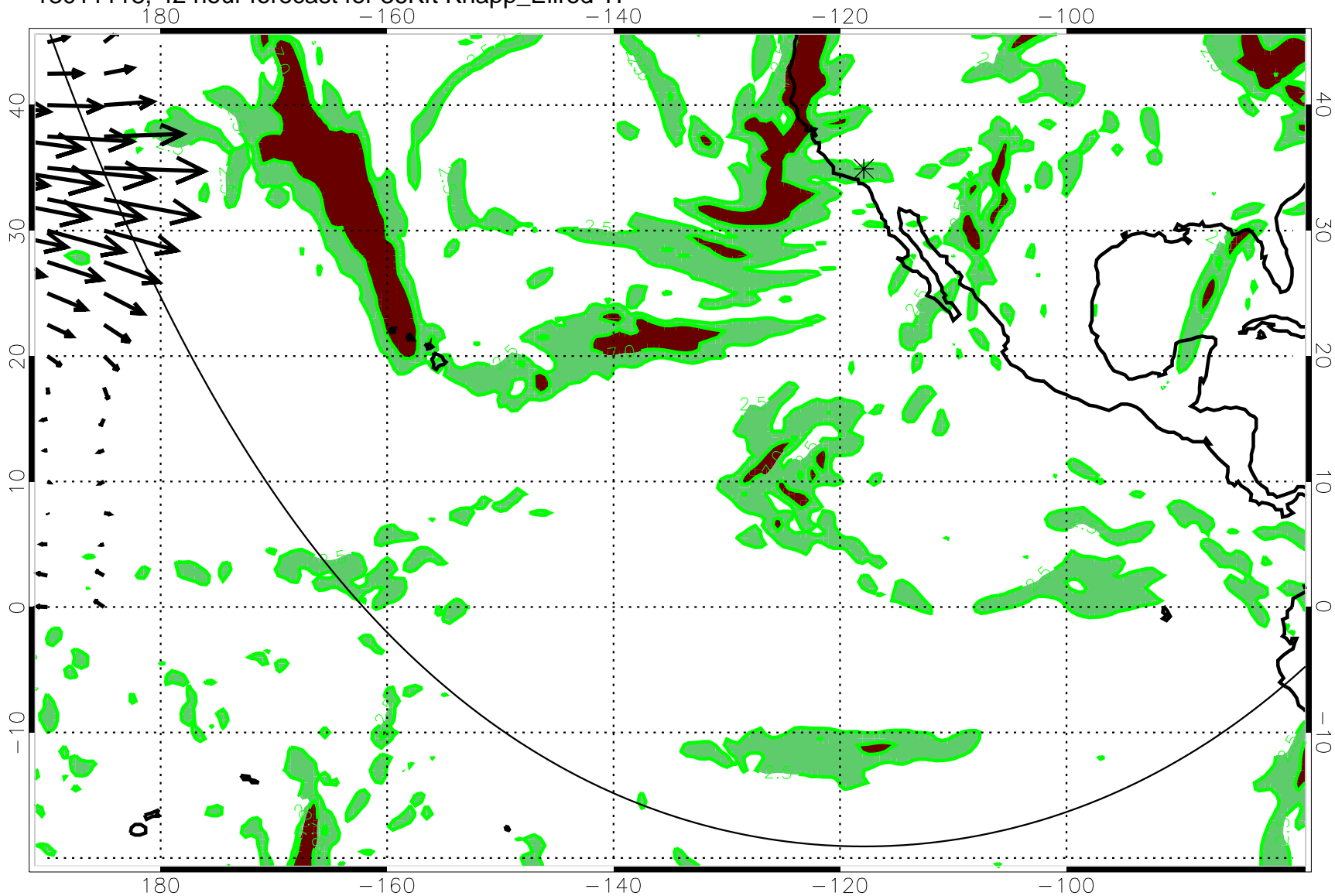
13011118, 42 hour forecast for 36Kft Knapp_Ellrod TI
