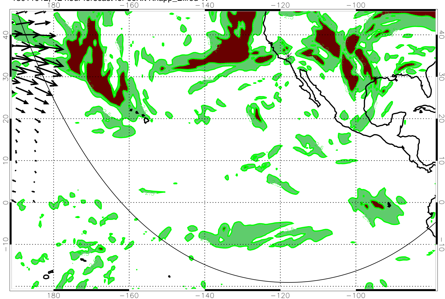
13011012, 12 hour forecast for 36Kft Knapp_Ellrod TI
