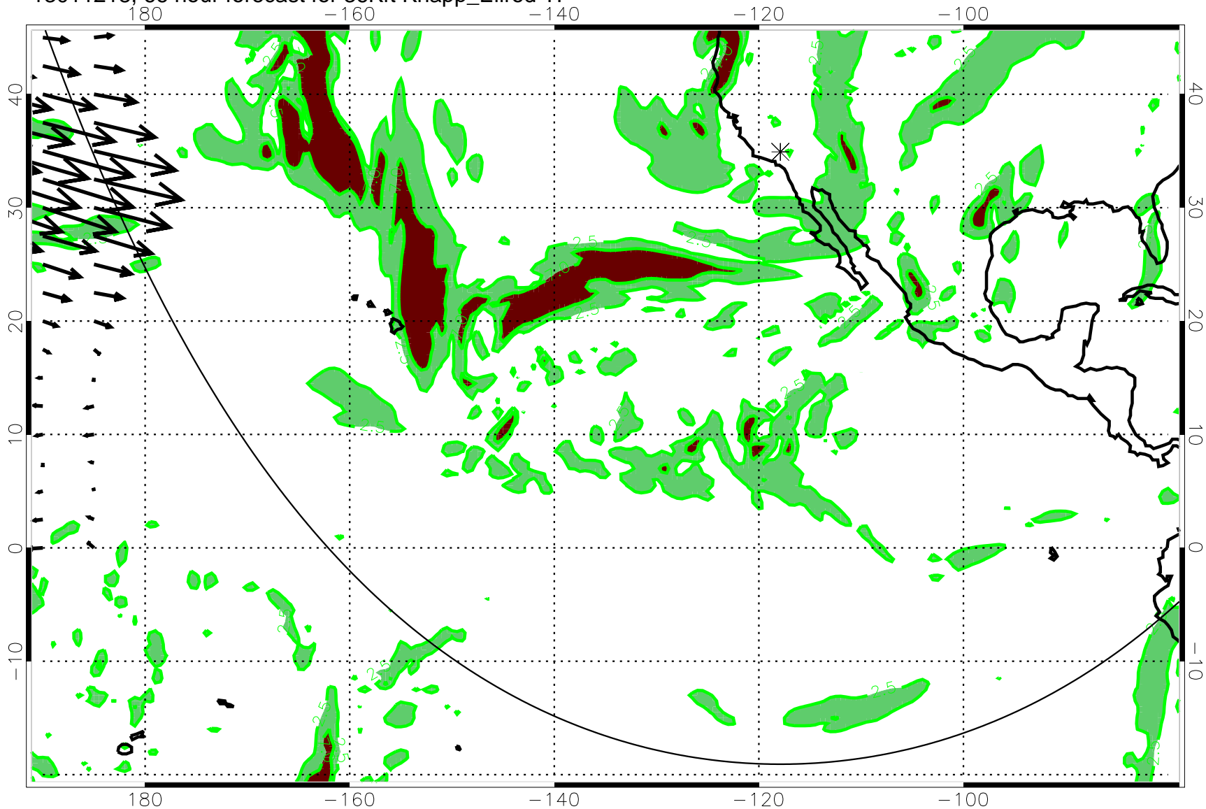
13011218, 66 hour forecast for 36Kft Knapp_Ellrod TI
