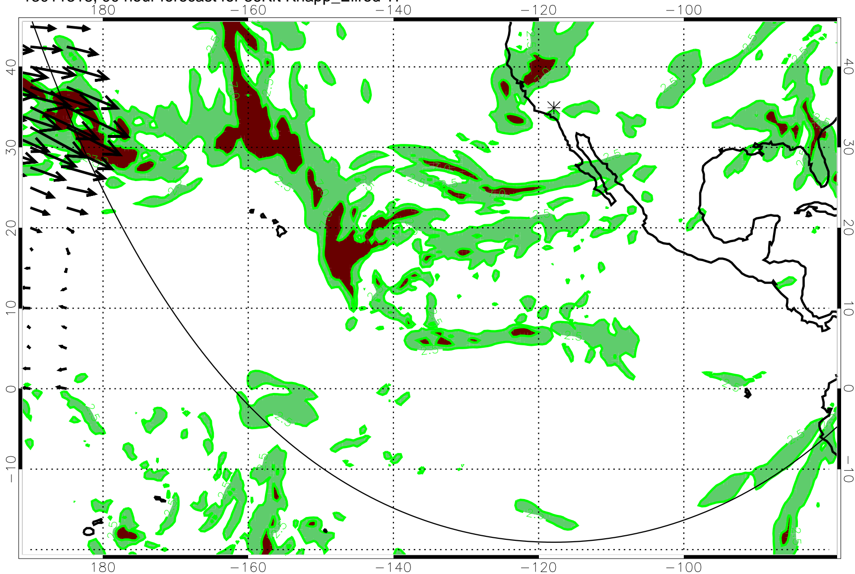
13011318, 90 hour forecast for 36Kft Knapp_Ellrod TI
