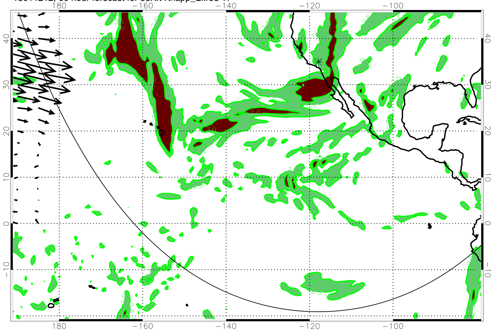
13011212, 60 hour forecast for 36Kft Knapp_Ellrod TI
