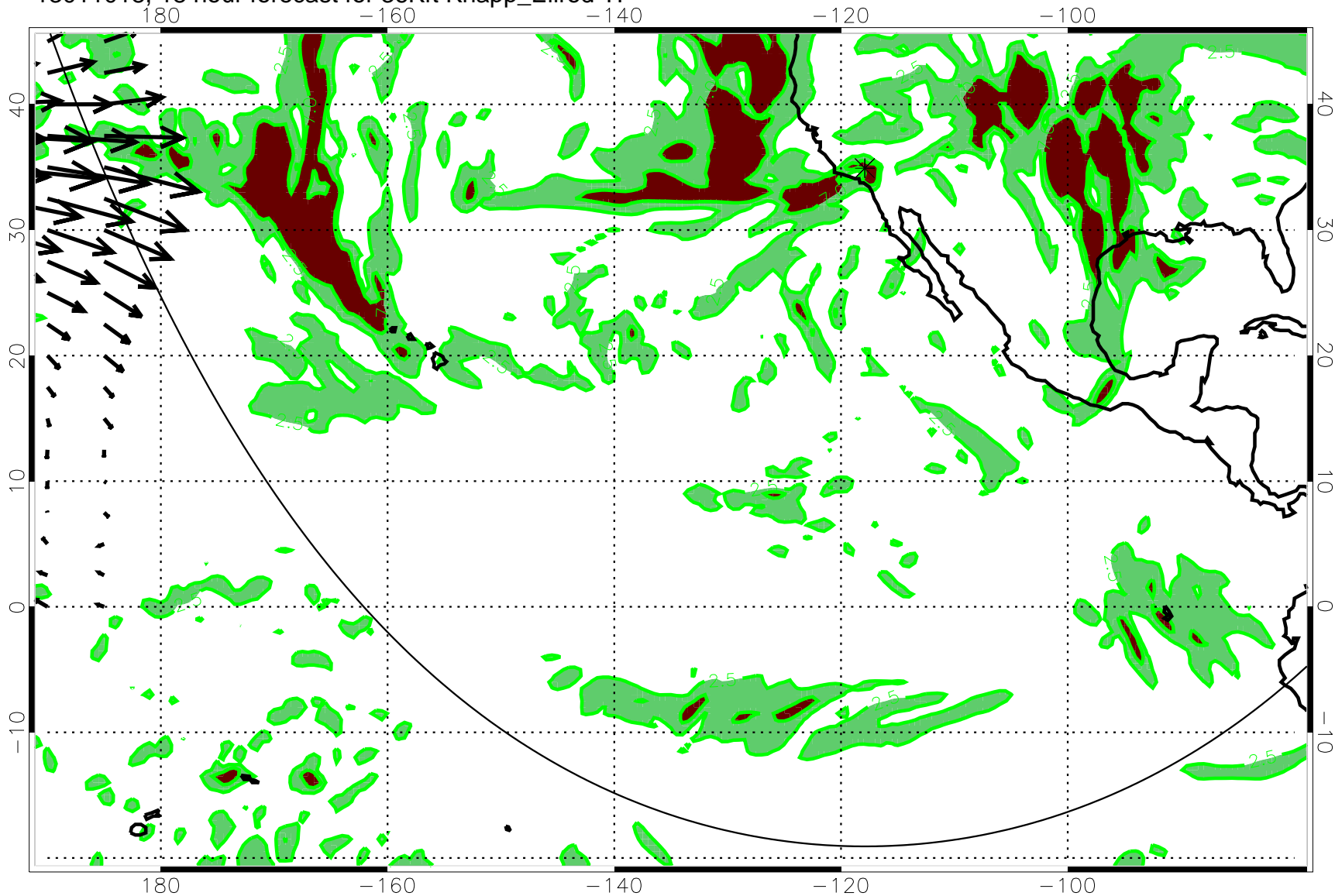
13011018, 18 hour forecast for 36Kft Knapp_Ellrod TI
