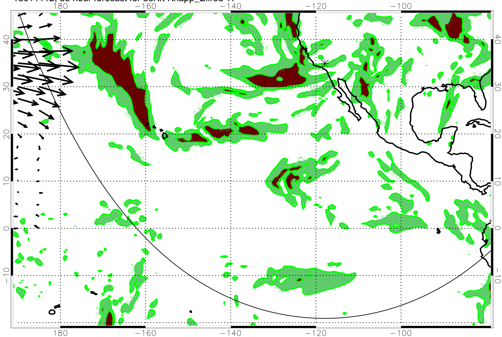
13011112, 36 hour forecast for 36Kft Knapp_Ellrod TI
