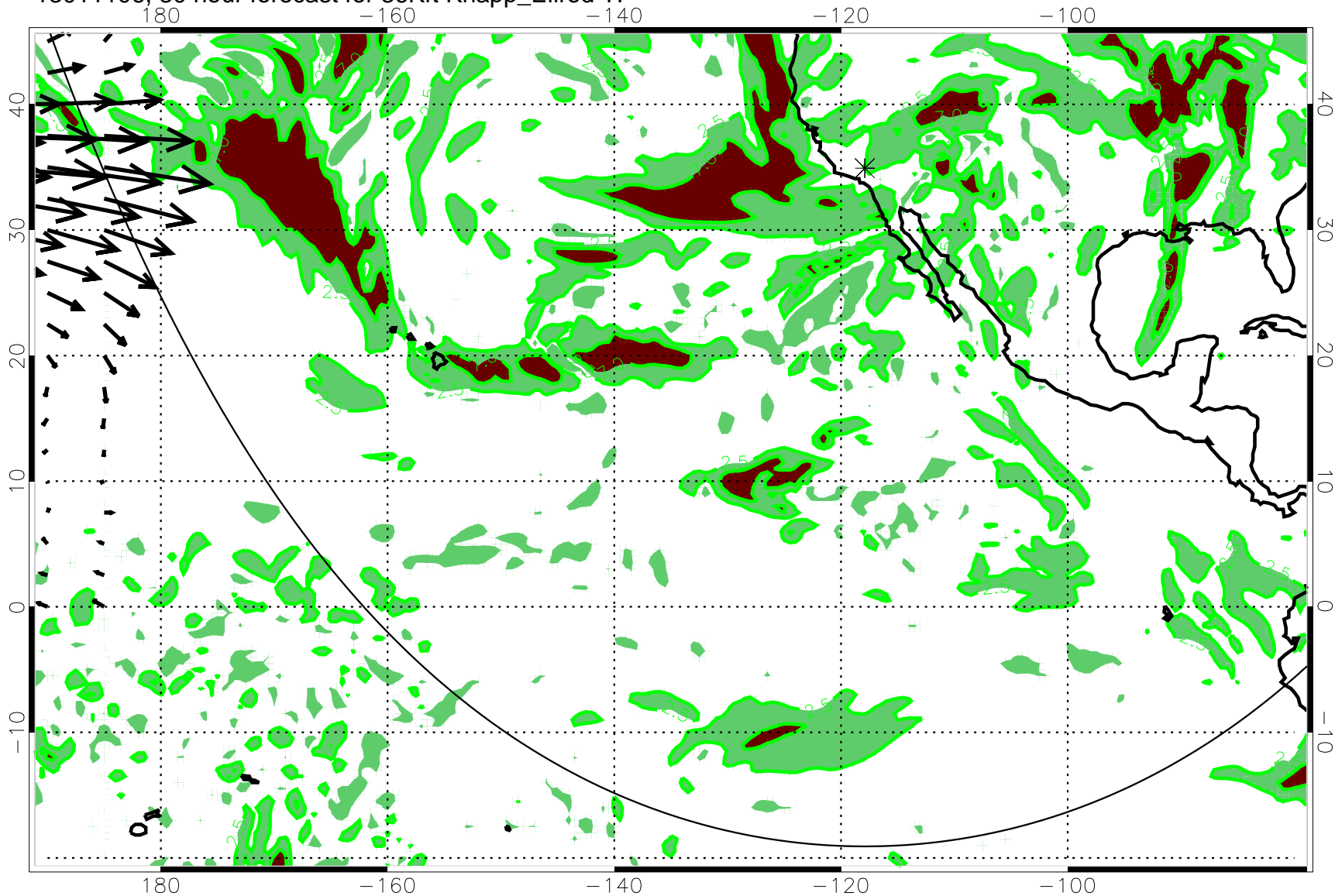
13011106, 30 hour forecast for 36Kft Knapp_Ellrod TI
