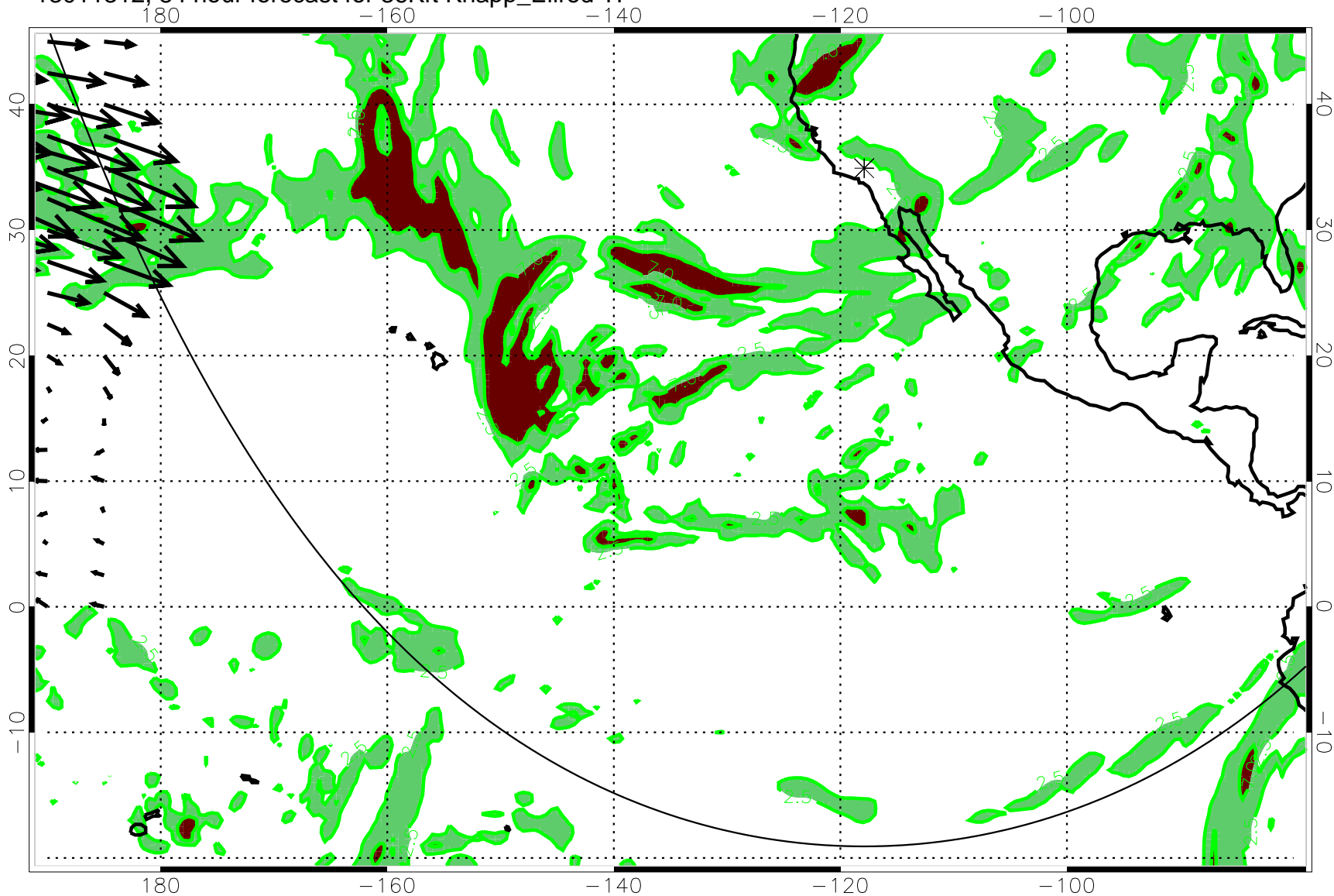
13011312, 84 hour forecast for 36Kft Knapp_Ellrod TI
