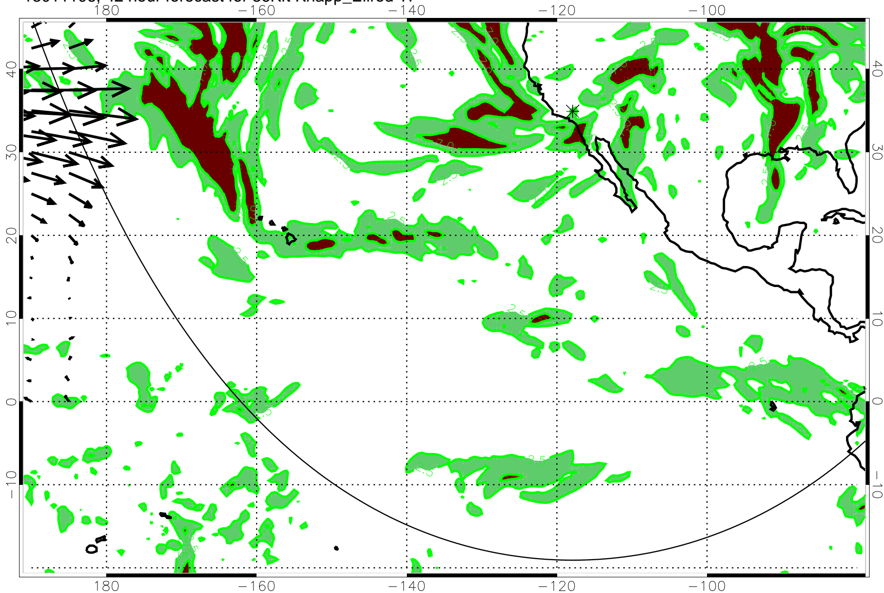
13011106, 42 hour forecast for 36Kft Knapp_Ellrod TI
