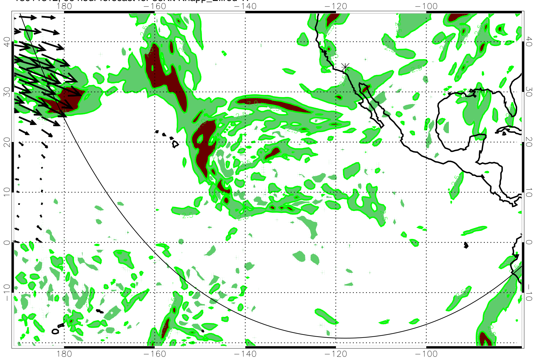
13011312, 96 hour forecast for 36Kft Knapp_Ellrod TI
