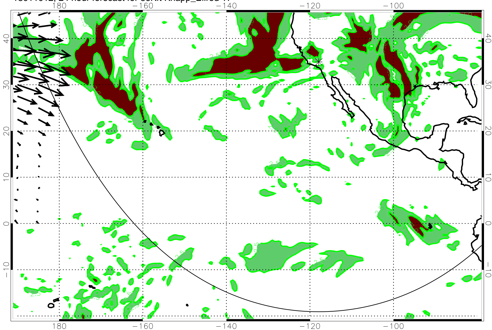
13011012, 24 hour forecast for 36Kft Knapp_Ellrod TI
