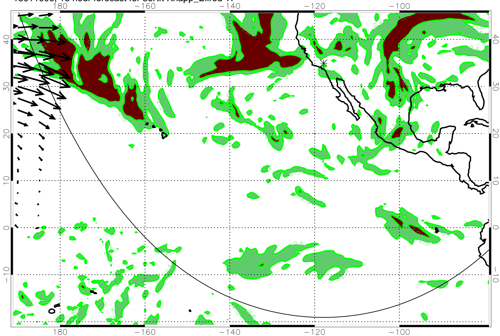
13011006, 18 hour forecast for 36Kft Knapp_Ellrod TI
