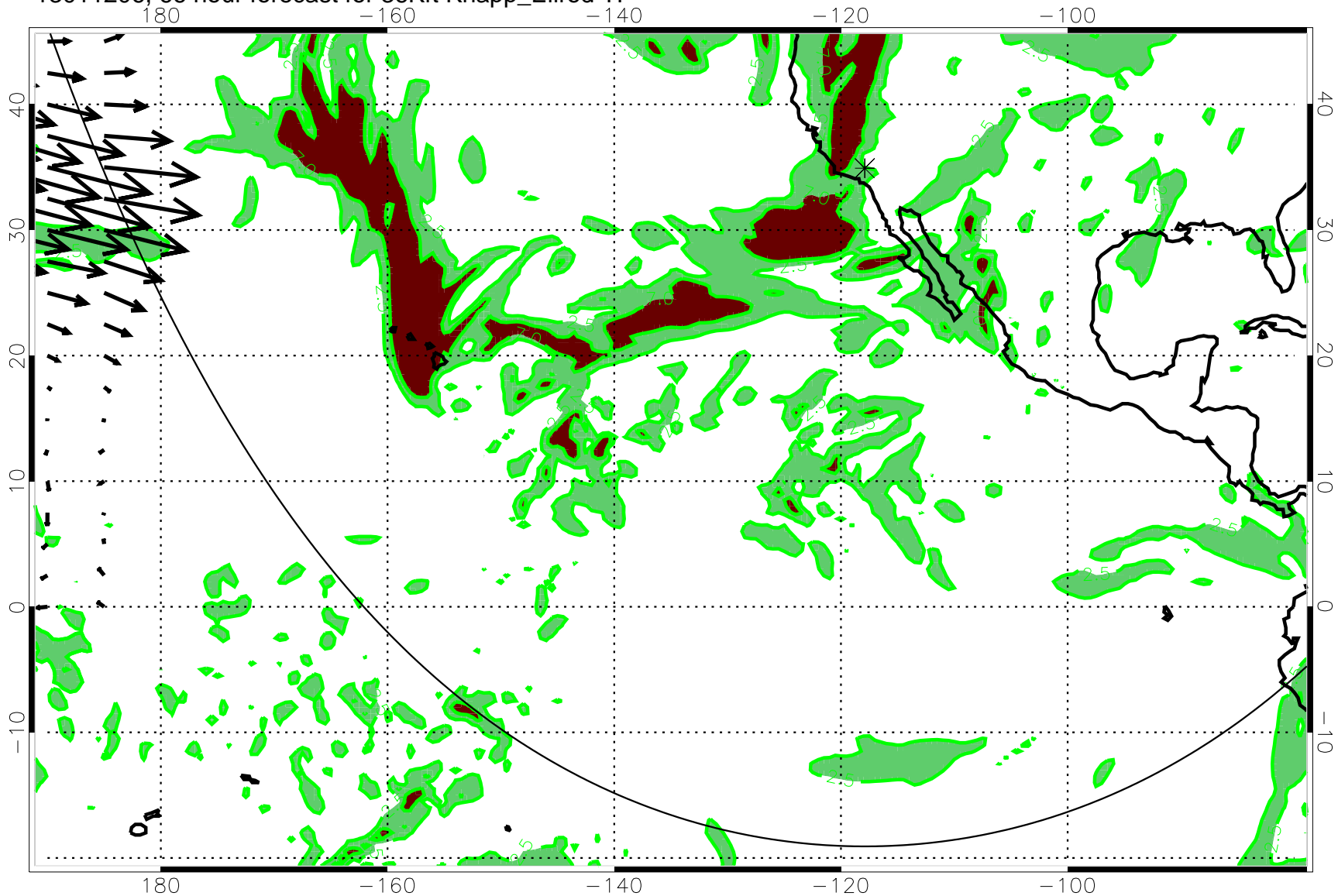
13011206, 66 hour forecast for 36Kft Knapp_Ellrod TI
