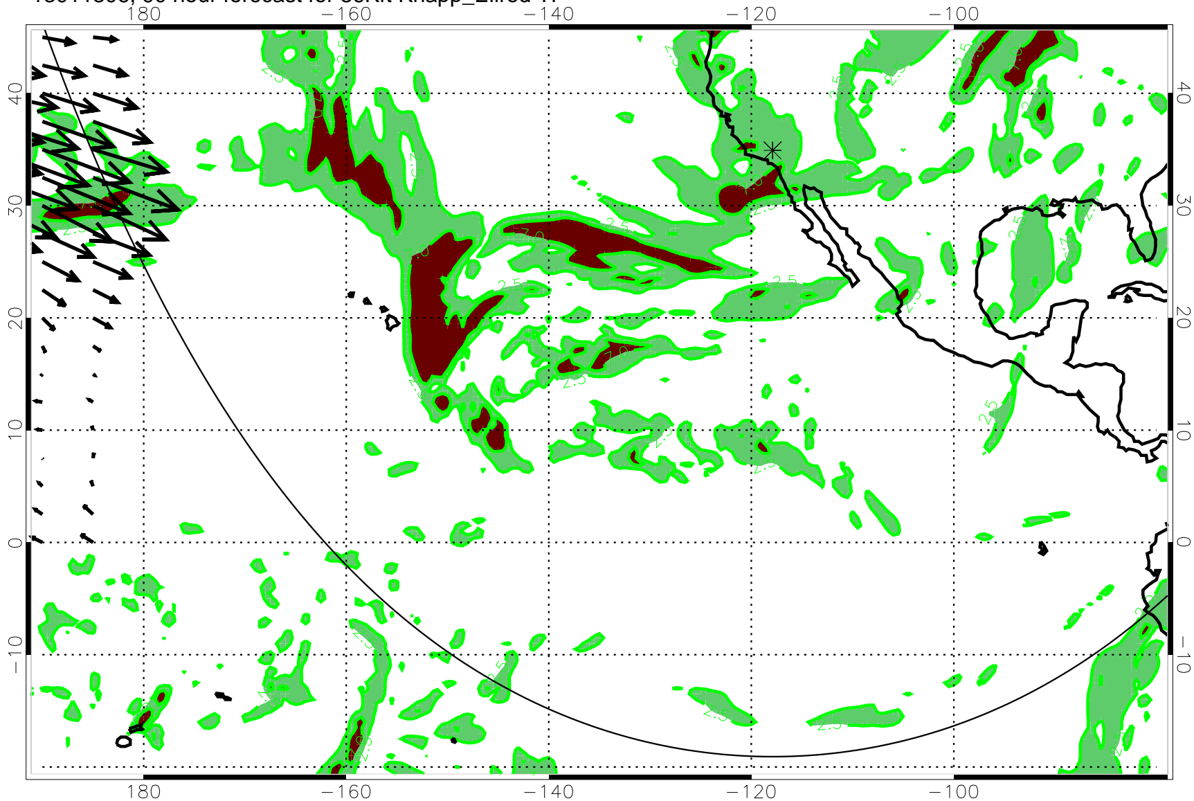
13011306, 90 hour forecast for 36Kft Knapp_Ellrod TI
