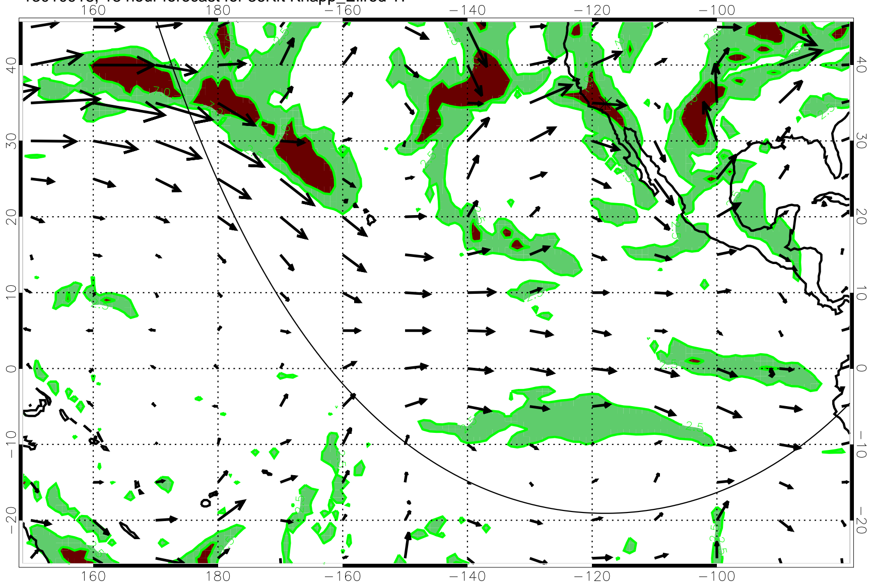
13010918, 18 hour forecast for 36Kft Knapp_Ellrod T1
