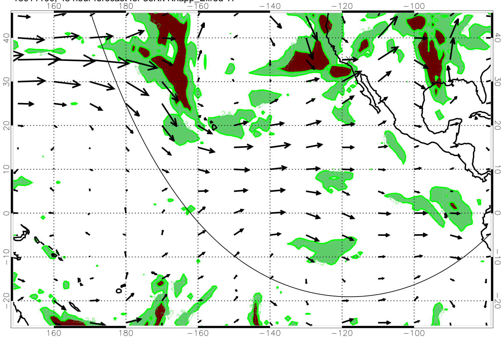
13011100, 48 hour forecast for 36Kft Knapp_Ellrod T1
