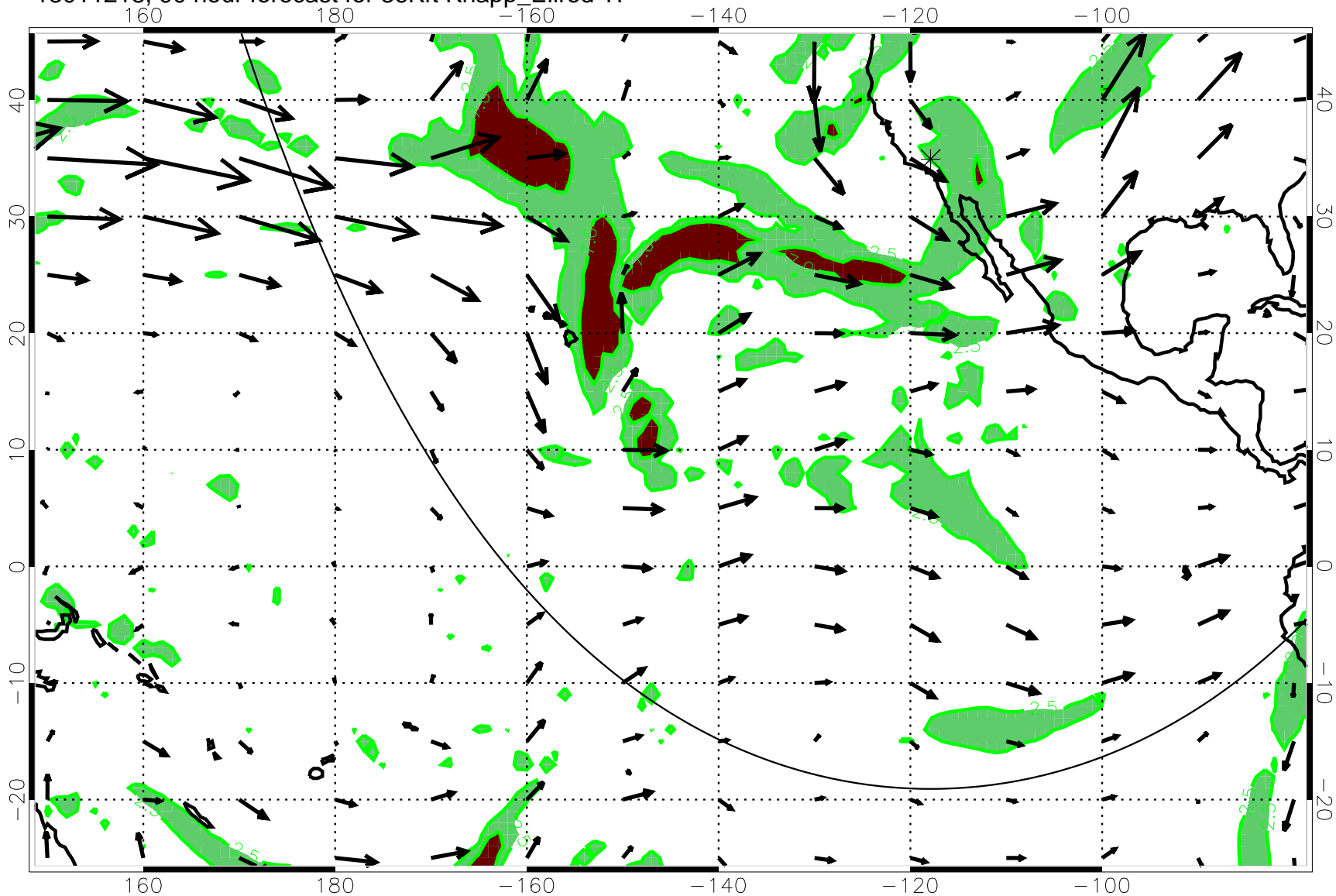
13011218, 90 hour forecast for 36Kft Knapp_Ellrod T1
