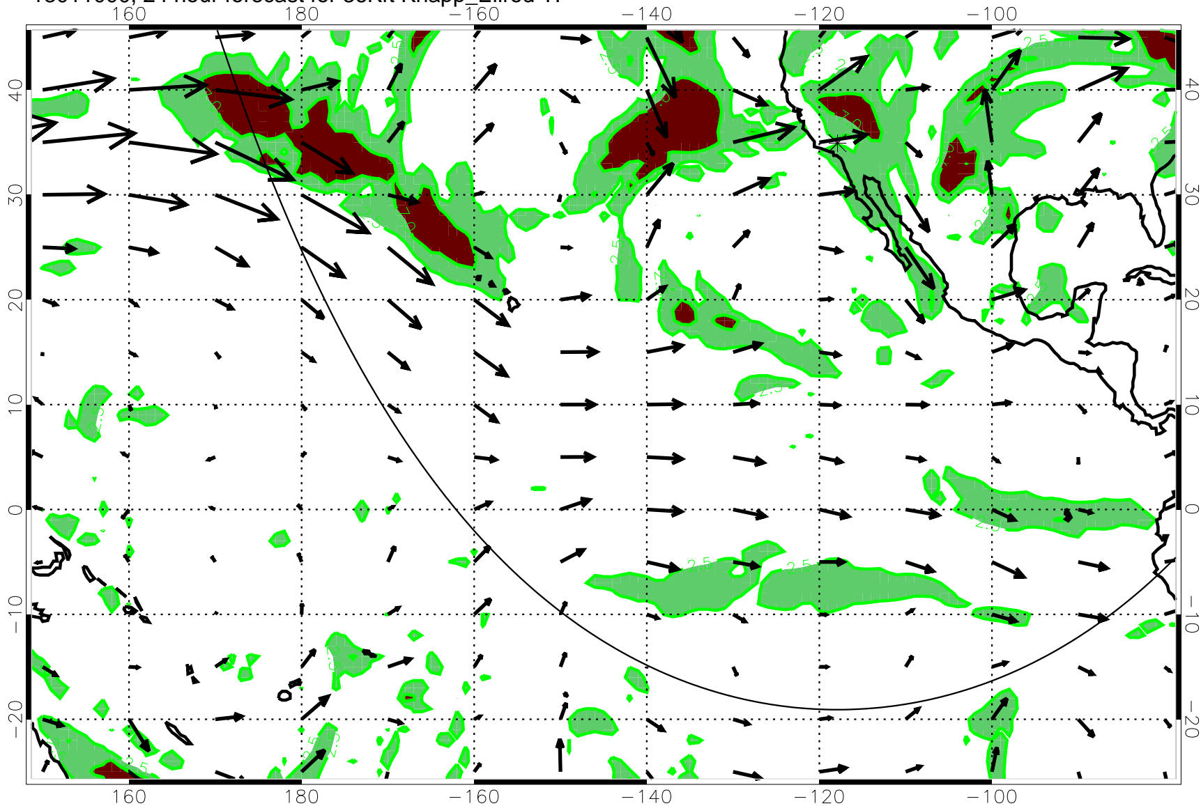
13011000, 24 hour forecast for 36Kft Knapp_Ellrod T1
