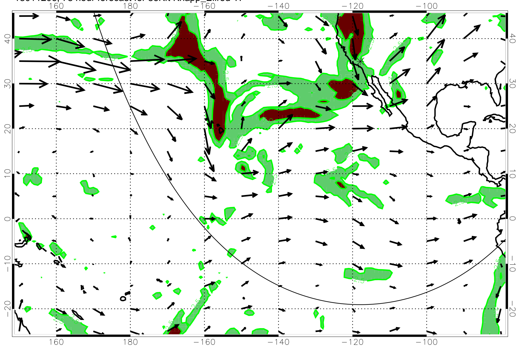
13011206, 78 hour forecast for 36Kft Knapp_Ellrod T1
