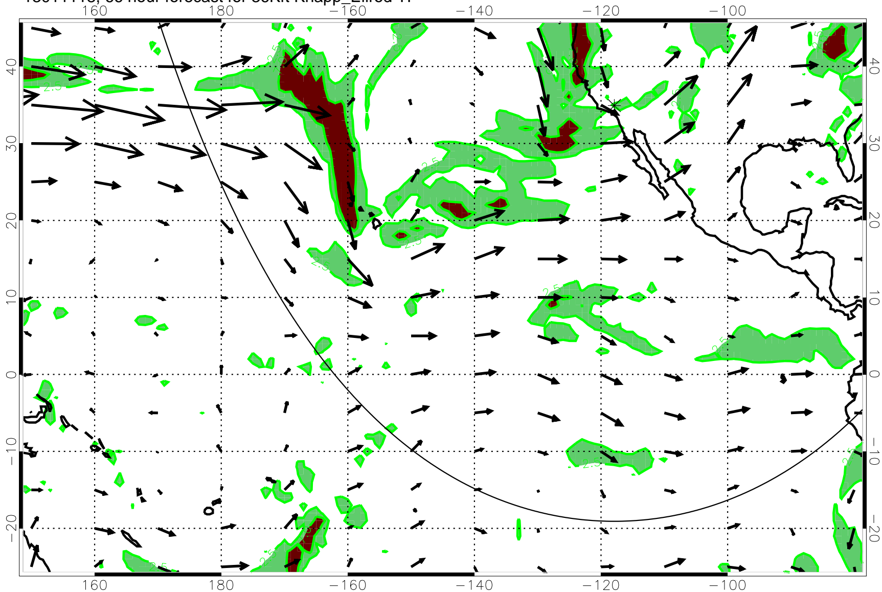
13011118, 66 hour forecast for 36Kft Knapp_Ellrod TI
