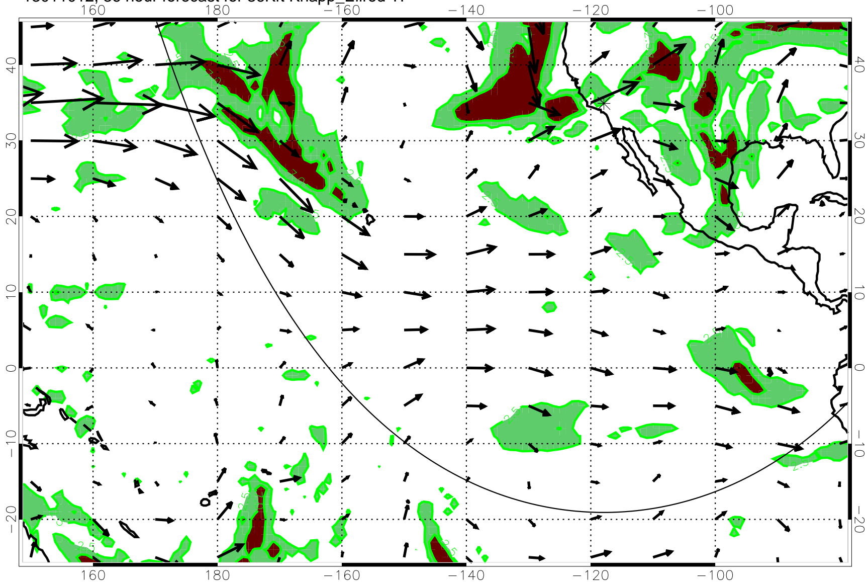
13011012, 36 hour forecast for 36Kft Knapp_Ellrod T1
