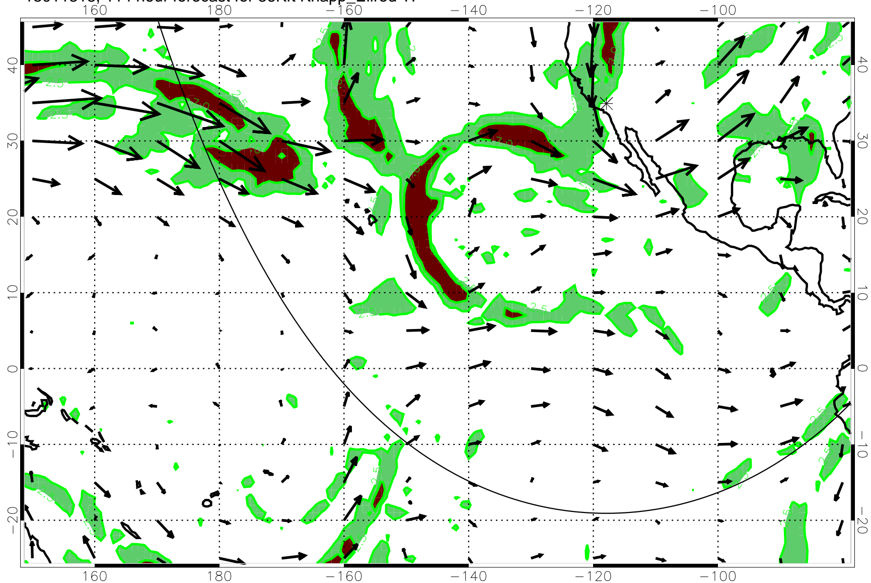
13011318, 114 hour forecast for 36Kft Knapp_Ellrod T1
