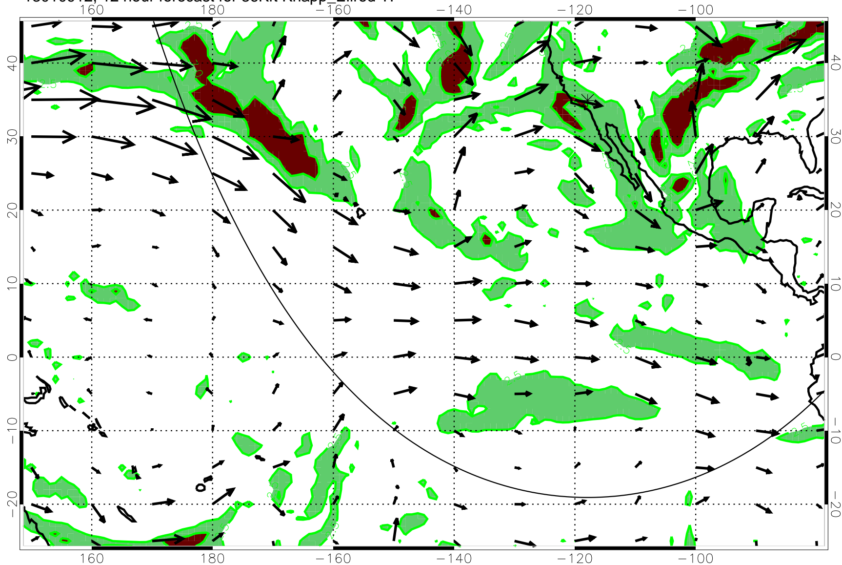
13010912, 12 hour forecast for 36Kft Knapp_Ellrod T1
