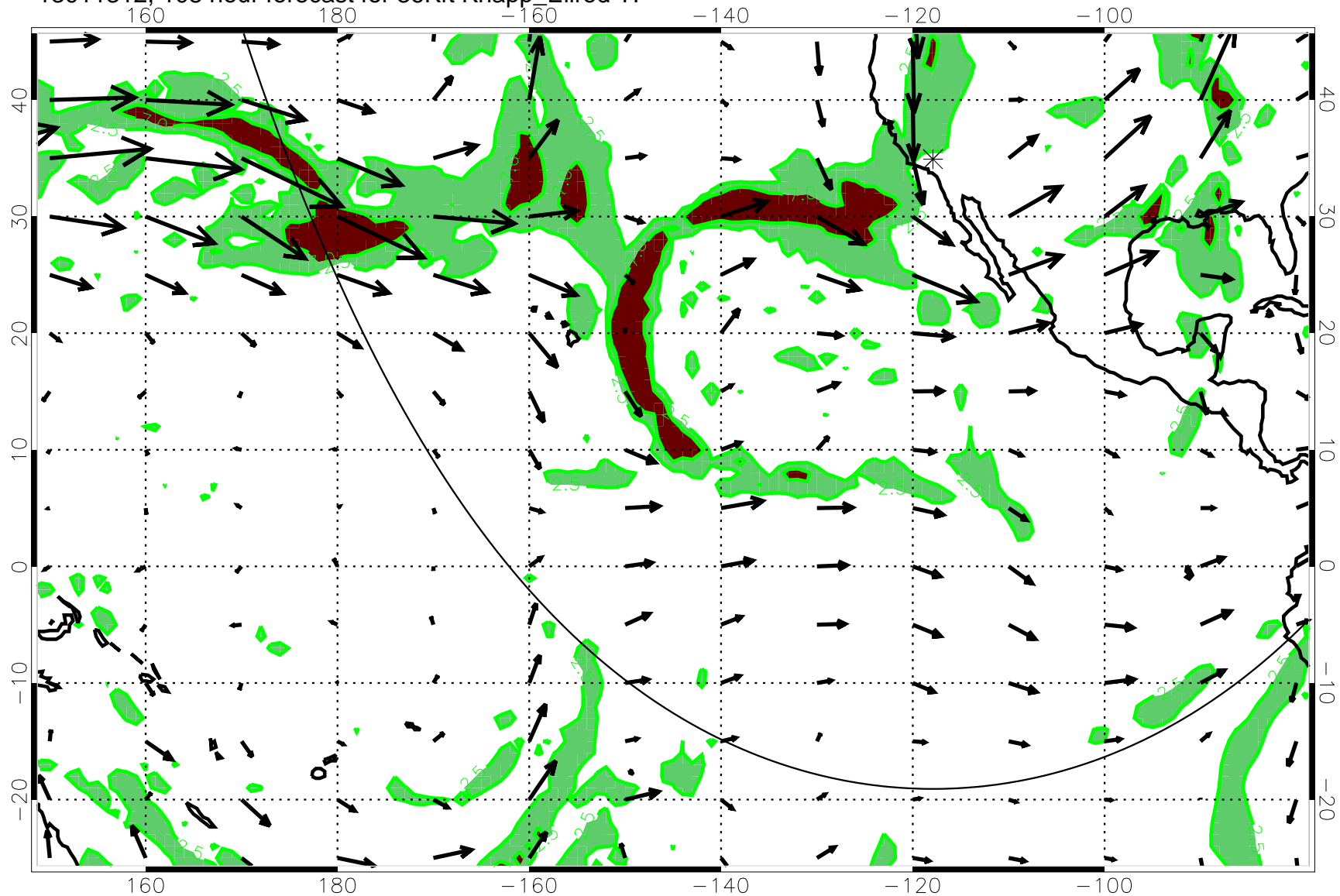
13011312, 108 hour forecast for 36Kft Knapp_Ellrod T1
