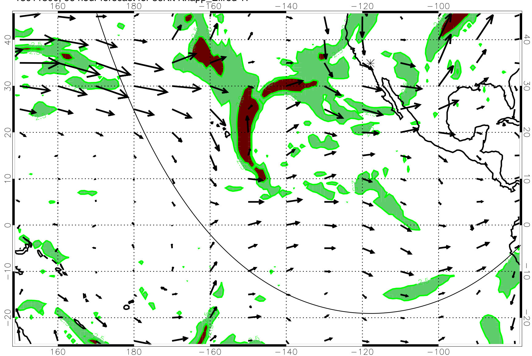
13011300, 96 hour forecast for 36Kft Knapp_Ellrod T1
