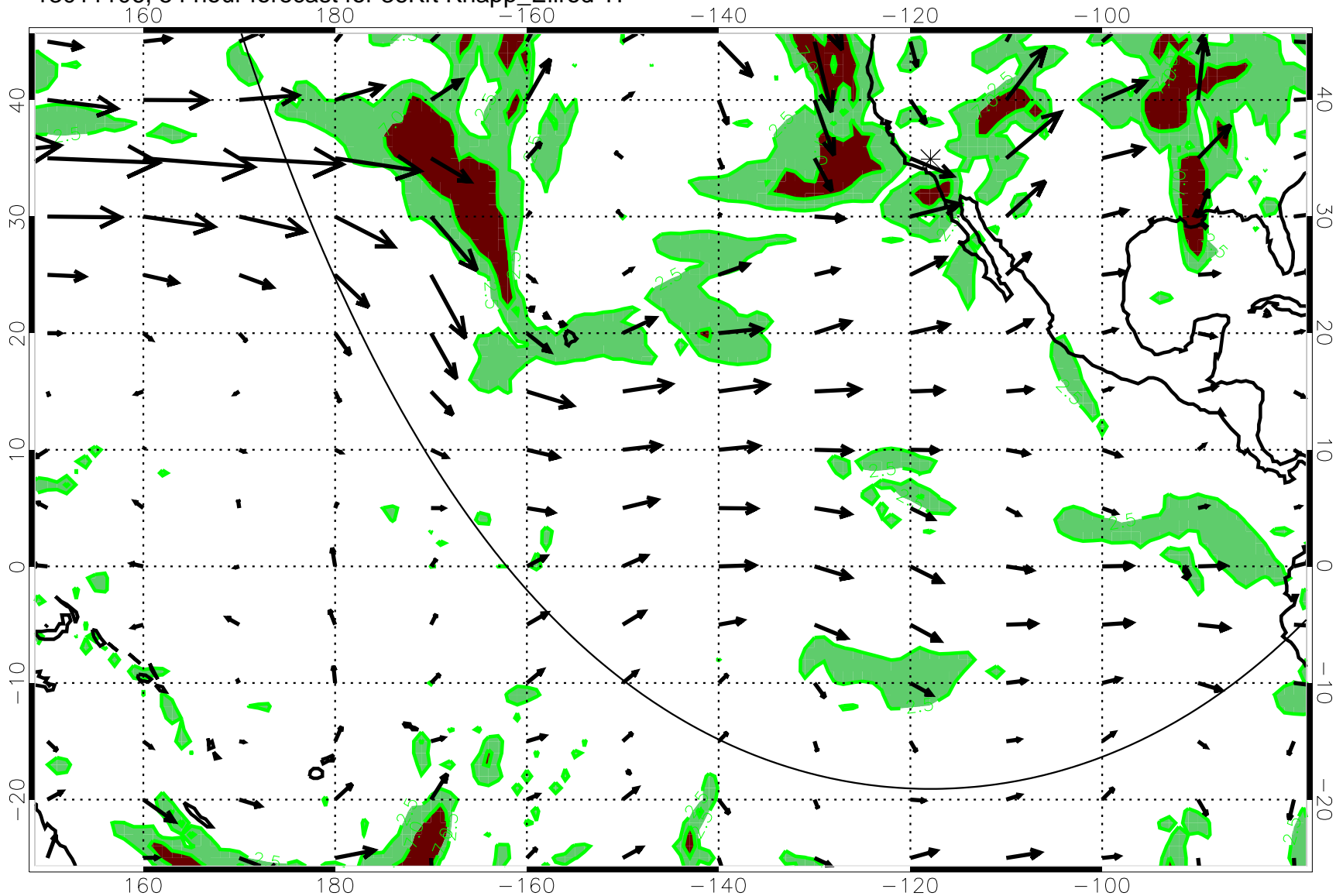
13011106, 54 hour forecast for 36Kft Knapp_Ellrod T1
