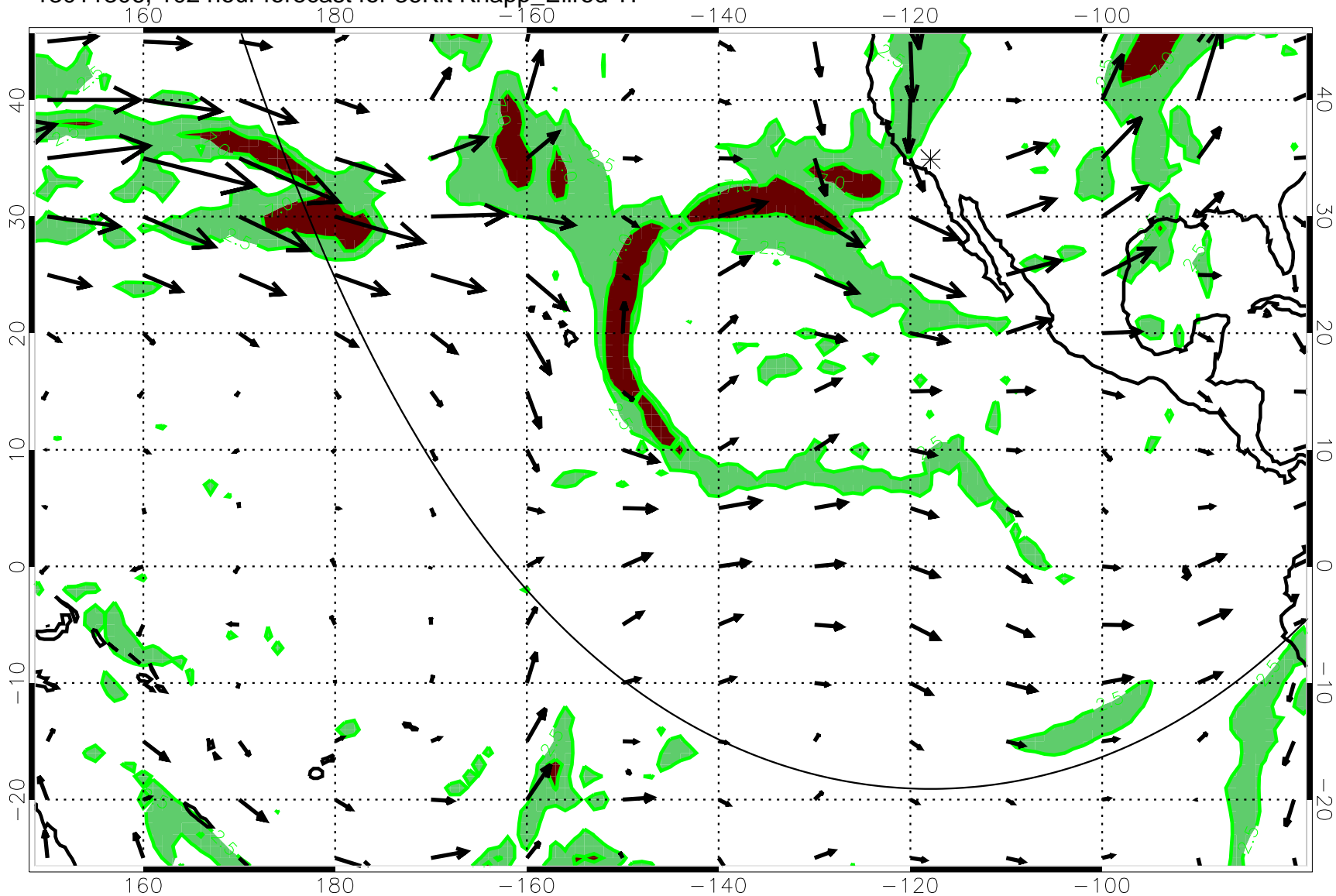
13011306, 102 hour forecast for 36Kft Knapp_Ellrod T1
