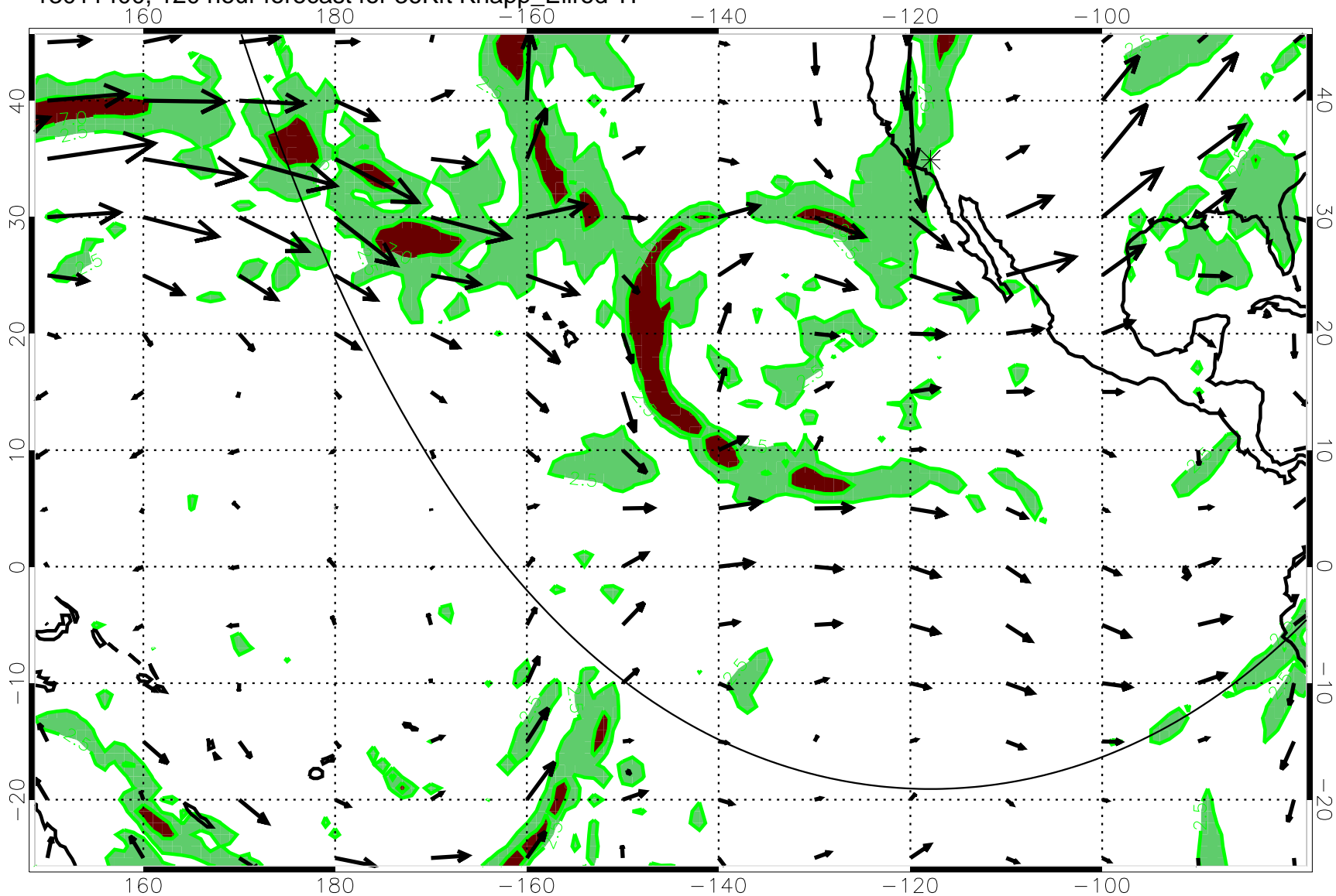
13011400, 120 hour forecast for 36Kft Knapp_Ellrod T1
