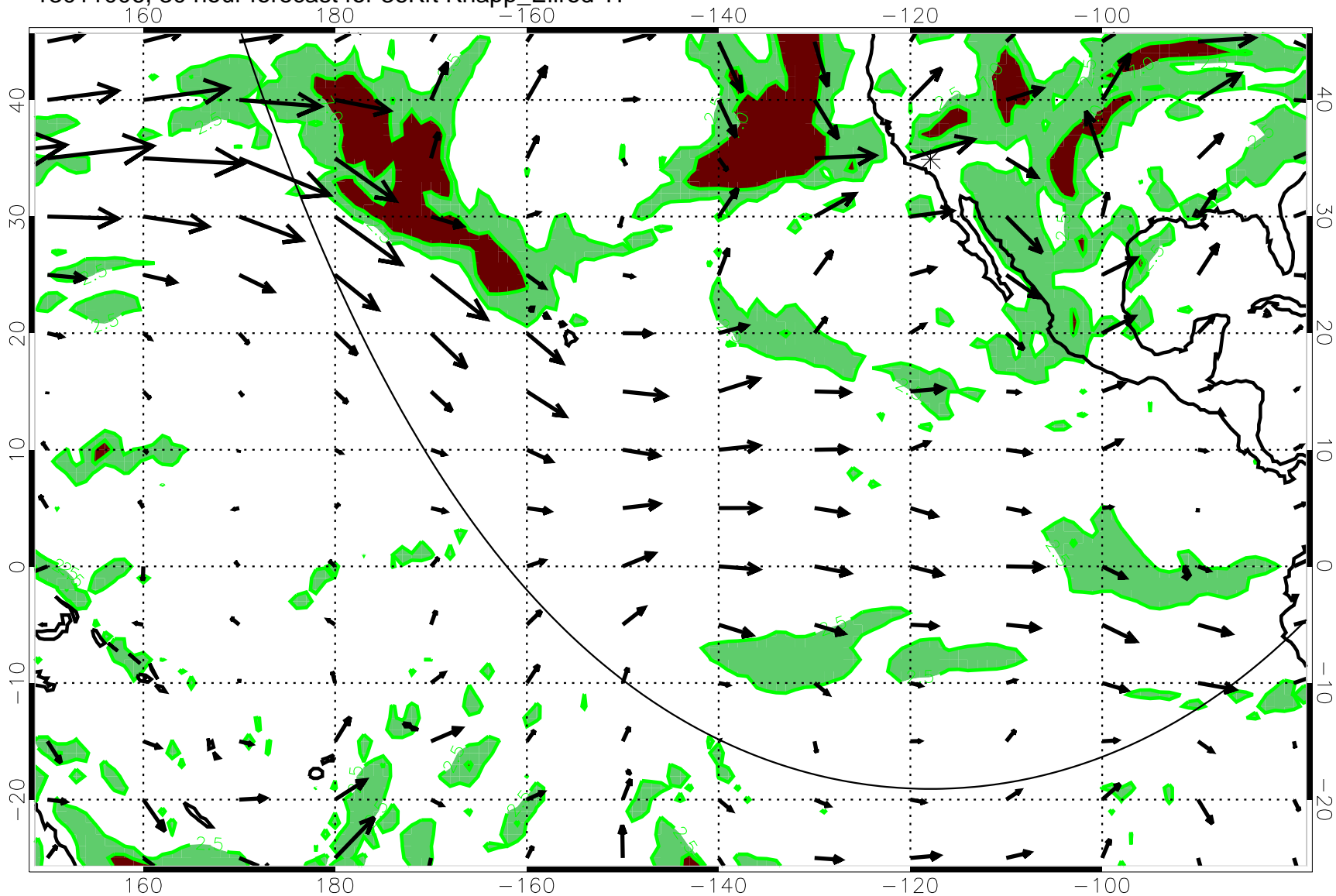
13011006, 30 hour forecast for 36Kft Knapp_Ellrod T1
