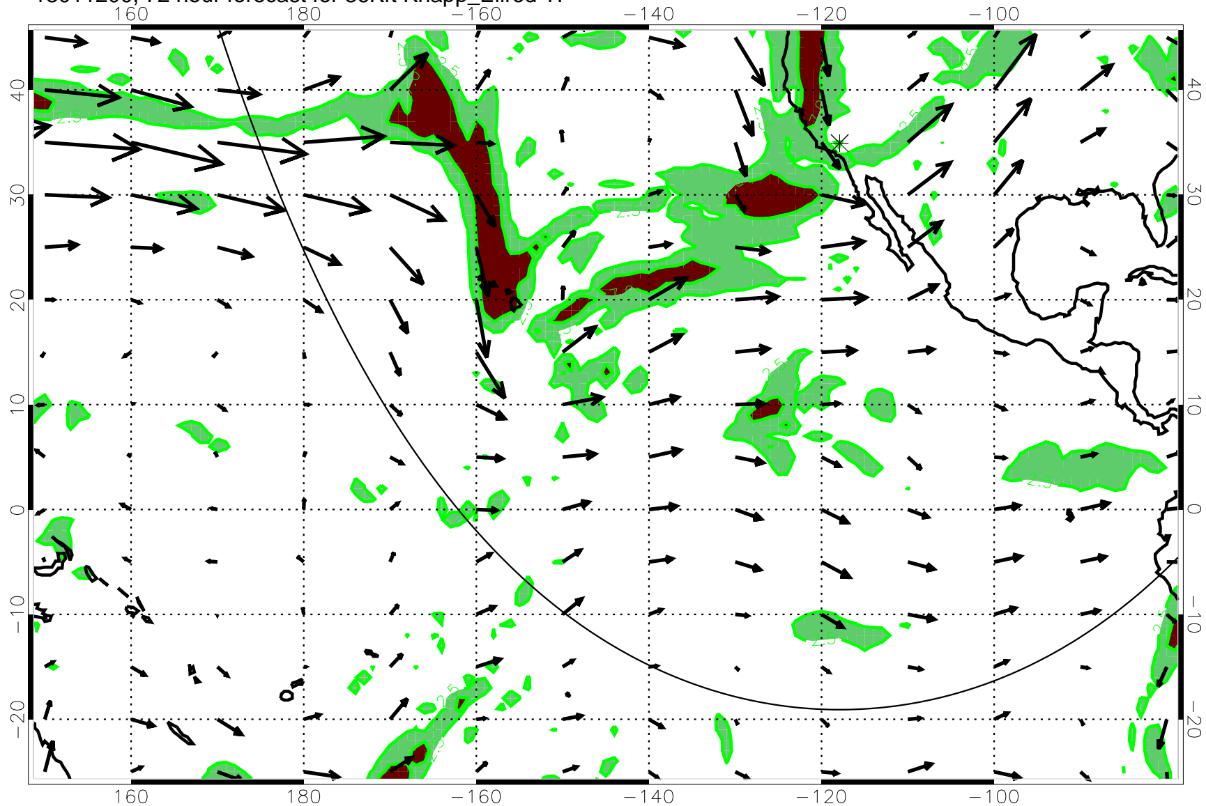
13011200, 72 hour forecast for 36Kft Knapp_Ellrod T1
