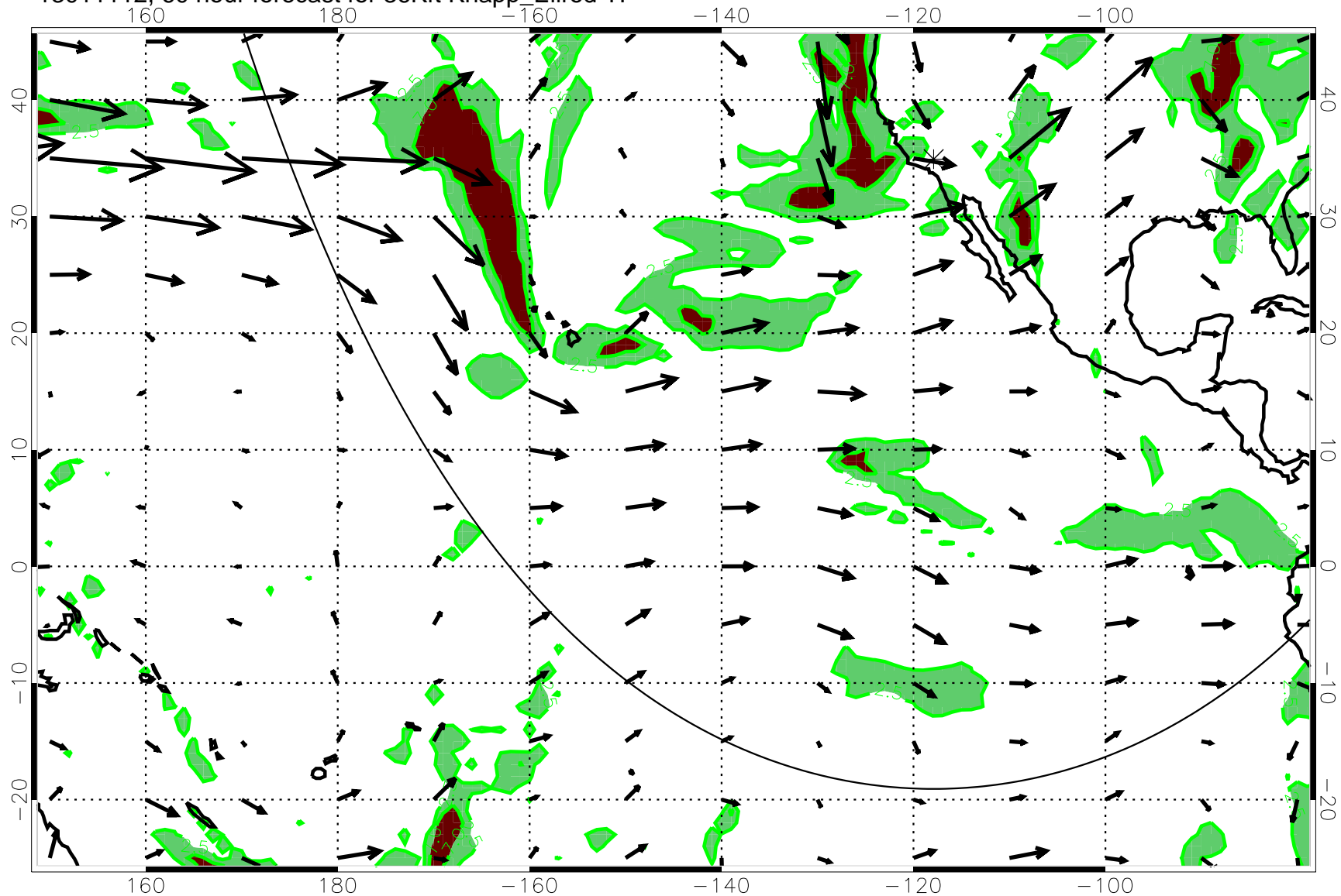
13011112, 60 hour forecast for 36Kft Knapp_Ellrod TI
