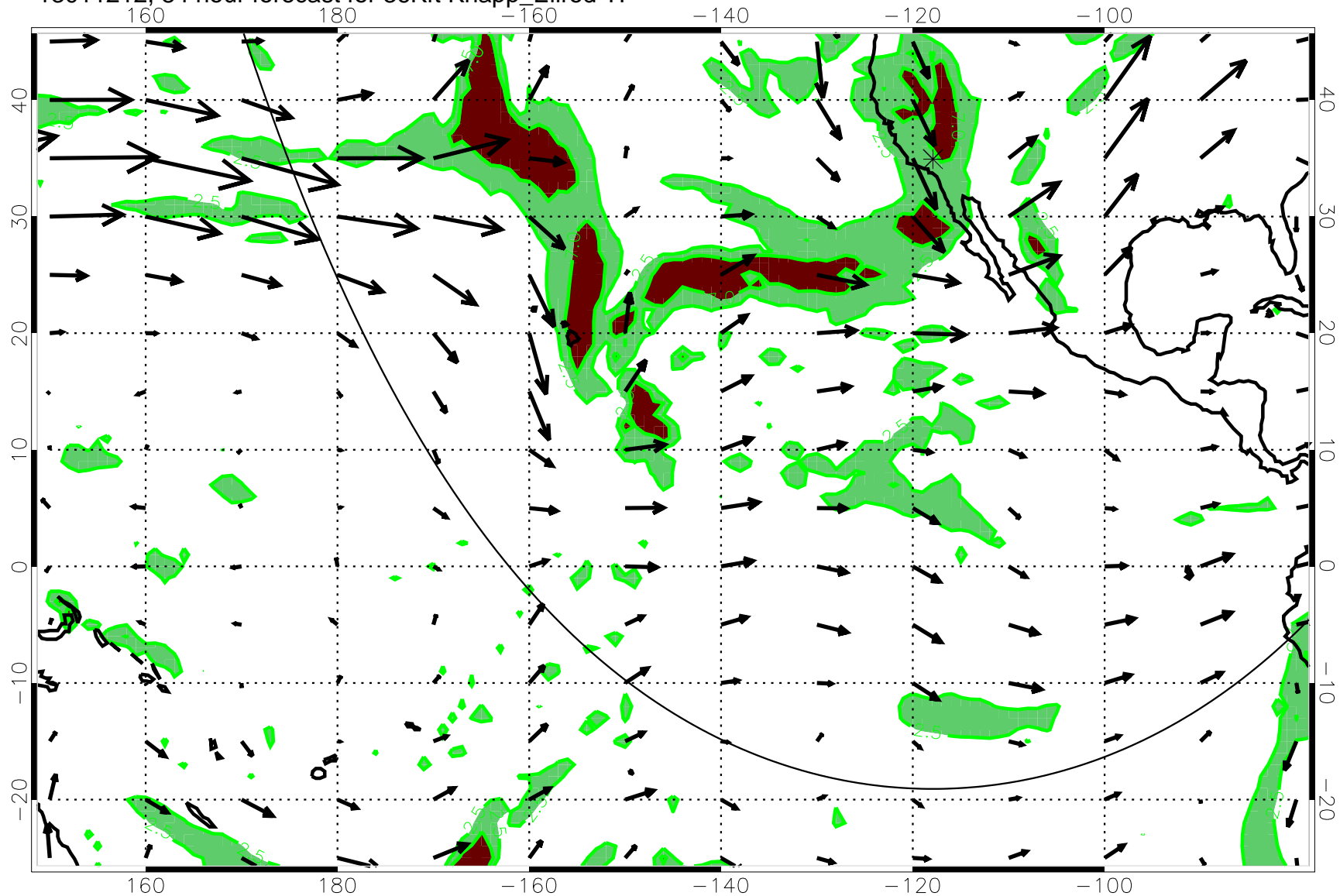
13011212, 84 hour forecast for 36Kft Knapp_Ellrod T1
