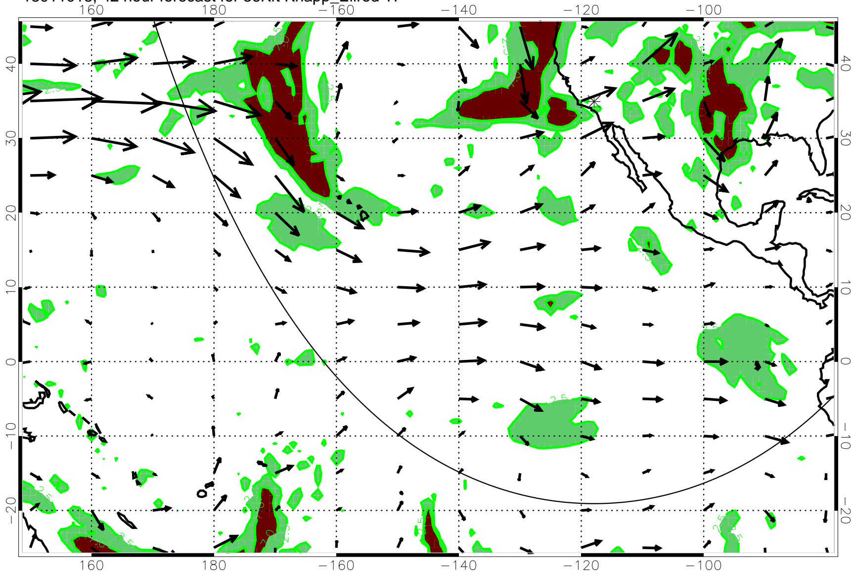
13011018, 42 hour forecast for 36Kft Knapp_Ellrod T1
