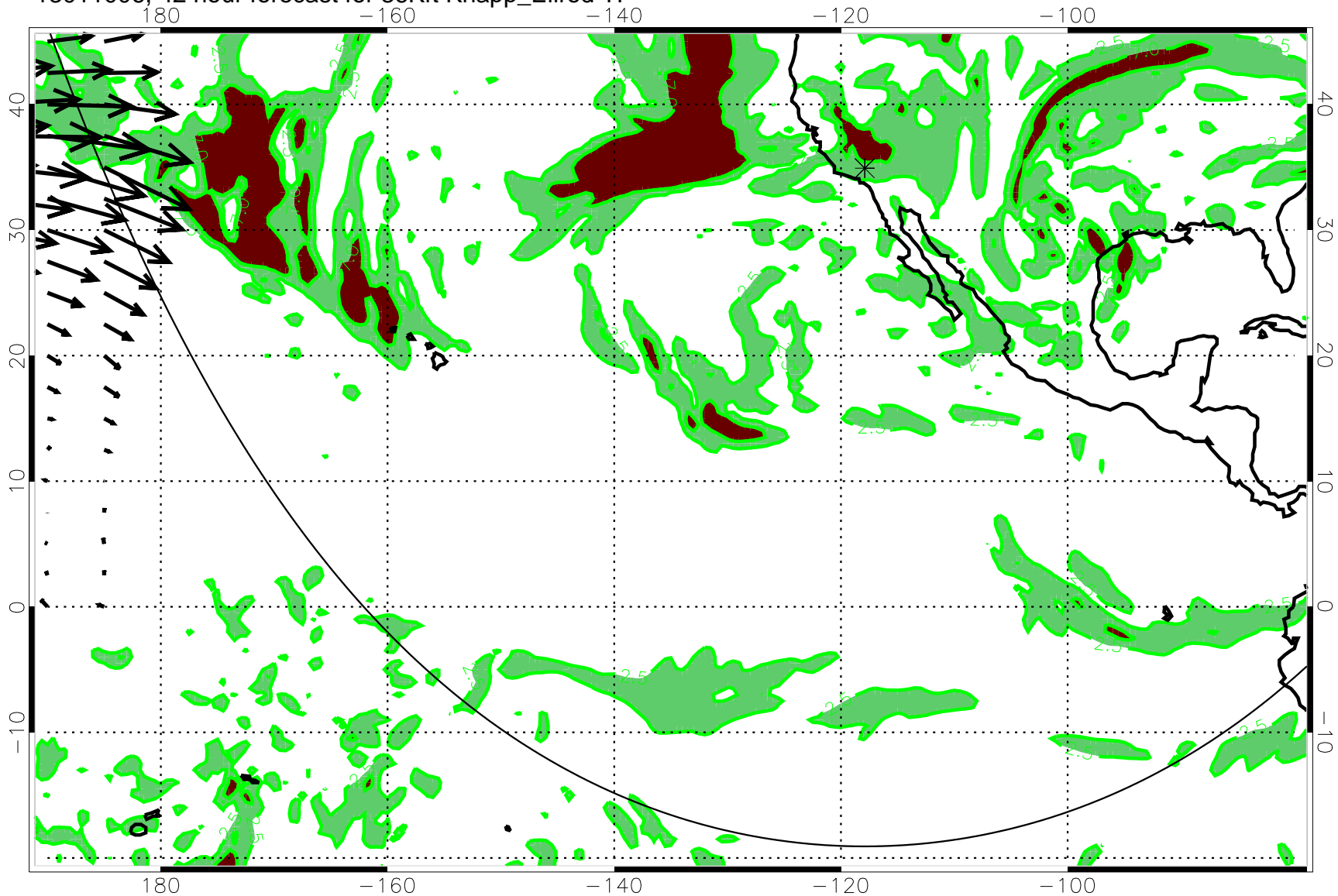
13011006, 42 hour forecast for 36Kft Knapp_Ellrod TI
