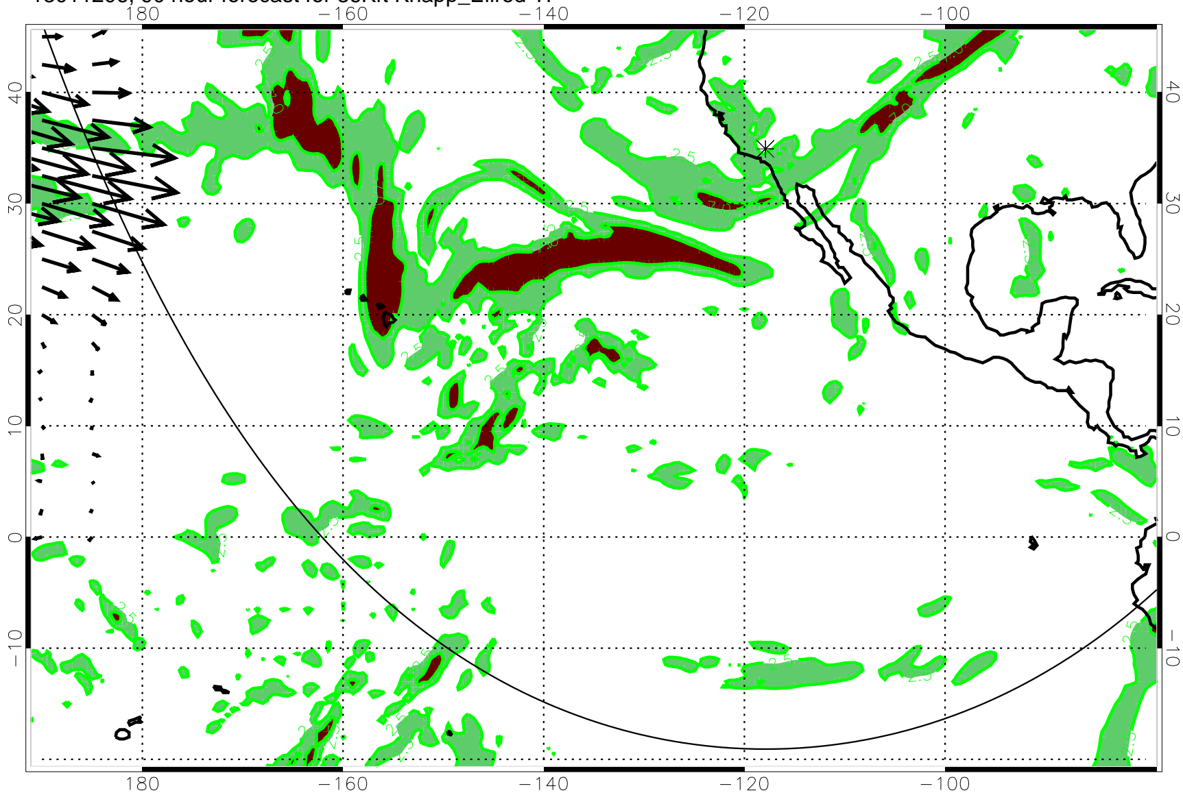
13011206, 90 hour forecast for 36Kft Knapp_Ellrod TI
