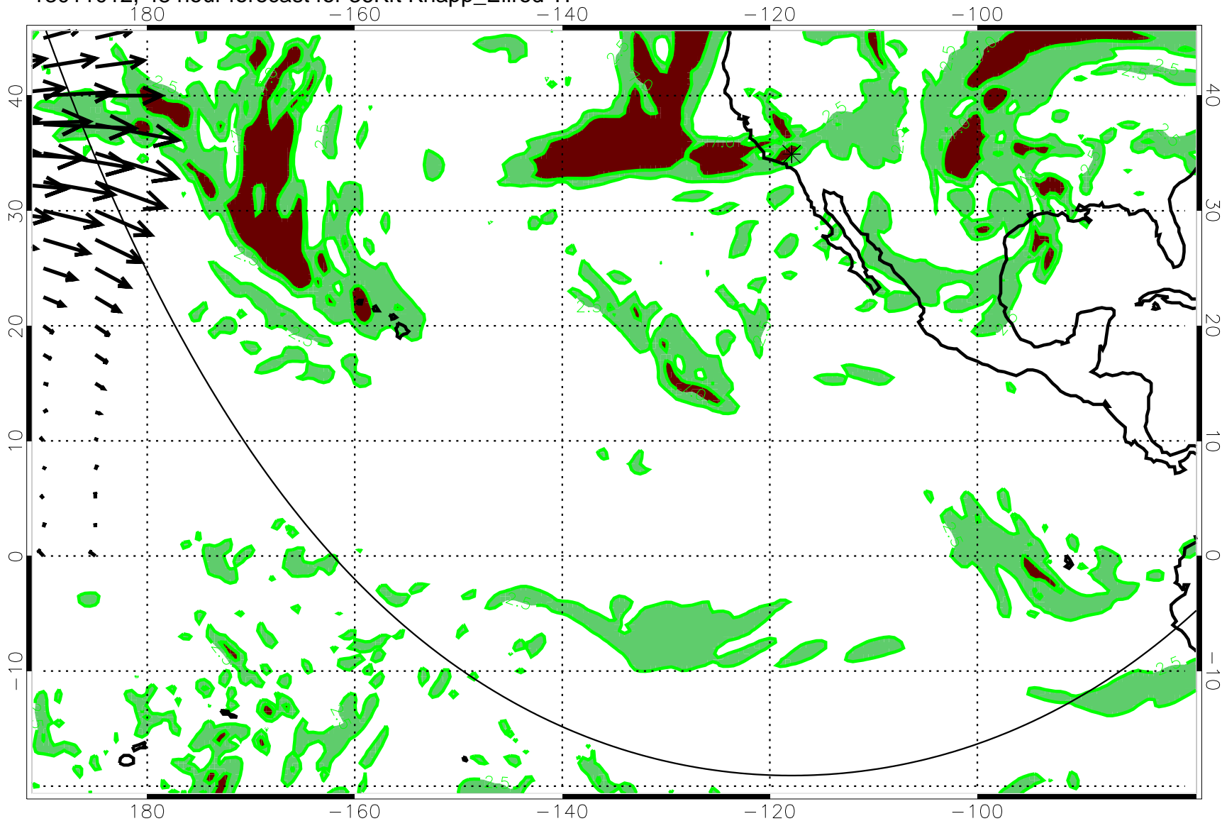
13011012, 48 hour forecast for 36Kft Knapp_Ellrod TI
