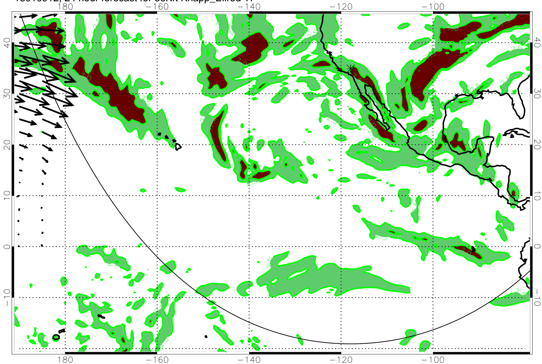
13010912, 24 hour forecast for 36Kft Knapp_Ellrod TI
