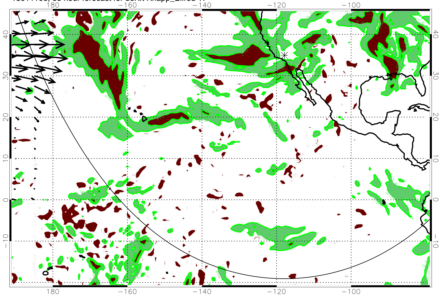
13011106, 66 hour forecast for 36Kft Knapp_Ellrod TI
