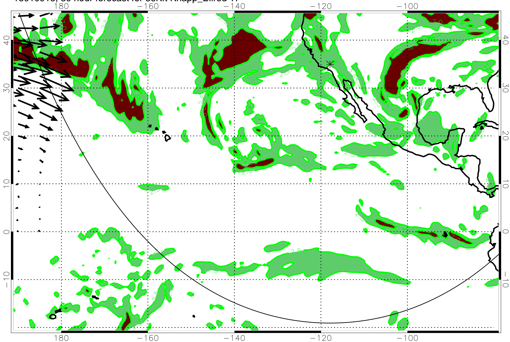
13010918, 30 hour forecast for 36Kft Knapp_Ellrod TI
