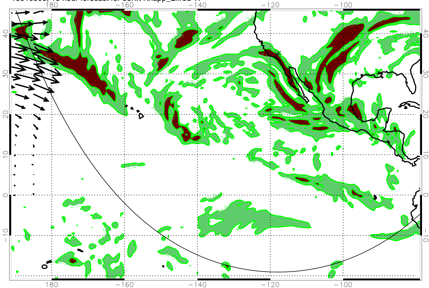
13010906, 18 hour forecast for 36Kft Knapp_Ellrod TI
