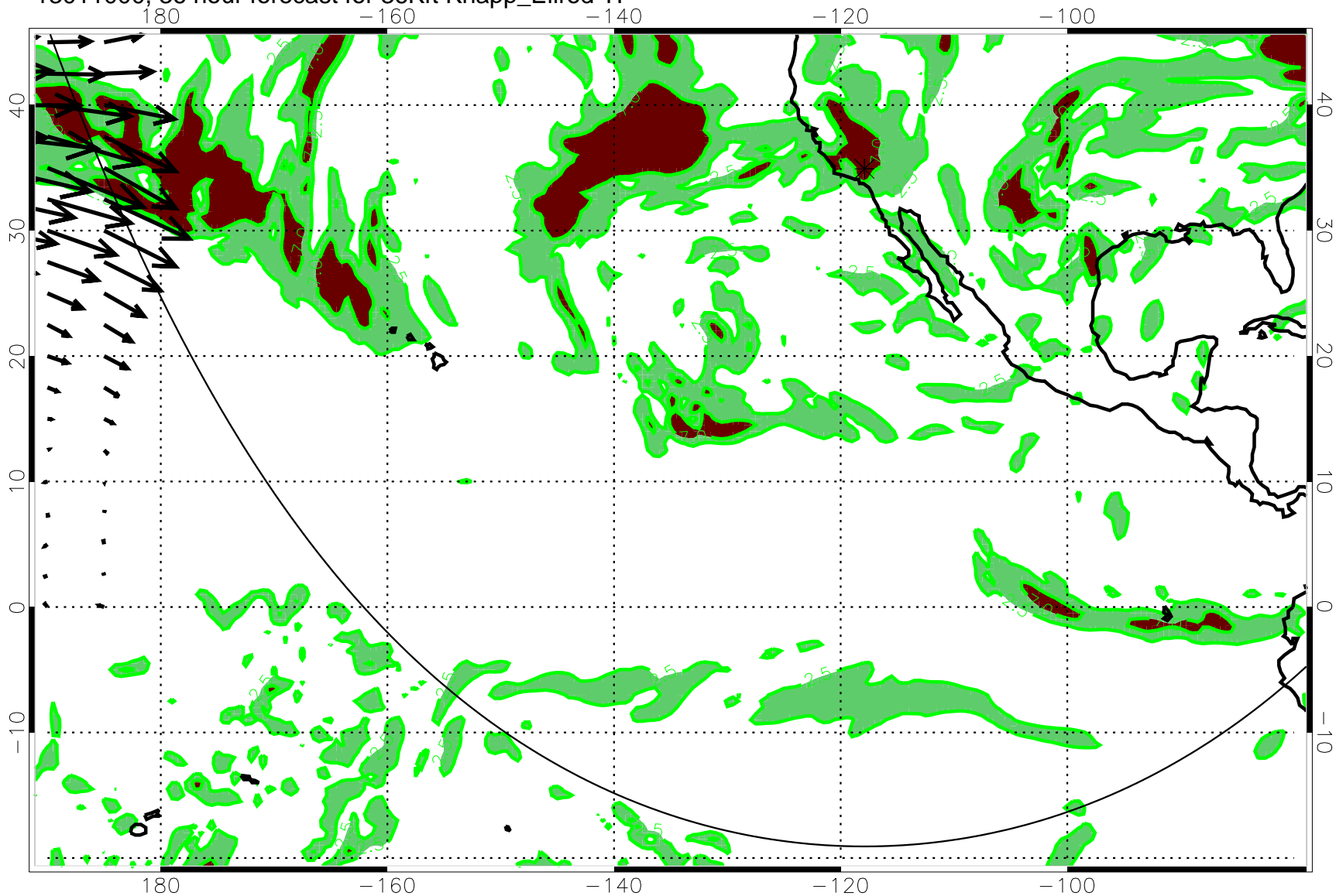
13011000, 36 hour forecast for 36Kft Knapp_Ellrod TI
