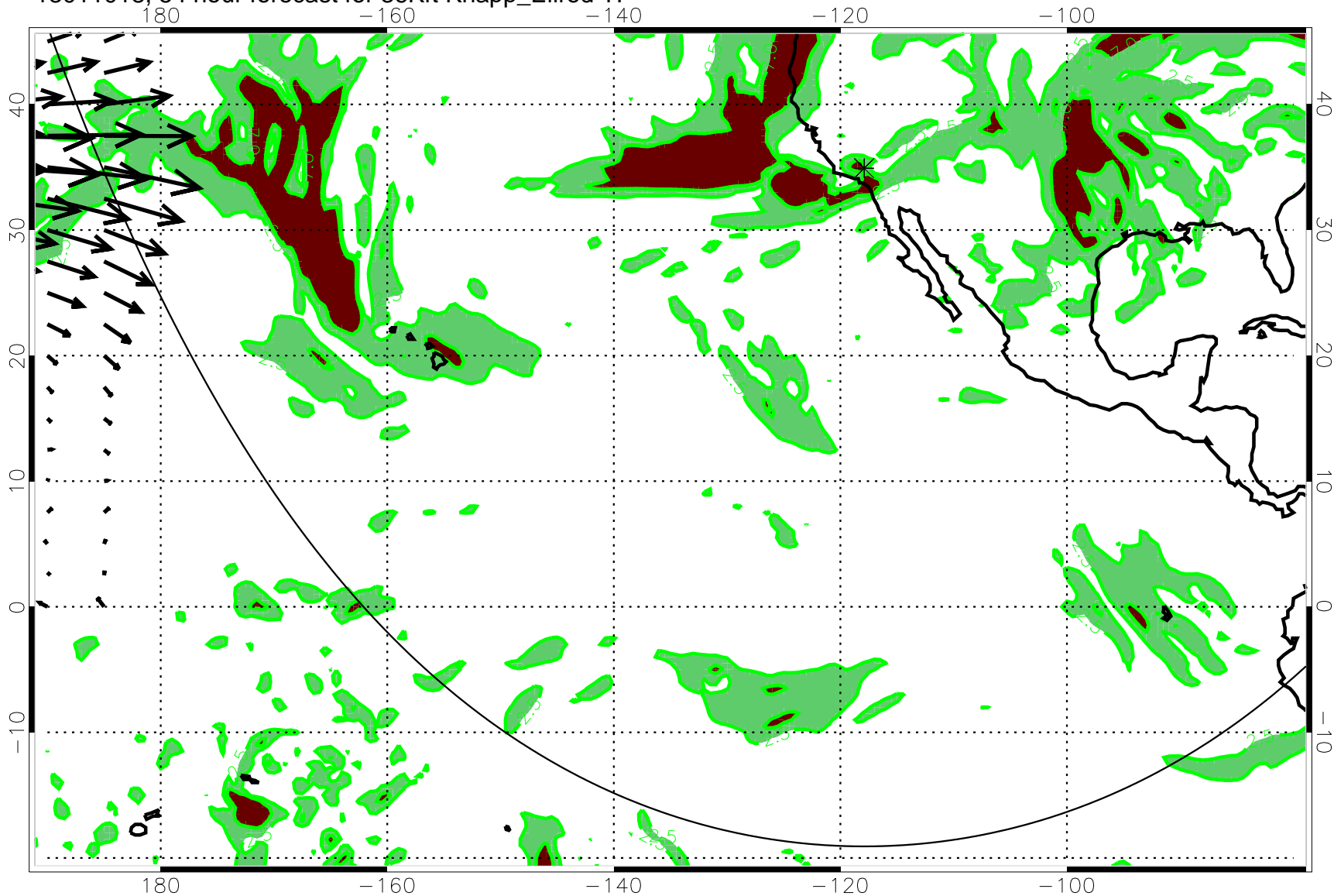
13011018, 54 hour forecast for 36Kft Knapp_Ellrod TI
