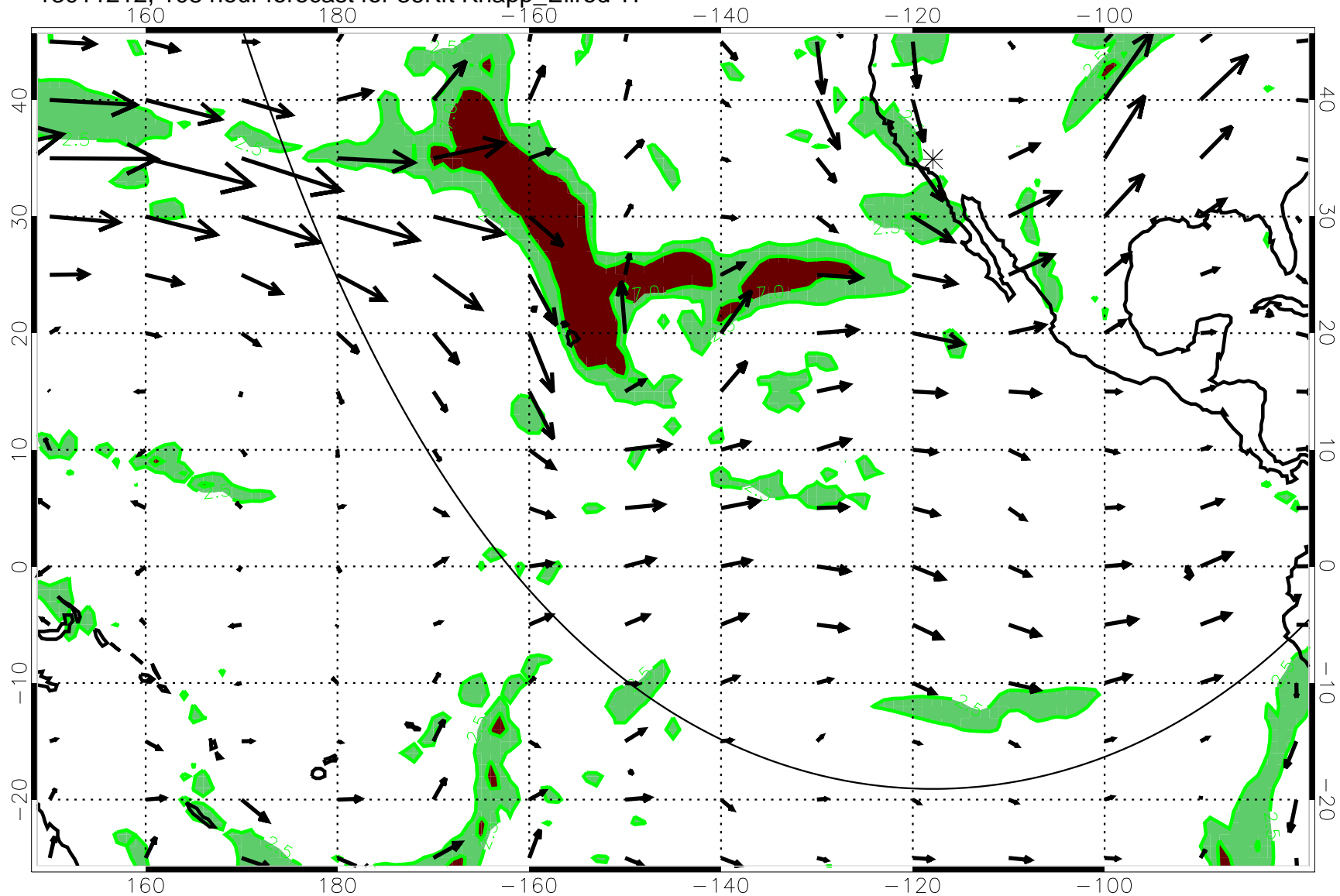
13011212, 108 hour forecast for 36Kft Knapp_Ellrod T1
