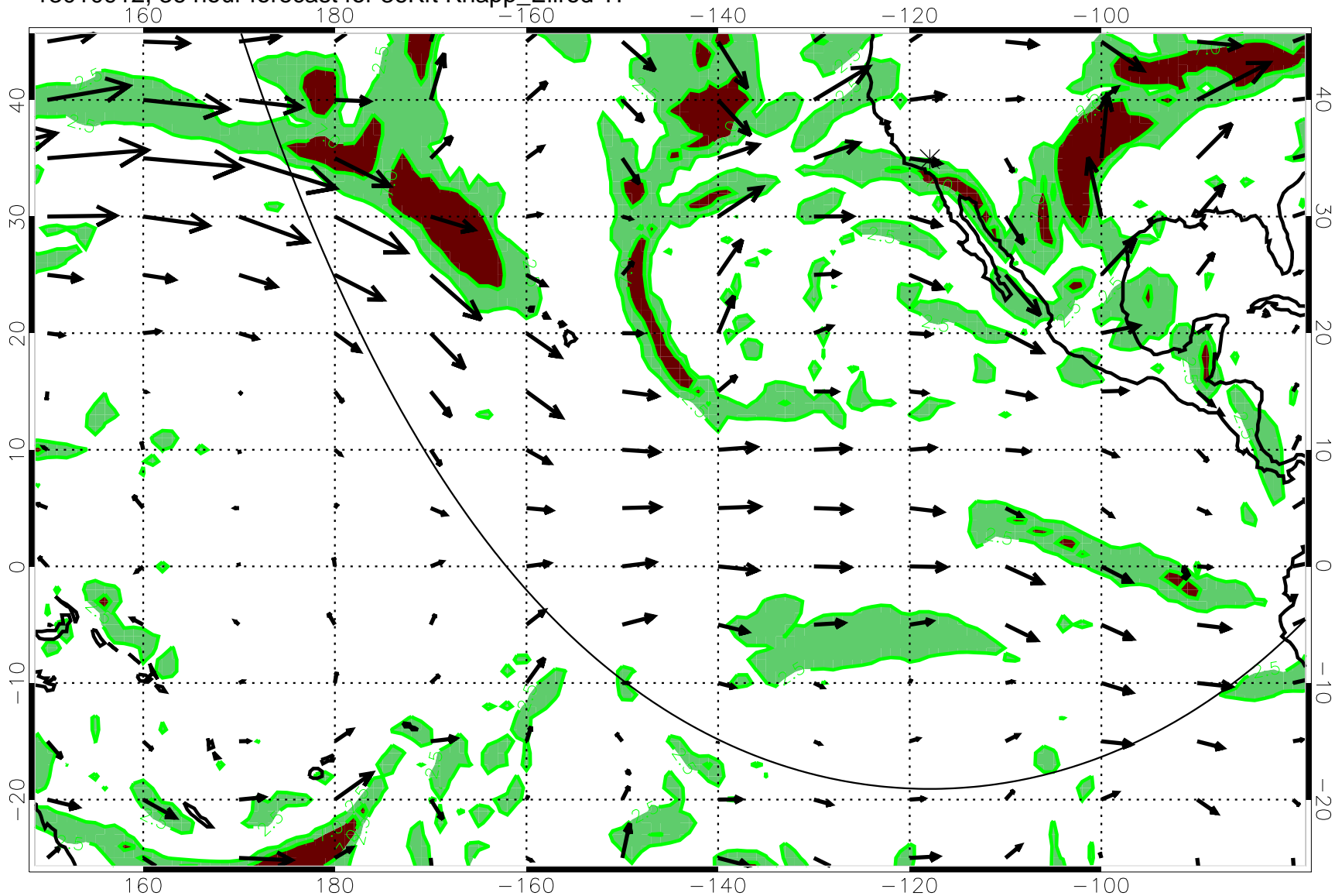
13010912, 36 hour forecast for 36Kft Knapp_Ellrod T1
