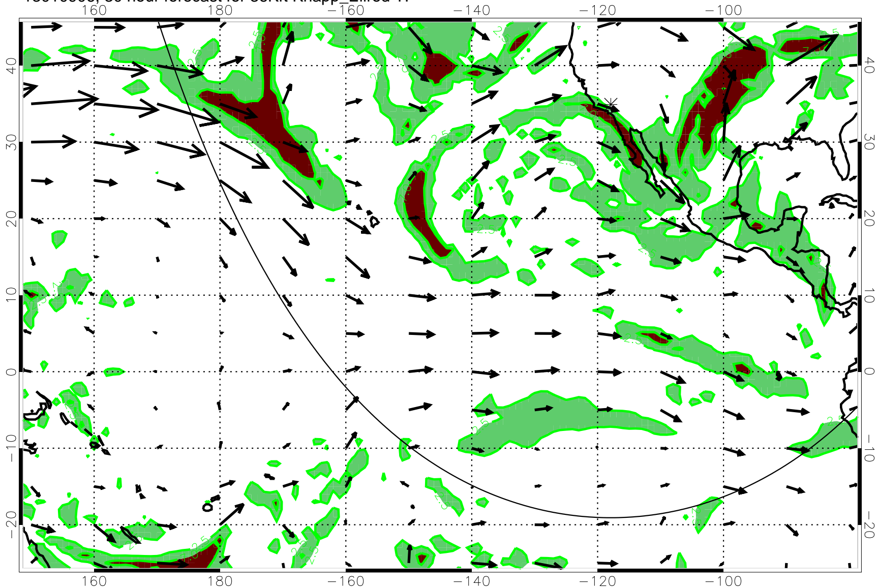
13010906, 30 hour forecast for 36Kft Knapp_Ellrod T1
