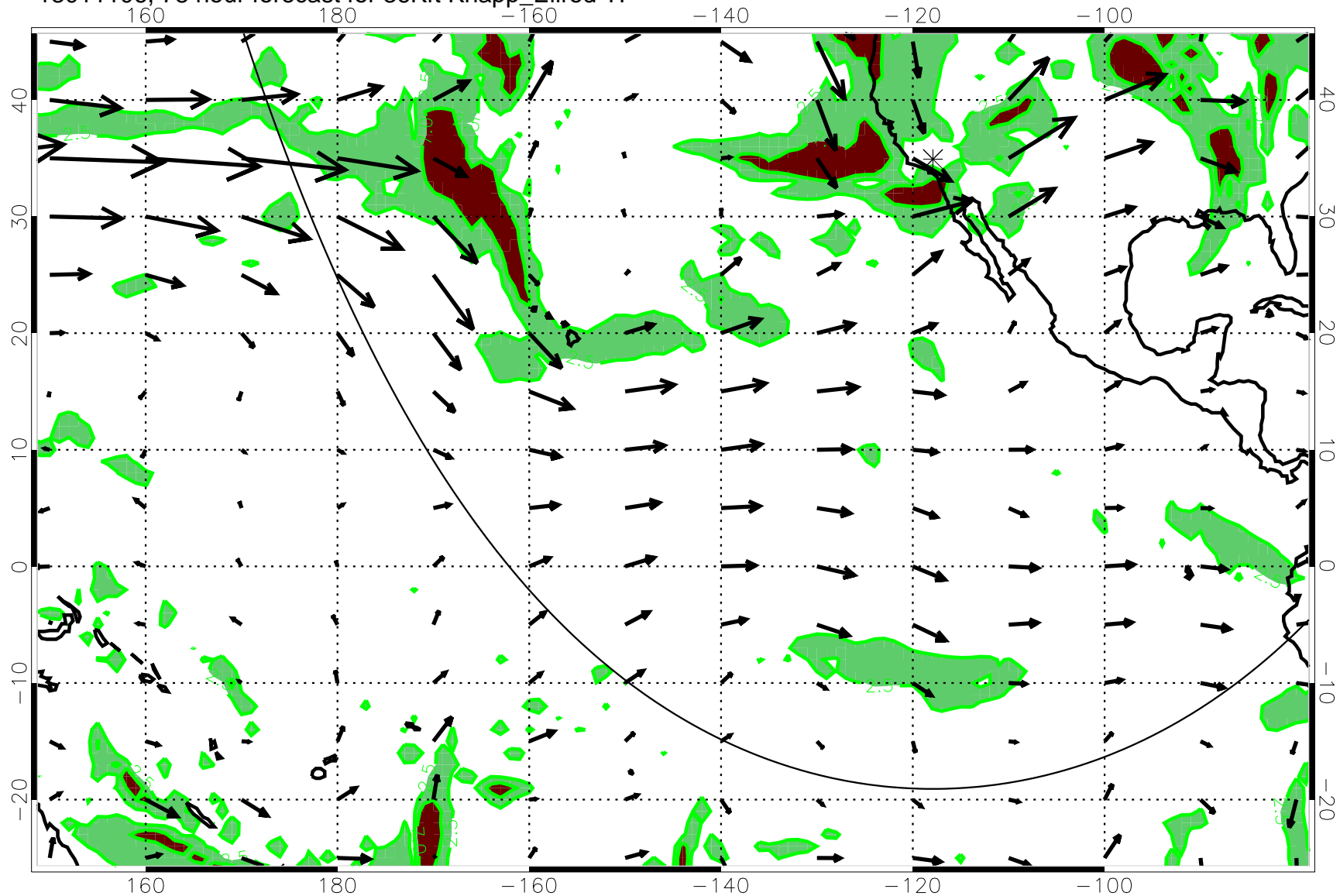
13011106, 78 hour forecast for 36Kft Knapp_Ellrod T1
