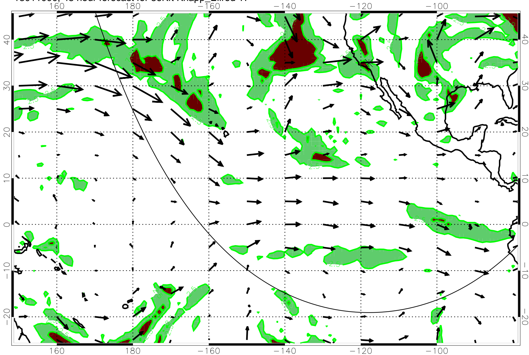
13011000, 48 hour forecast for 36Kft Knapp_Ellrod T1
