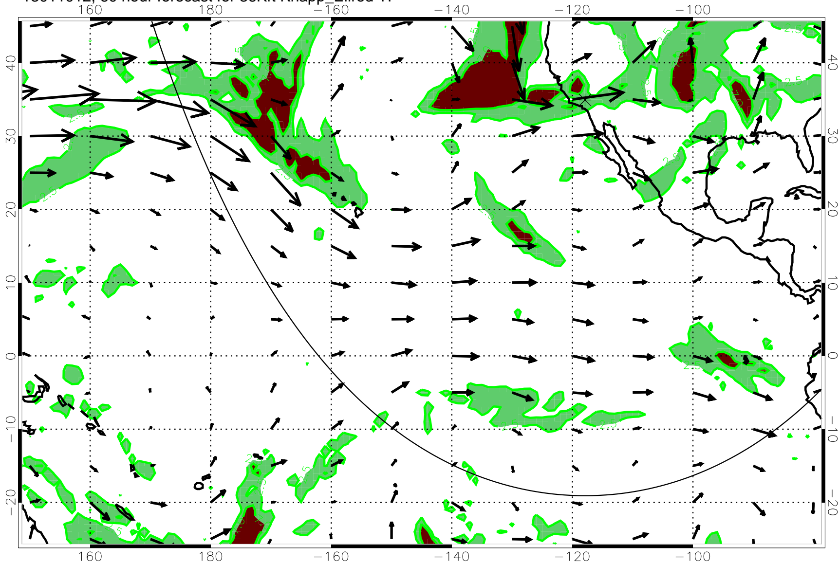
13011012, 60 hour forecast for 36Kft Knapp_Ellrod T1
