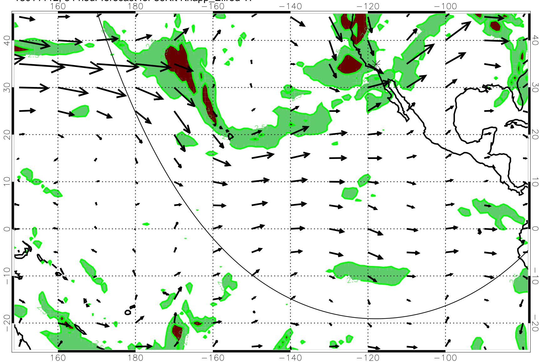
13011112, 84 hour forecast for 36Kft Knapp_Ellrod T1
