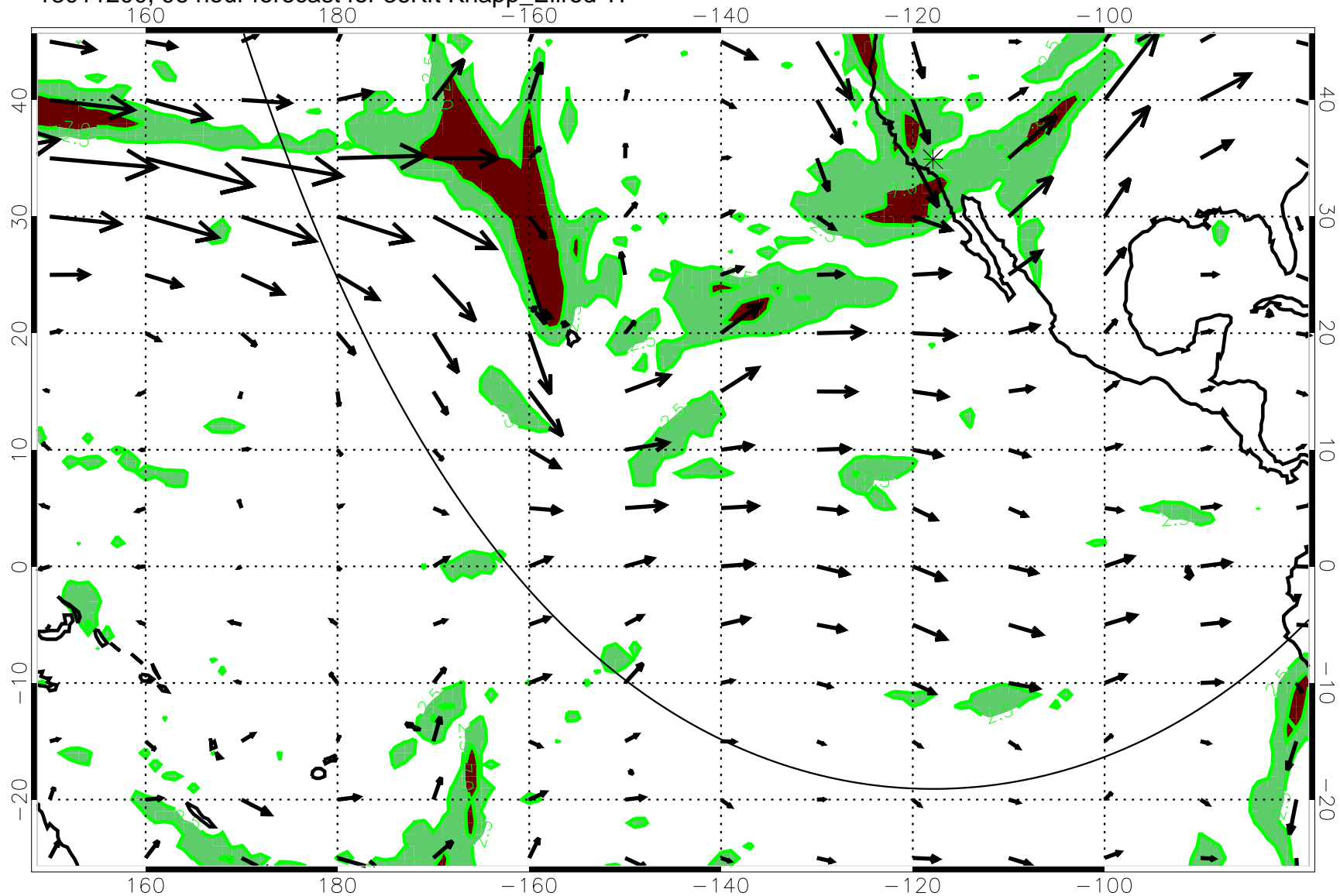
13011200, 96 hour forecast for 36Kft Knapp_Ellrod T1
