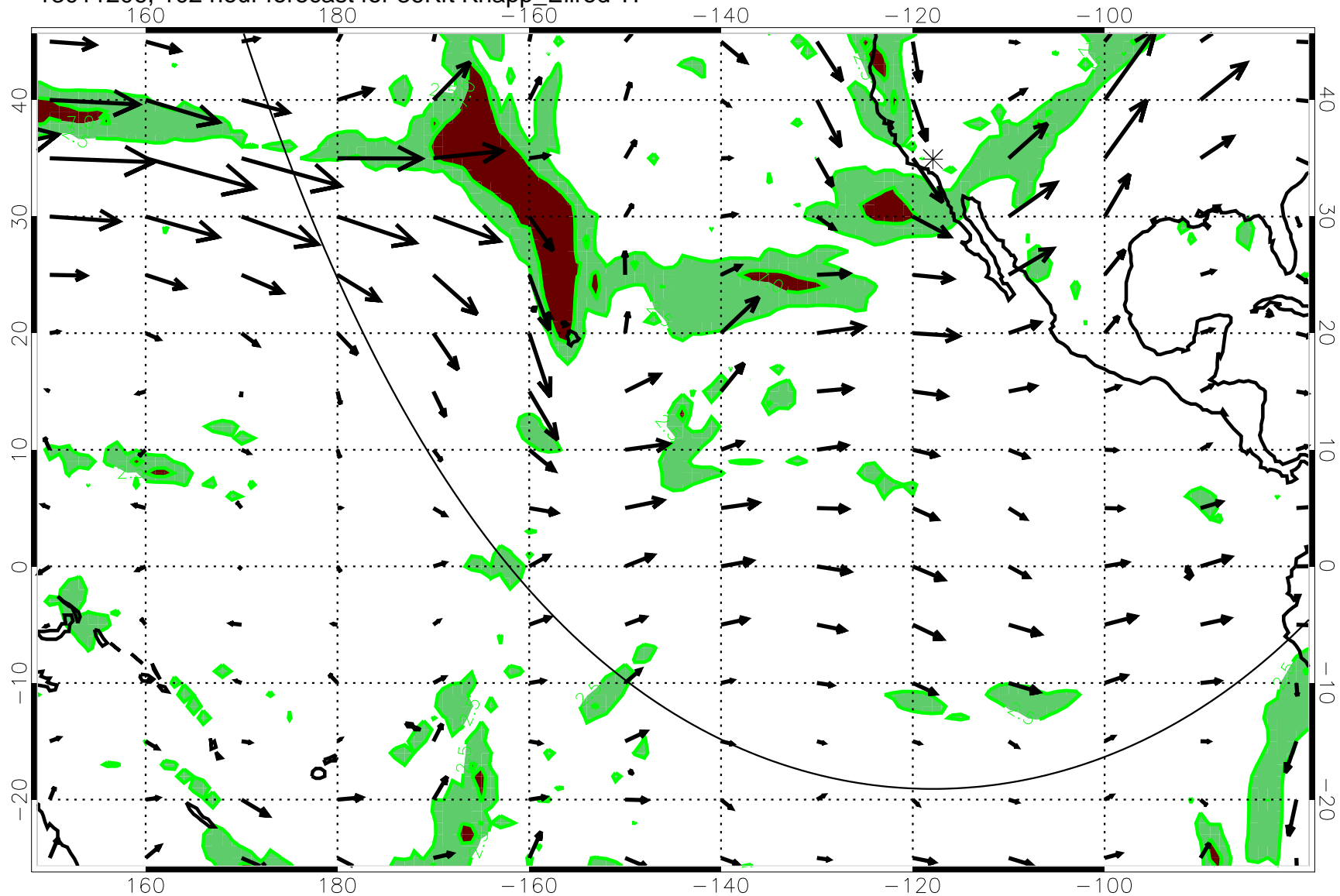
13011206, 102 hour forecast for 36Kft Knapp_Ellrod T1
