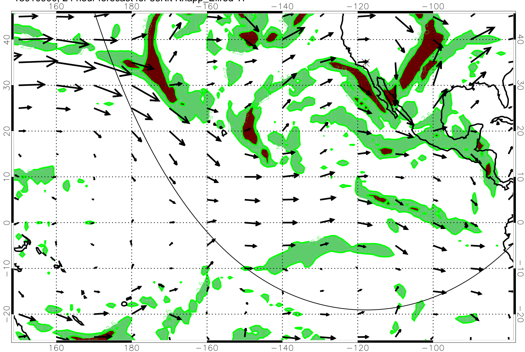
13010900, 24 hour forecast for 36Kft Knapp_Ellrod T1
