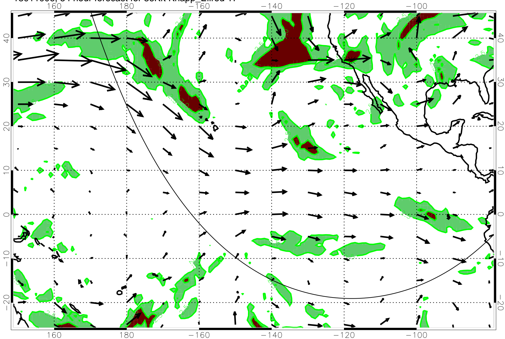
13011006, 54 hour forecast for 36Kft Knapp_Ellrod T1
