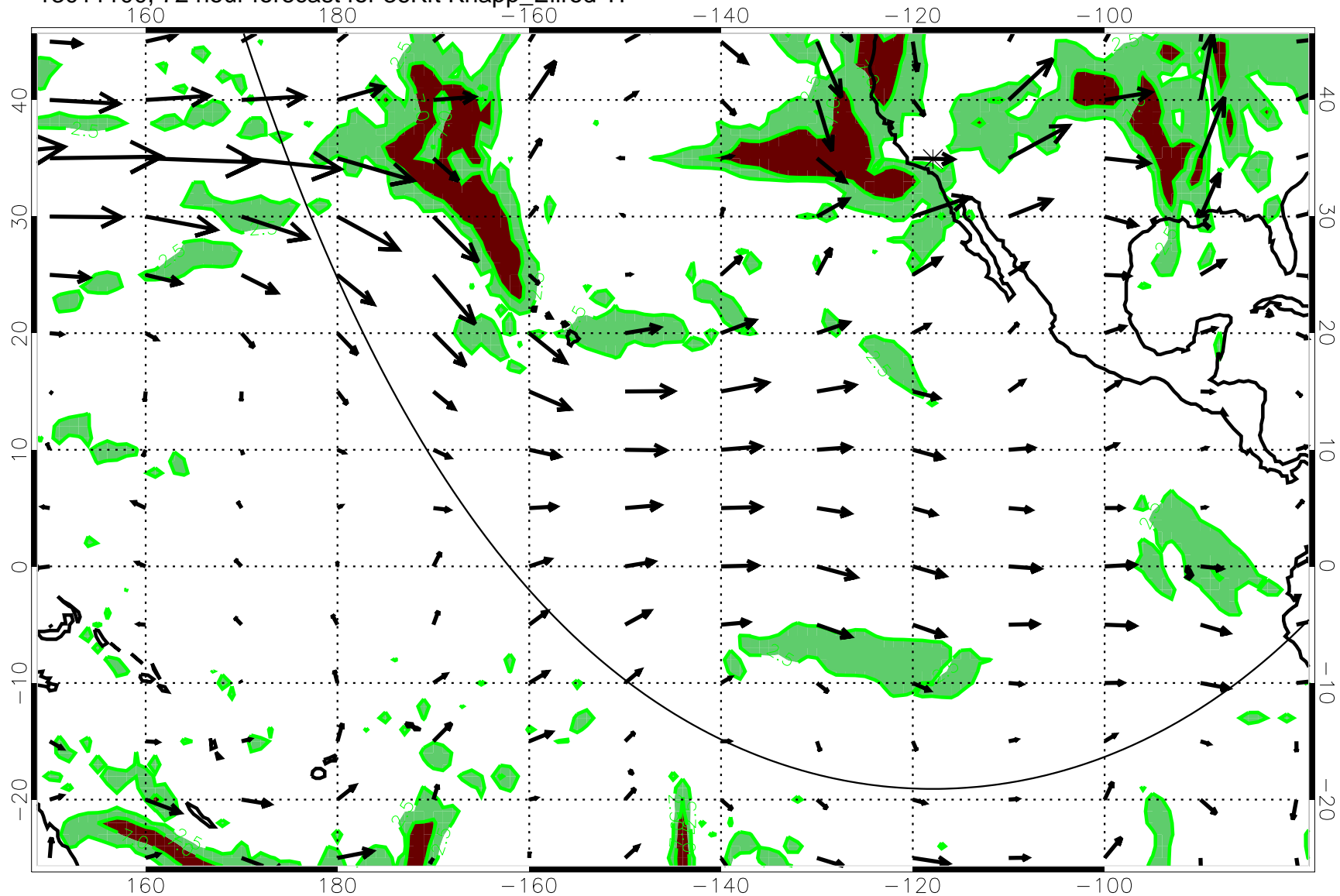
13011100, 72 hour forecast for 36Kft Knapp_Ellrod T1
