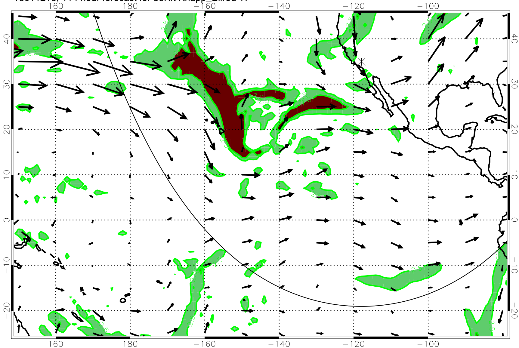
13011218, 114 hour forecast for 36Kft Knapp_Ellrod T1
