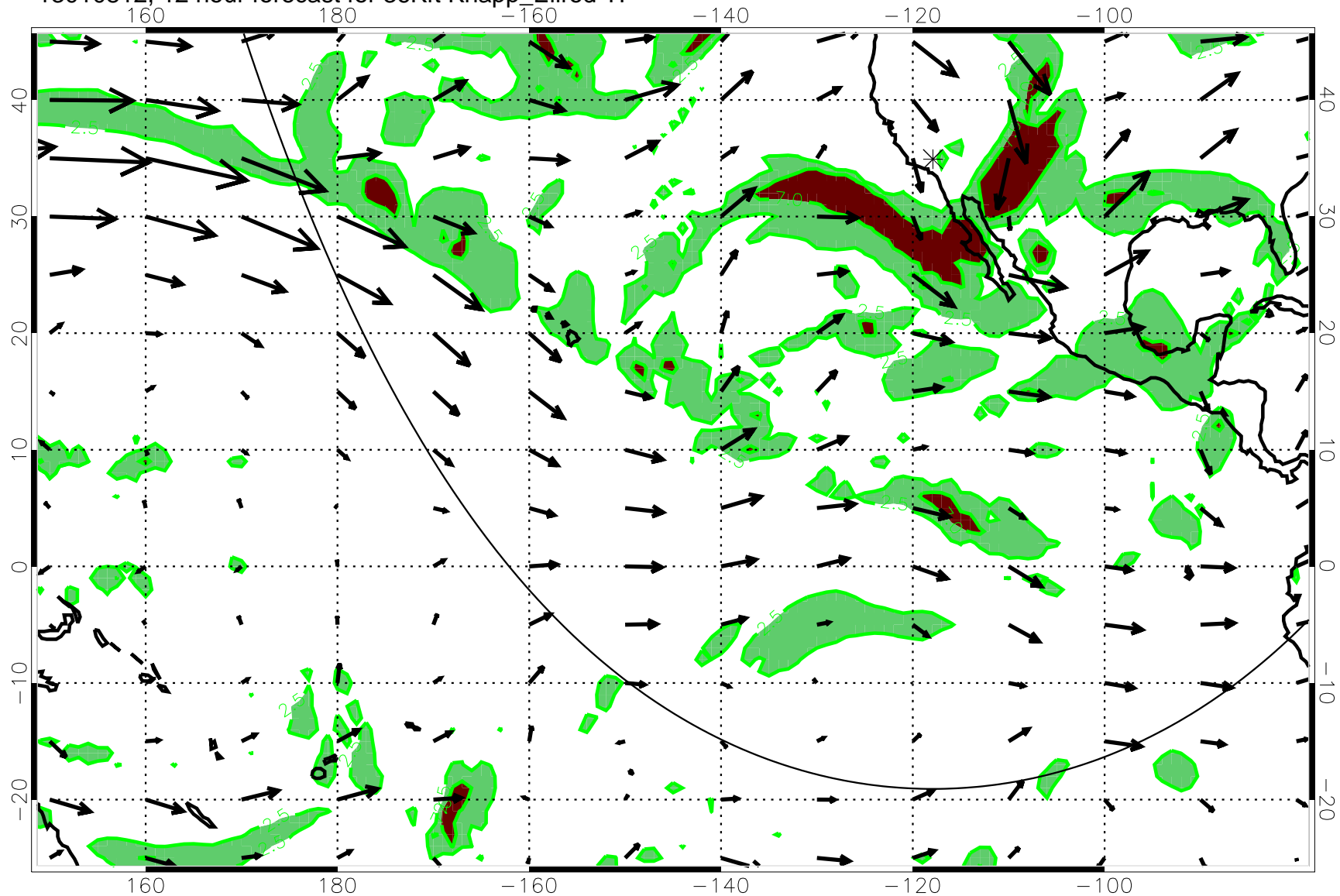
13010812, 12 hour forecast for 36Kft Knapp_Ellrod TI
