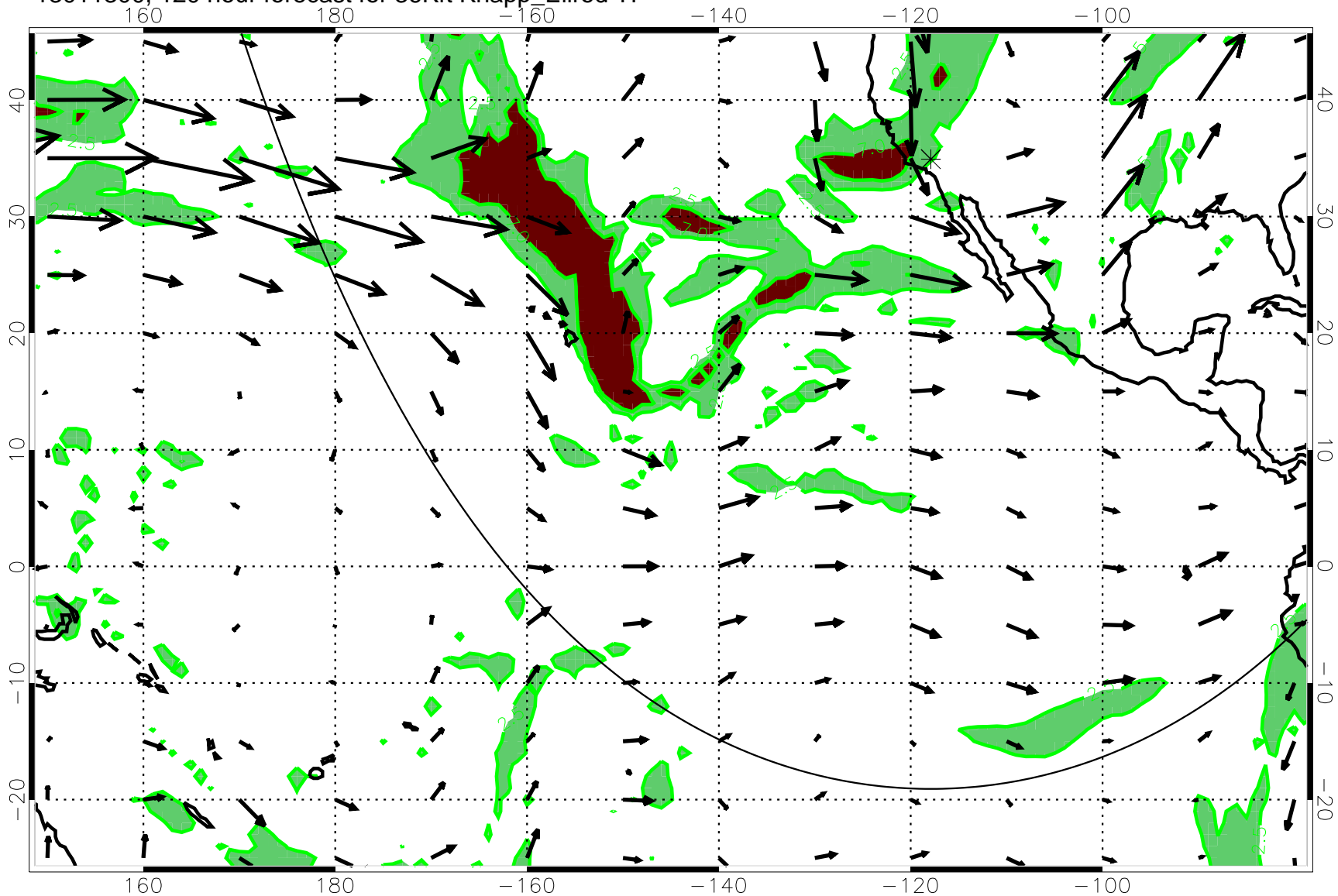
13011300, 120 hour forecast for 36Kft Knapp_Ellrod T1
