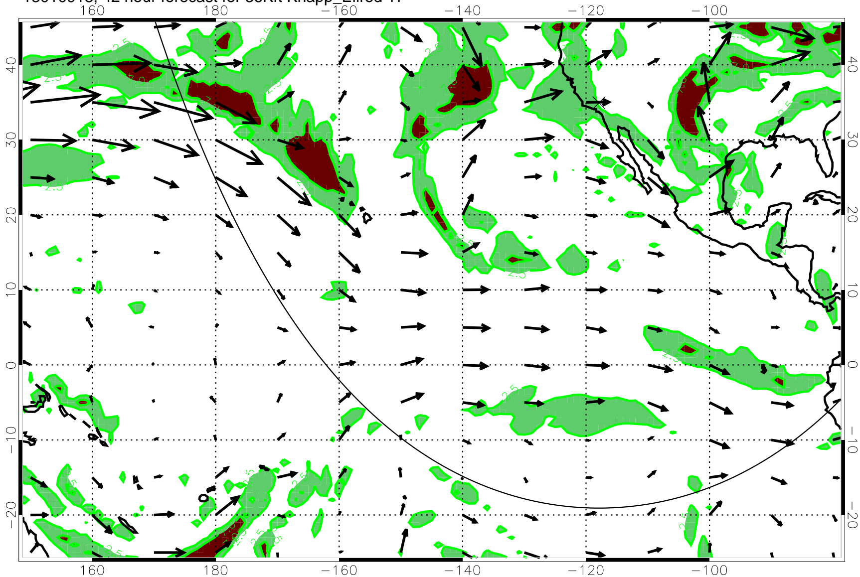
13010918, 42 hour forecast for 36Kft Knapp_Ellrod T1
