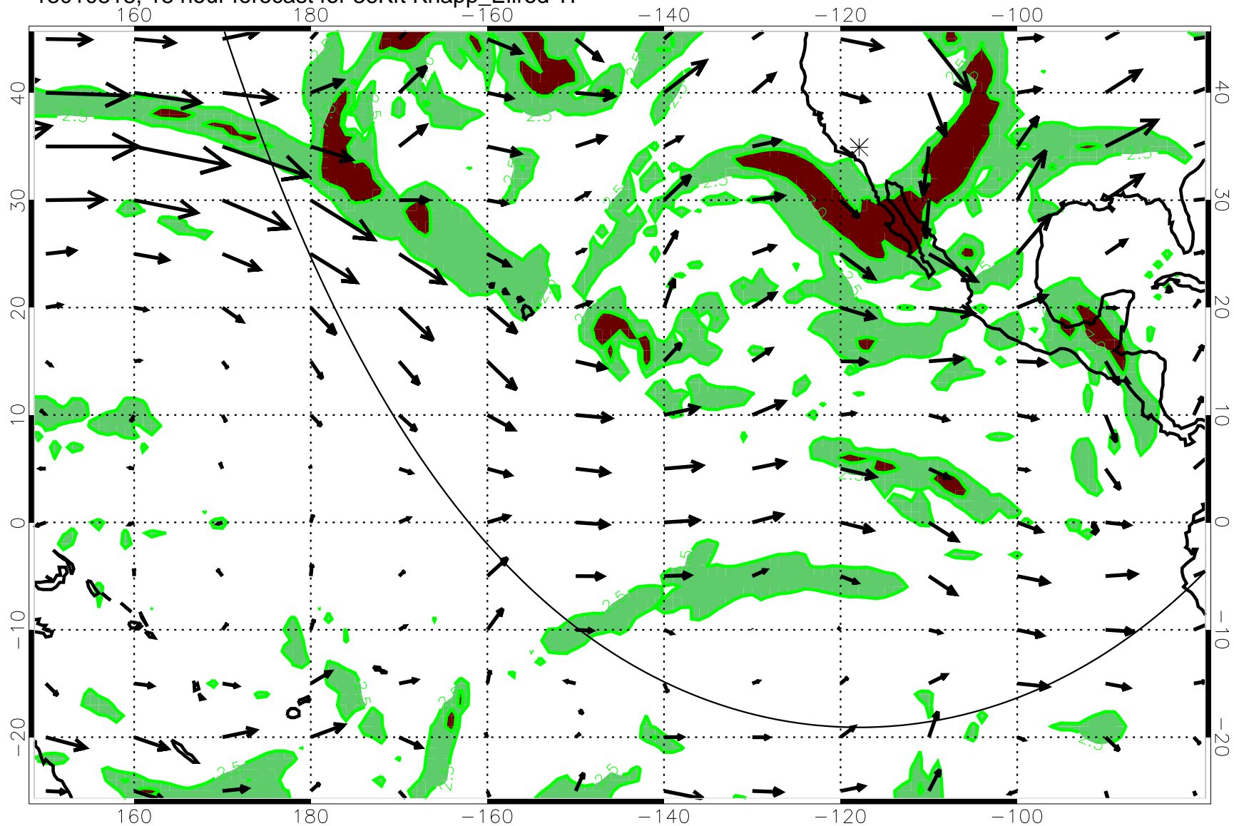
13010818, 18 hour forecast for 36Kft Knapp_Ellrod TI
