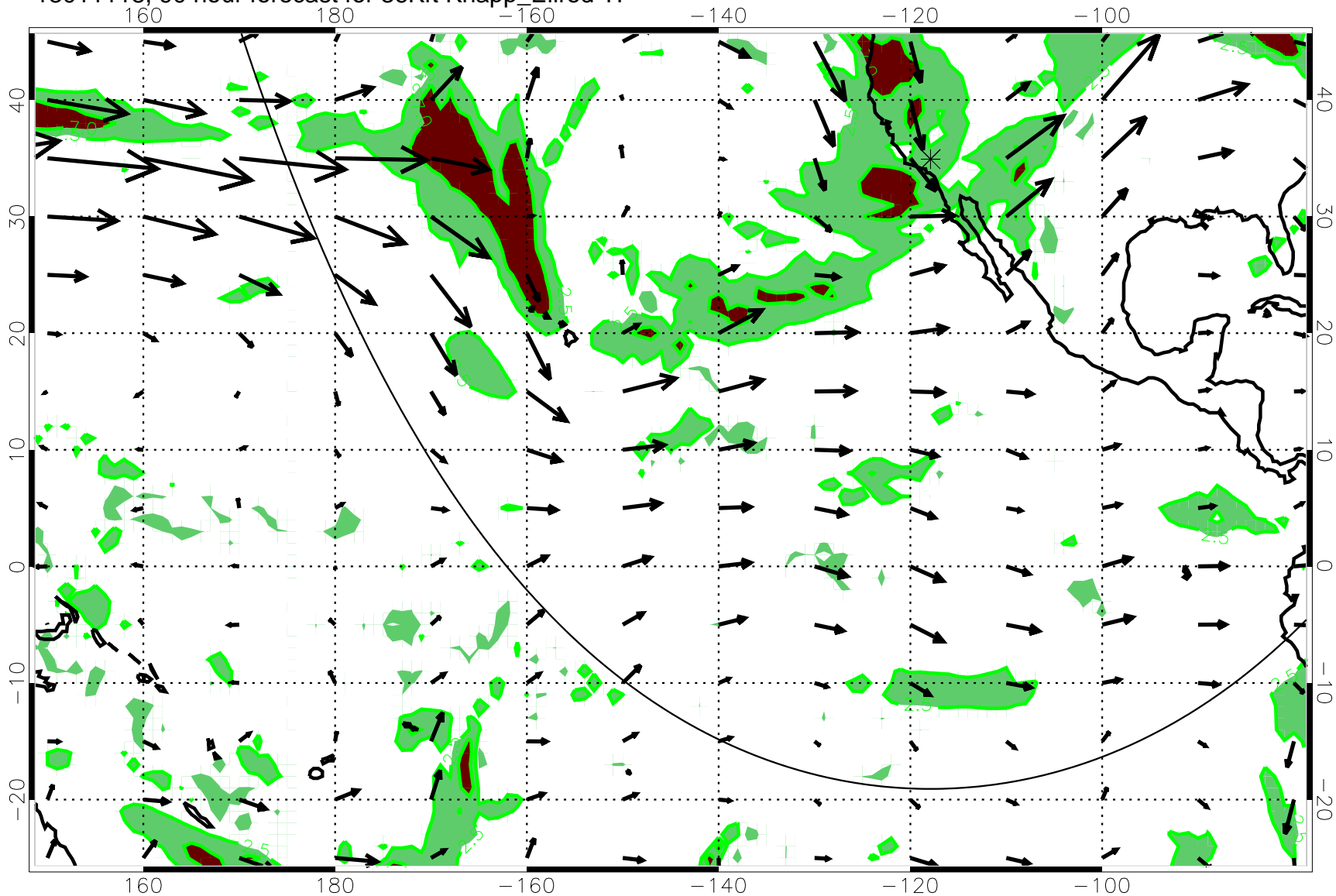
13011118, 90 hour forecast for 36Kft Knapp_Ellrod T1
