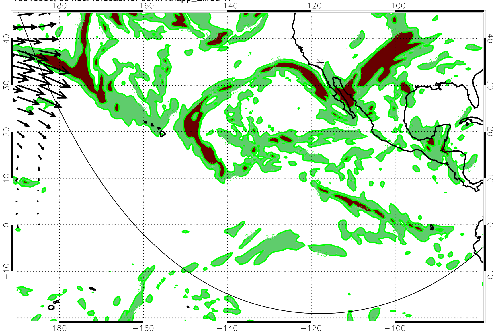
13010900, 36 hour forecast for 36Kft Knapp_Ellrod TI
