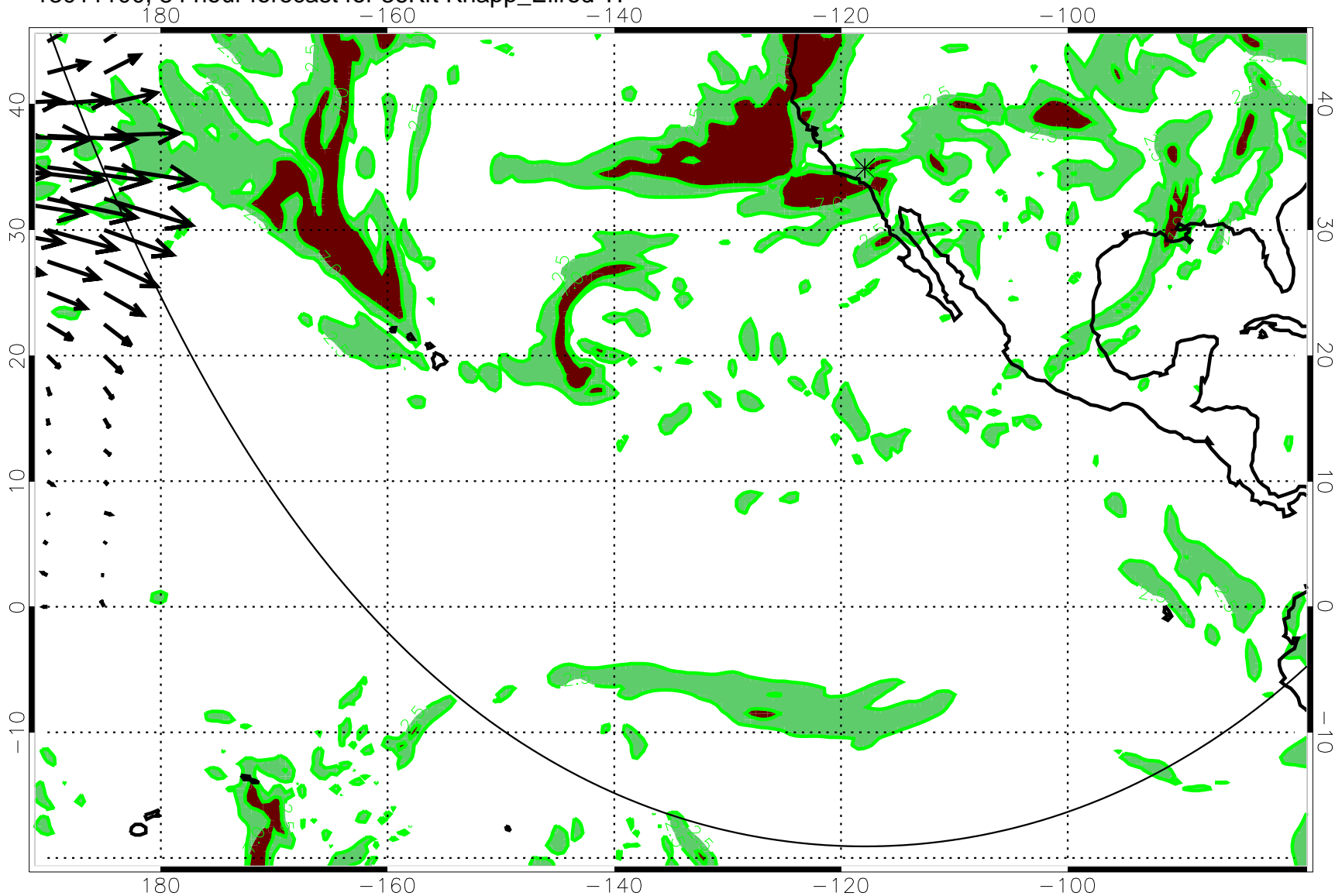
13011100, 84 hour forecast for 36Kft Knapp_Ellrod TI
