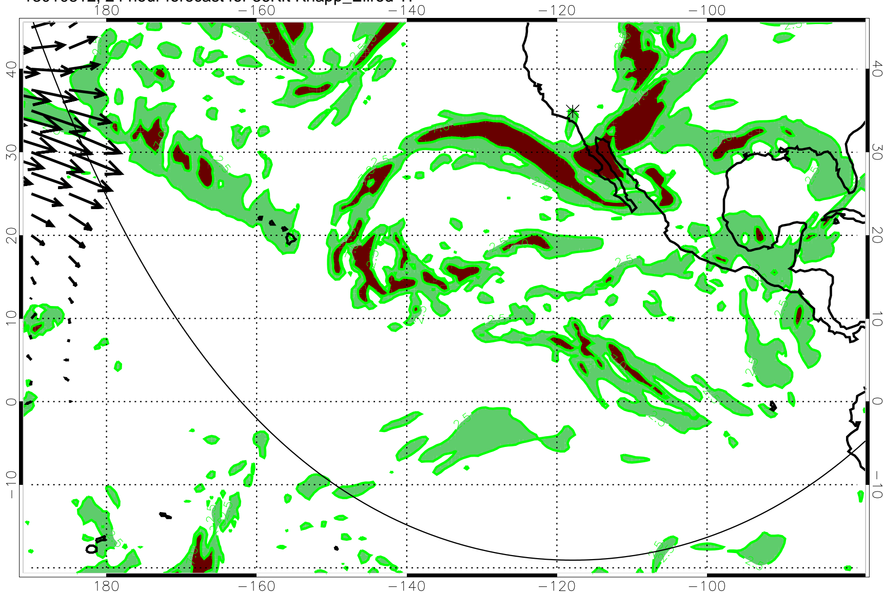
13010812, 24 hour forecast for 36Kft Knapp_Ellrod TI
