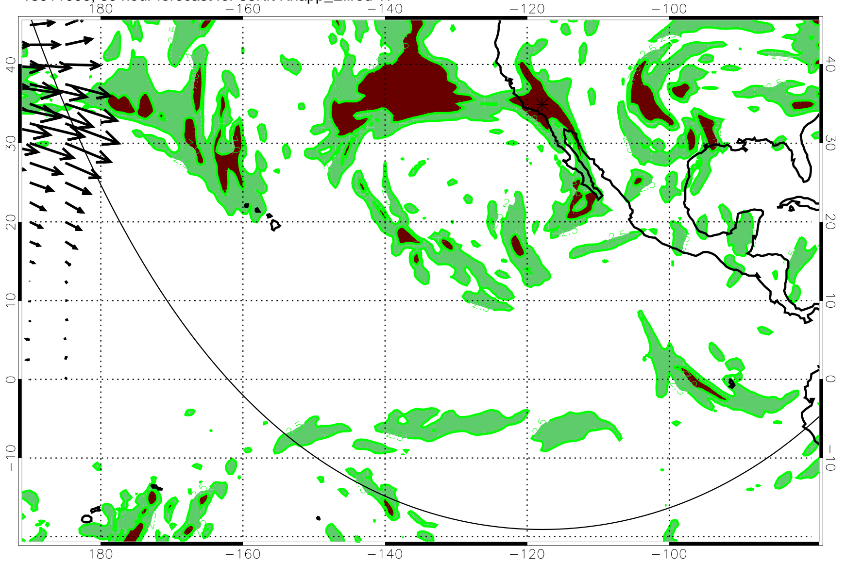
13011000, 60 hour forecast for 36Kft Knapp_Ellrod TI
