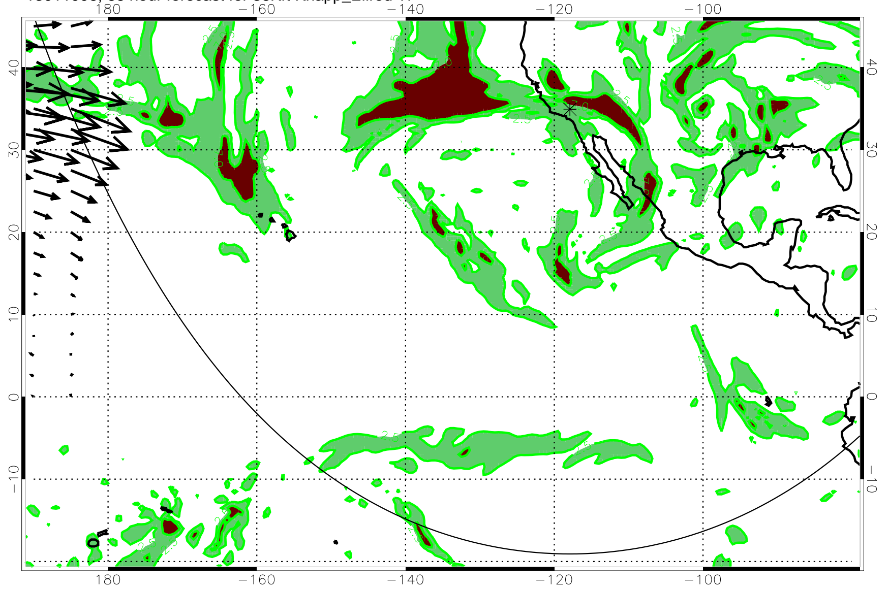
13011006, 66 hour forecast for 36Kft Knapp_Ellrod TI
