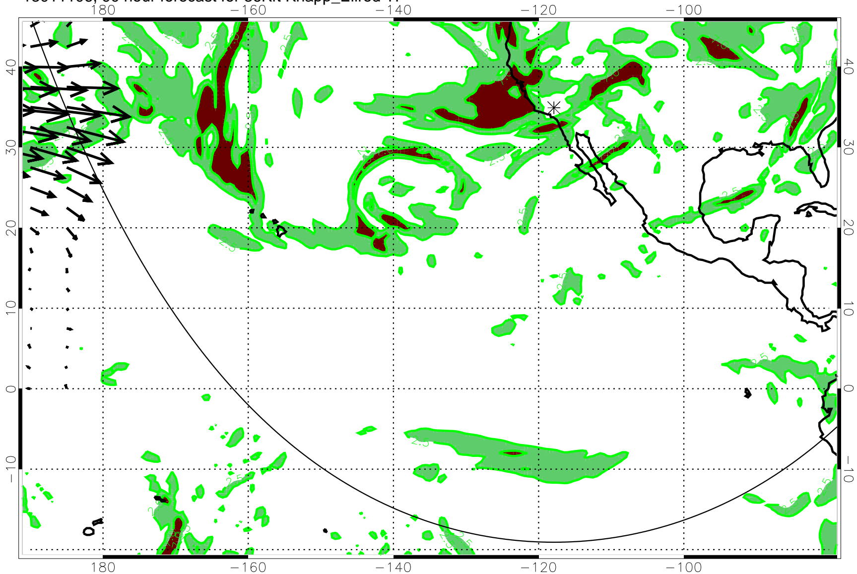
13011106, 90 hour forecast for 36Kft Knapp_Ellrod TI
