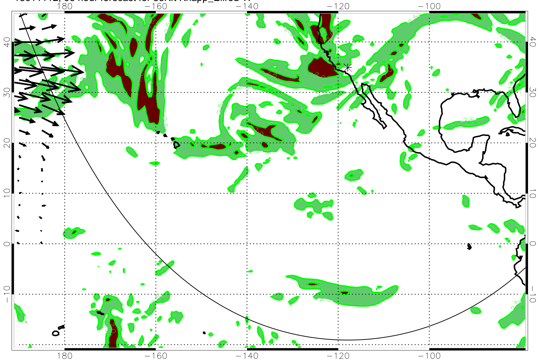
13011112, 96 hour forecast for 36Kft Knapp_Ellrod TI
