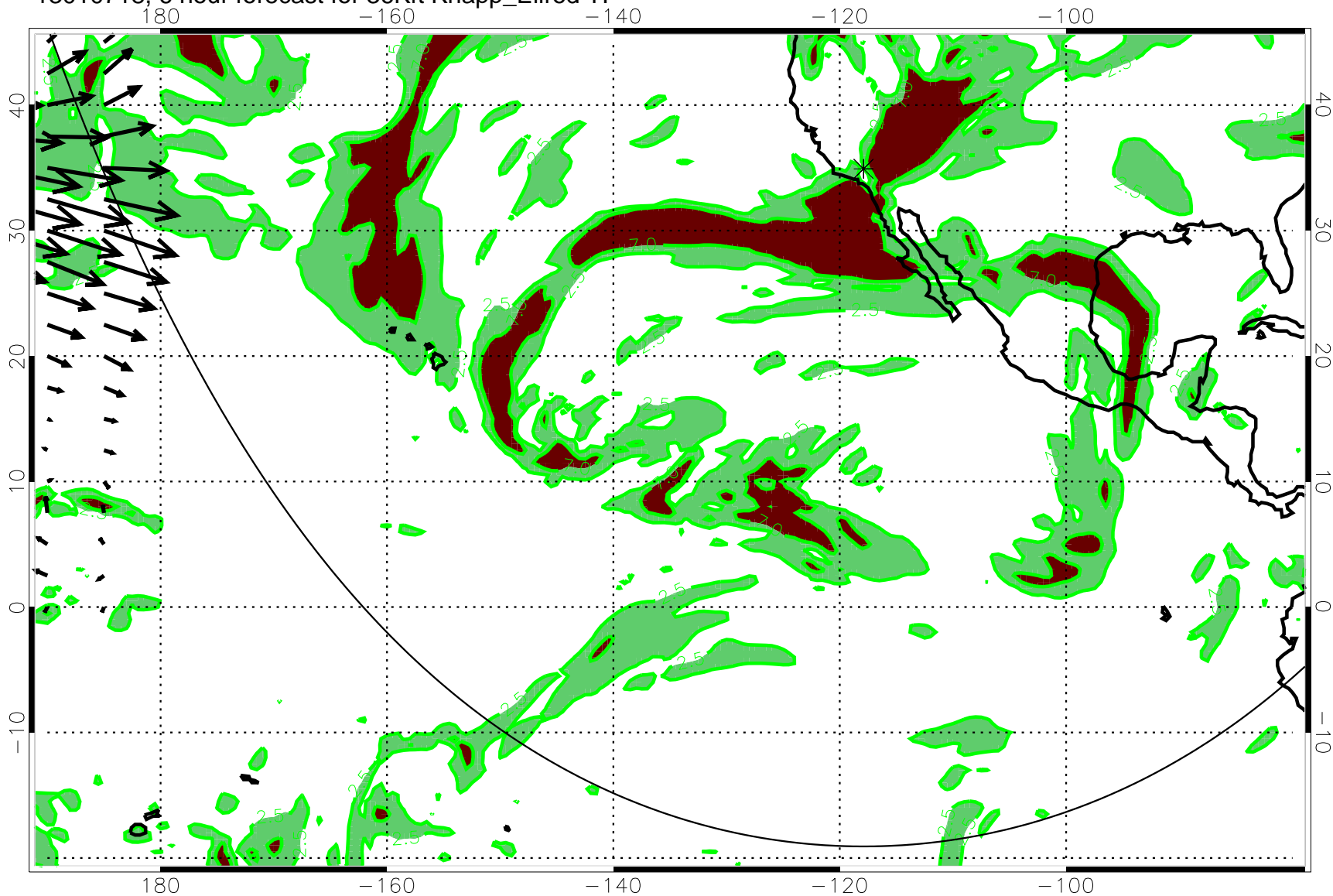
13010718, 6 hour forecast for 36Kft Knapp_Ellrod TI
