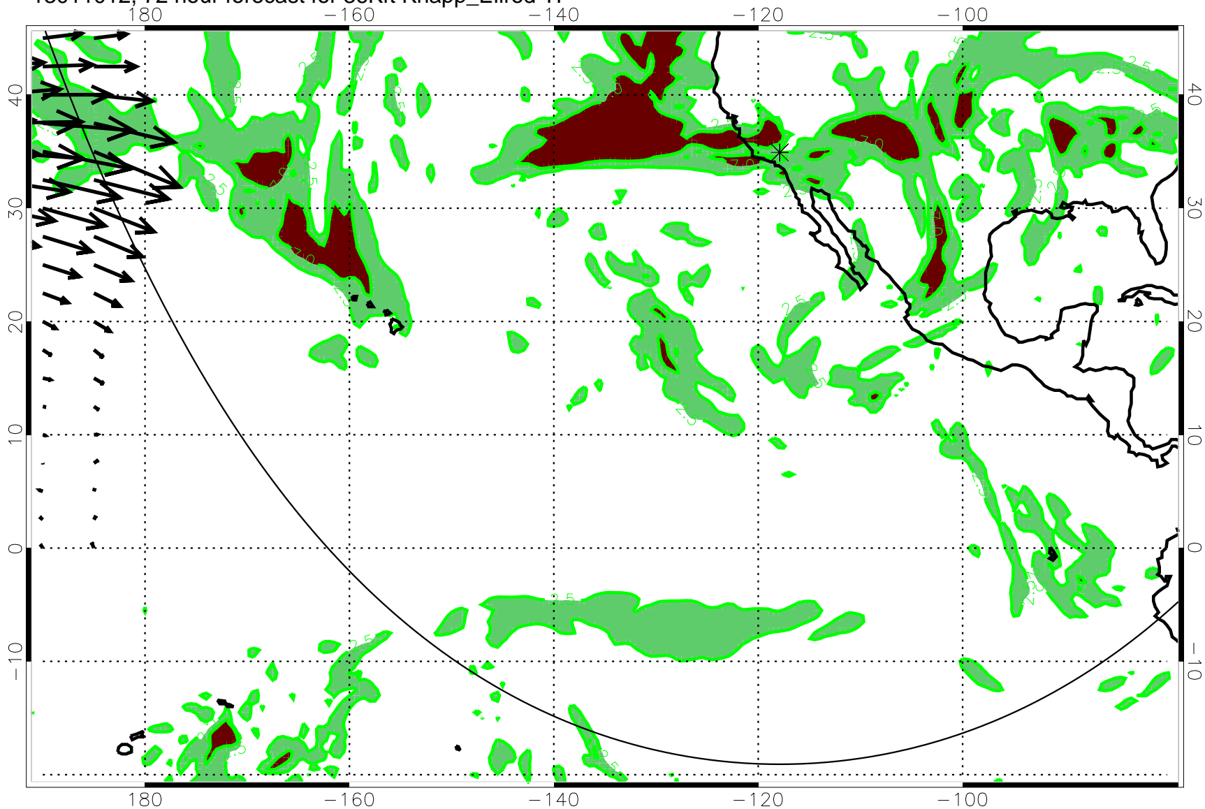
13011012, 72 hour forecast for 36Kft Knapp_Ellrod TI
