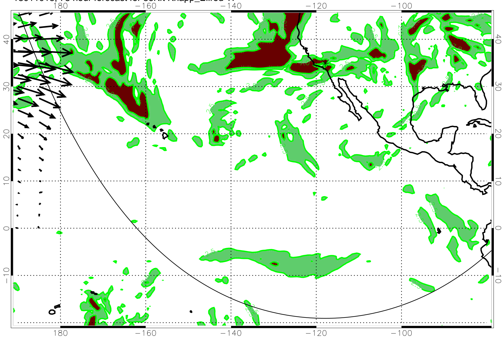
13011018, 78 hour forecast for 36Kft Knapp_Ellrod TI
