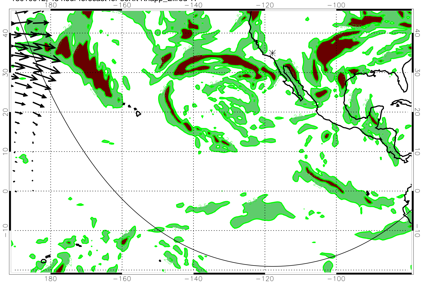
13010912, 48 hour forecast for 36Kft Knapp_Ellrod TI
