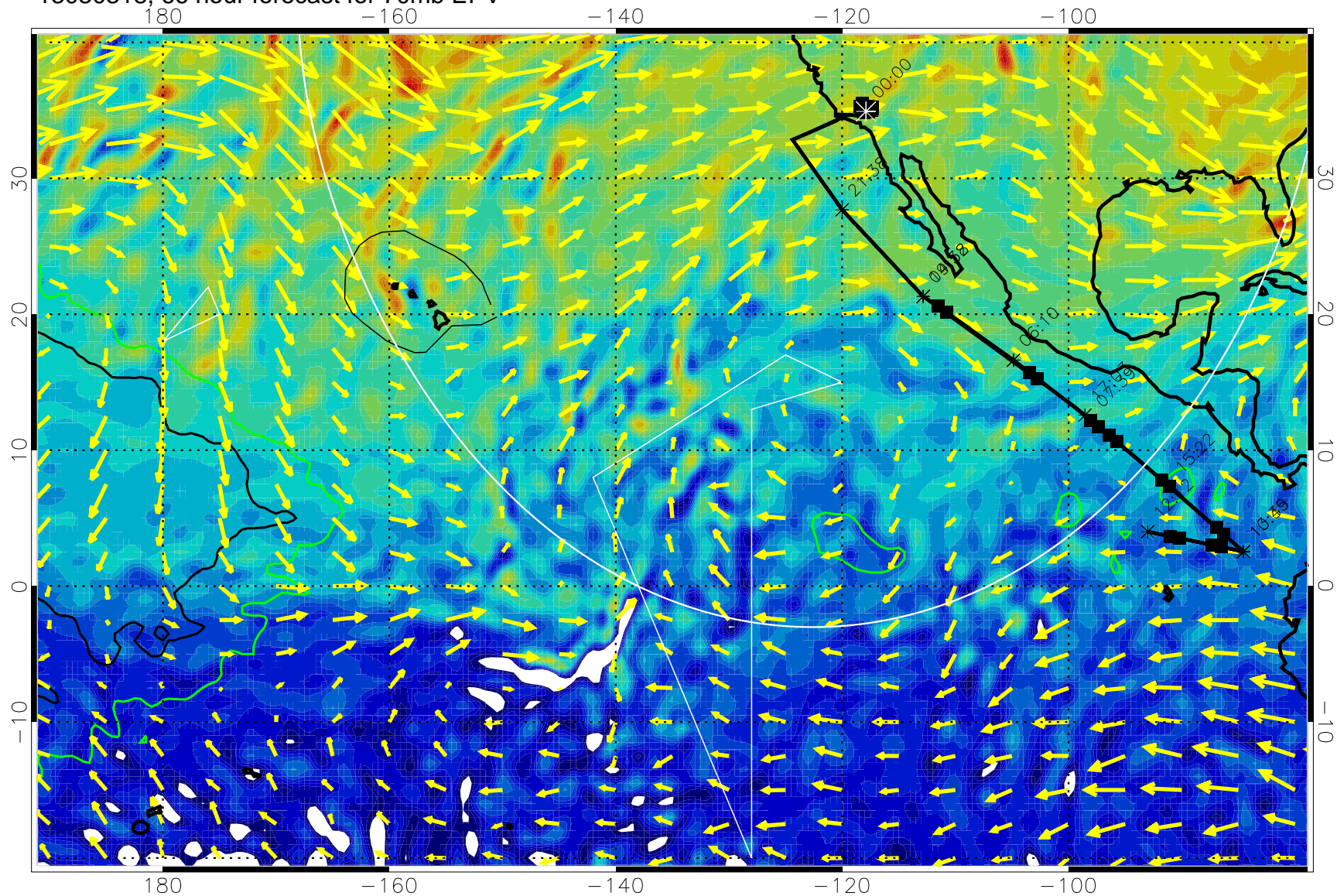
13030318, 66 hour forecast for 70mb EPV
