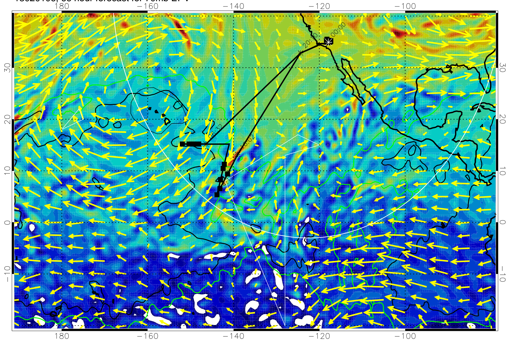
13020106, 66 hour forecast for 70mb EPV
