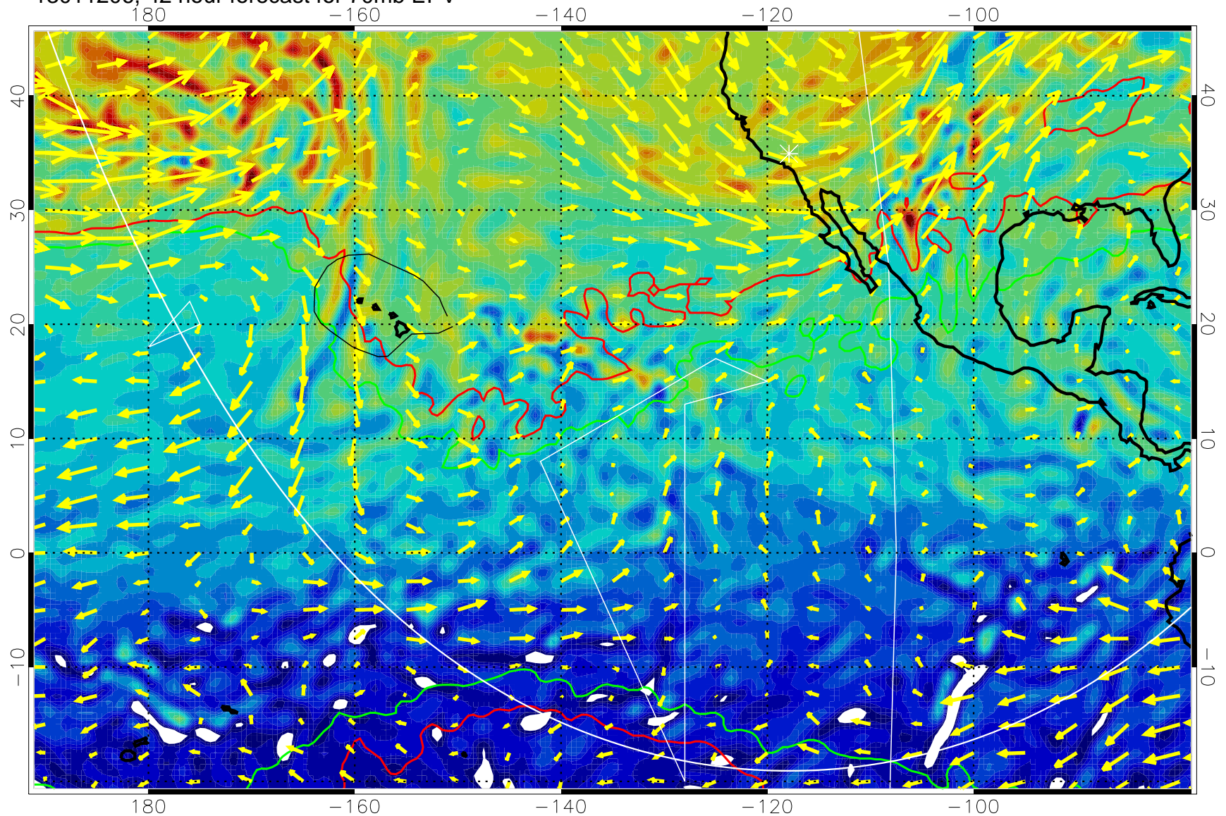
13011206, 42 hour forecast for 70mb EPV
