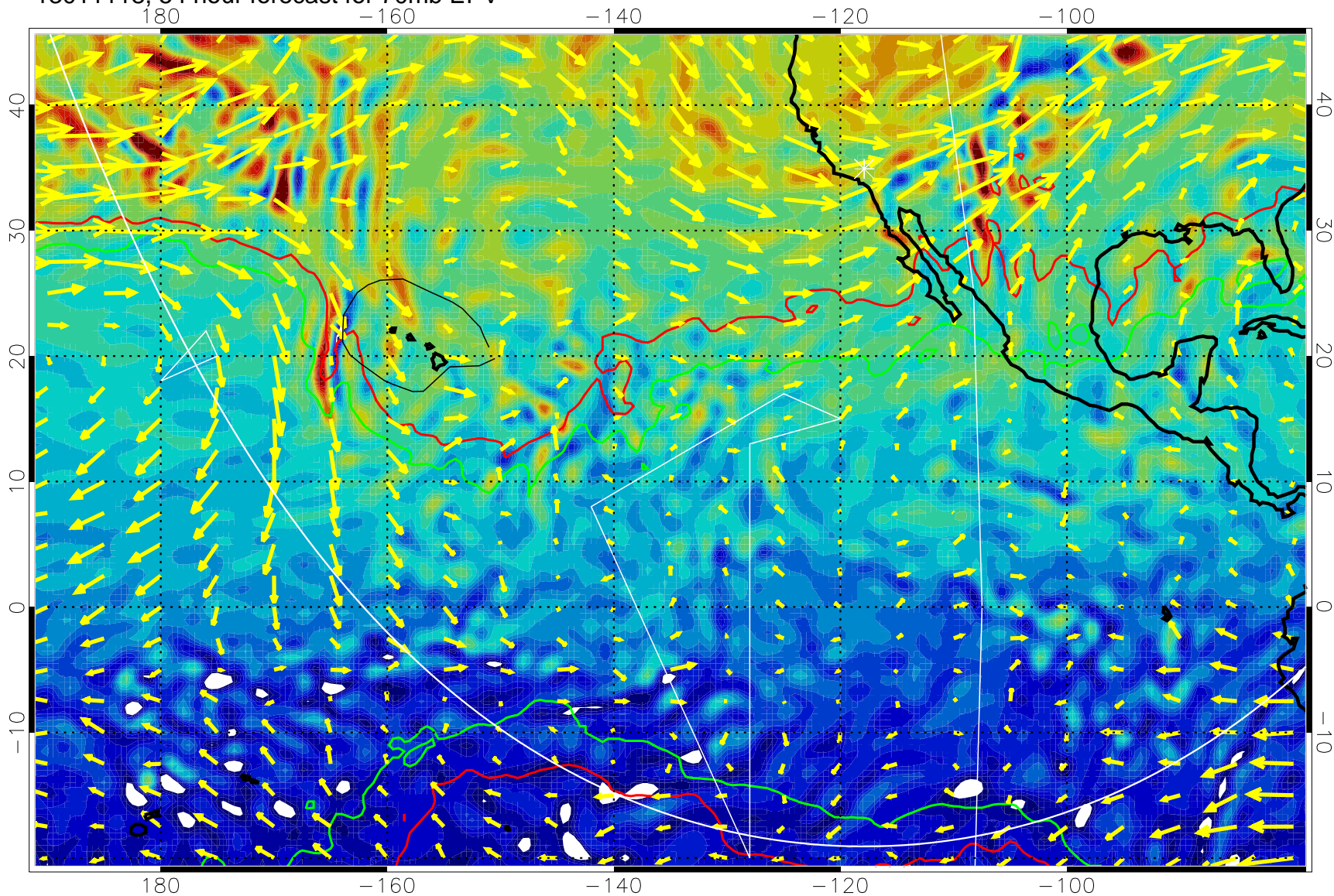
13011118, 54 hour forecast for 70mb EPV
