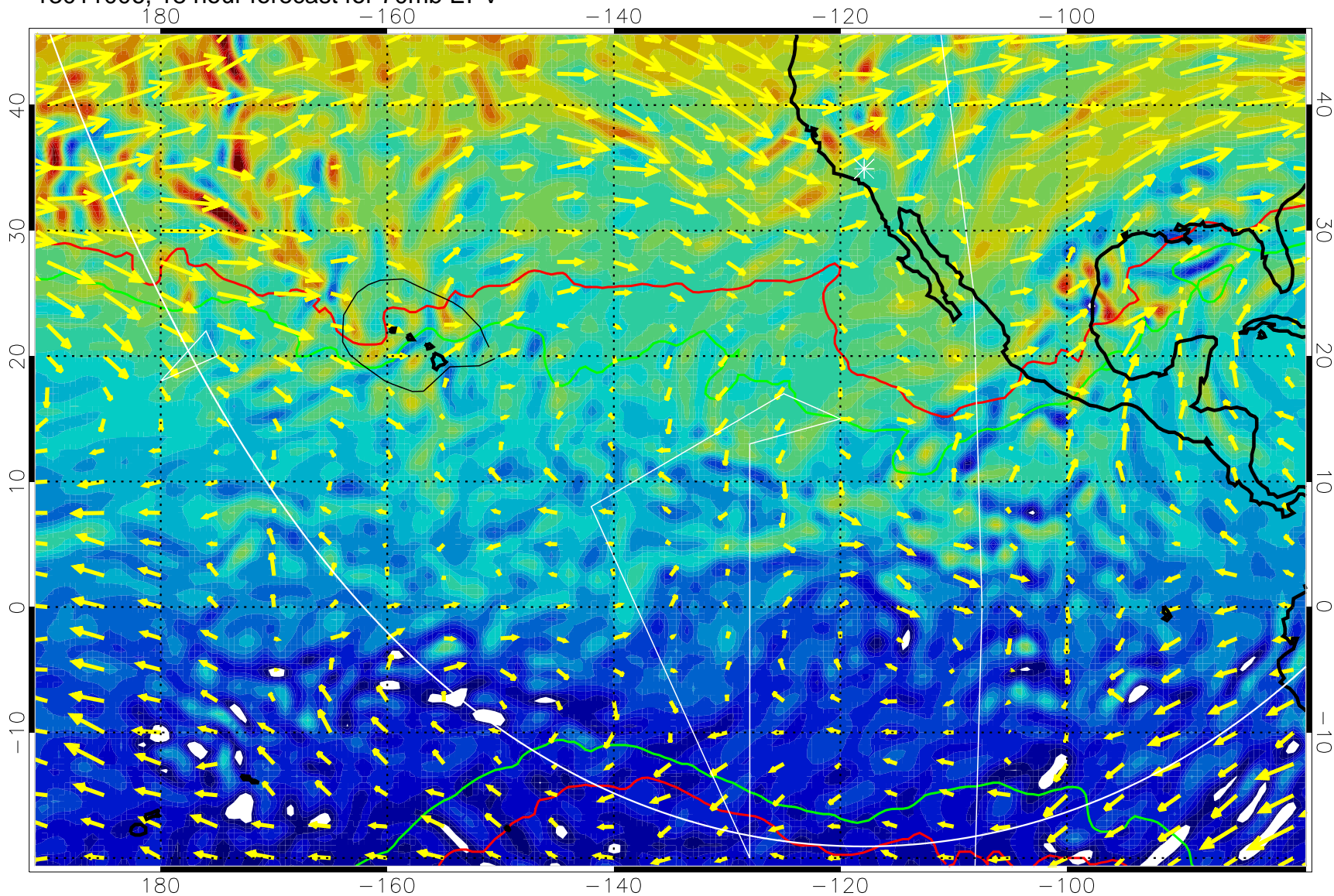
13011006, 18 hour forecast for 70mb EPV
