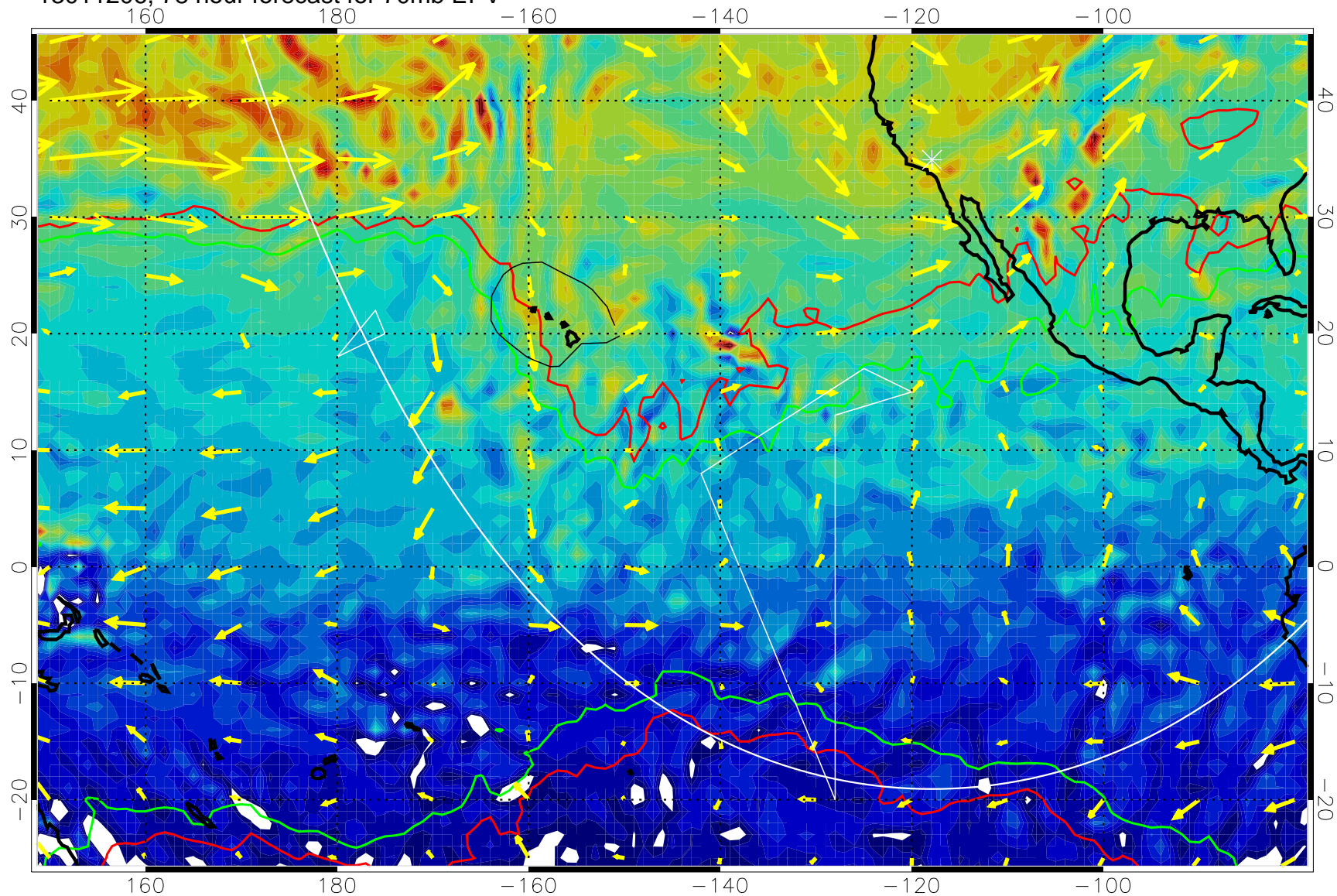
13011206, 78 hour forecast for 70mb EPV
