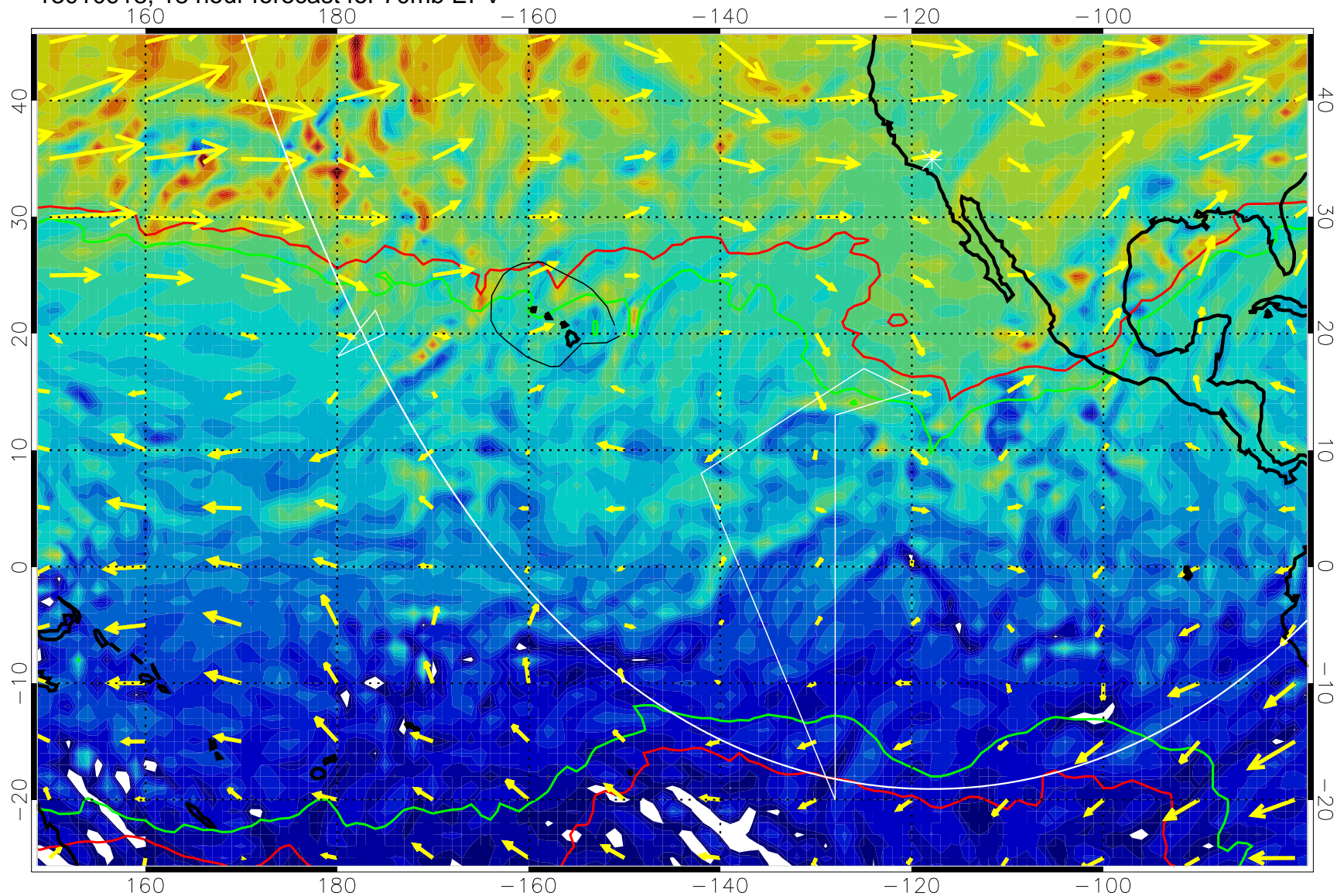
13010918, 18 hour forecast for 70mb EPV
