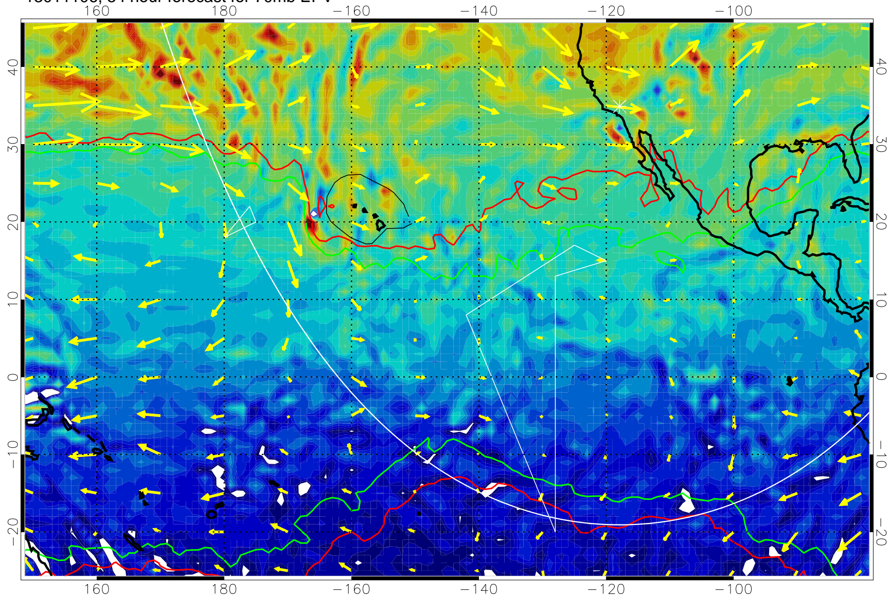
13011106, 54 hour forecast for 70mb EPV
