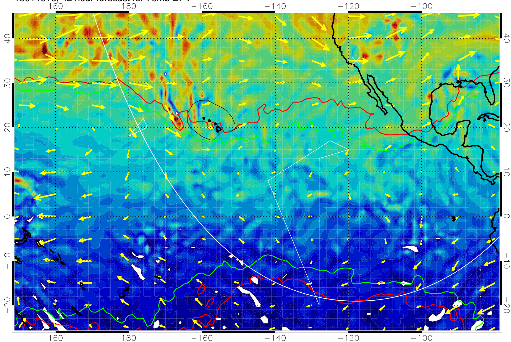
13011018, 42 hour forecast for 70mb EPV
