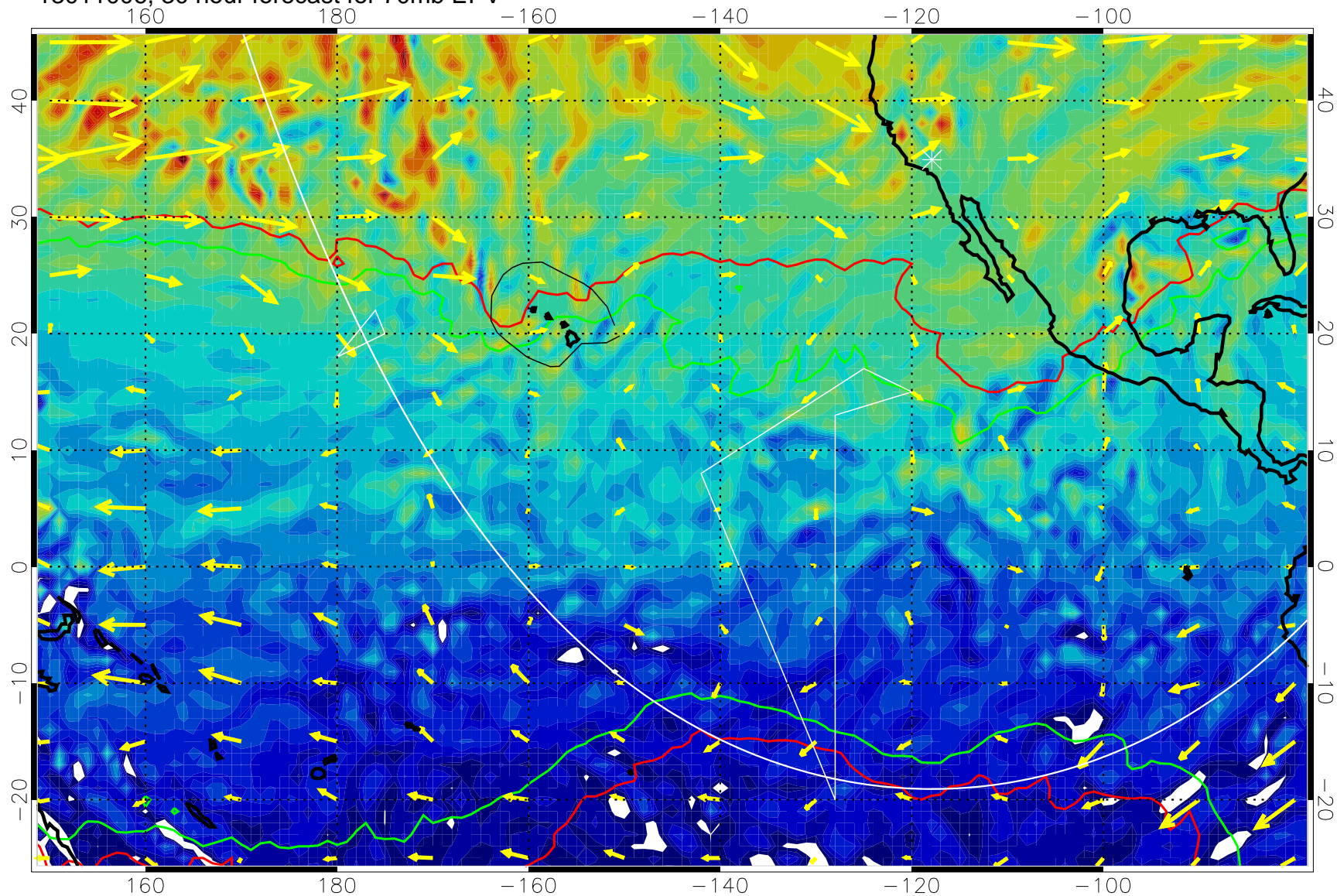
13011006, 30 hour forecast for 70mb EPV
