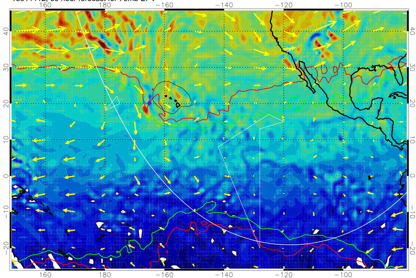
13011112, 60 hour forecast for 70mb EPV
