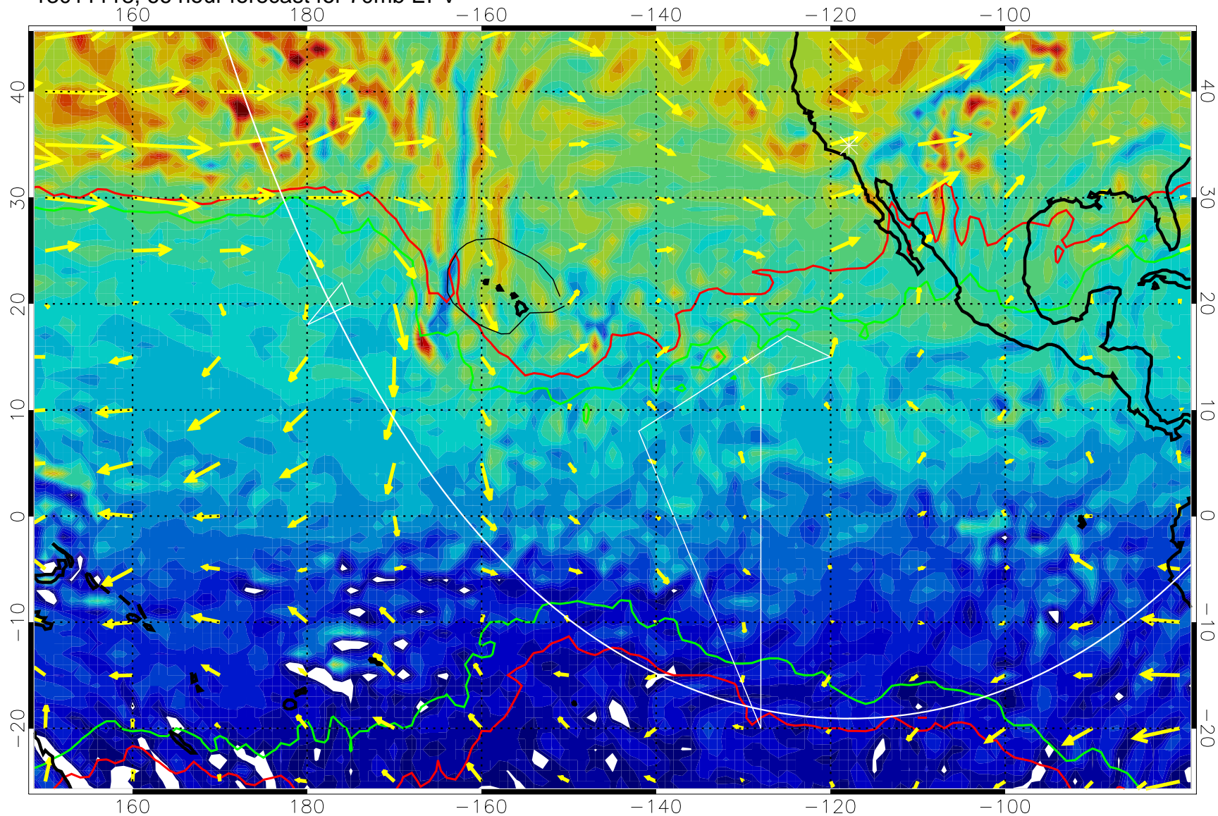
13011118, 66 hour forecast for 70mb EPV
