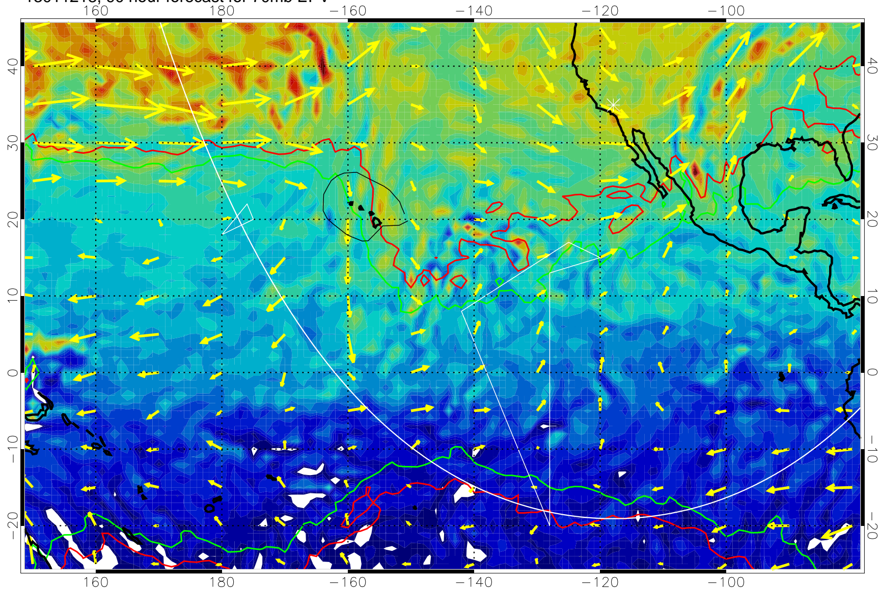
13011218, 90 hour forecast for 70mb EPV
