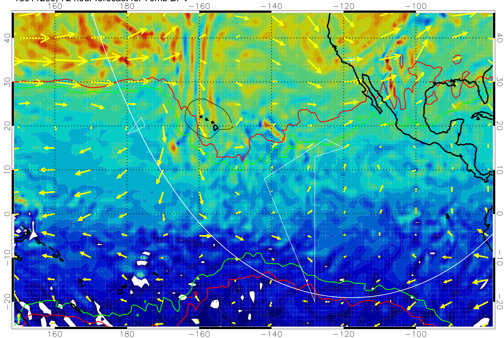
13011200, 72 hour forecast for 70mb EPV
