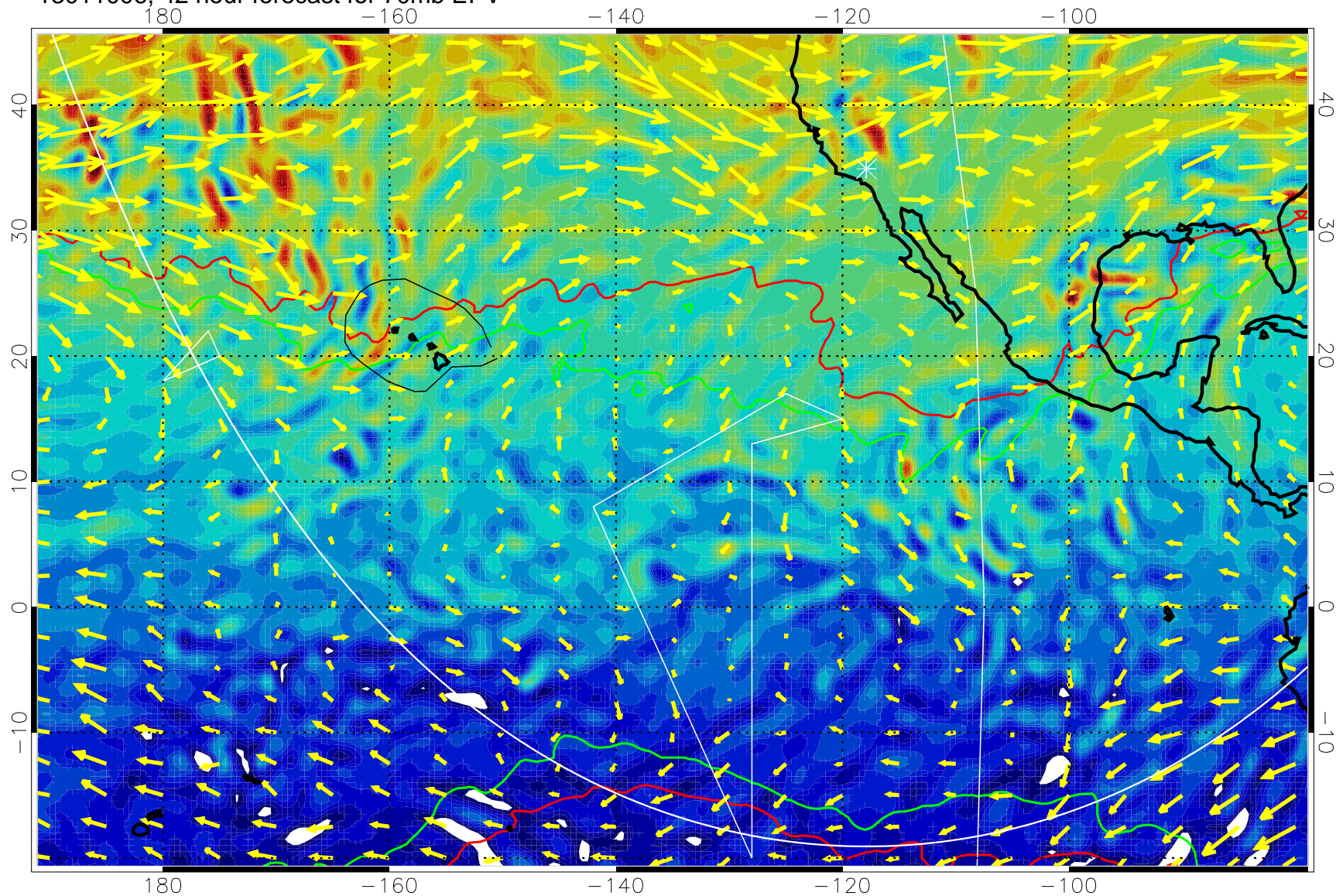
13011006, 42 hour forecast for 70mb EPV
