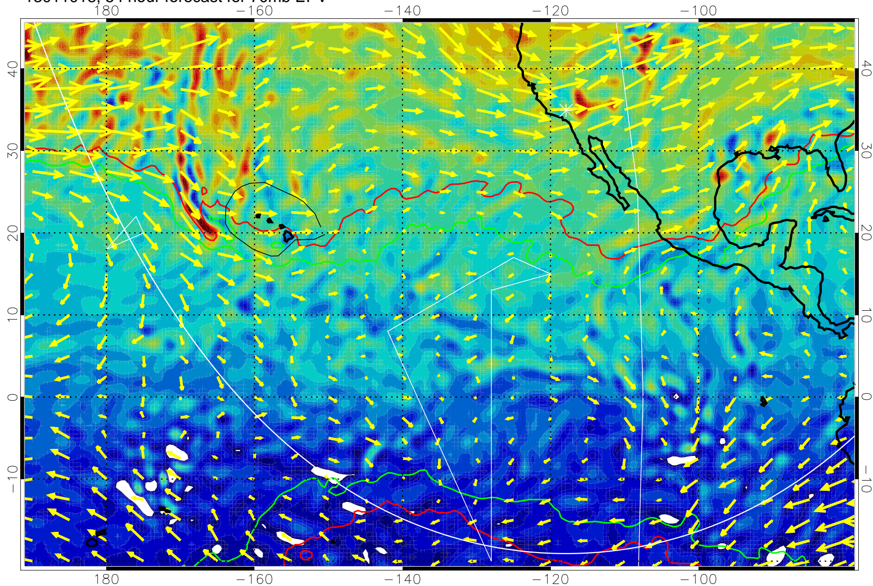
13011018, 54 hour forecast for 70mb EPV
