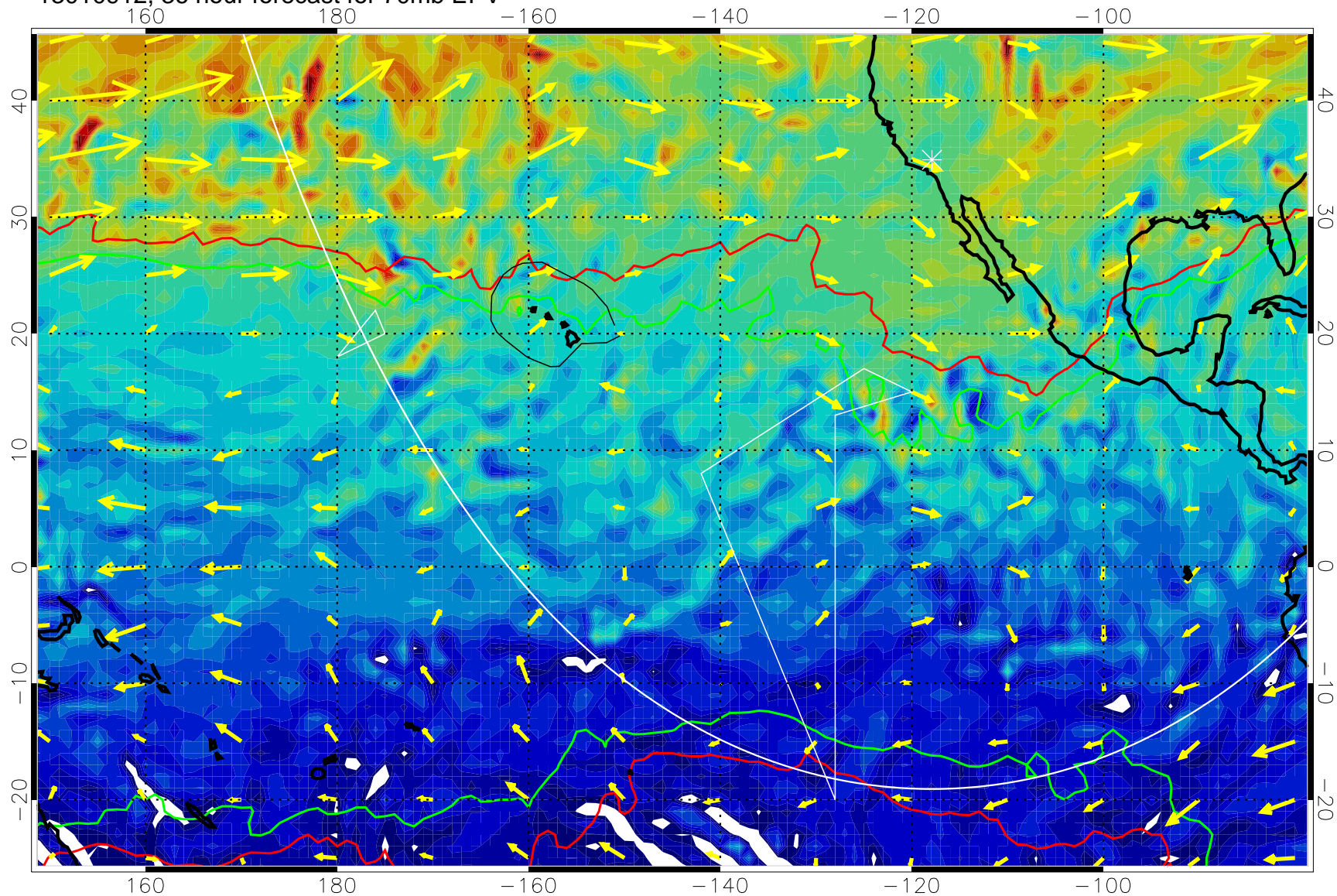
13010912, 36 hour forecast for 70mb EPV
