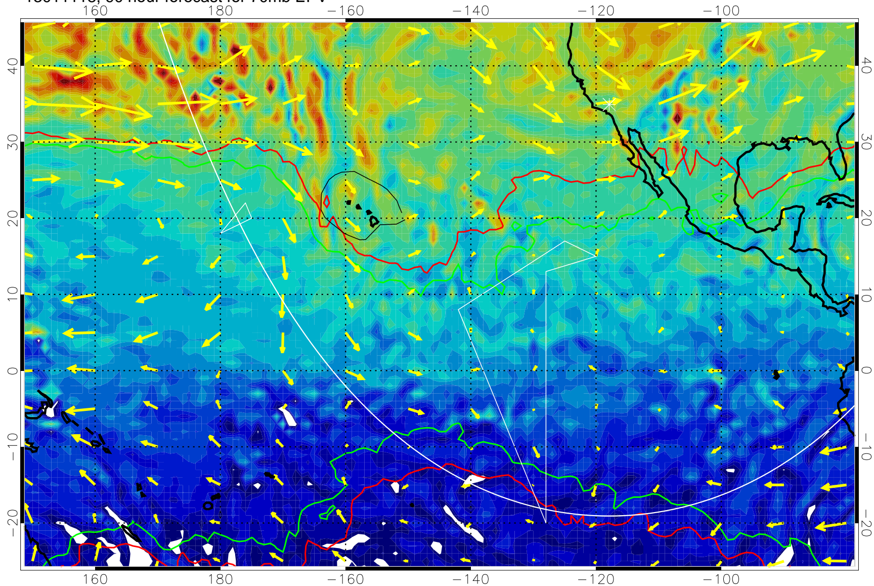
13011118, 90 hour forecast for 70mb EPV
