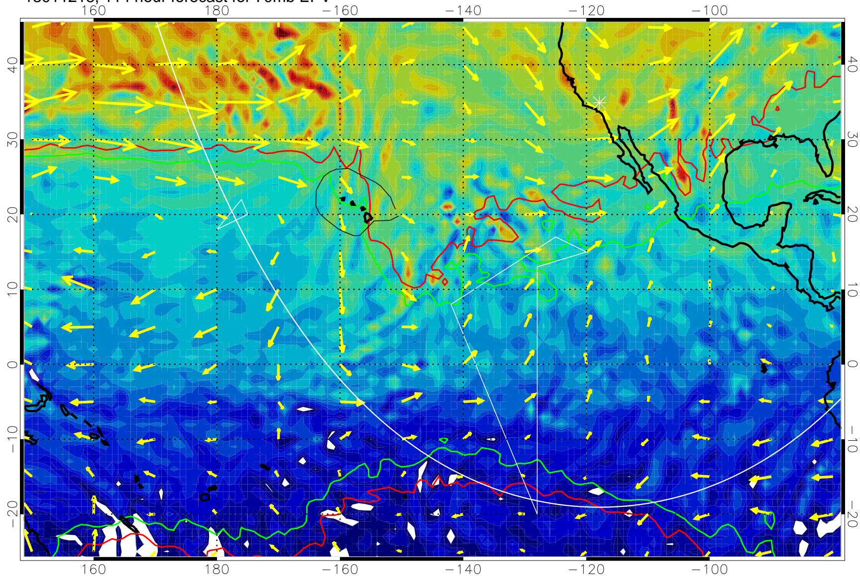
13011218, 114 hour forecast for 70mb EPV
