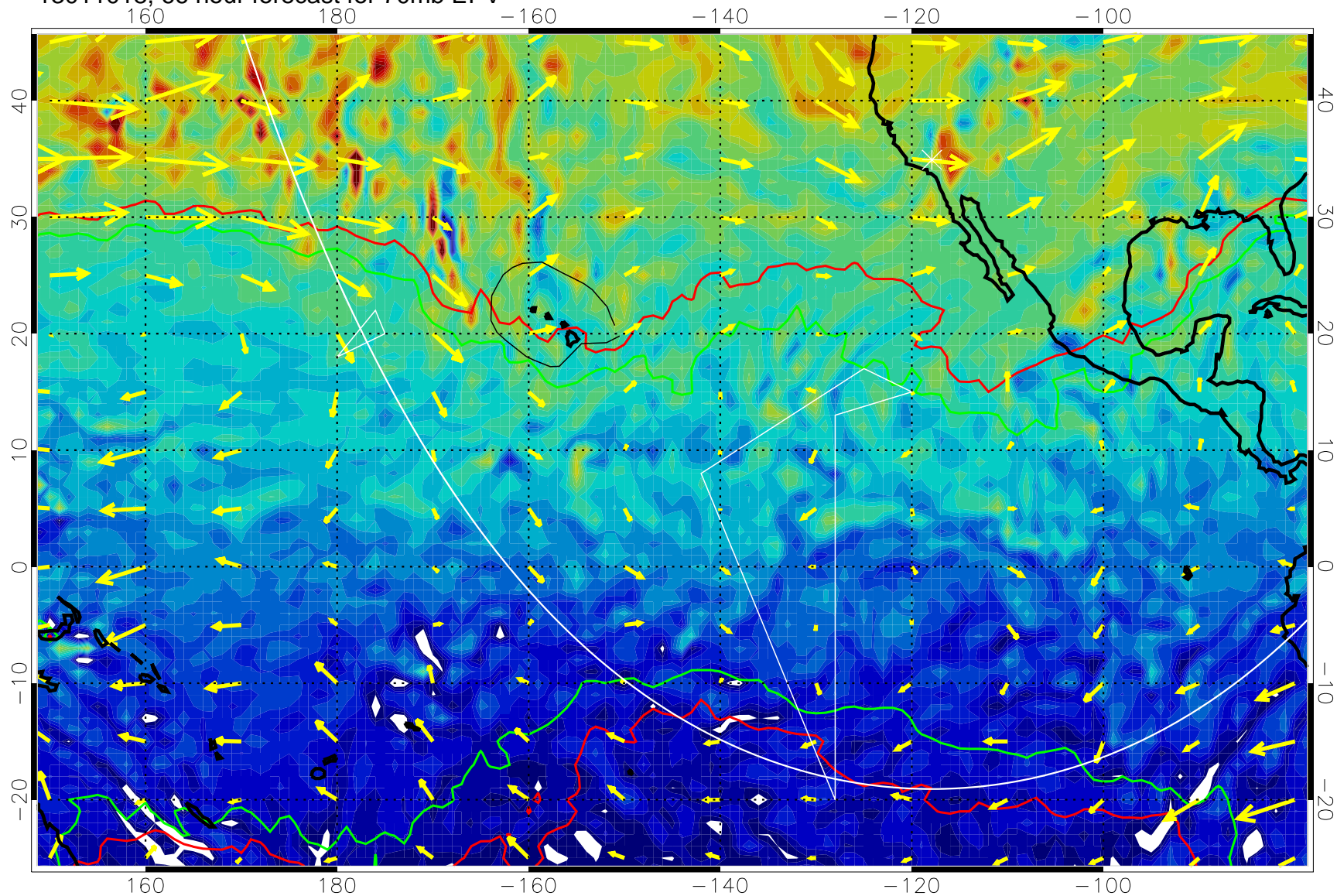
13011018, 66 hour forecast for 70mb EPV
