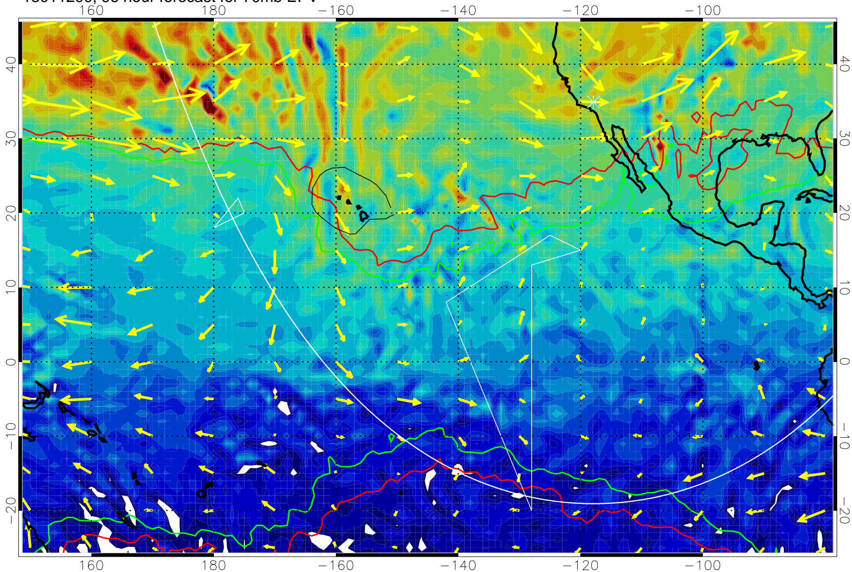
13011200, 96 hour forecast for 70mb EPV
