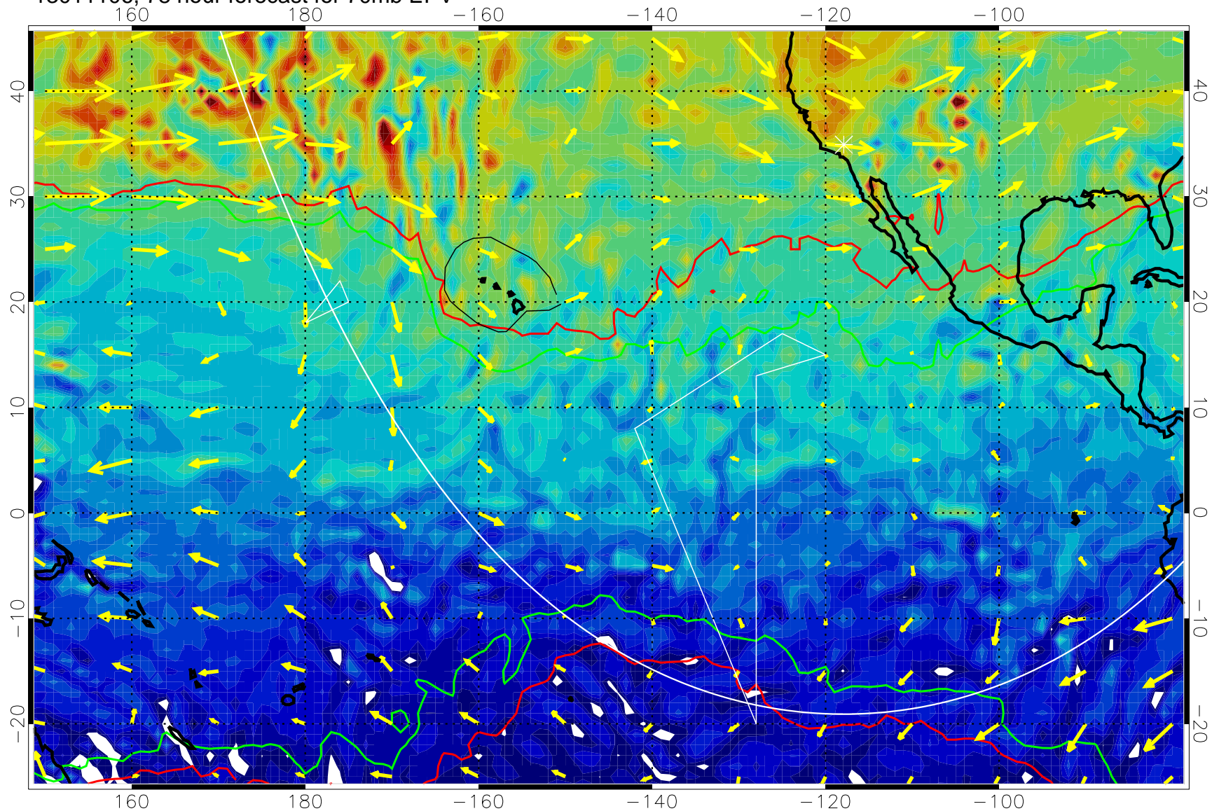
13011106, 78 hour forecast for 70mb EPV
