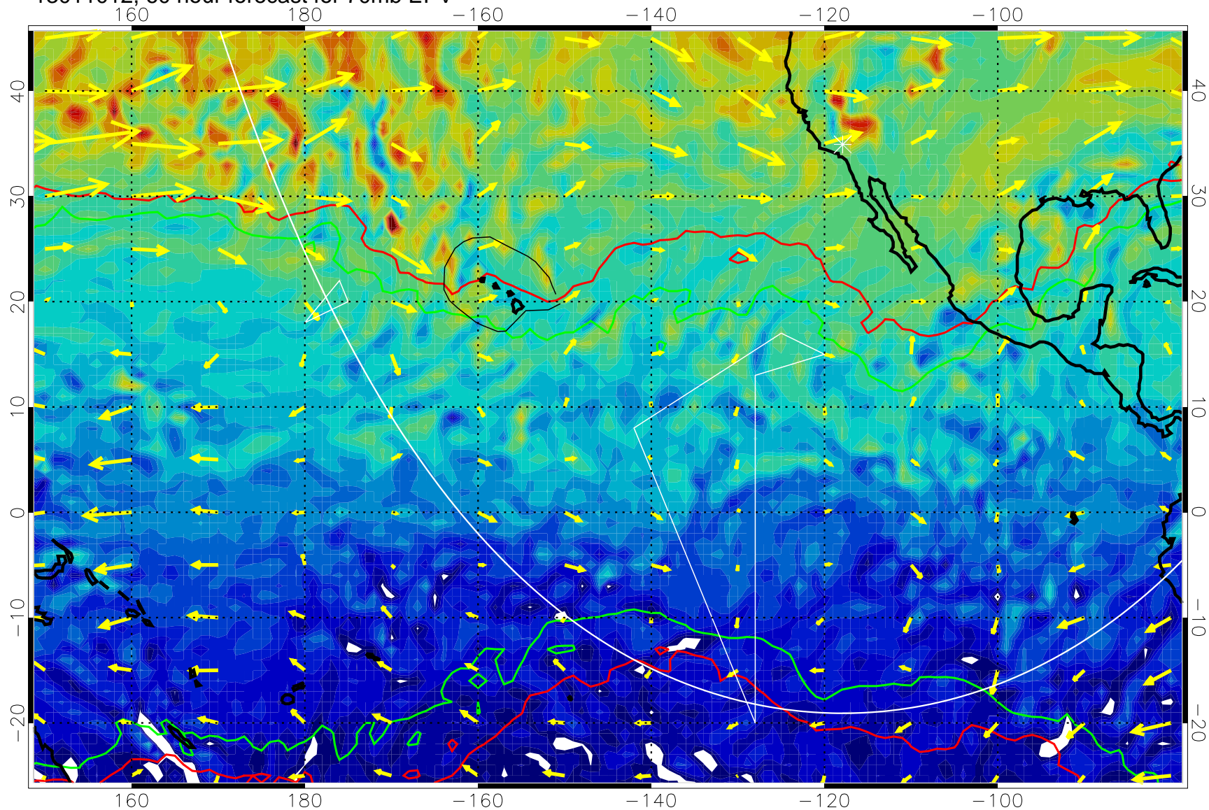
13011012, 60 hour forecast for 70mb EPV
