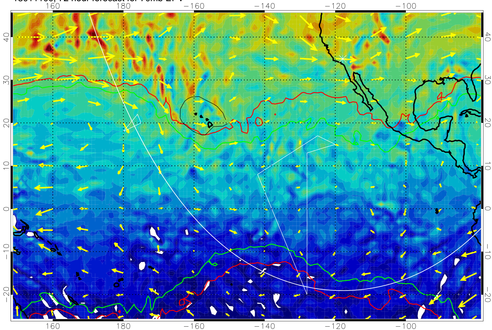
13011100, 72 hour forecast for 70mb EPV
