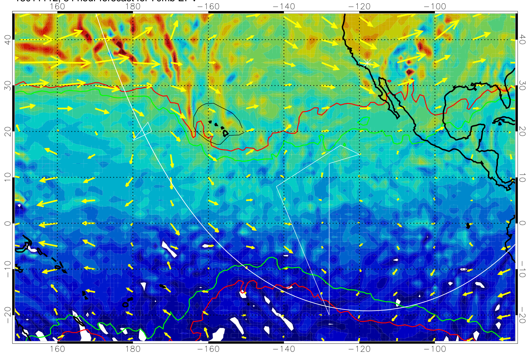
13011112, 84 hour forecast for 70mb EPV
