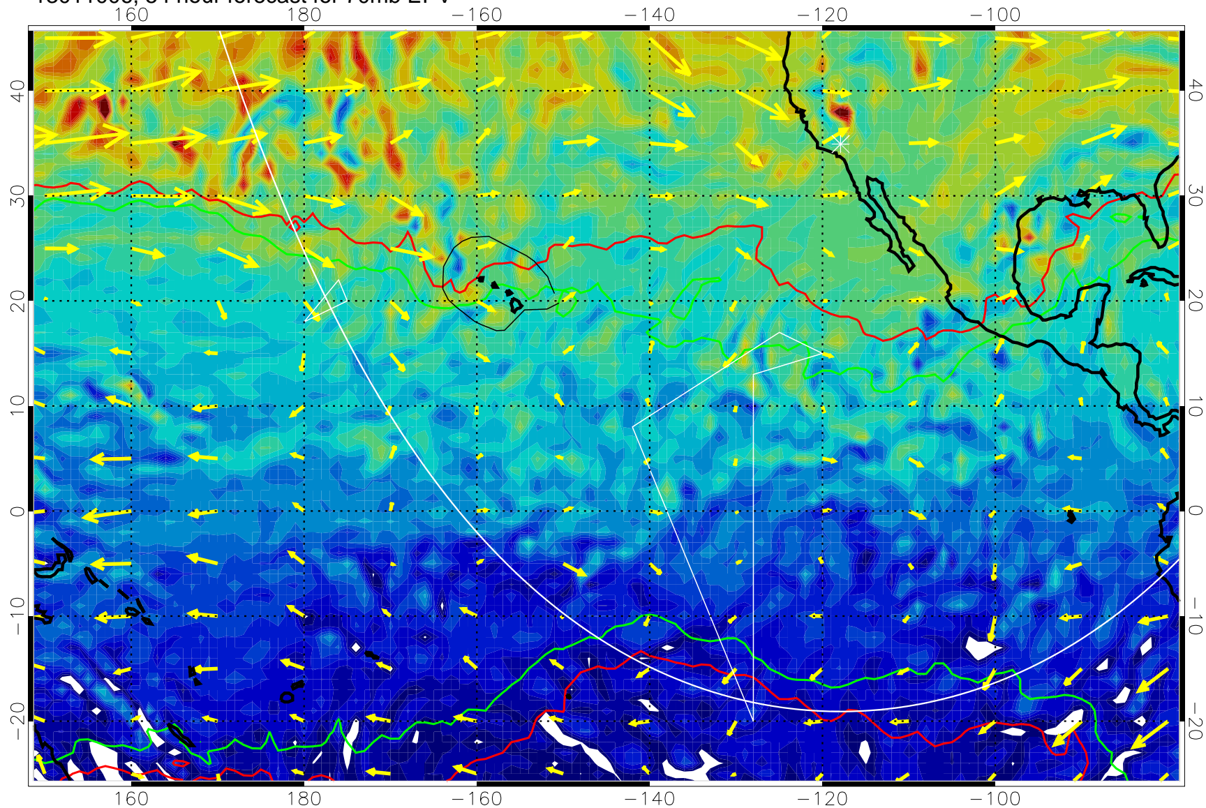
13011006, 54 hour forecast for 70mb EPV
