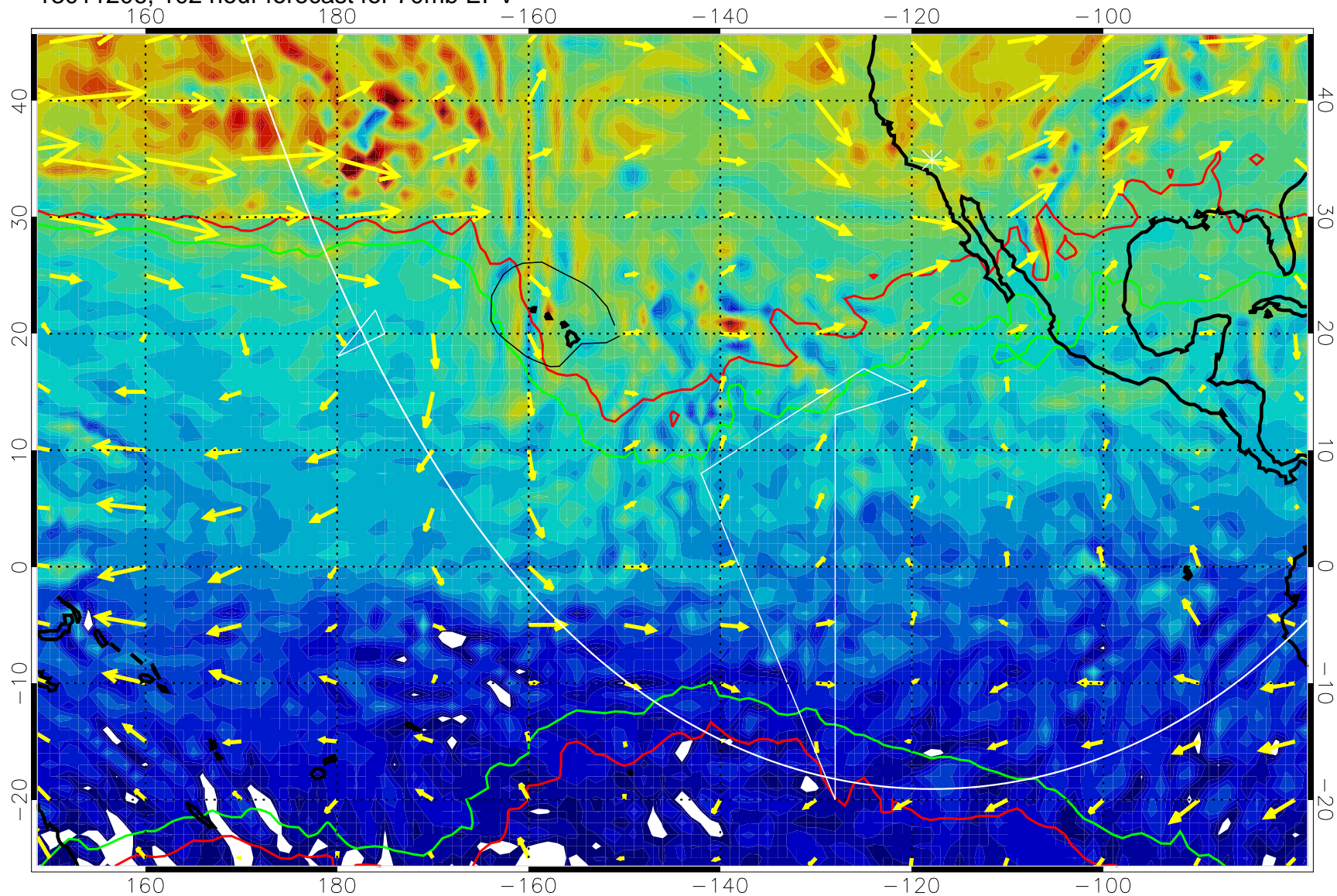
13011206, 102 hour forecast for 70mb EPV
