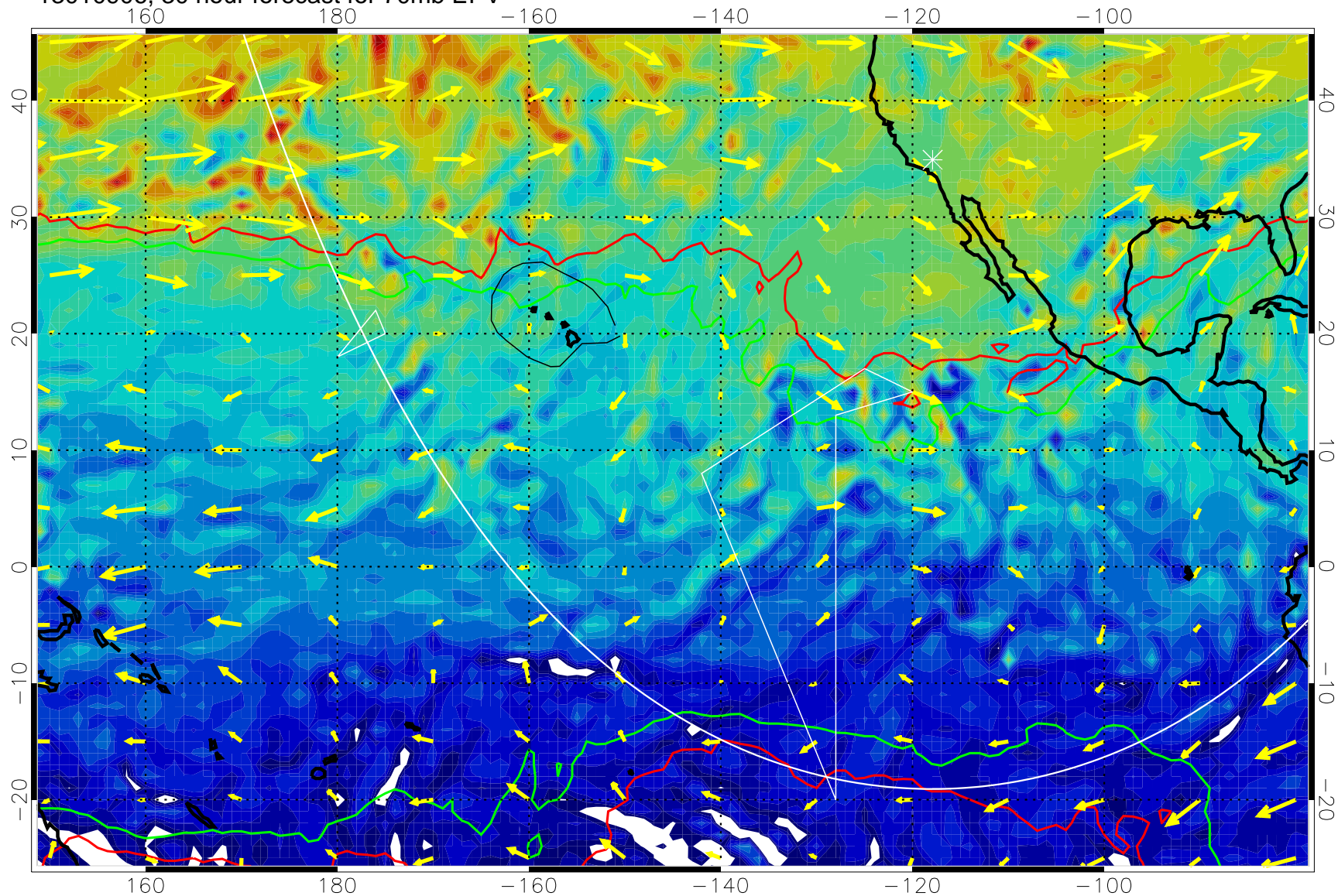
13010906, 30 hour forecast for 70mb EPV
