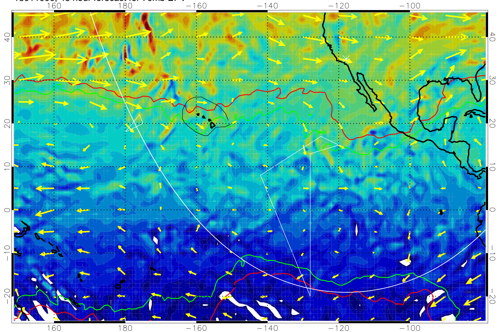
13011000, 48 hour forecast for 70mb EPV
