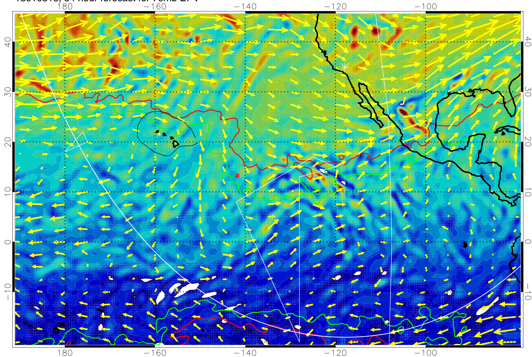
13010818, 54 hour forecast for 70mb EPV
