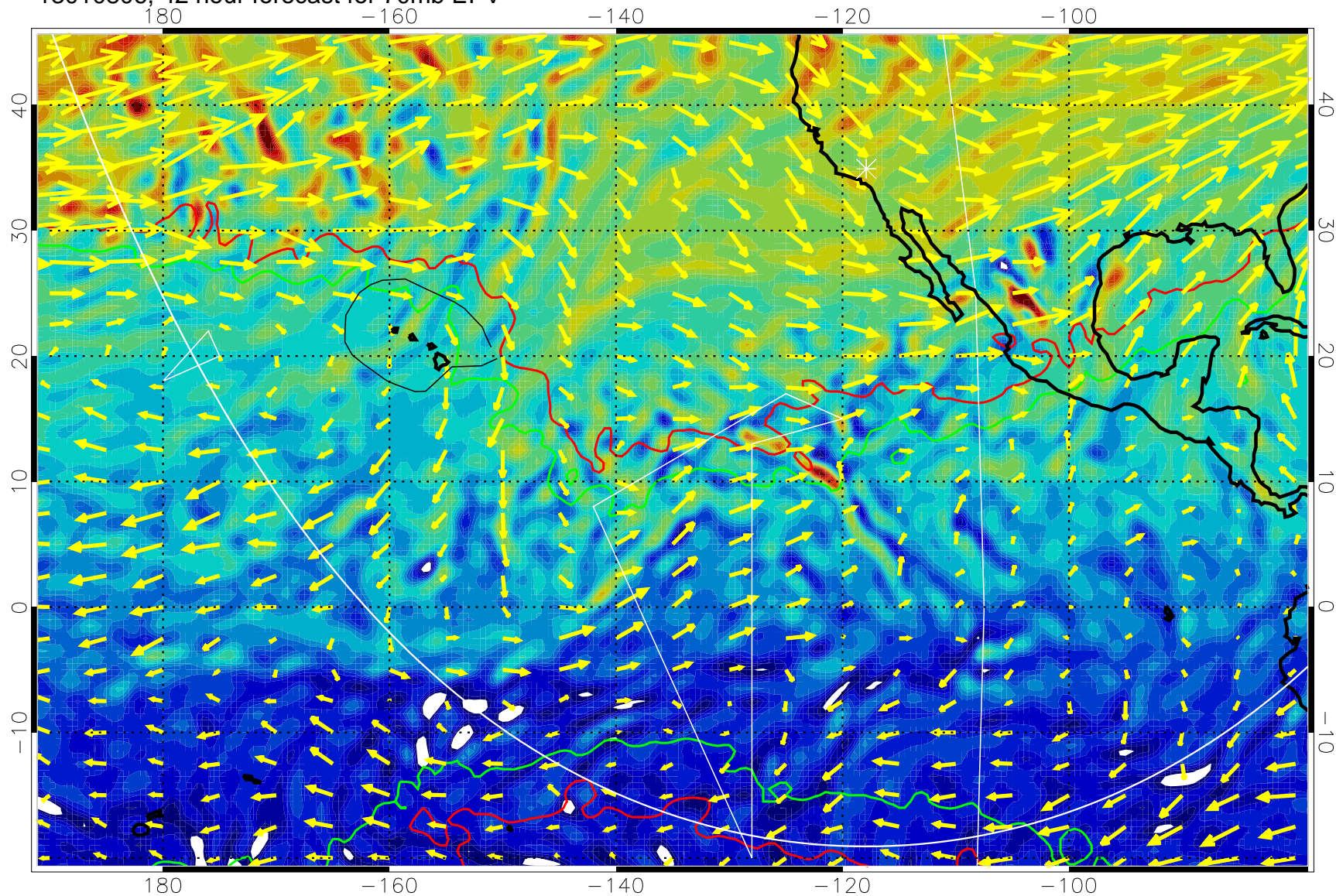
13010806, 42 hour forecast for 70mb EPV
