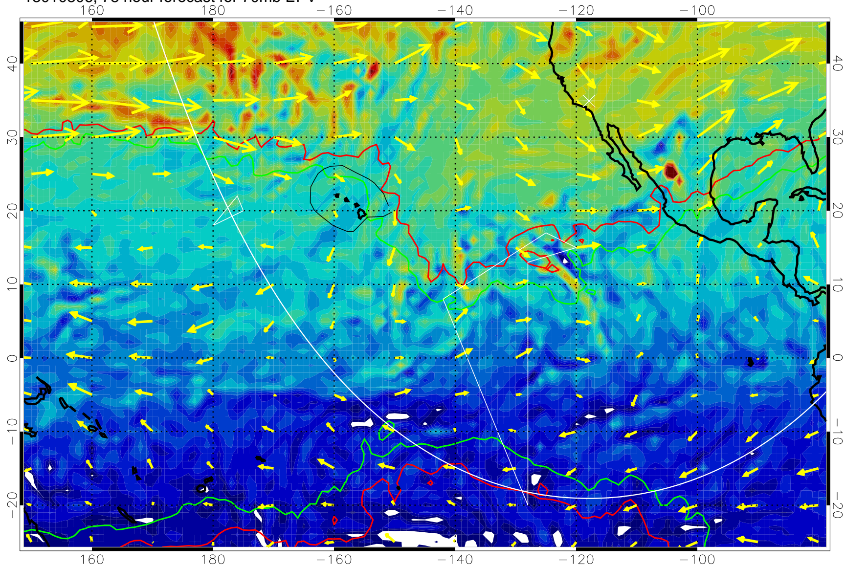
13010806, 78 hour forecast for 70mb EPV
