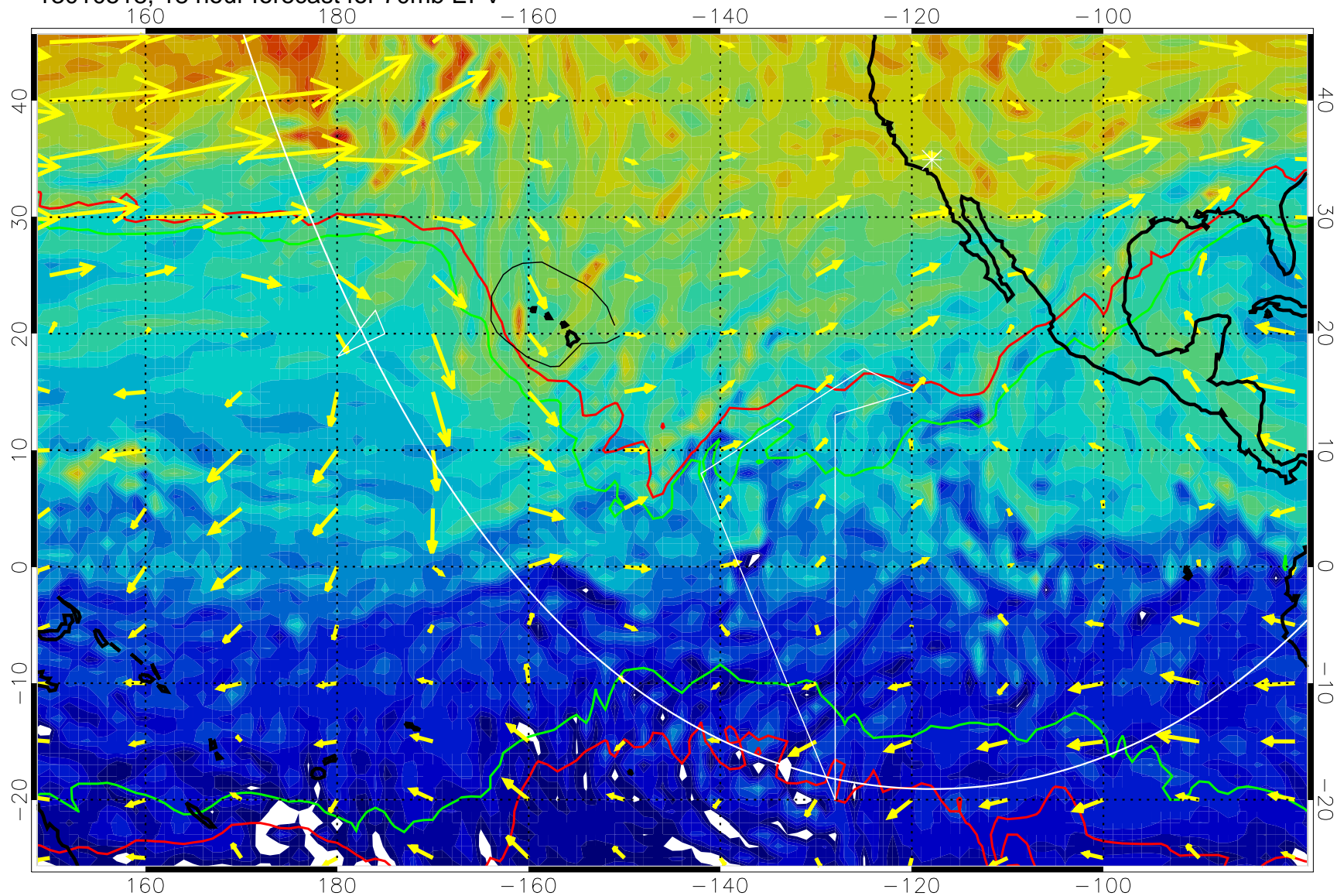
13010518, 18 hour forecast for 70mb EPV
