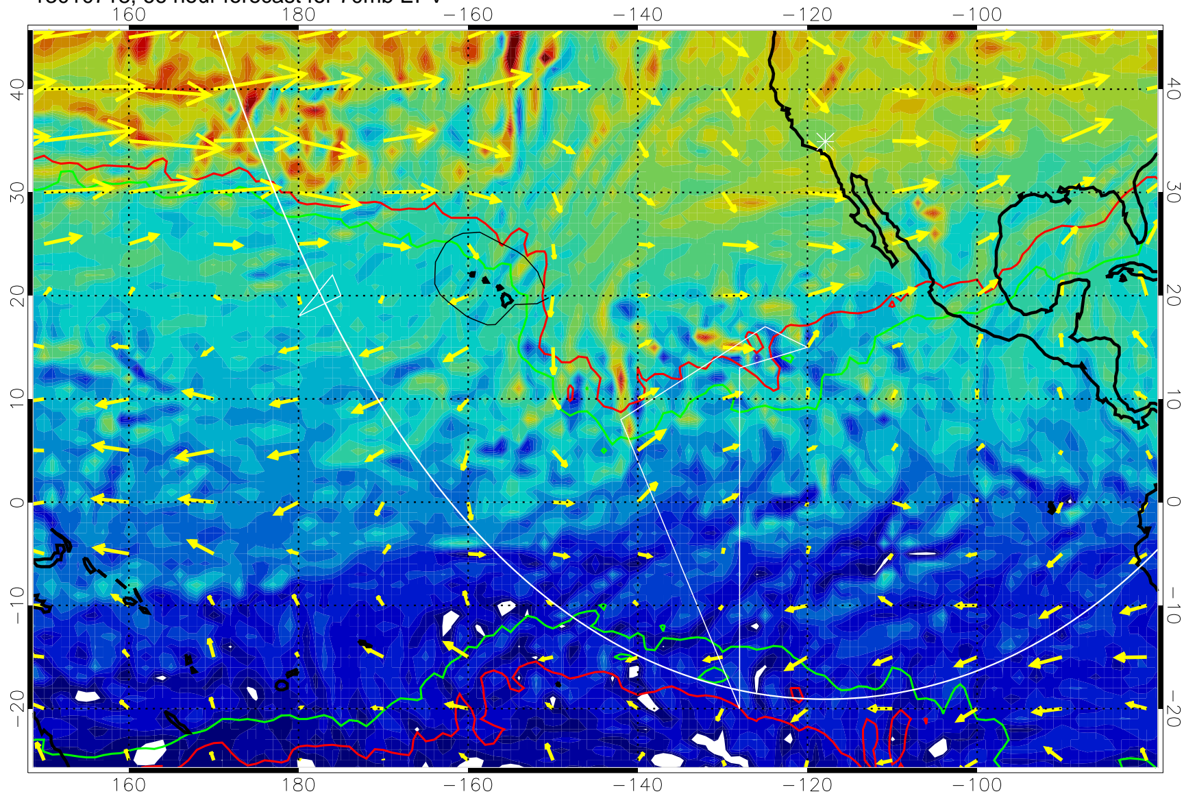
13010718, 66 hour forecast for 70mb EPV
