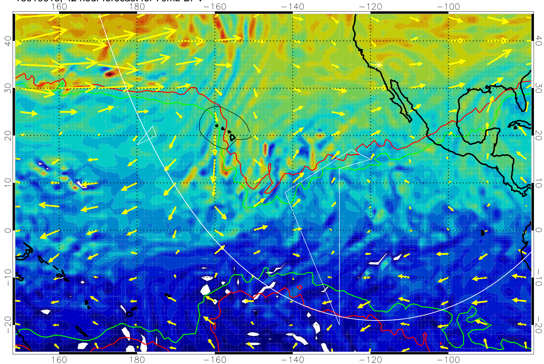
13010618, 42 hour forecast for 70mb EPV
