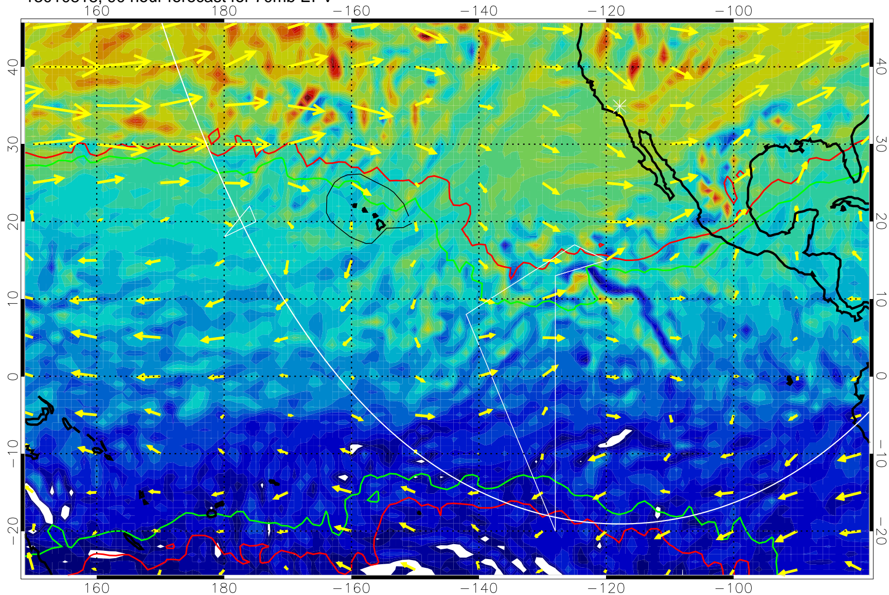
13010818, 90 hour forecast for 70mb EPV
