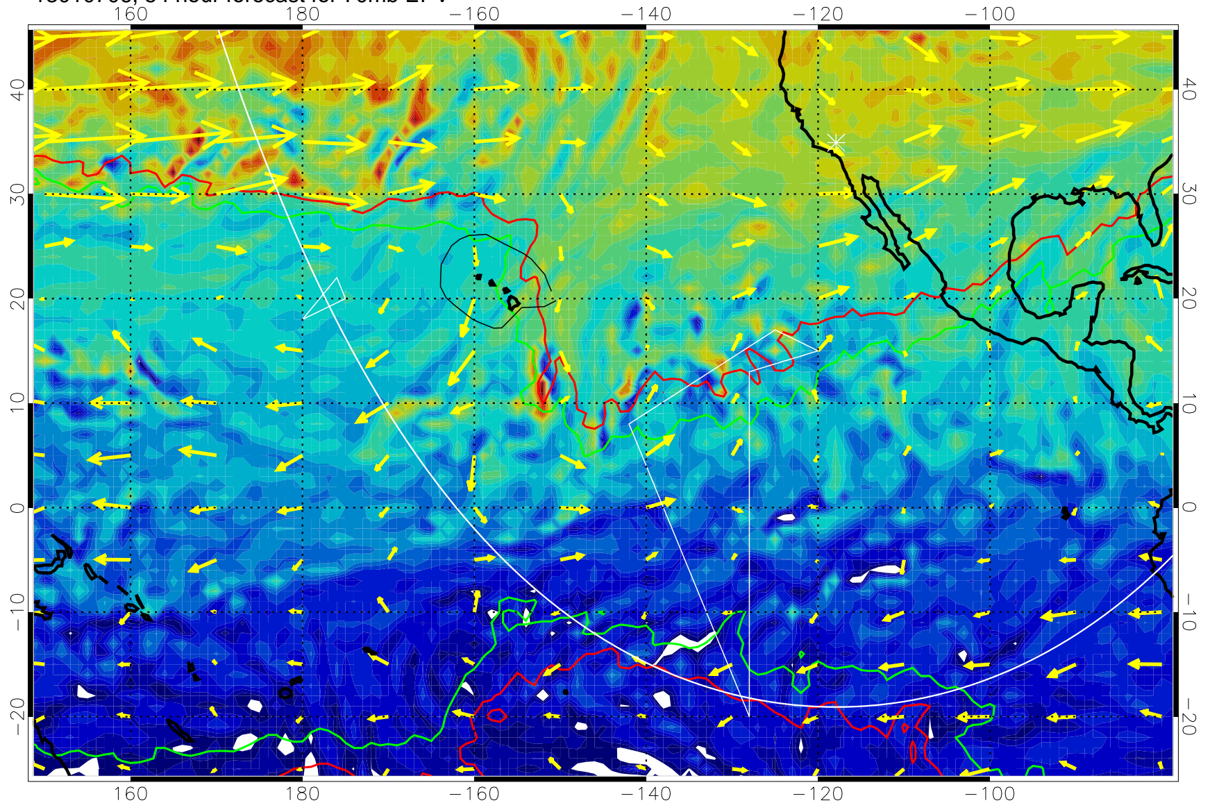
13010706, 54 hour forecast for 70mb EPV
