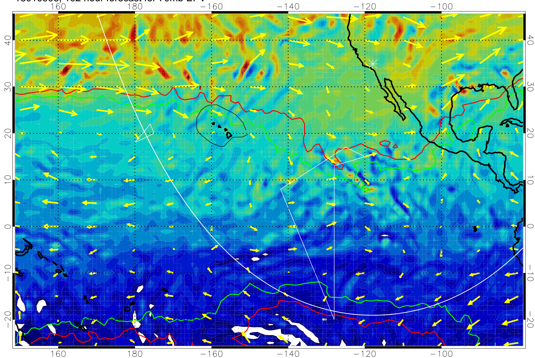
13010906, 102 hour forecast for 70mb EPV
