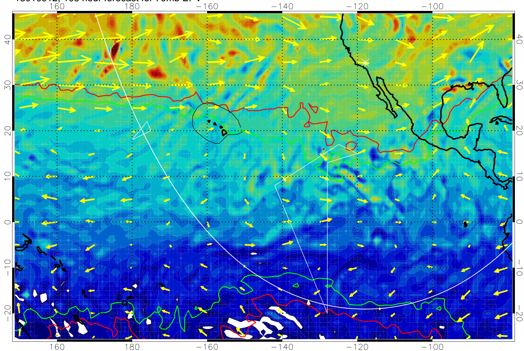
13010912, 108 hour forecast for 70mb EPV
