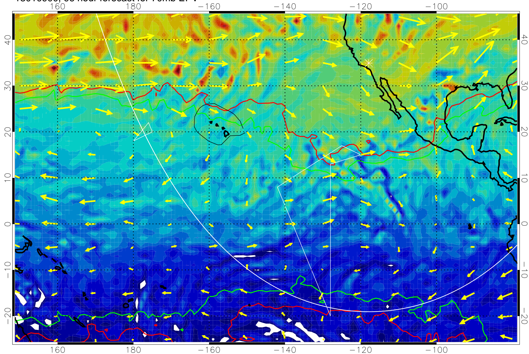
13010900, 96 hour forecast for 70mb EPV
