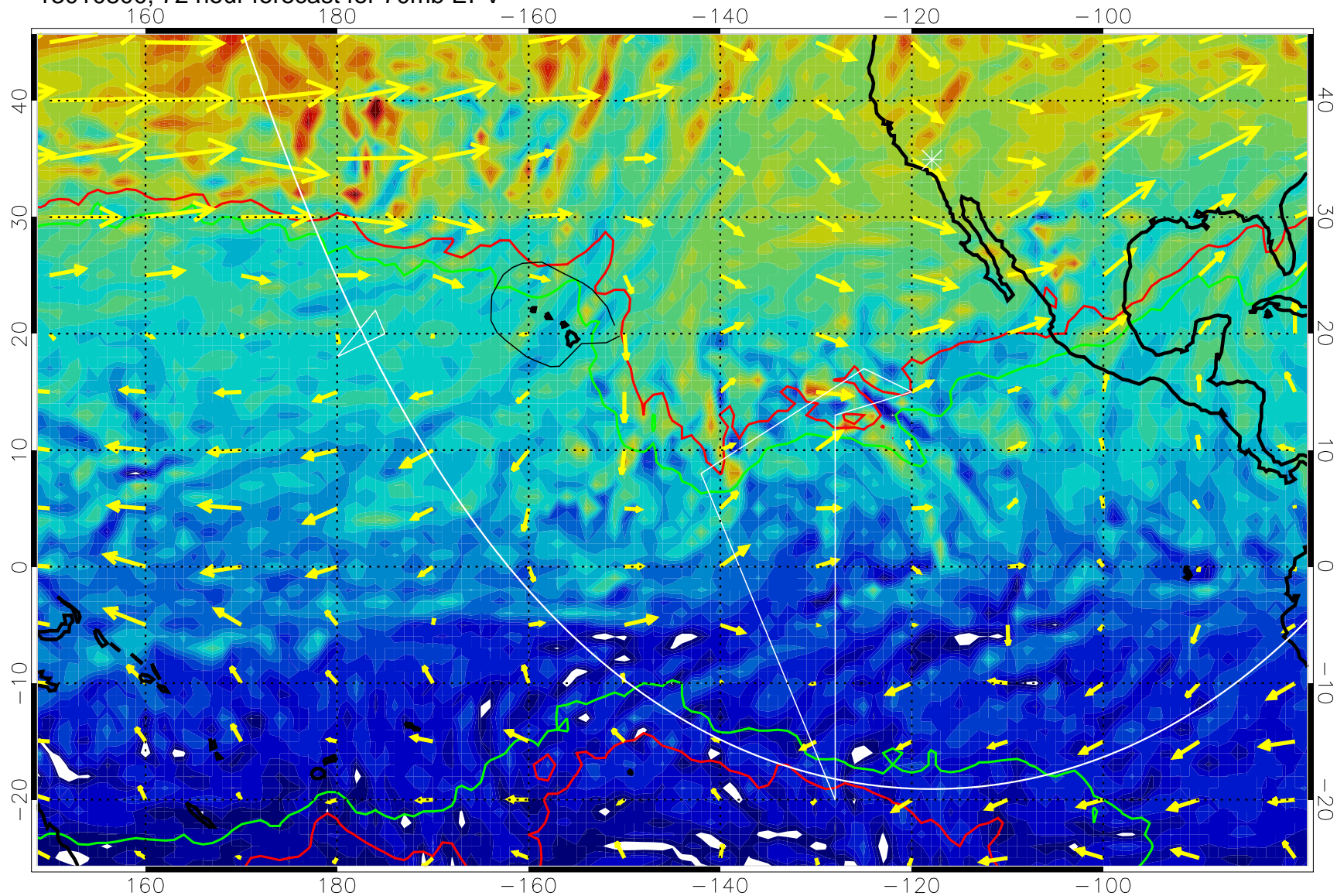
13010800, 72 hour forecast for 70mb EPV
