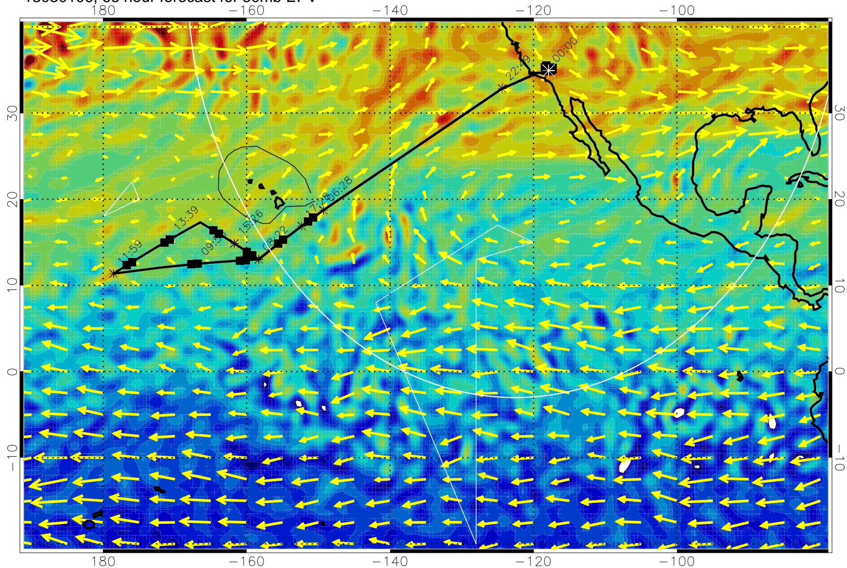
13030106, 66 hour forecast for 50mb EPV
