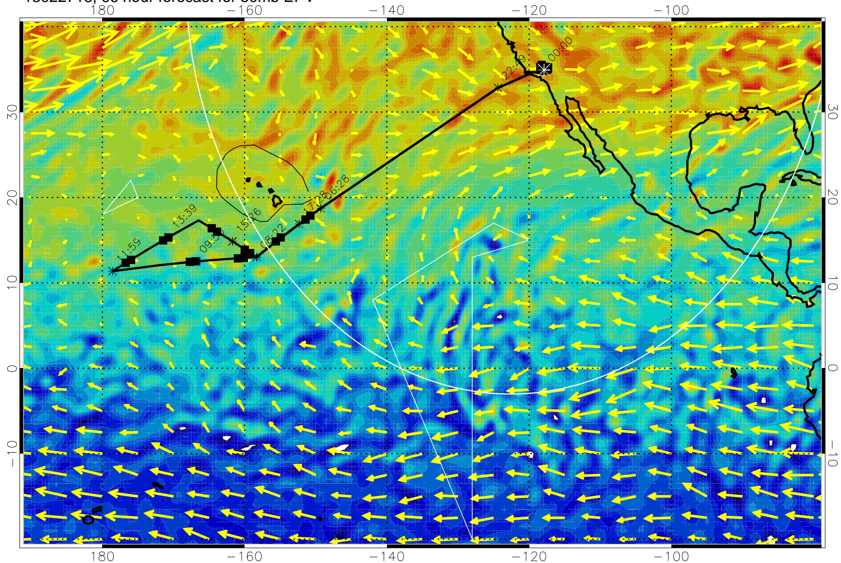
13022718, 66 hour forecast for 50mb EPV
