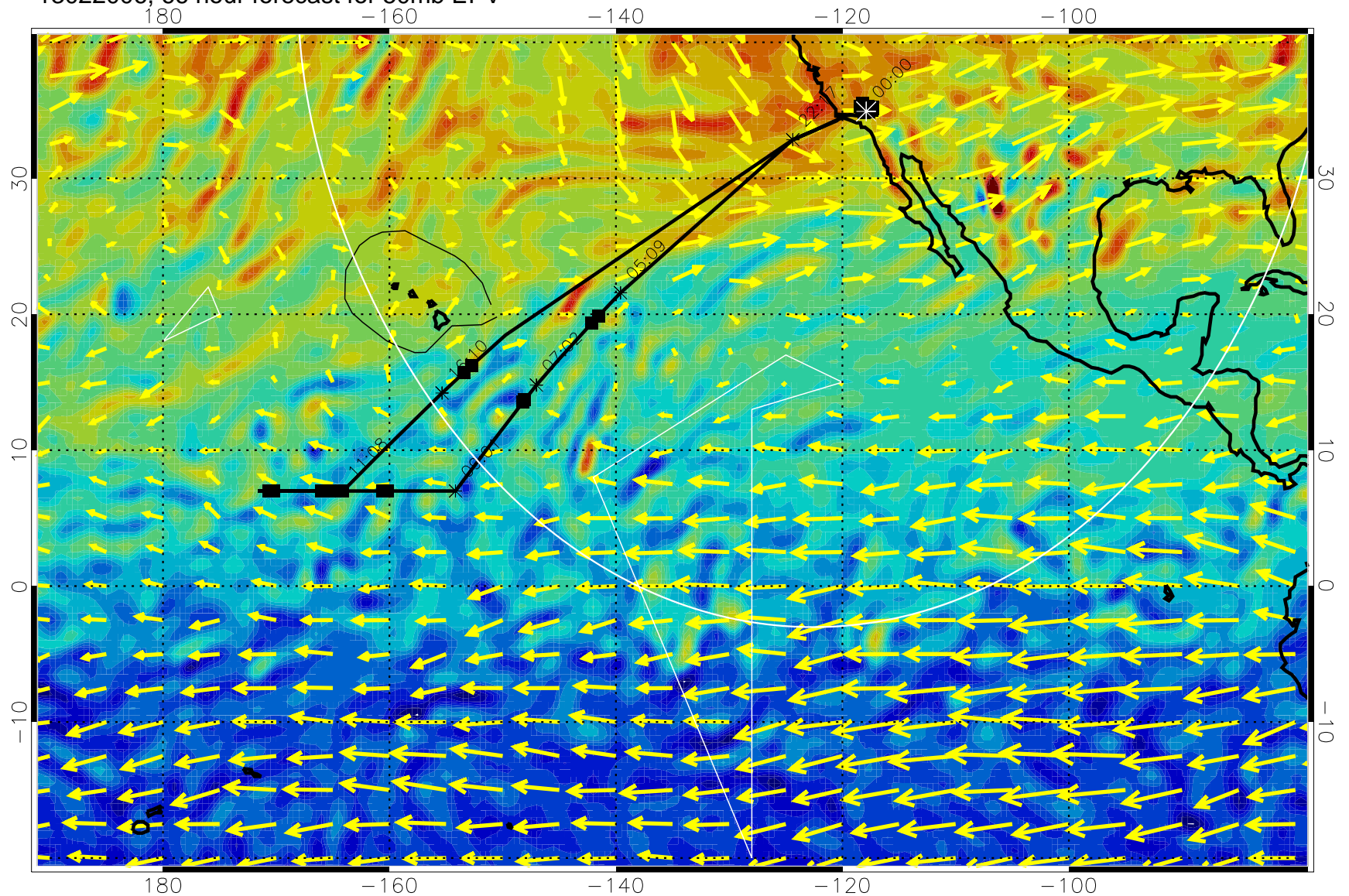
13022006, 66 hour forecast for 50mb EPV
