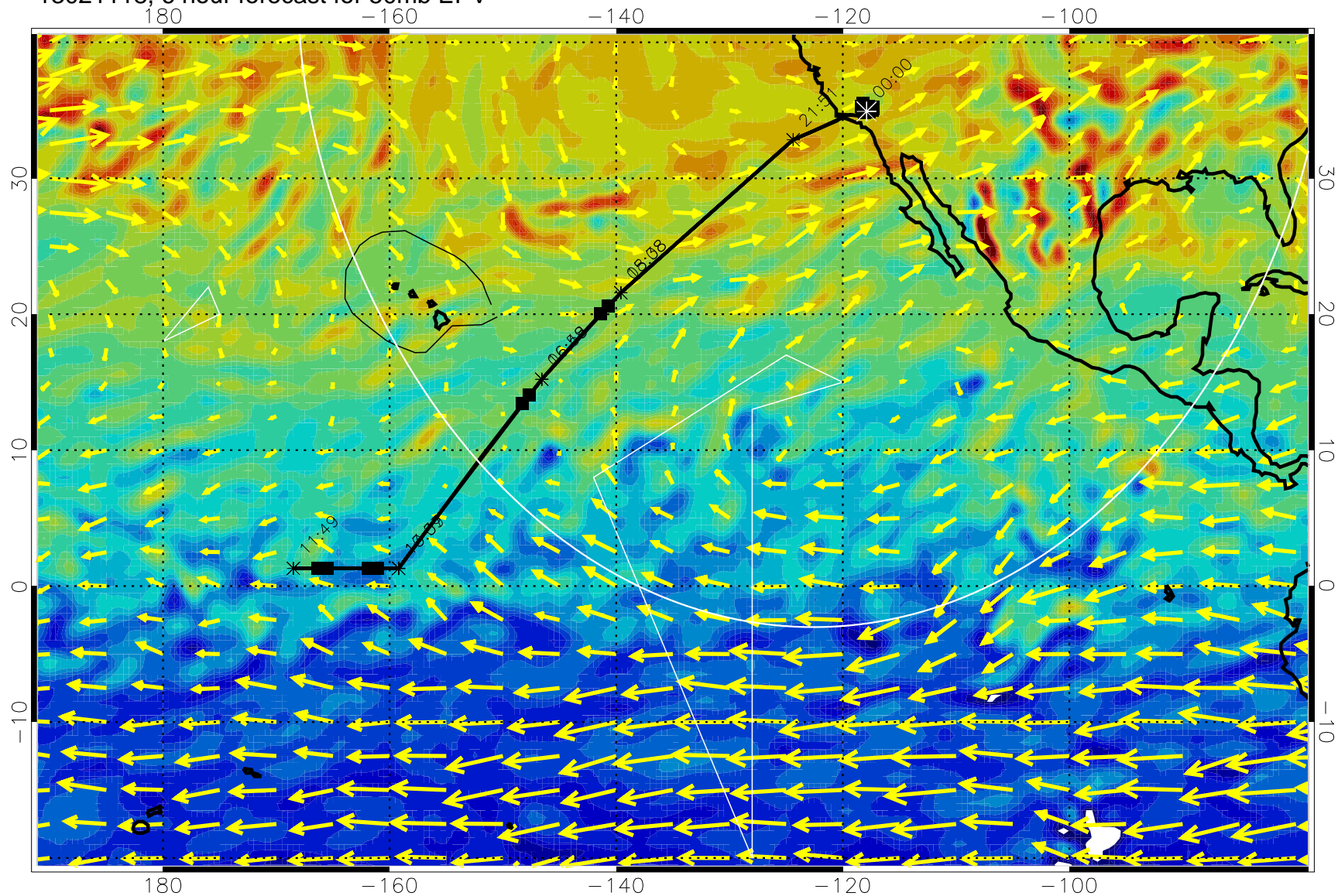
13021118, 6 hour forecast for 50mb EPV
