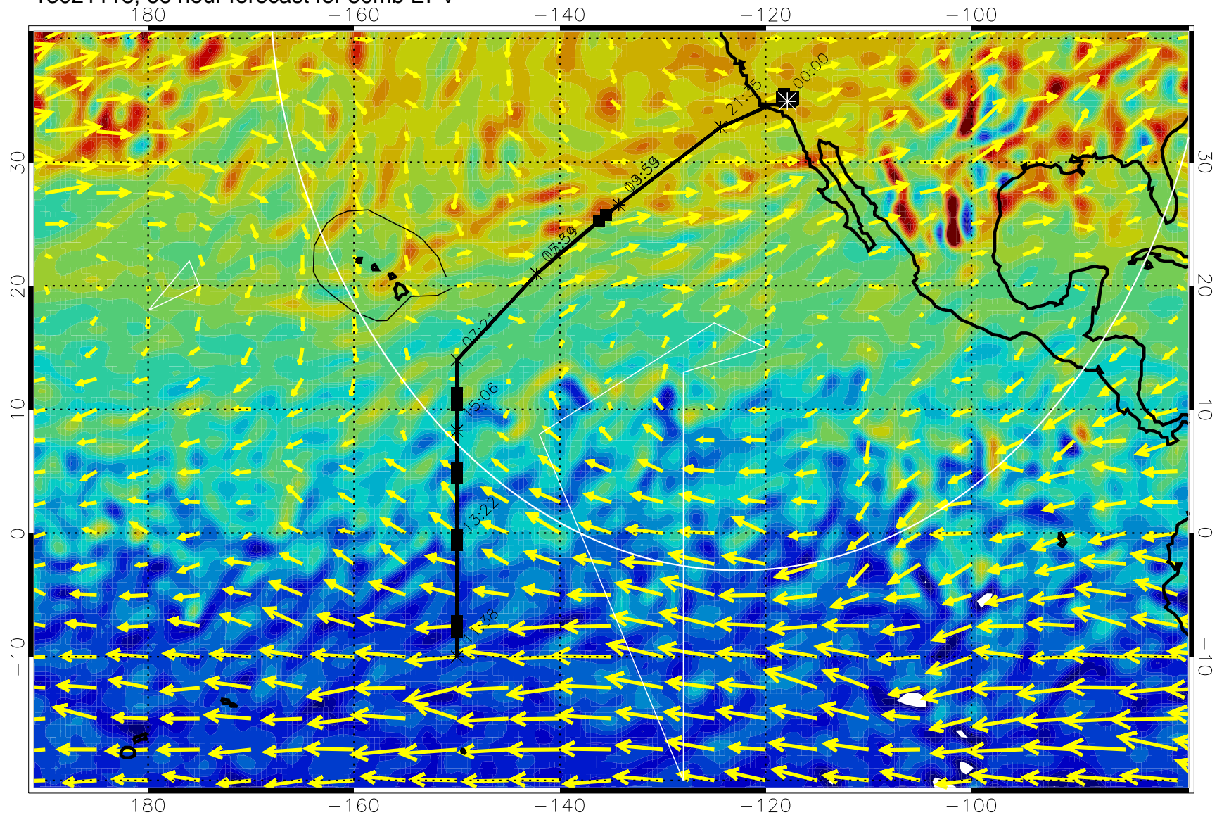
13021118, 66 hour forecast for 50mb EPV
