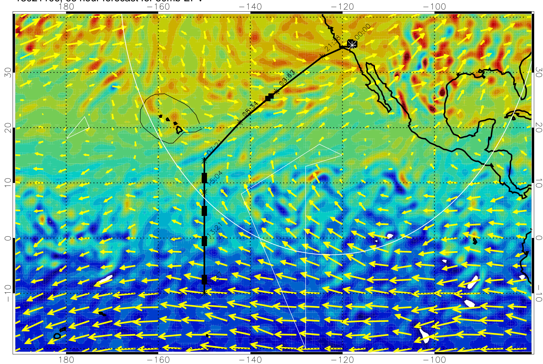
13021106, 66 hour forecast for 50mb EPV
