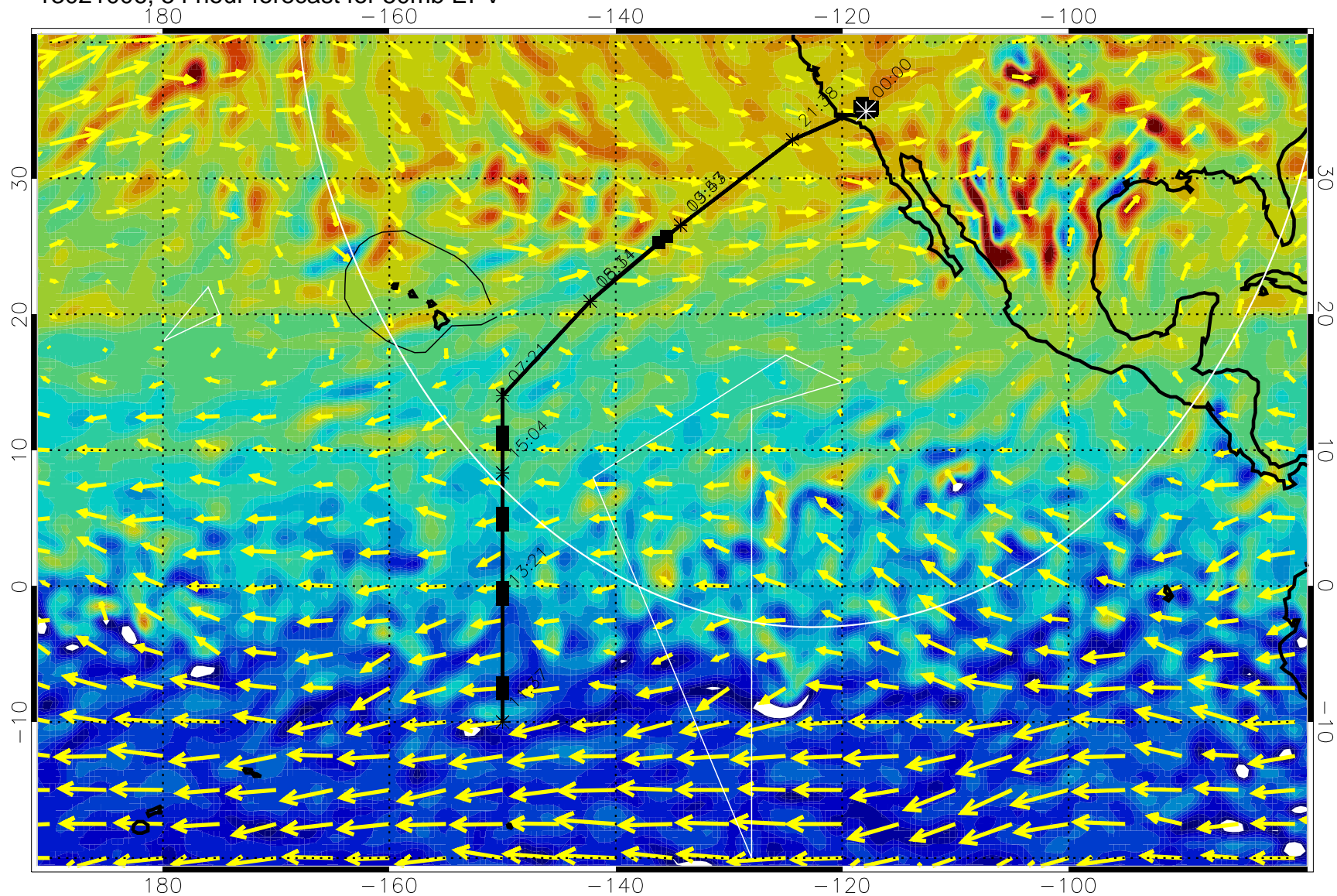
13021006, 54 hour forecast for 50mb EPV
