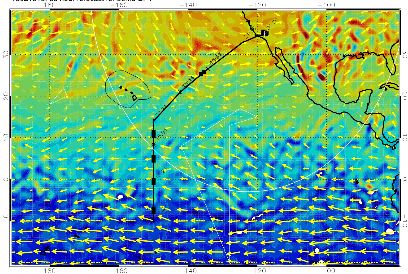
13021018, 66 hour forecast for 50mb EPV
