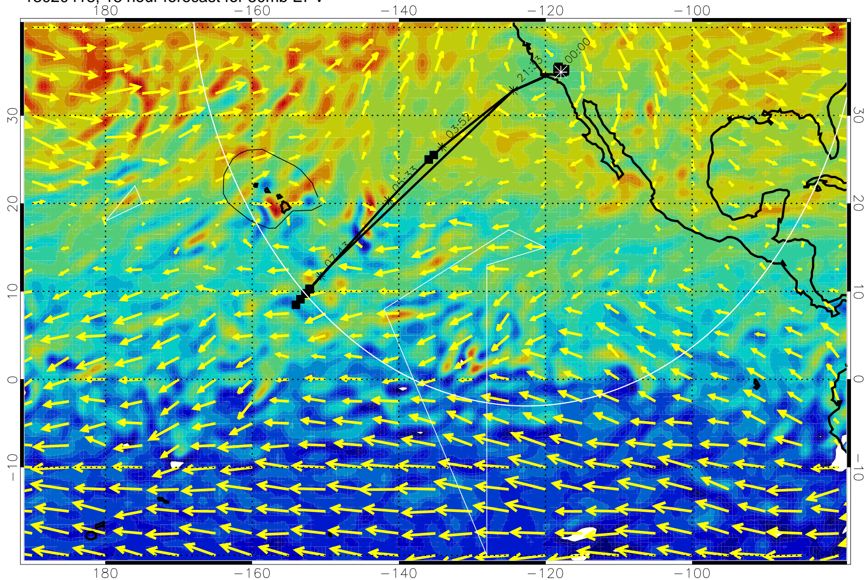
13020418, 18 hour forecast for 50mb EPV
