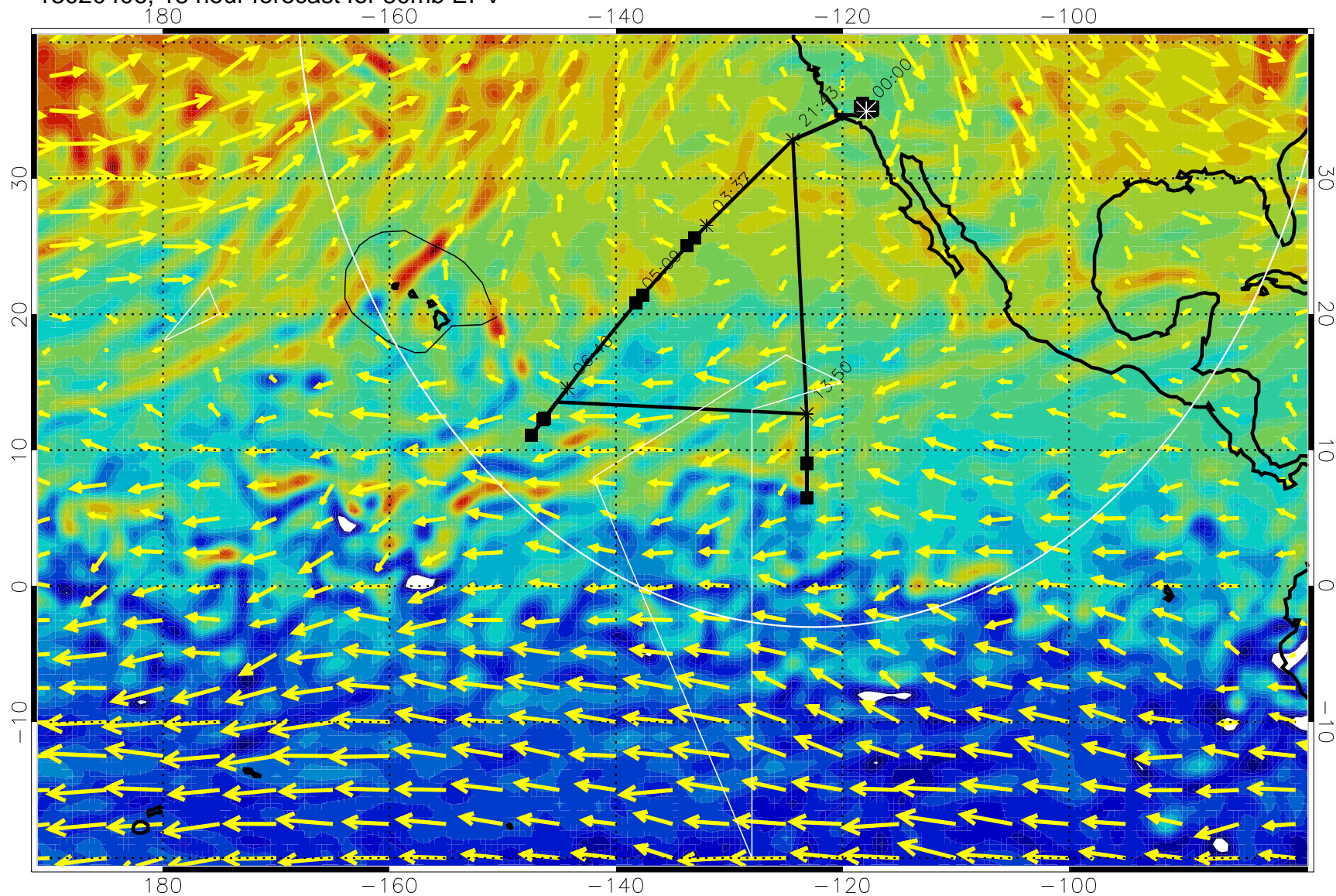
13020406, 18 hour forecast for 50mb EPV
