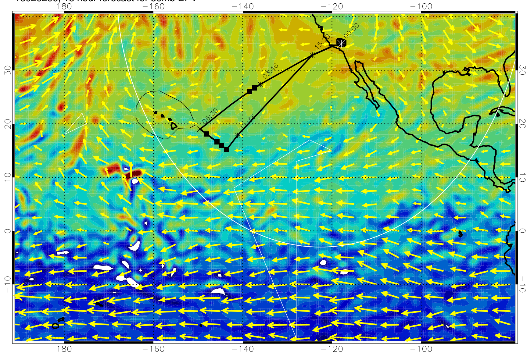
13020206, 18 hour forecast for 50mb EPV
