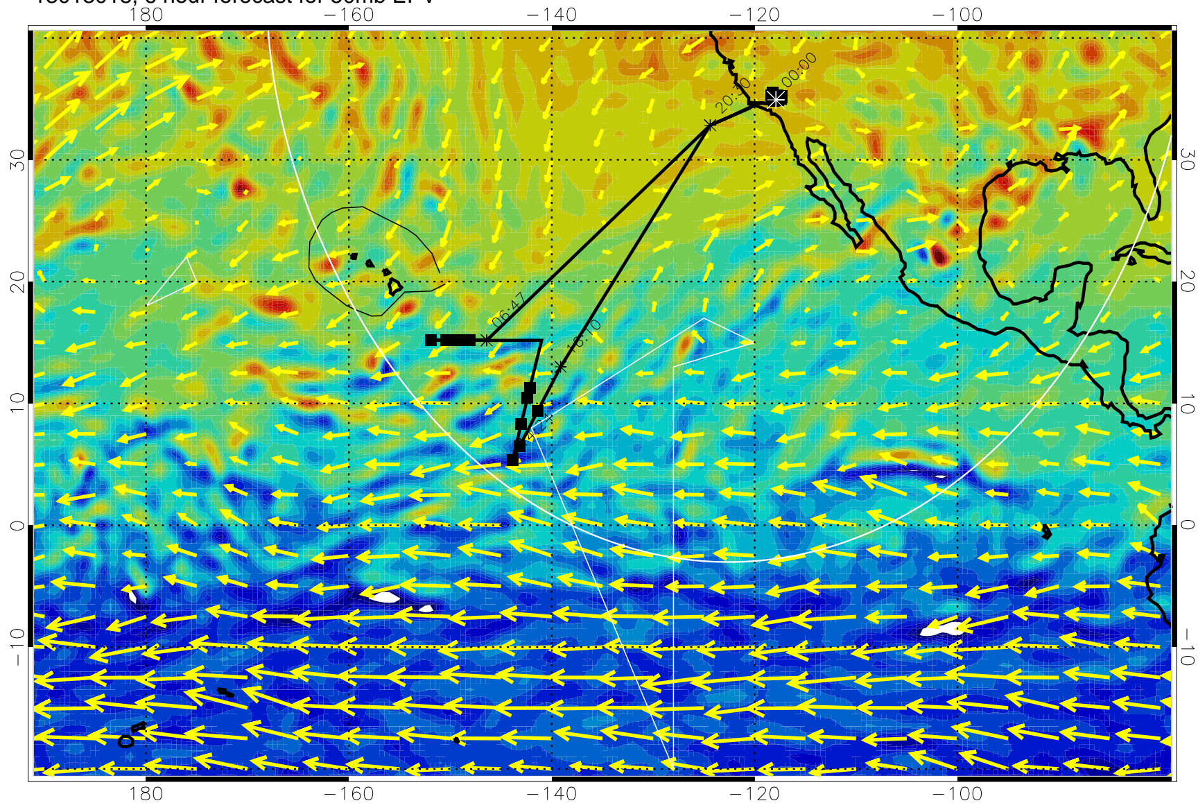
13013018, 6 hour forecast for 50mb EPV
