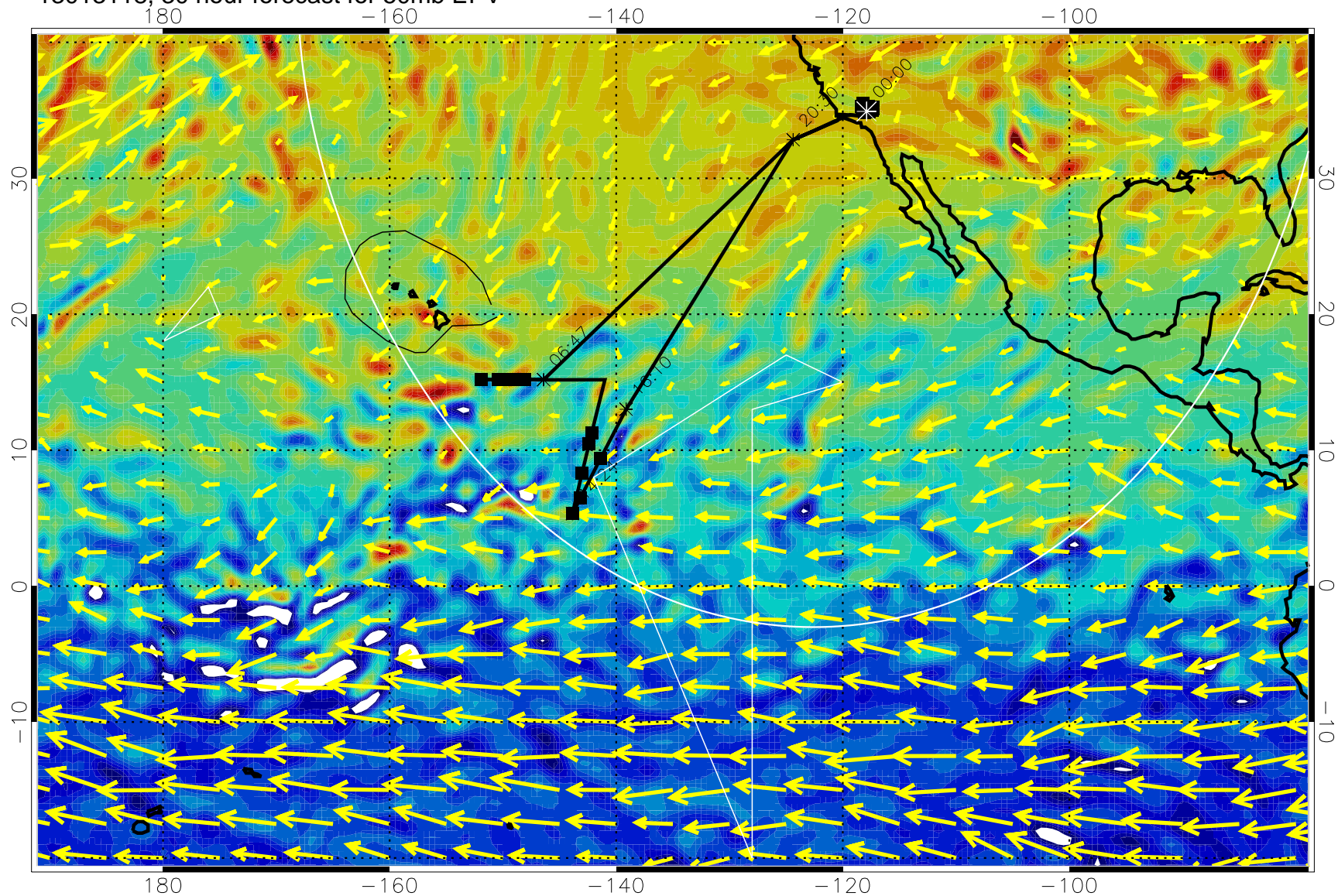
13013118, 30 hour forecast for 50mb EPV
