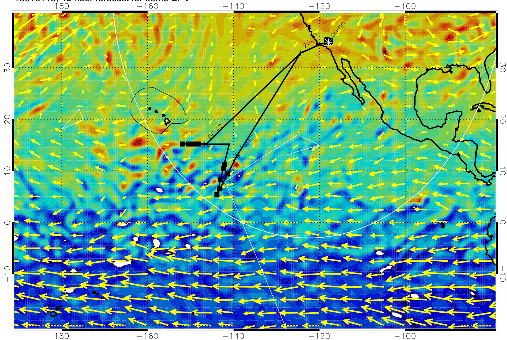
13013118, 42 hour forecast for 50mb EPV
