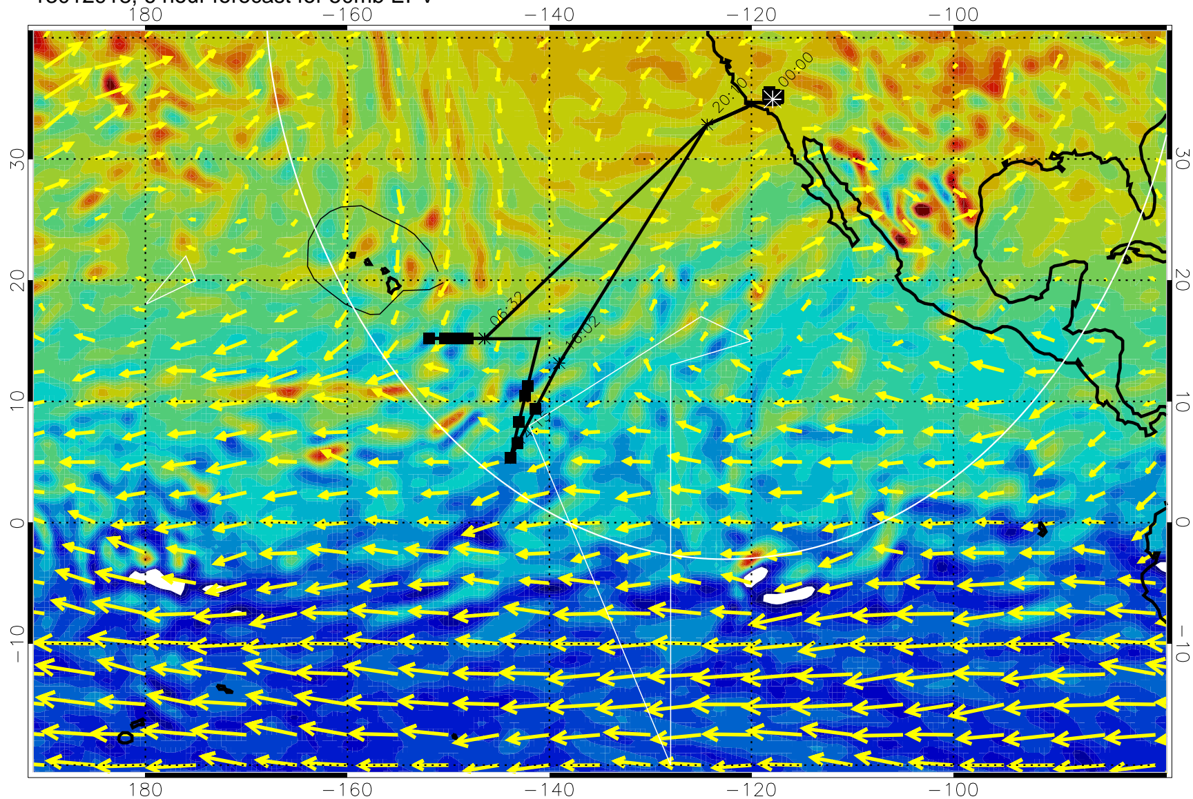
13012918, 6 hour forecast for 50mb EPV
